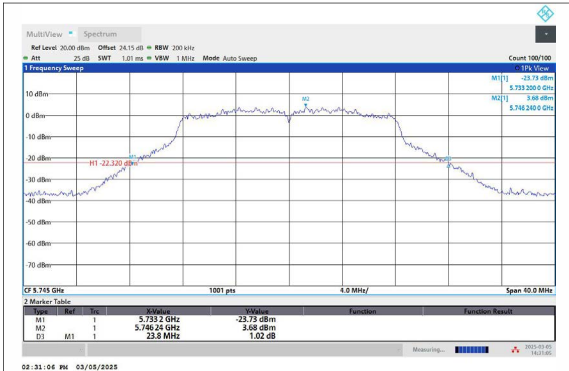
11A-Ant2-5745
