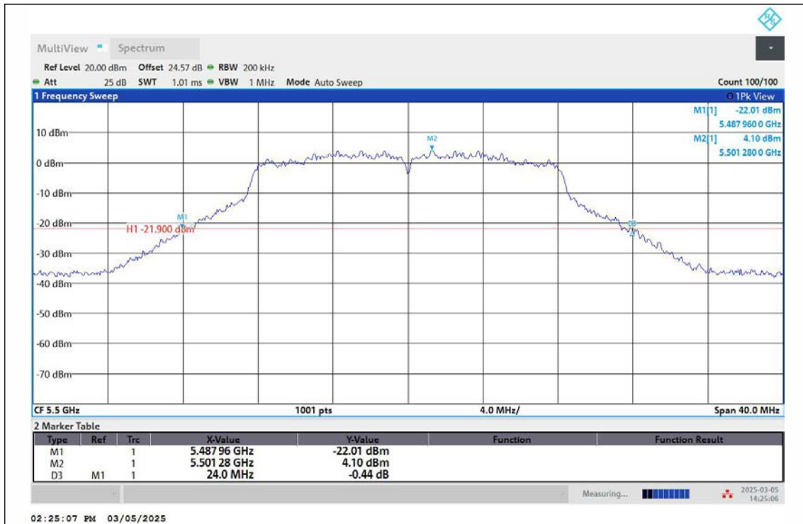
11A-Ant2-5500
