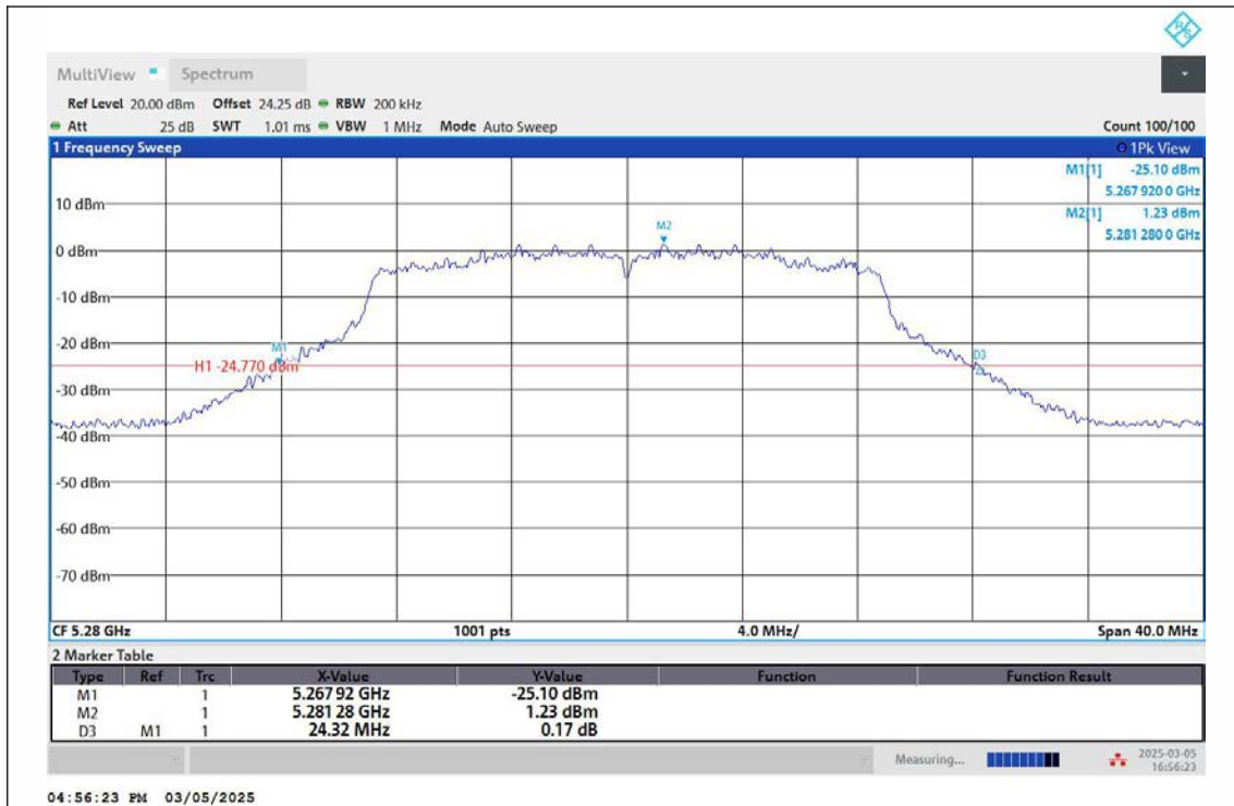
11AC20MIMO-Ant2-5280
