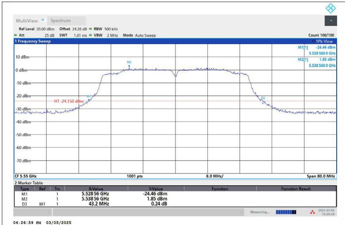
11N40MIMO-Ant2-5550
