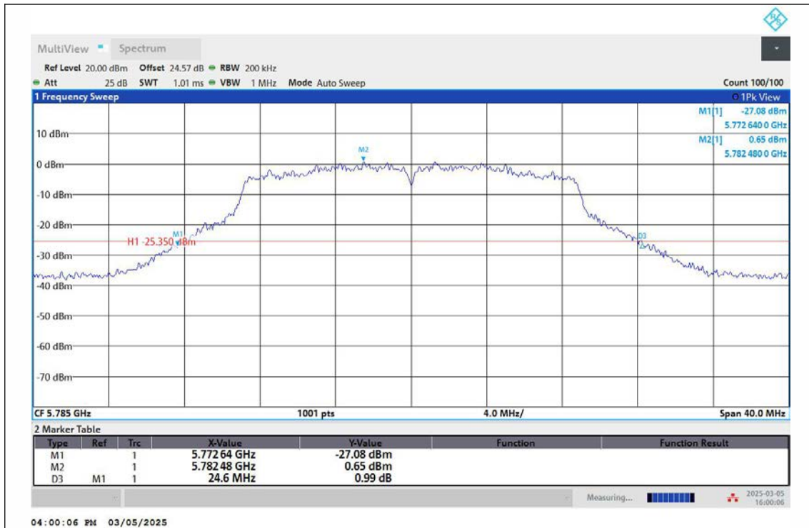
11N20MIMO-Ant2-5785
