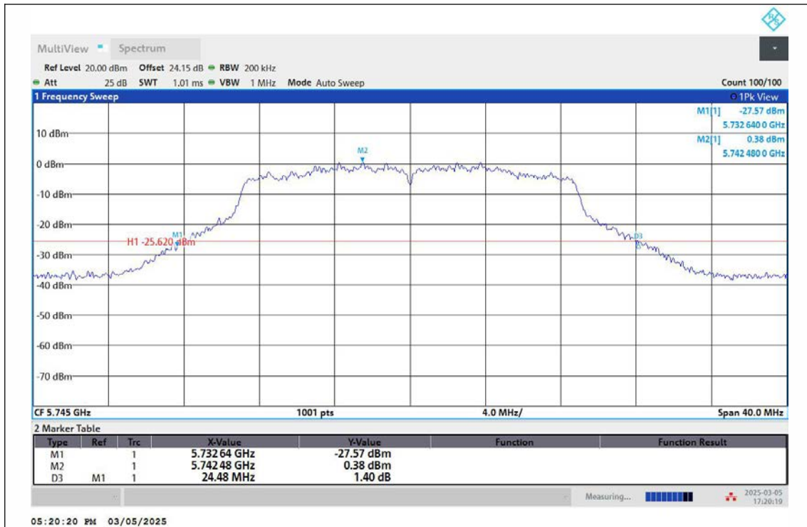
11AC20MIMO-Ant2-5745
