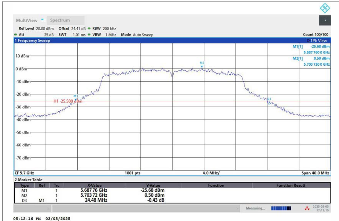
11AC20MIMO-Ant2-5700
