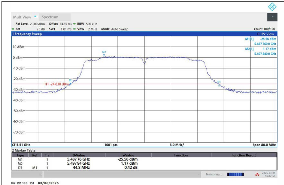
11N40MIMO-Ant2-5510
