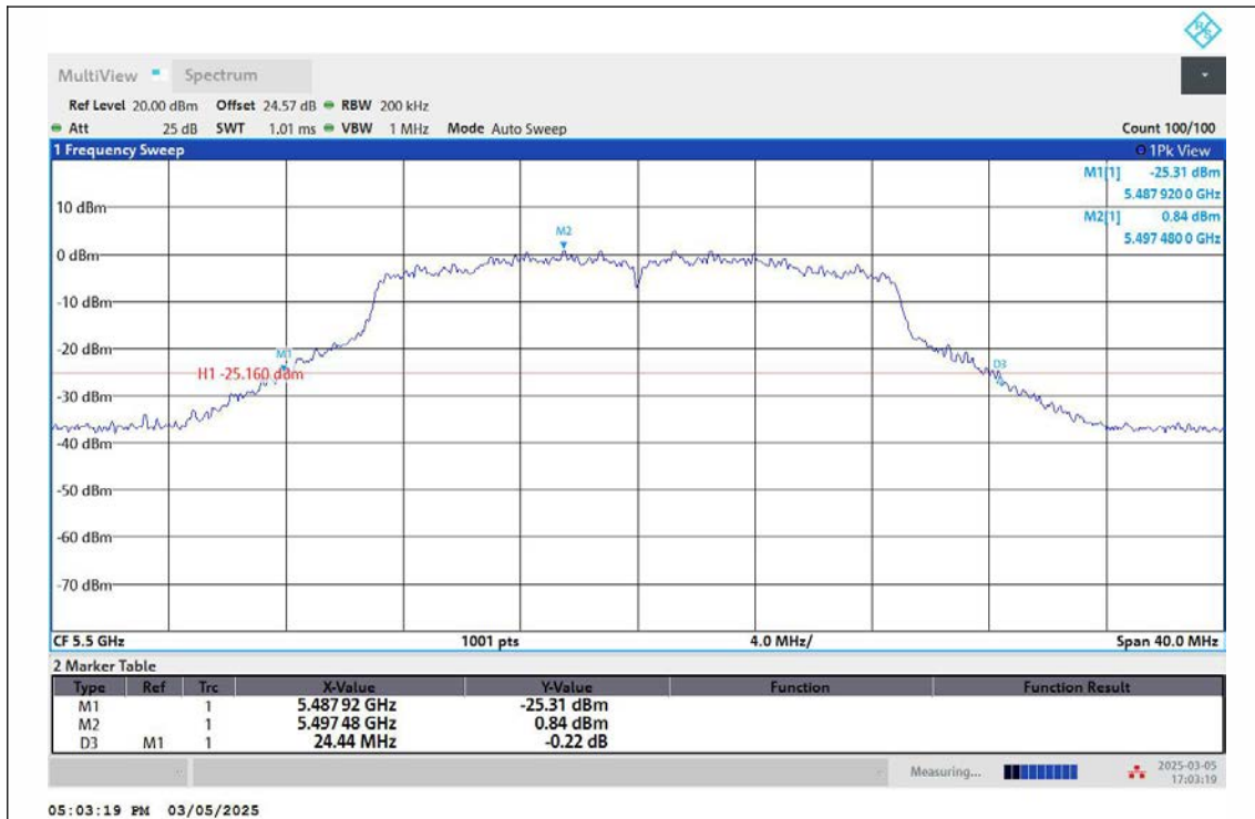
11AC20MIMO-Ant2-5500
