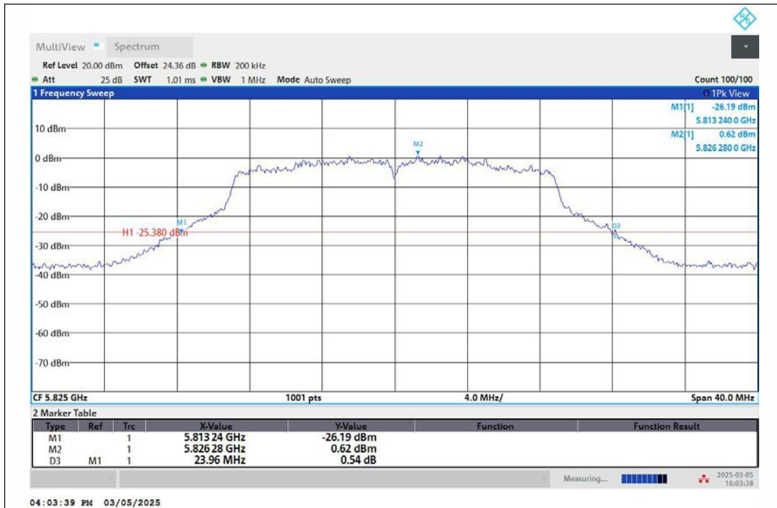
11N20MIMO-Ant2-5825
