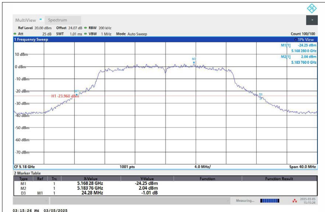
11N20MIMO-Ant2-5180
