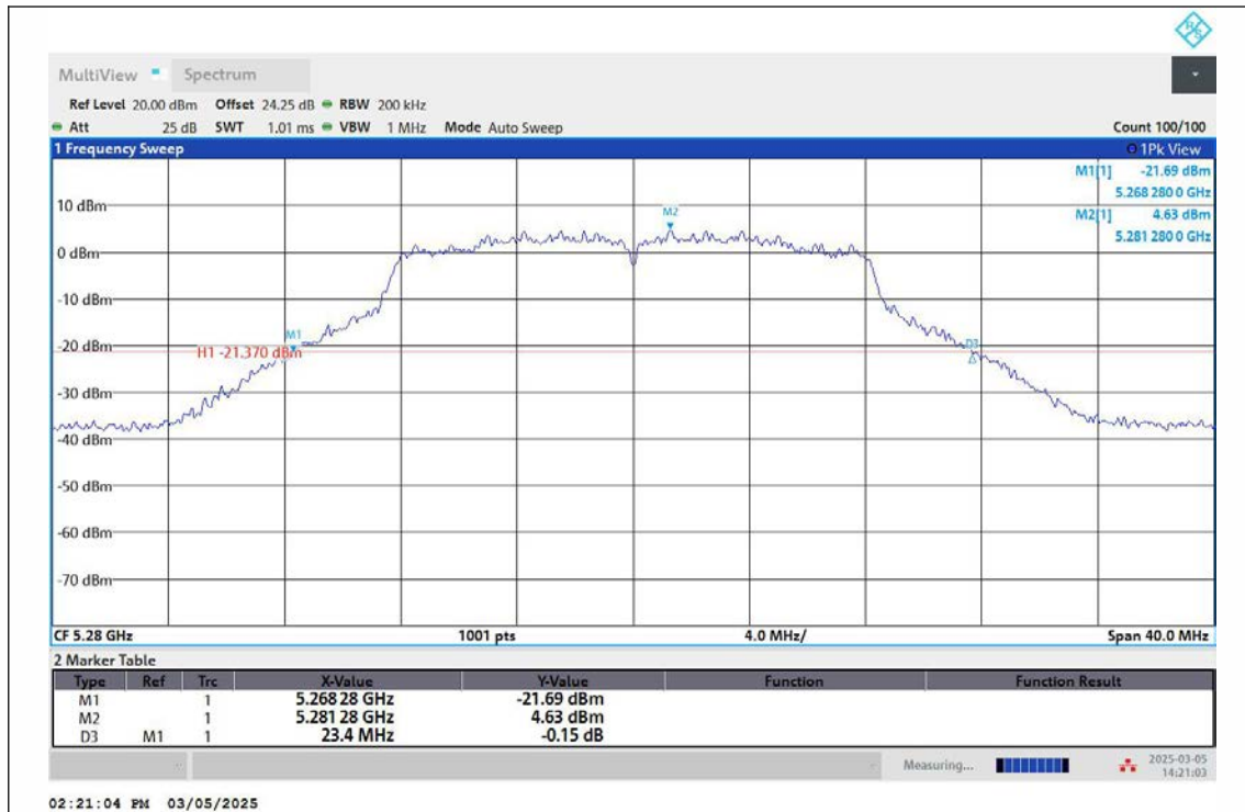
11A-Ant2-5280
