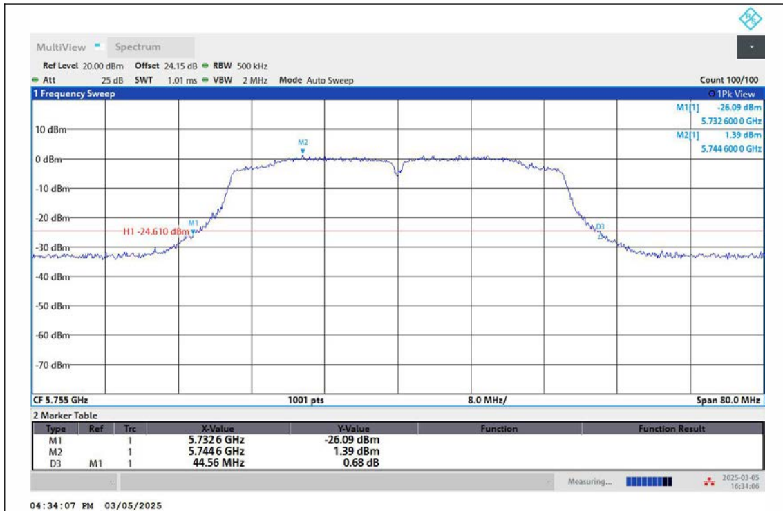
11N40MIMO-Ant2-5755
