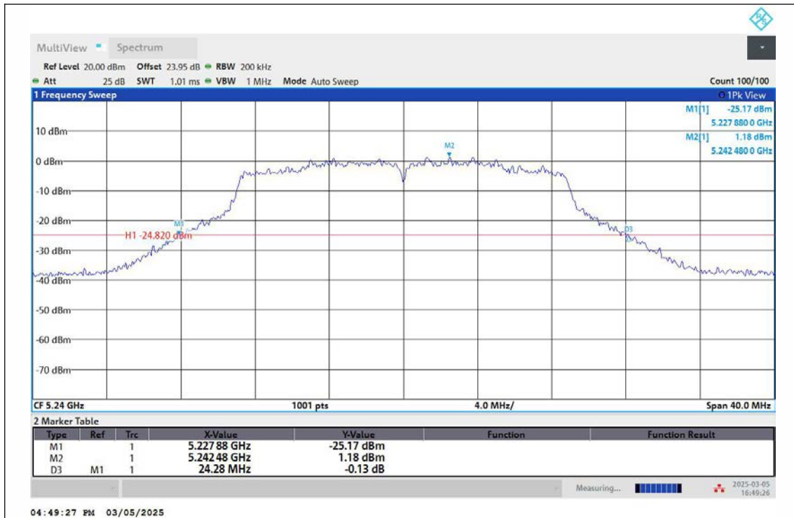
11AC20MIMO-Ant2-5240
