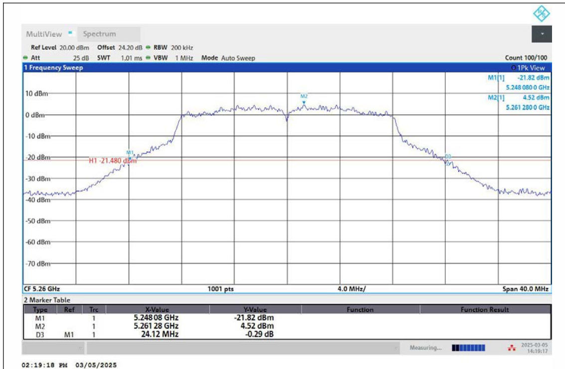
11A-Ant2-5260
