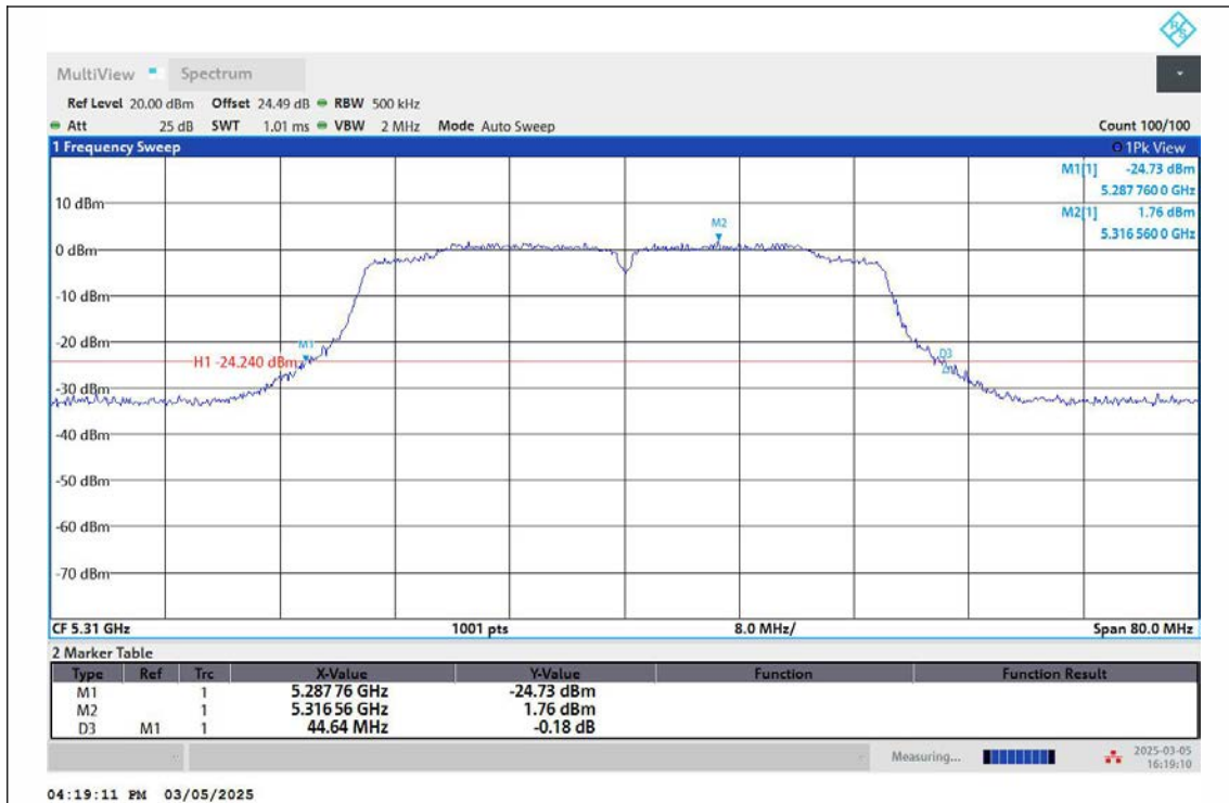
11N40MIMO-Ant2-5310
