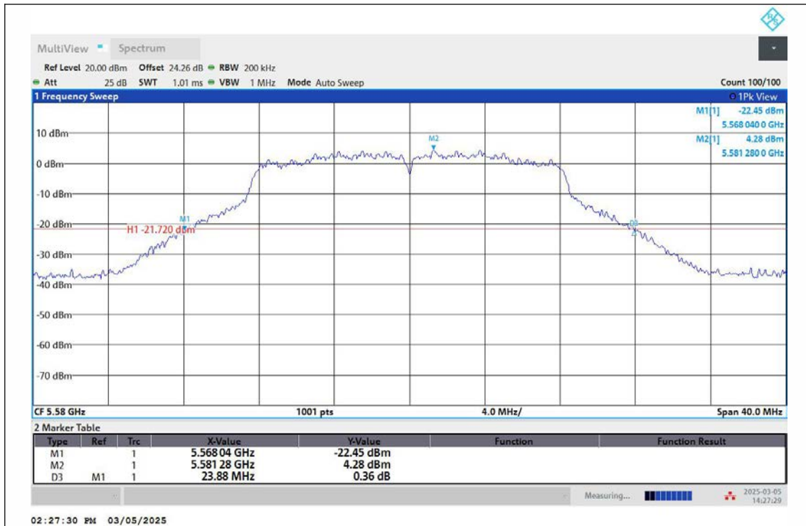
11A-Ant2-5580
