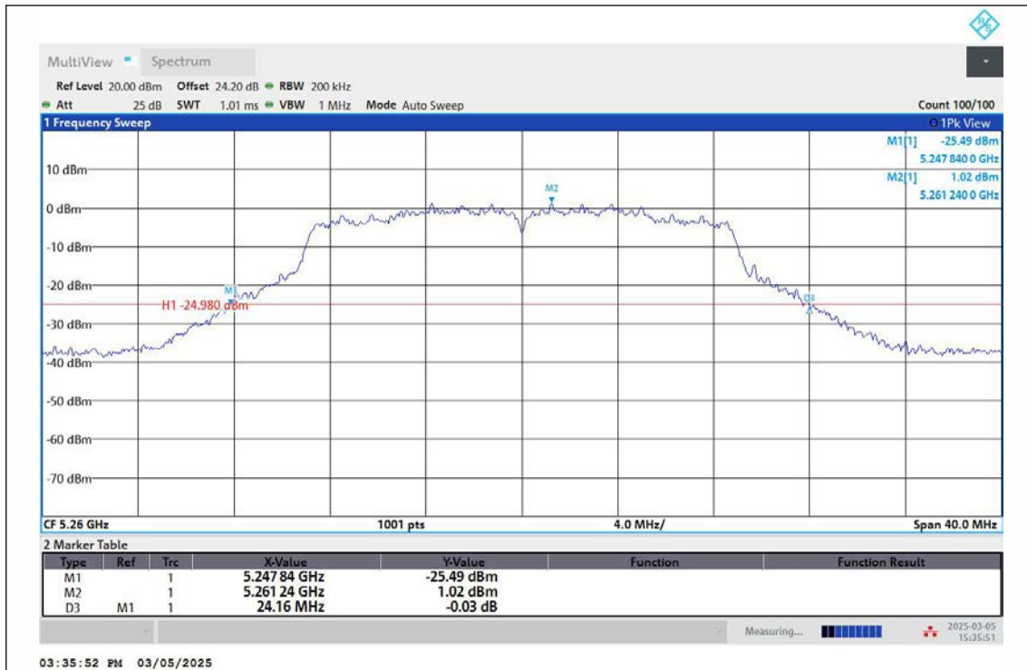
11N20MIMO-Ant2-5260
