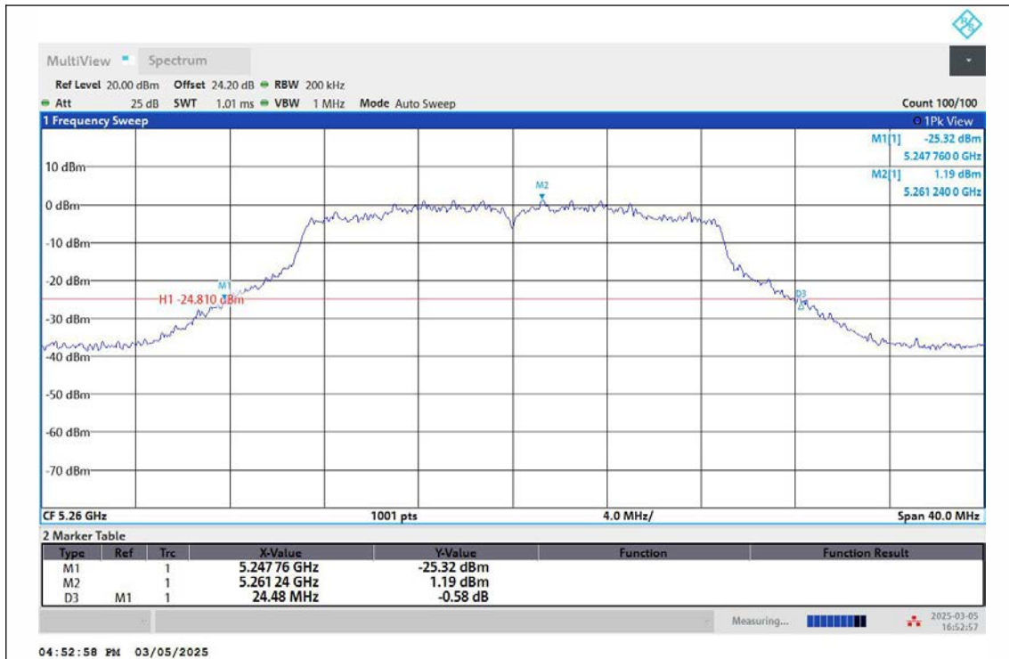
11AC20MIMO-Ant2-5260
