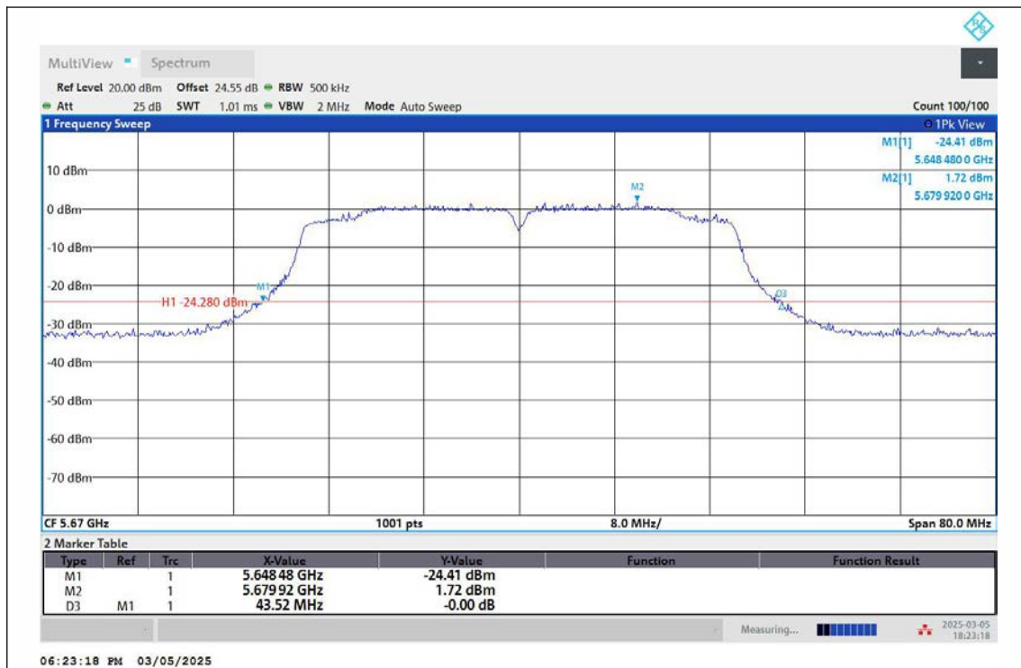
11AC40MIMO-Ant2-5670
