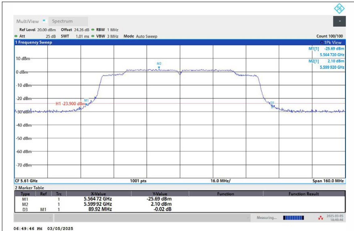
11AC80MIMO-Ant2-5610
