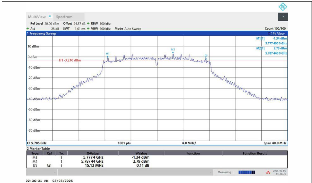
11A-Ant2-5785-PASS
