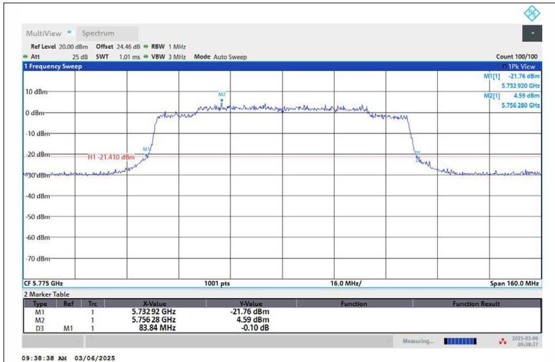
11AX80MIMO-Ant2-5775
