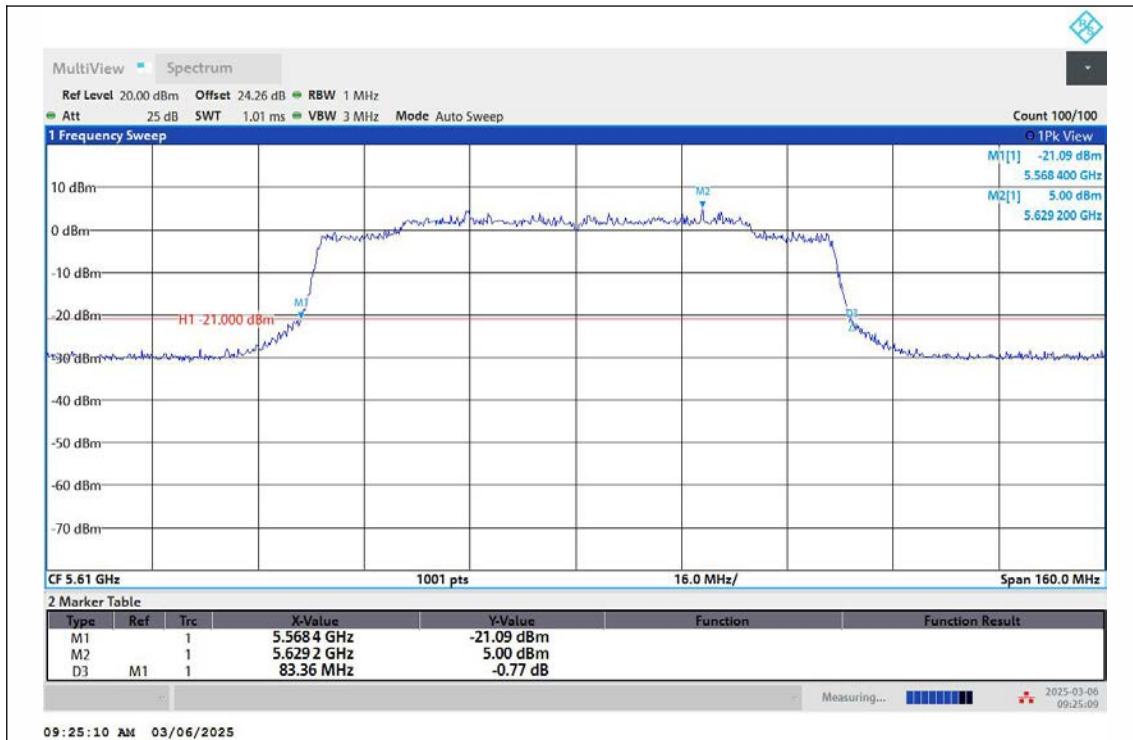
11AX80MIMO-Ant2-5610
