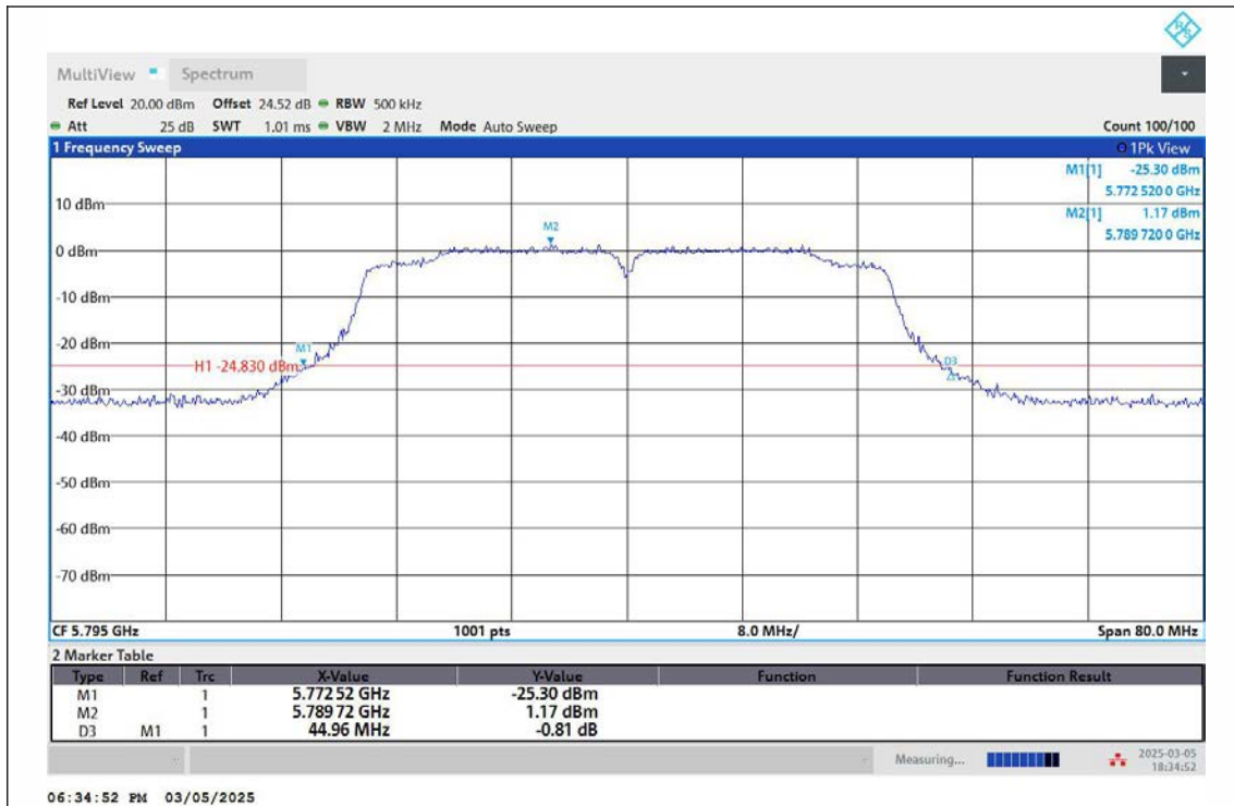
11AC40MIMO-Ant2-5795
