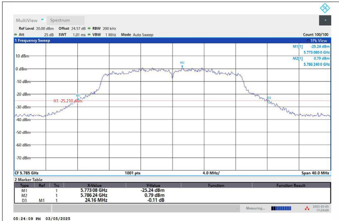
11AC20MIMO-Ant2-5785
