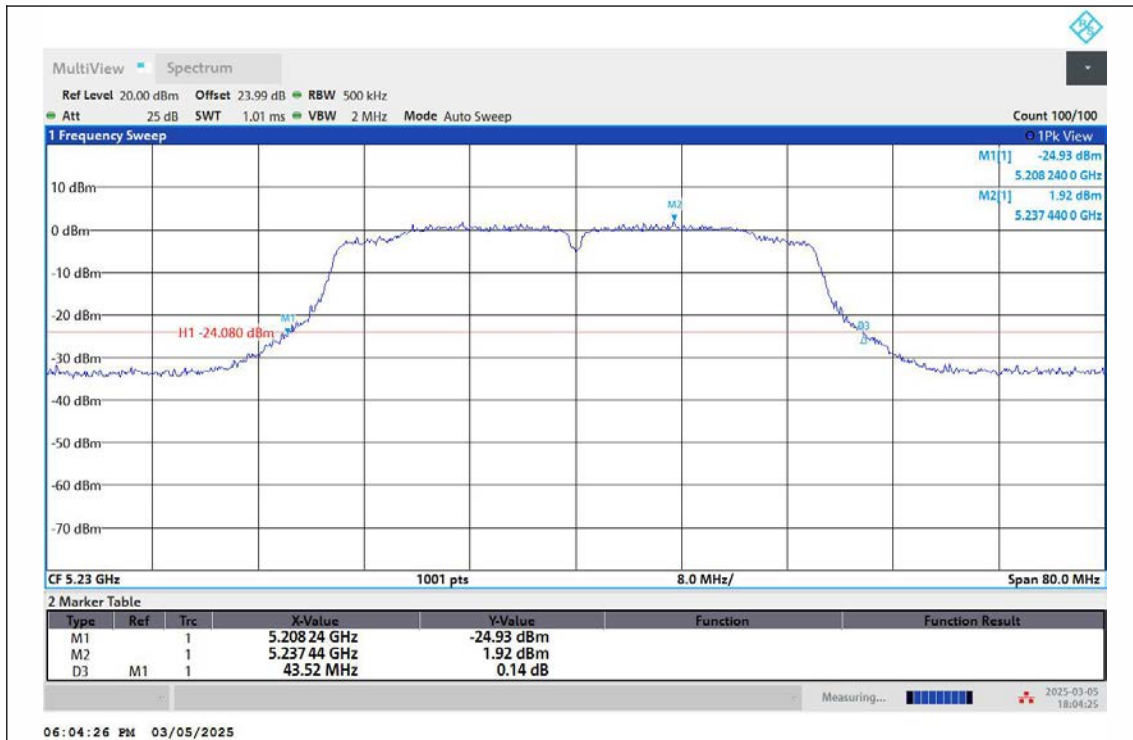
11AC40MIMO-Ant2-5230
