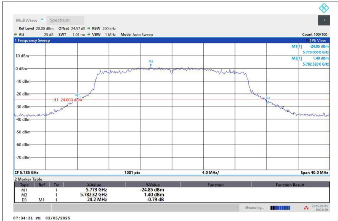
11AX20MIMO-Ant2-5785
