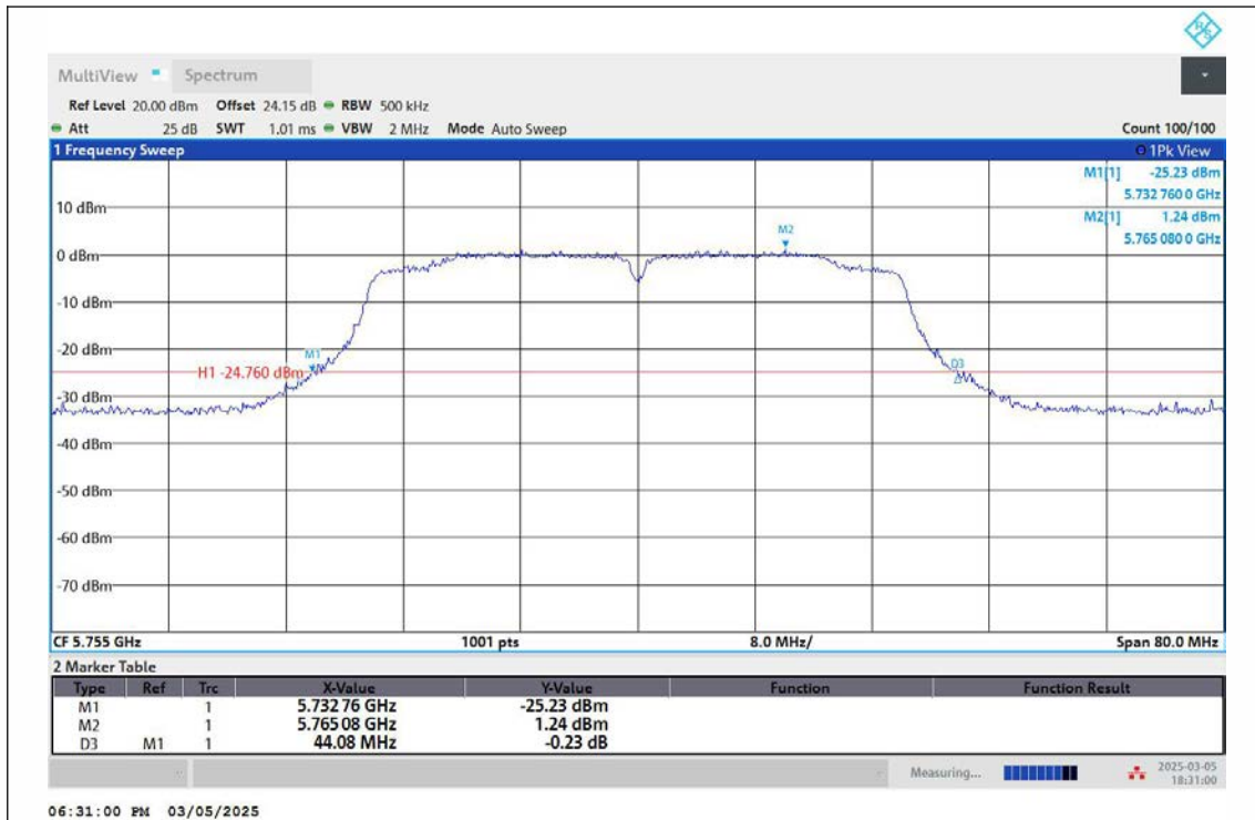
11AC40MIMO-Ant2-5755
