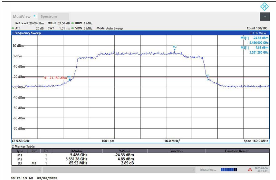
11AX80MIMO-Ant2-5530
