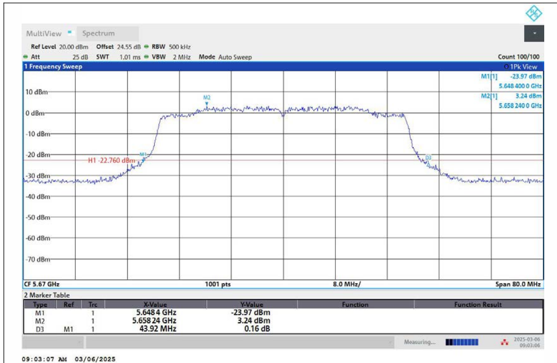
11AX40MIMO-Ant2-5670
