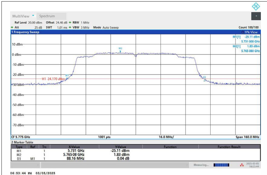
11AC80MIMO-Ant2-5775
