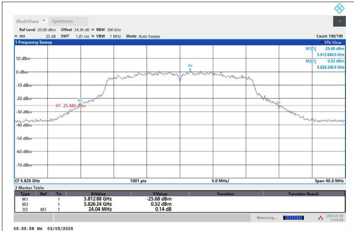
11AC20MIMO-Ant2-5825
