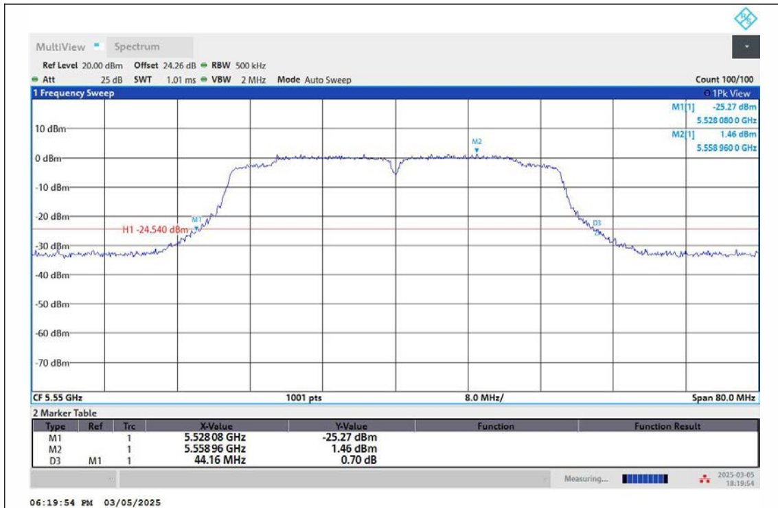
11AC40MIMO-Ant2-5550
