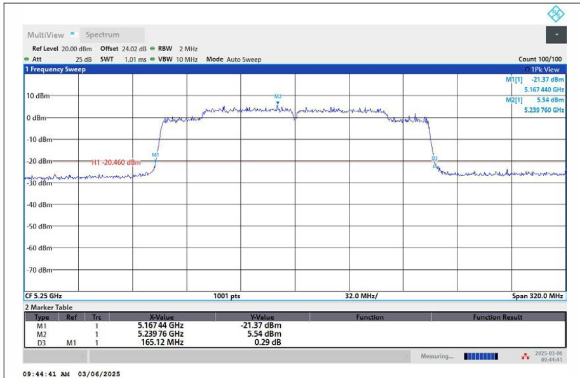
11AX160MIMO-Ant2-5250
