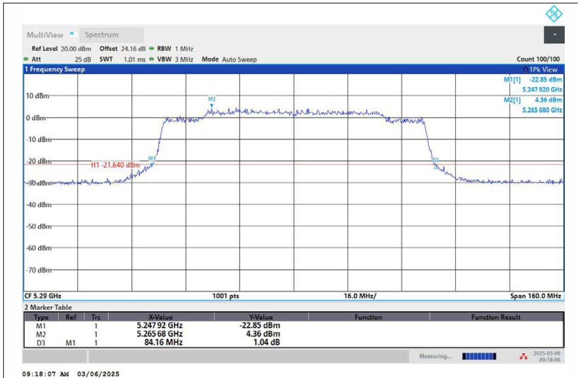
11AX80MIMO-Ant2-5290
