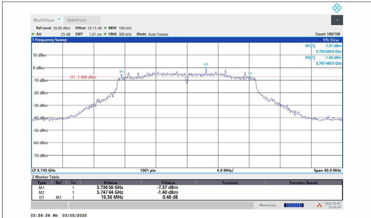
11N20MIMO-Ant2-5745-PASS
