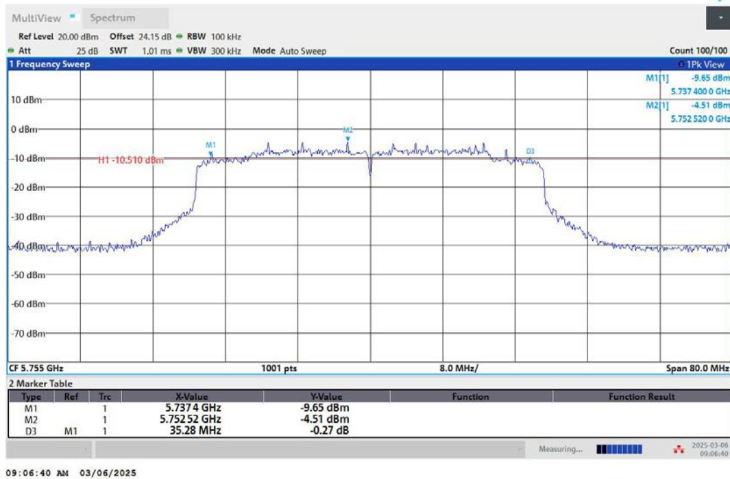
11AX40MIMO-Ant2-5755-PASS
