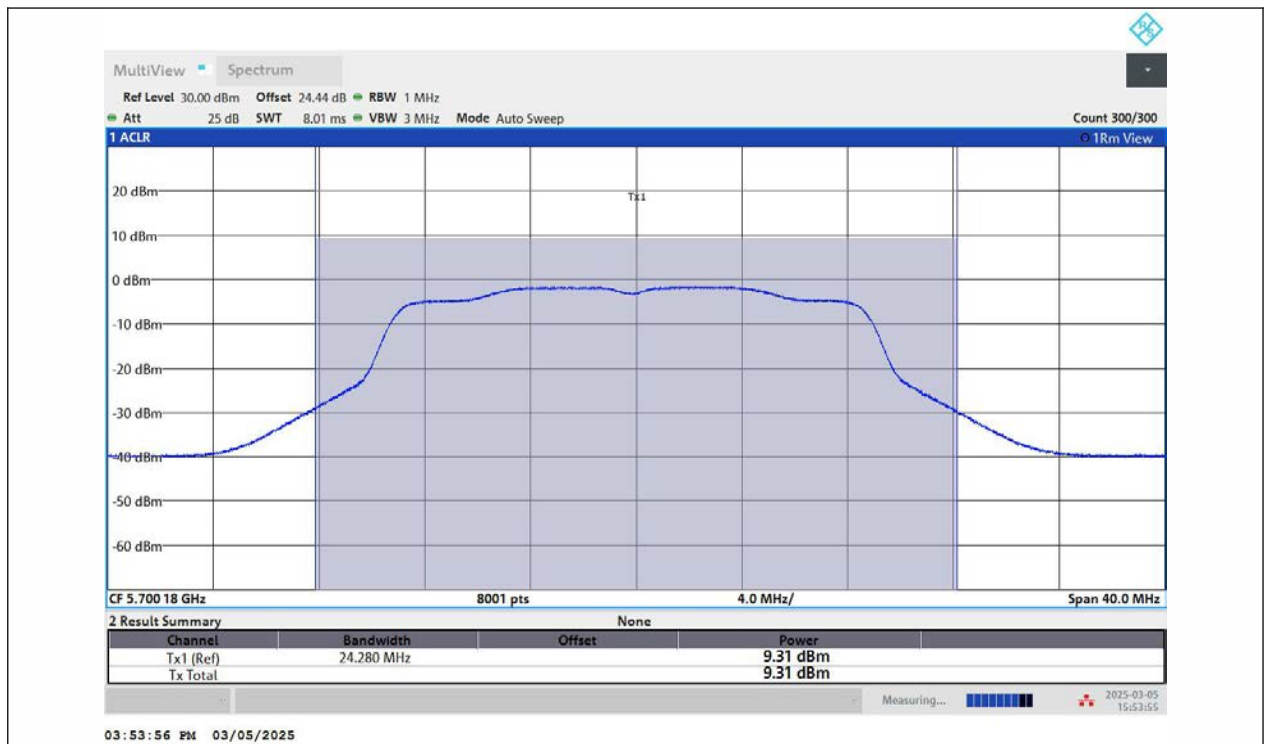
11N20MIMO-Ant2-5700-PASS
