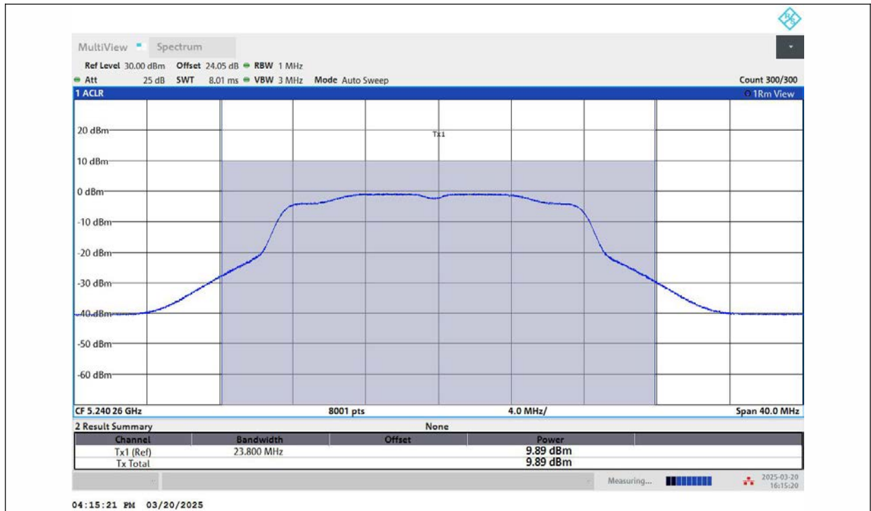
11A-Ant2-5240-PASS
