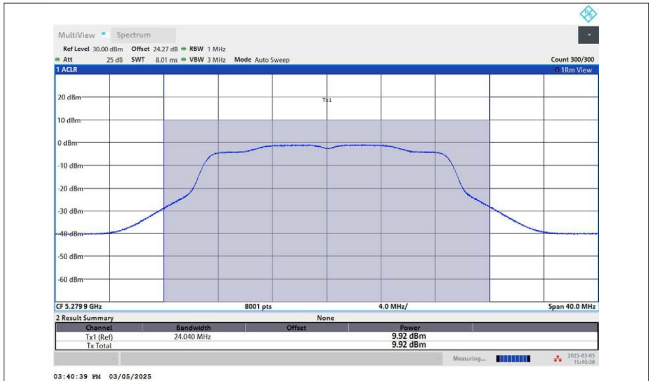
11N20MIMO-Ant2-5280-PASS
