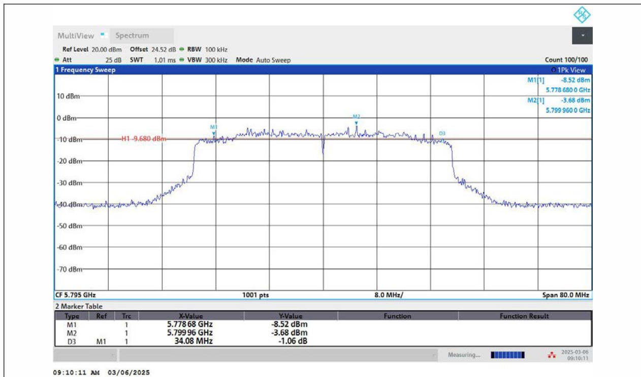
11AX40MIMO-Ant2-5795-PASS
