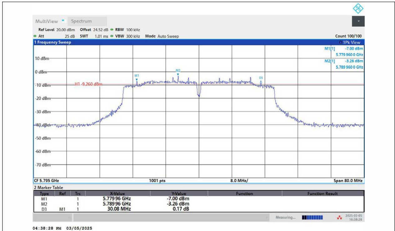
11N40MIMO-Ant2-5795-PASS
