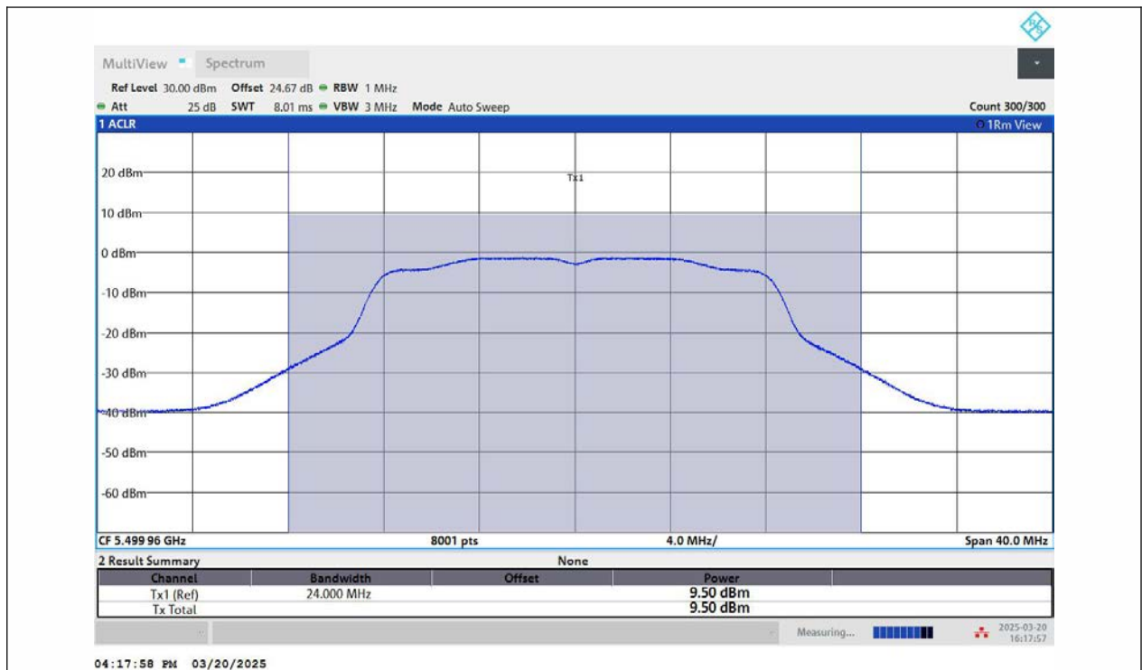
11A-Ant2-5500-PASS
