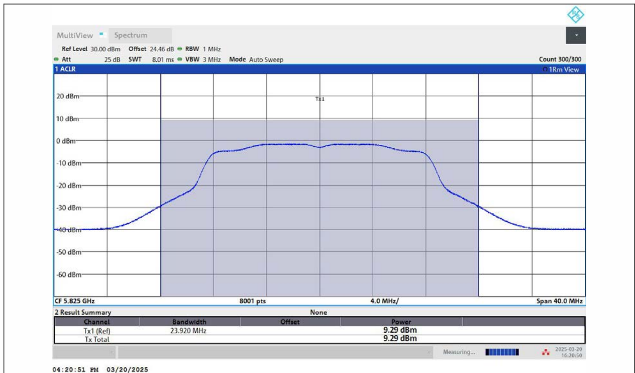
11A-Ant2-5825-PASS
