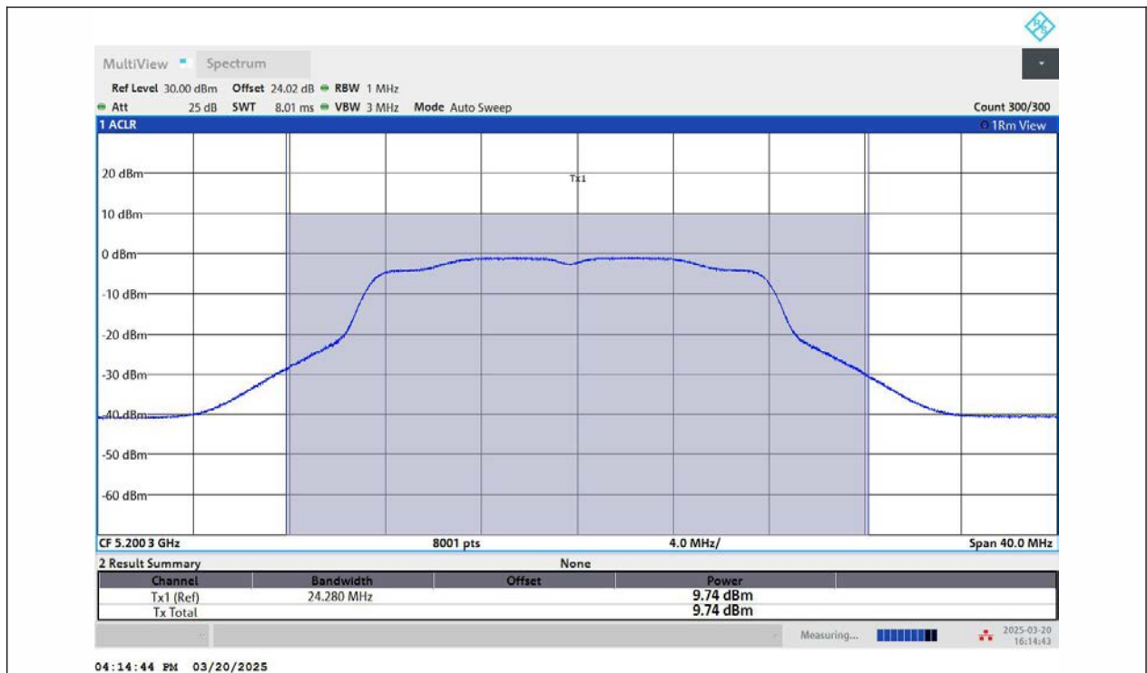
11A-Ant2-5200-PASS
