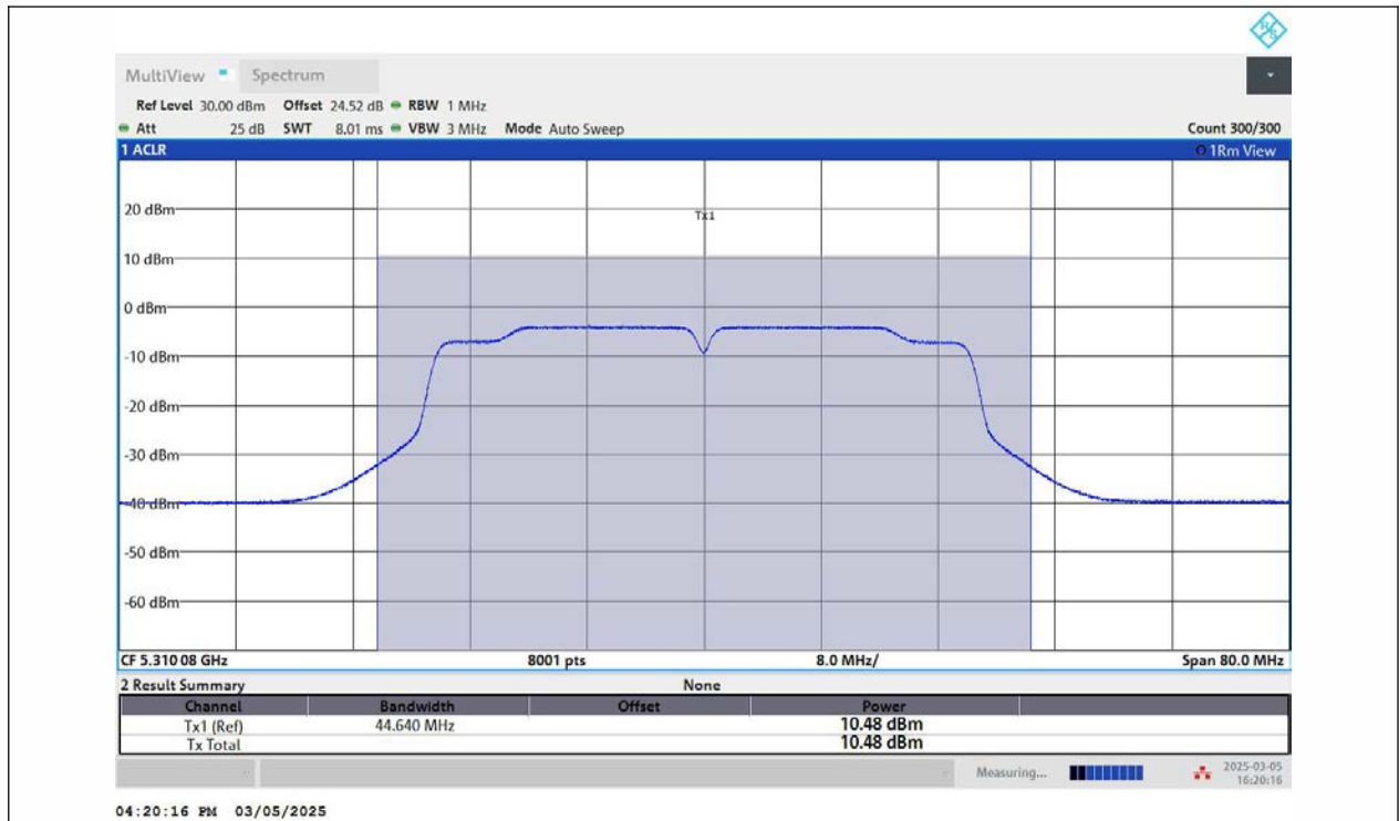
11N40MIMO-Ant2-5310-PASS
