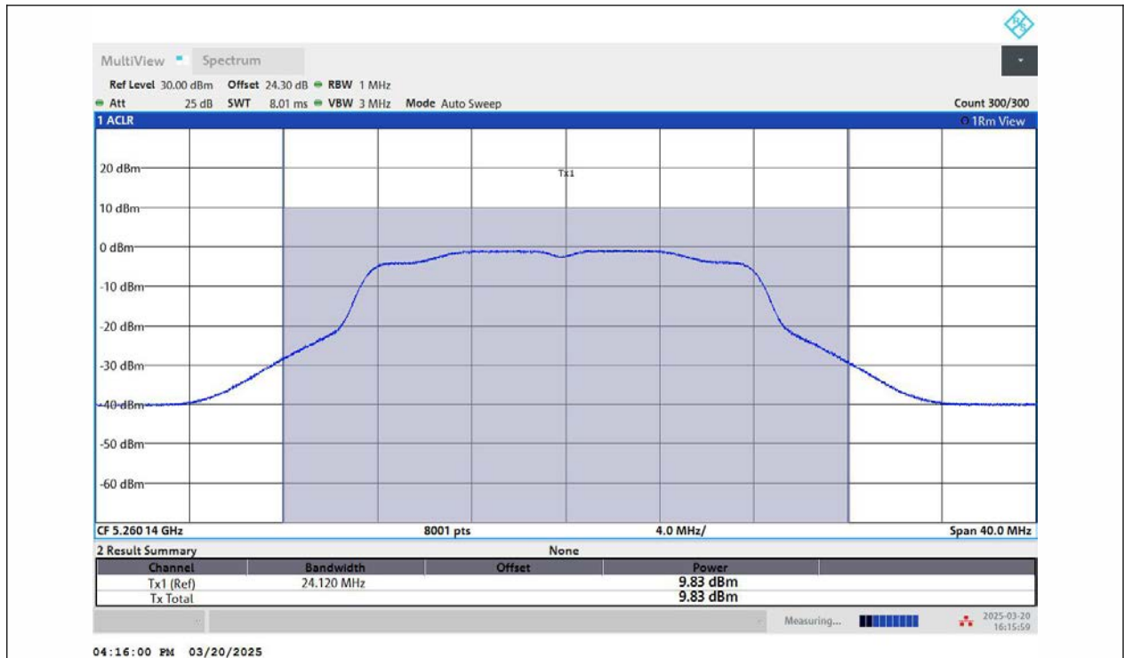
11A-Ant2-5260-PASS
