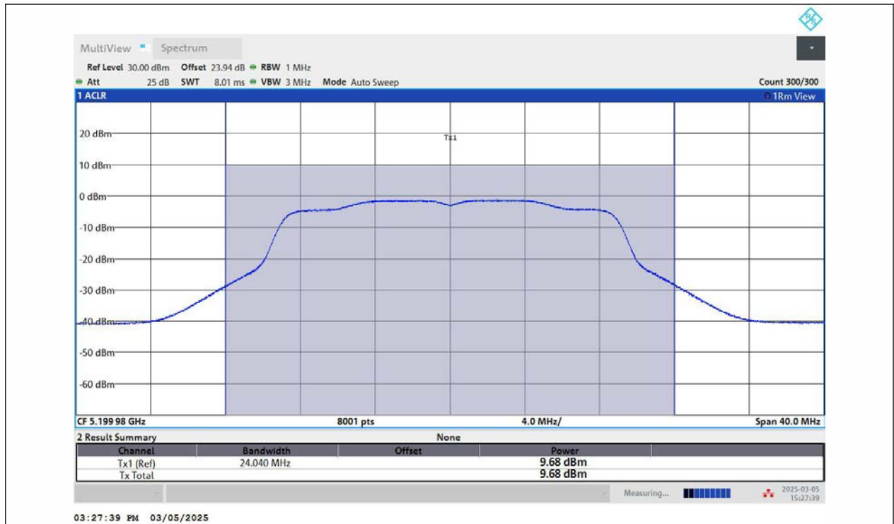
11N20MIMO-Ant2-5200-PASS
