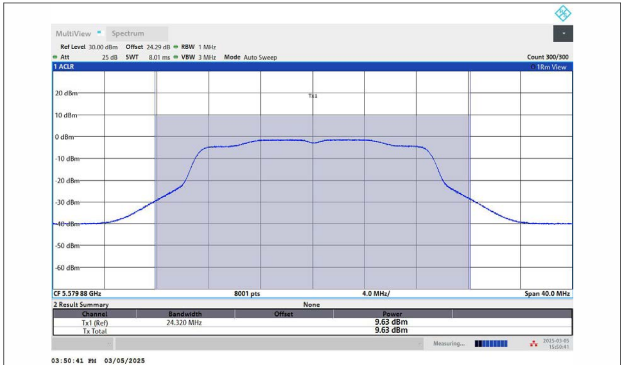
11N20MIMO-Ant2-5580-PASS
