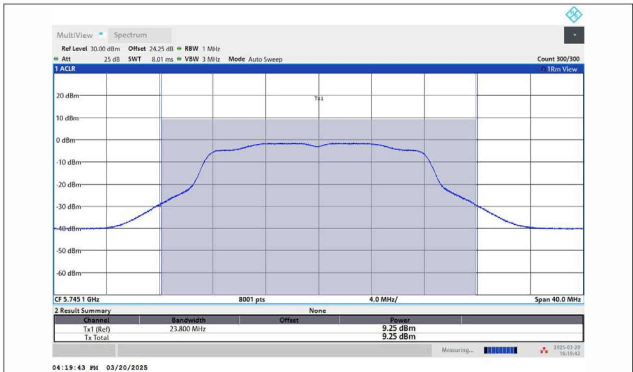
11A-Ant2-5745-PASS
