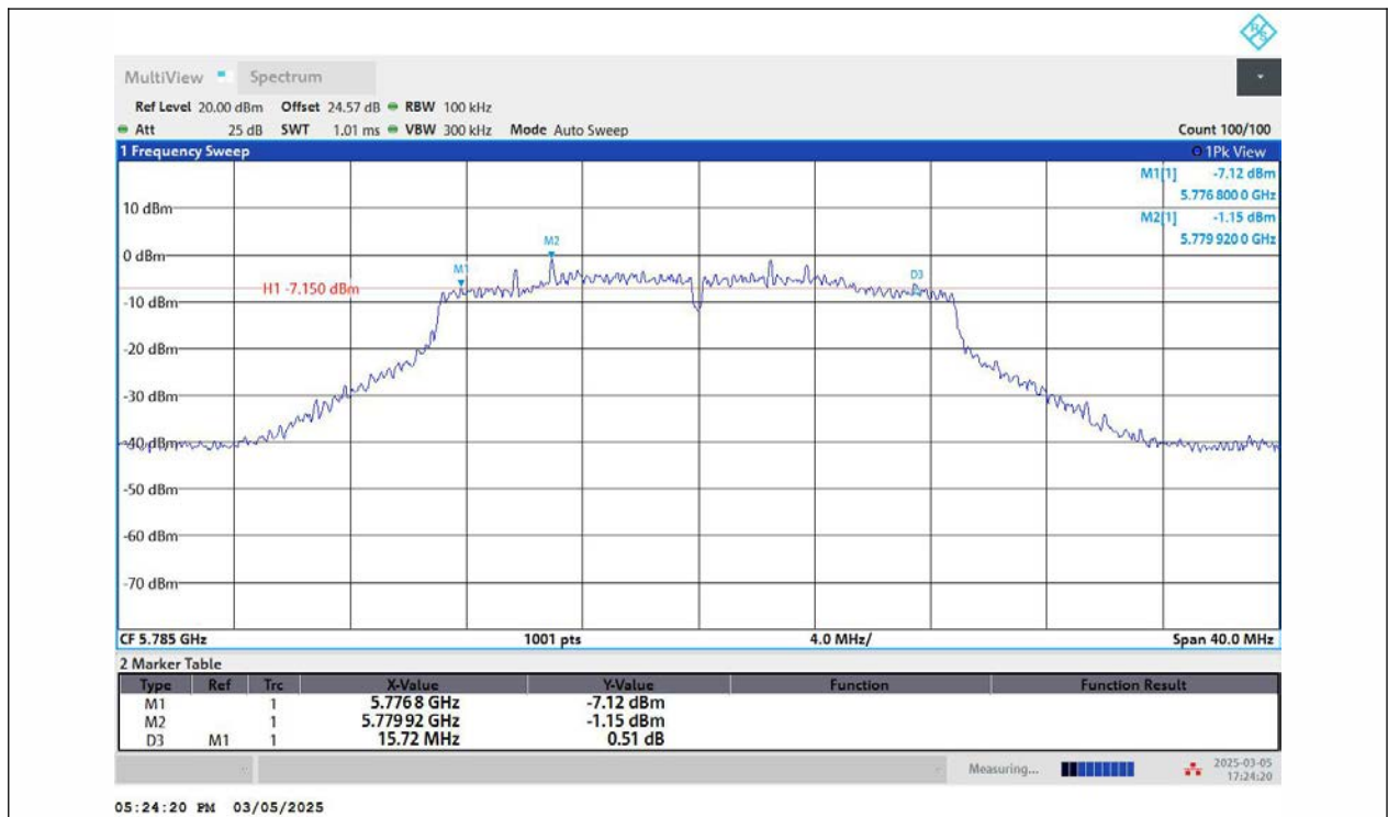
11AC20MIMO-Ant2-5785-PASS
