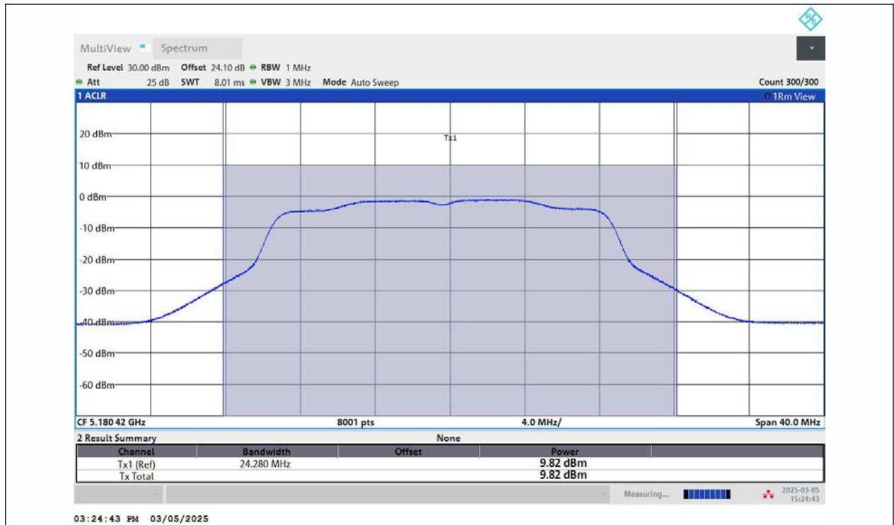
11N20MIMO-Ant2-5180-PASS
