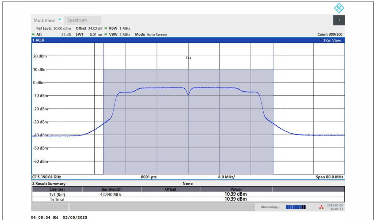
11N40MIMO-Ant2-5190-PASS
