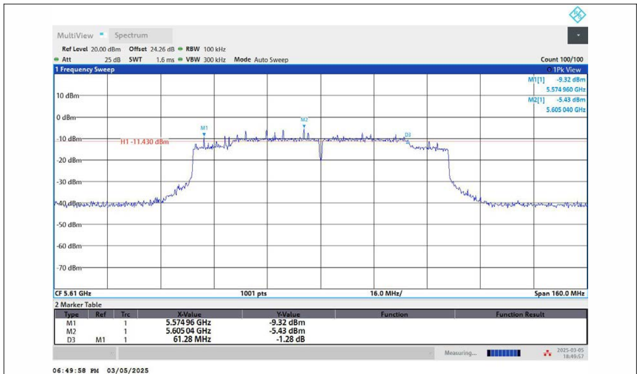
11AC80MIMO-Ant2-5610-PASS
