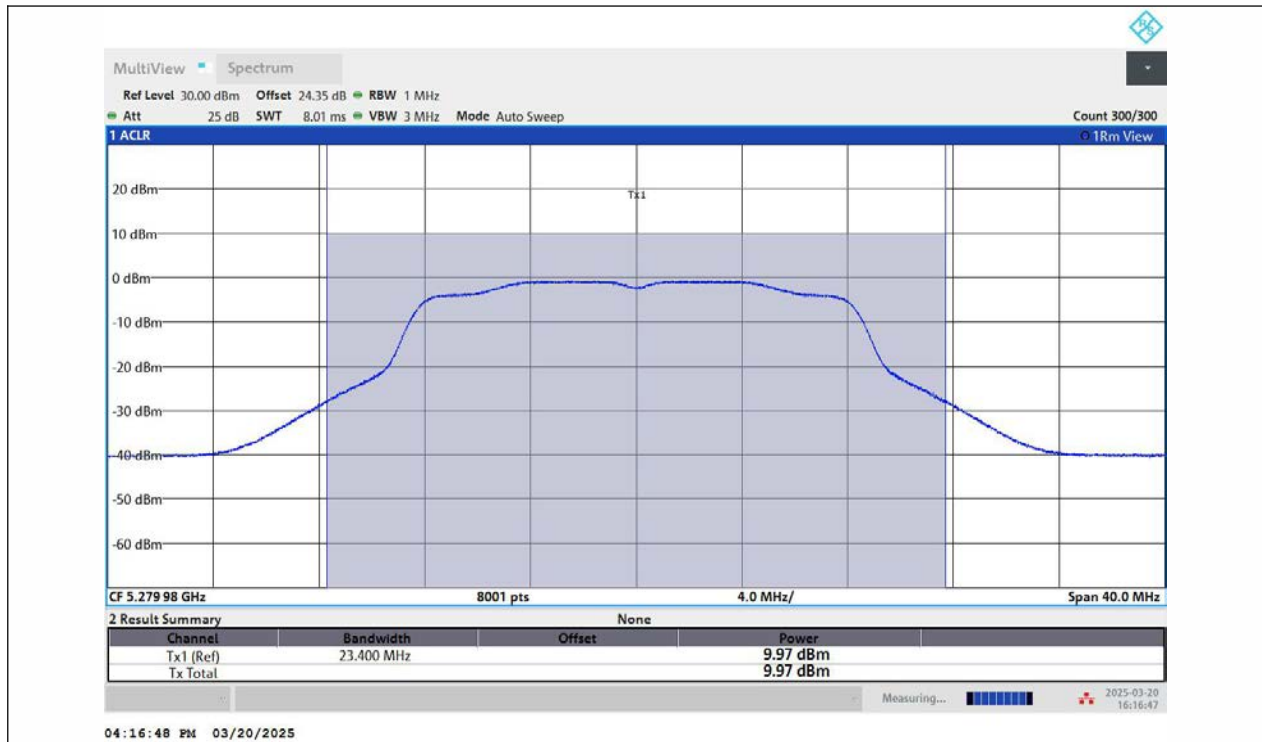
11A-Ant2-5280-PASS
