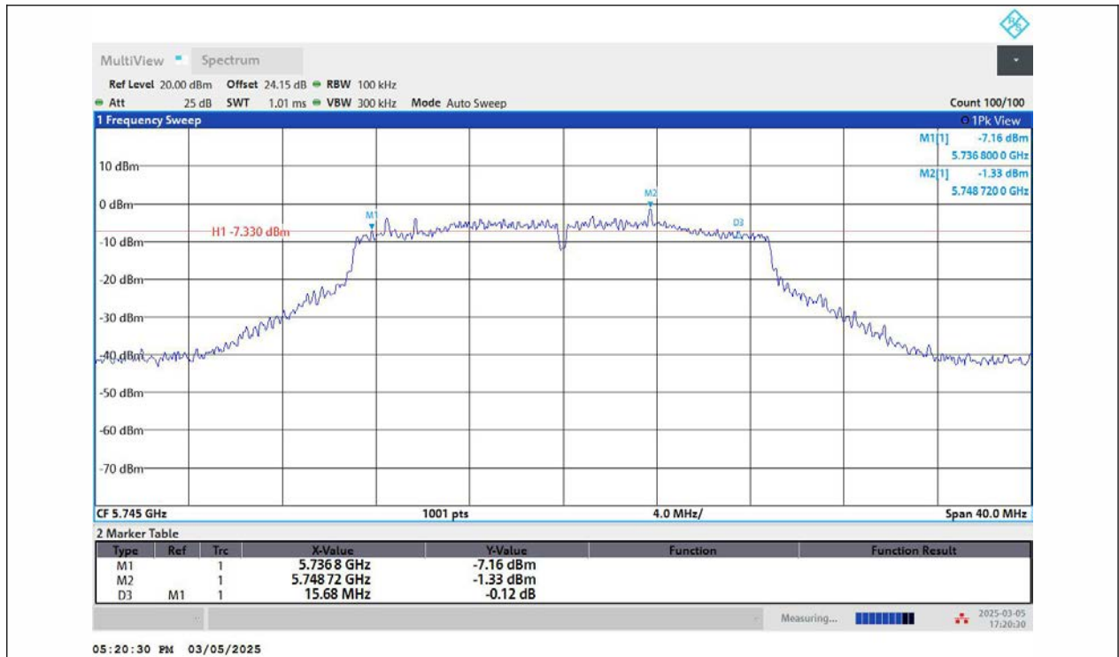
11AC20MIMO-Ant2-5745-PASS
