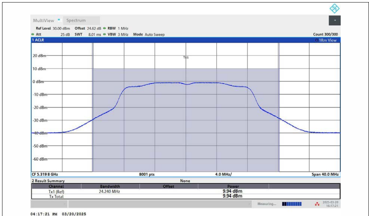
11A-Ant2-5320-PASS
