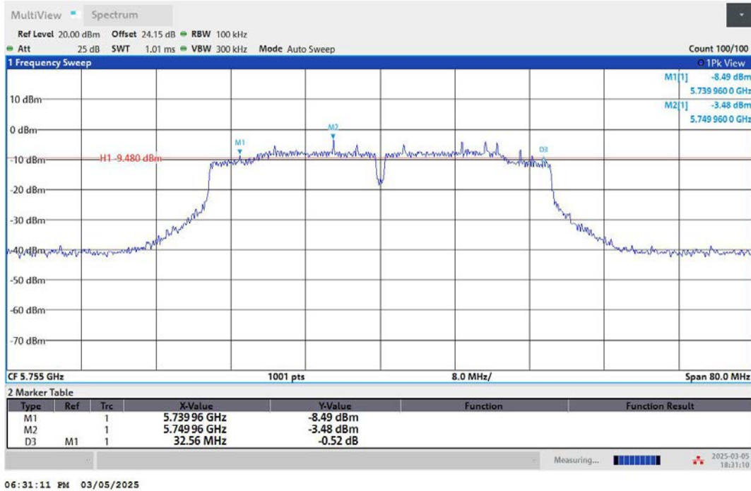
11AC40MIMO-Ant2-5755-PASS
