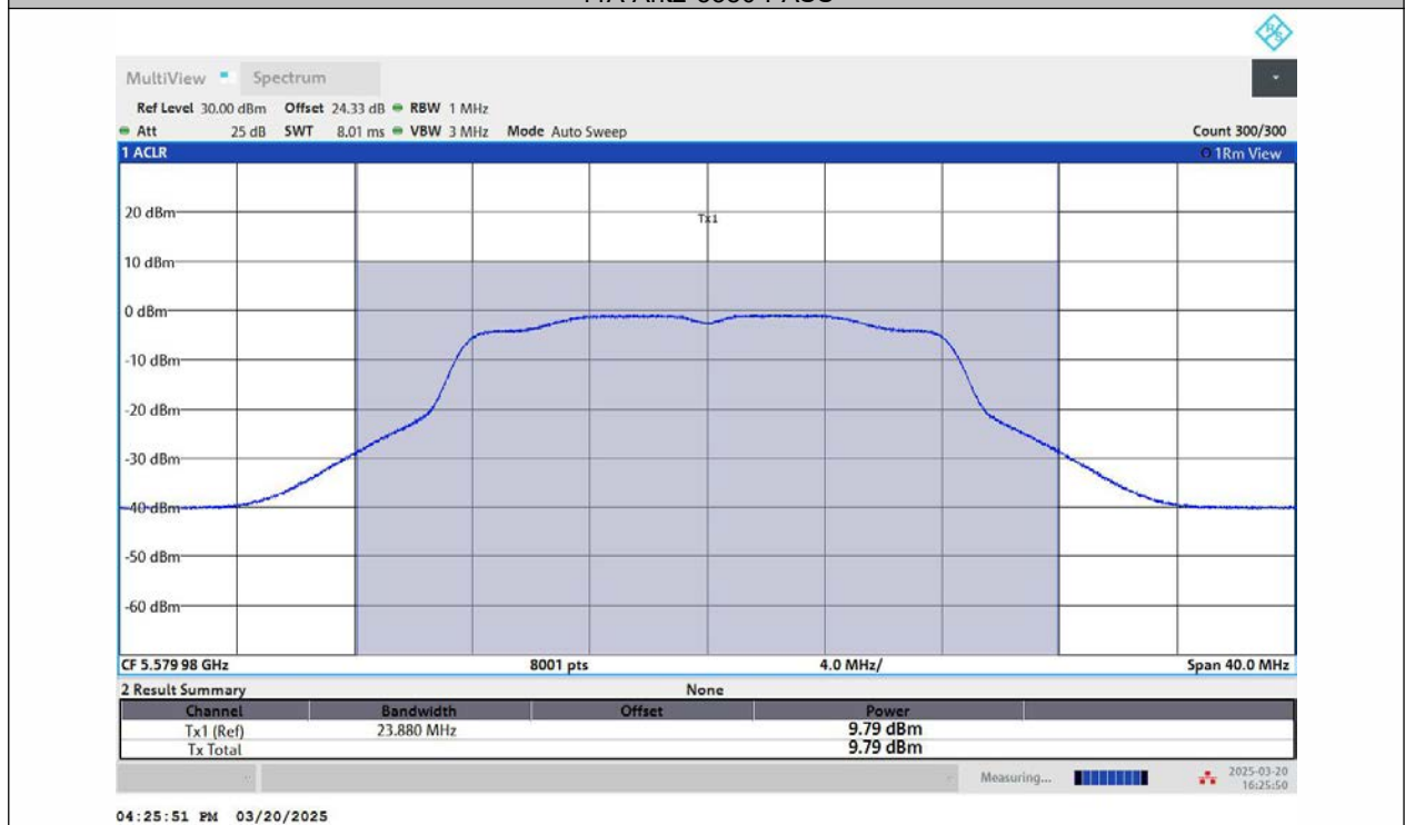
11A-Ant1-5700-PASS
