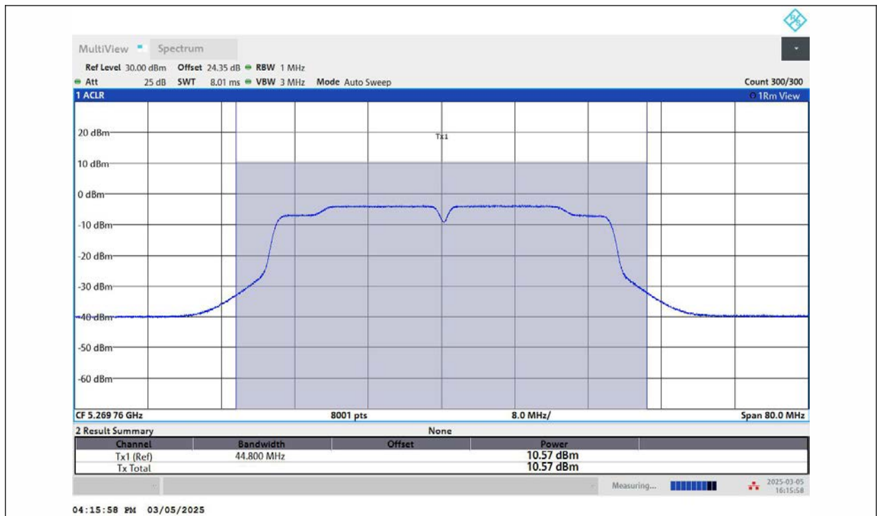
11N40MIMO-Ant2-5270-PASS
