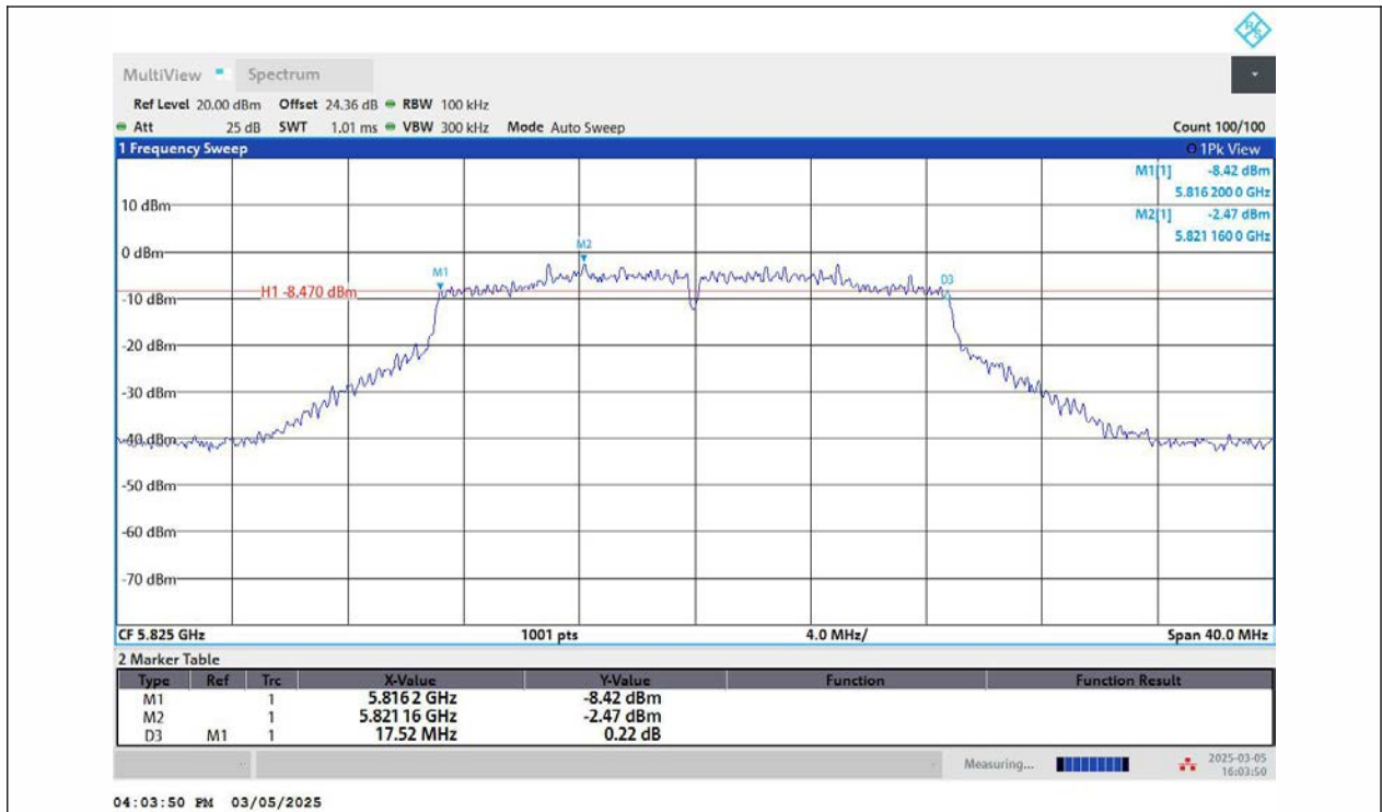
11N20MIMO-Ant2-5825-PASS
