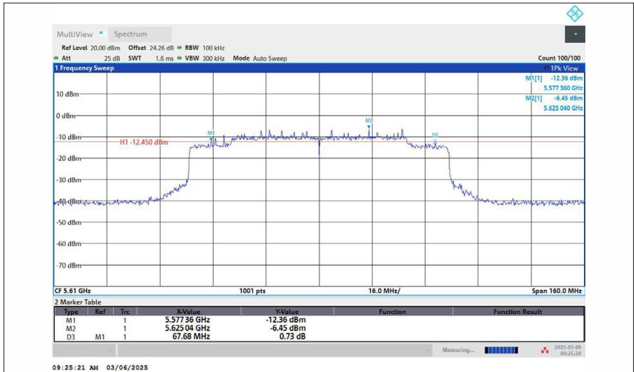
11AX80MIMO-Ant2-5610-PASS
