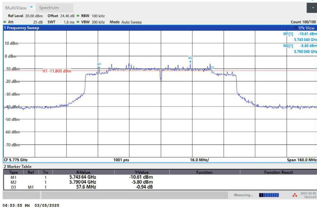
11AC80MIMO-Ant2-5775-PASS
