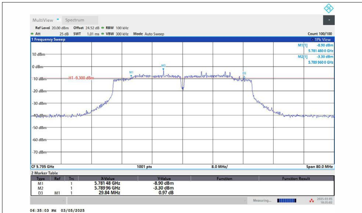
11AC40MIMO-Ant2-5795-PASS
