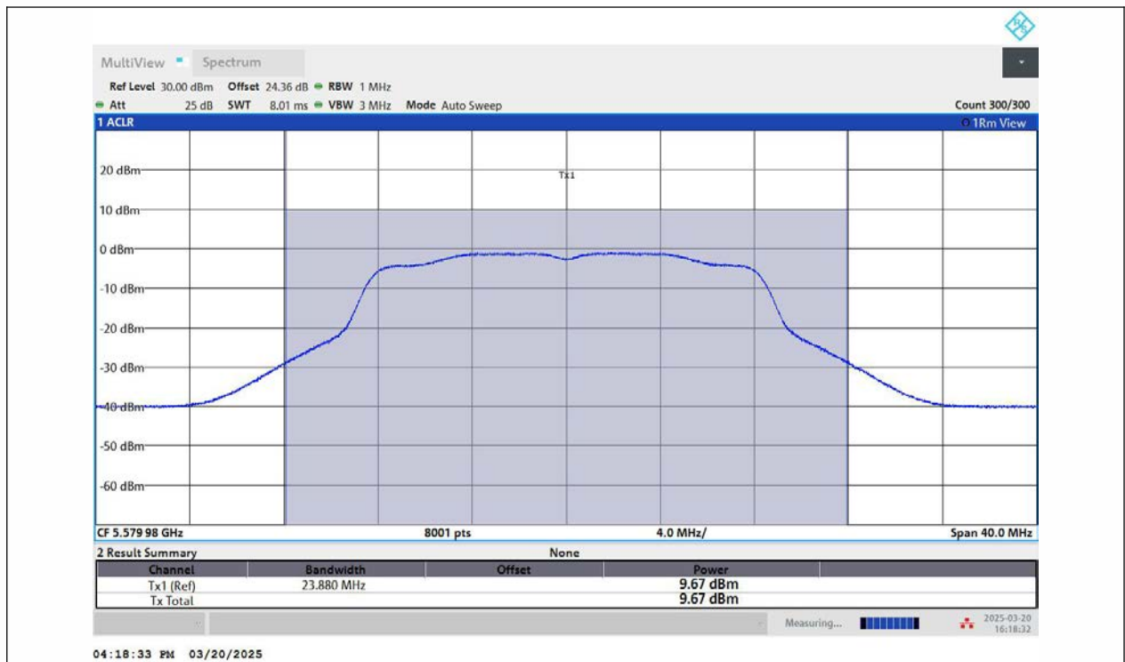
11A-Ant2-5580-PASS
