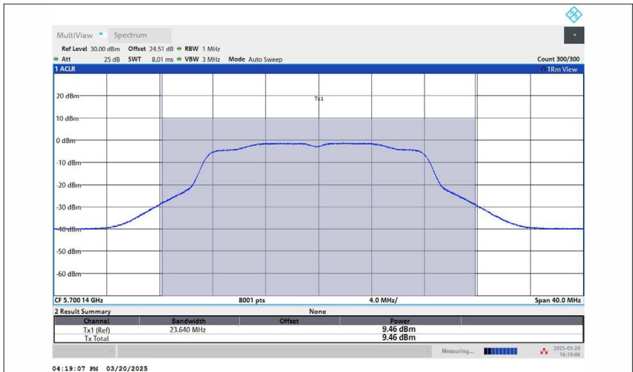
11A-Ant2-5700-PASS
