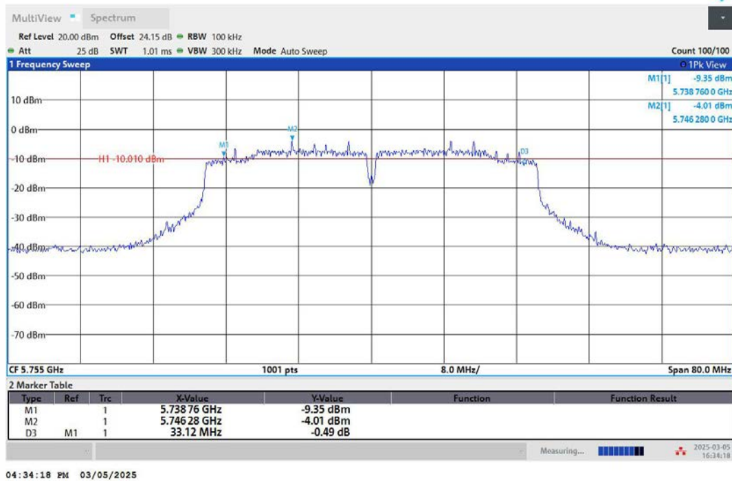
11N40MIMO-Ant2-5755-PASS
