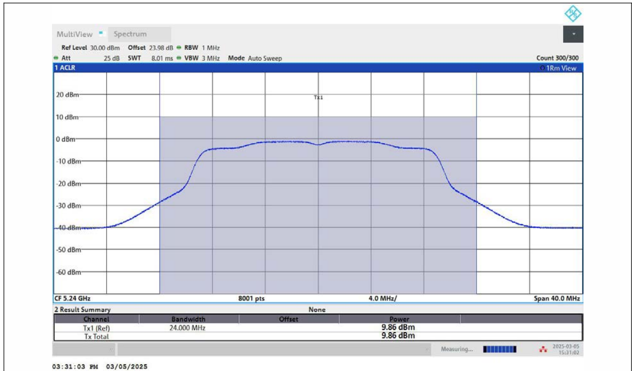
11N20MIMO-Ant2-5240-PASS
