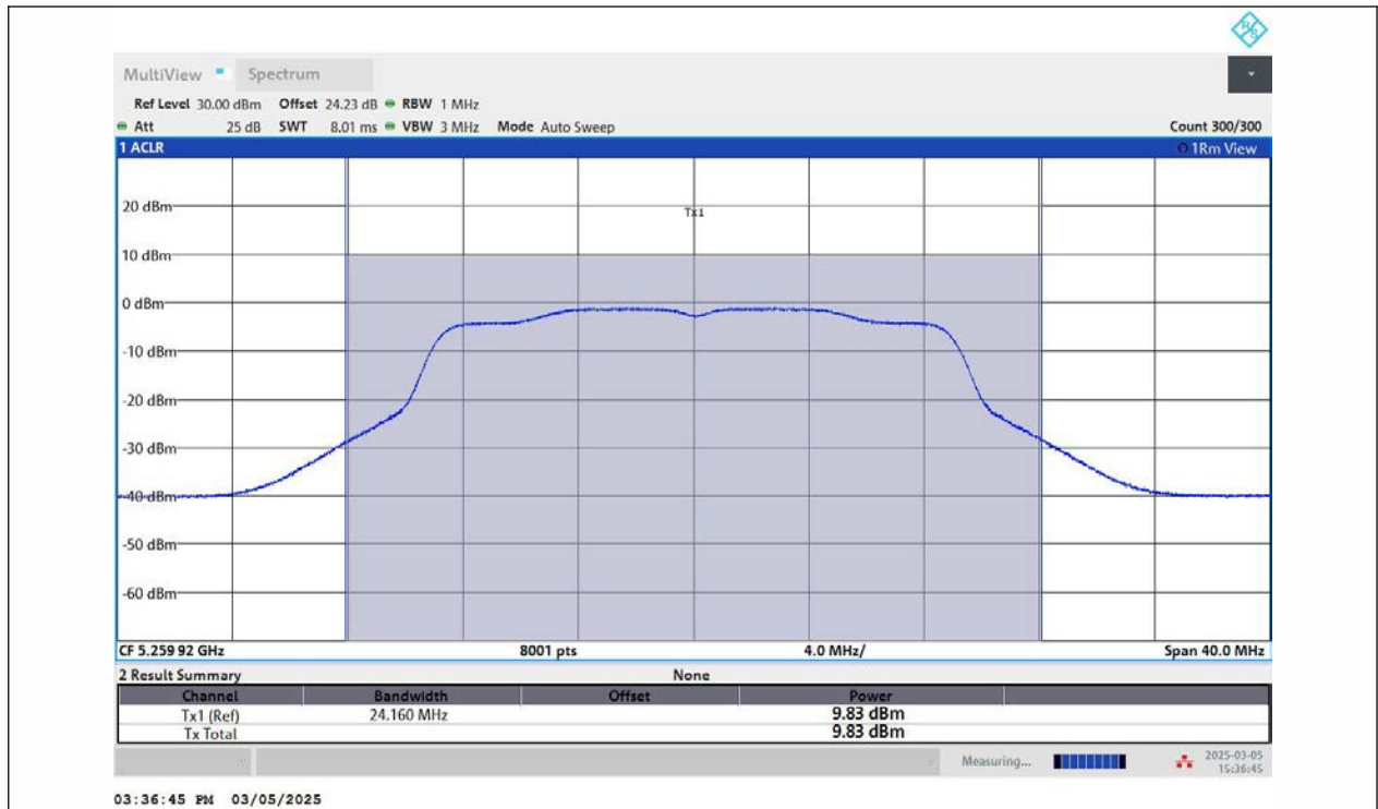
11N20MIMO-Ant2-5260-PASS
