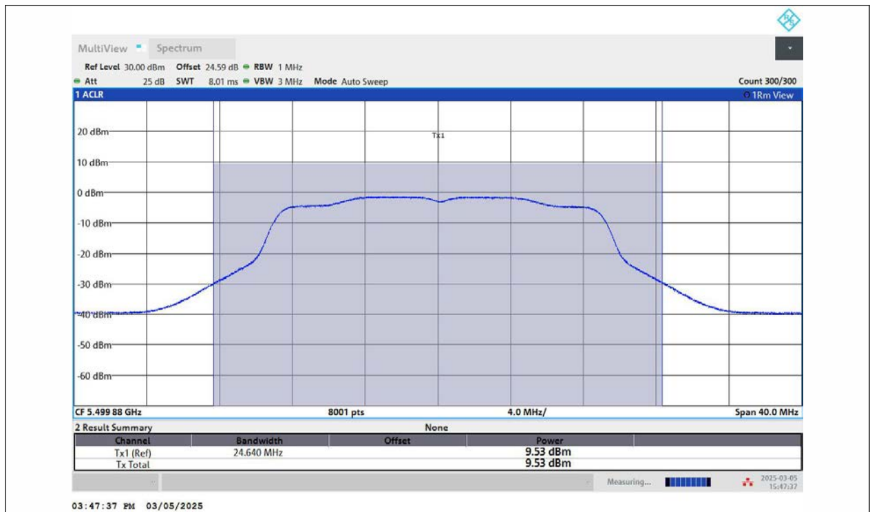
11N20MIMO-Ant2-5500-PASS
