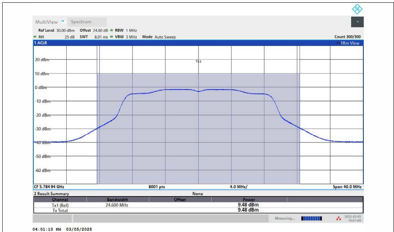
11N20MIMO-Ant2-5785-PASS
