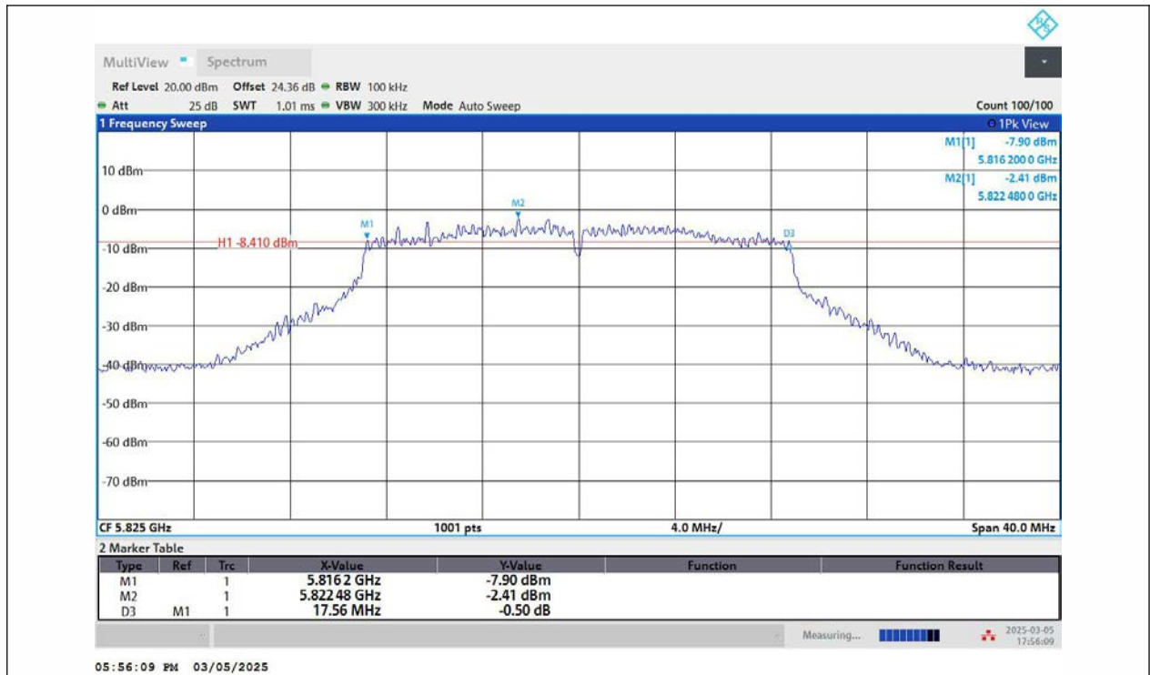
11AC20MIMO-Ant2-5825-PASS
