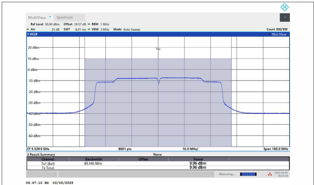
11AC80MIMO-Ant2-5530-PASS
