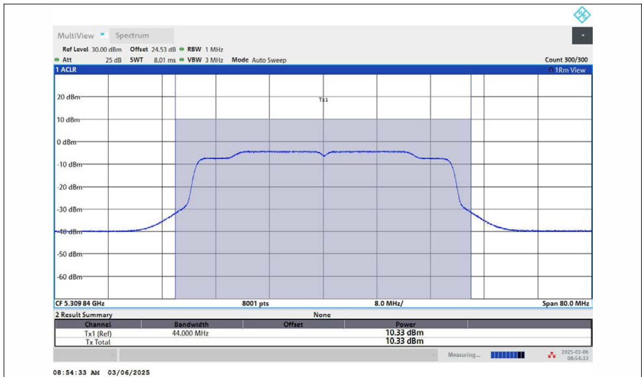
11AX40MIMO-Ant2-5310-PASS
