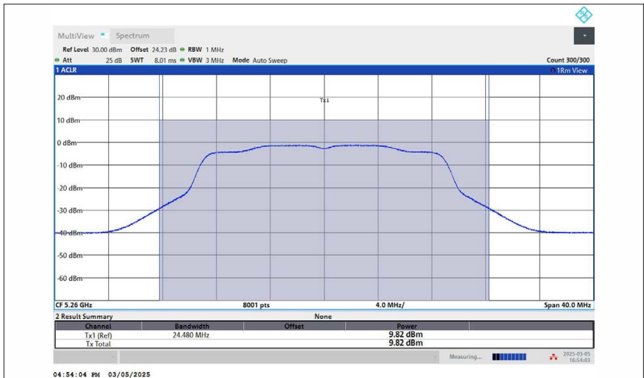
11AC20MIMO-Ant2-5260-PASS
