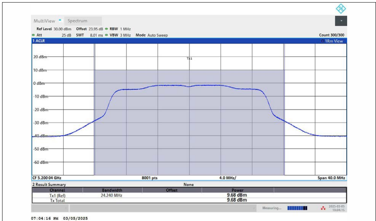
11AX20MIMO-Ant2-5200-PASS
