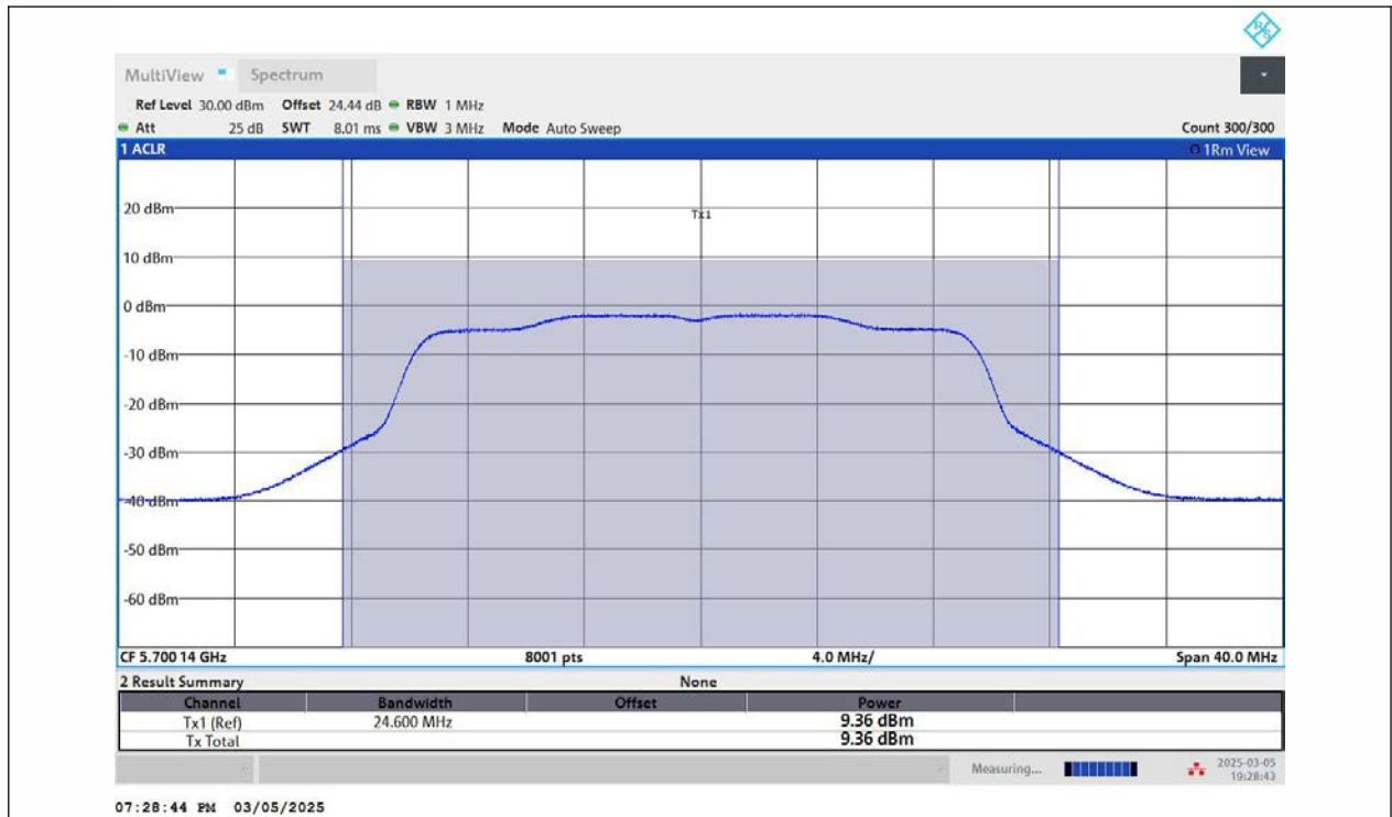
11AX20MIMO-Ant2-5700-PASS
