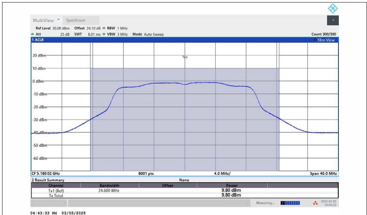
11AC20MIMO-Ant2-5180-PASS
