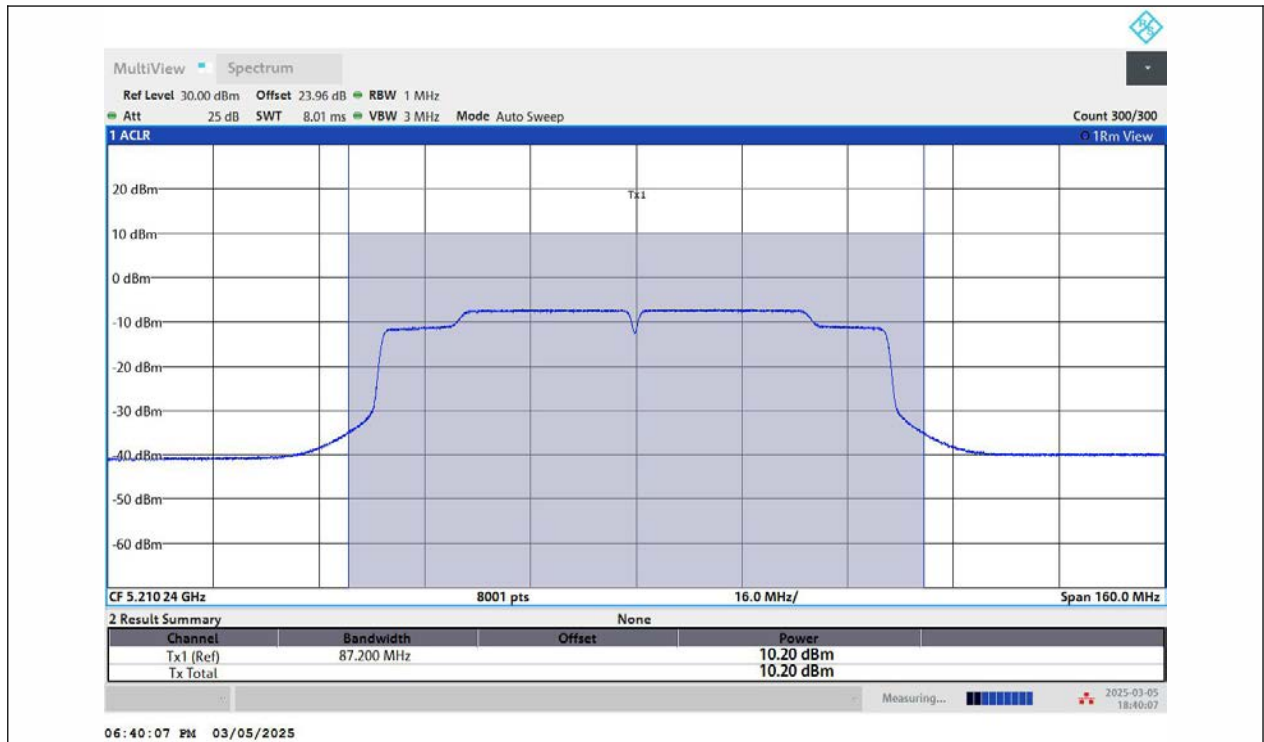
11AC80MIMO-Ant2-5210-PASS
