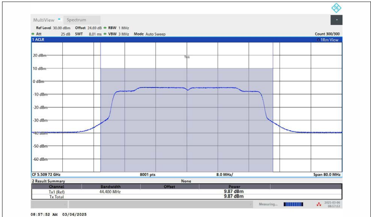
11AX40MIMO-Ant2-5510-PASS
