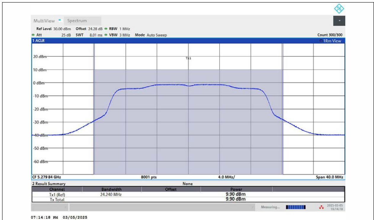
11AX20MIMO-Ant2-5280-PASS
