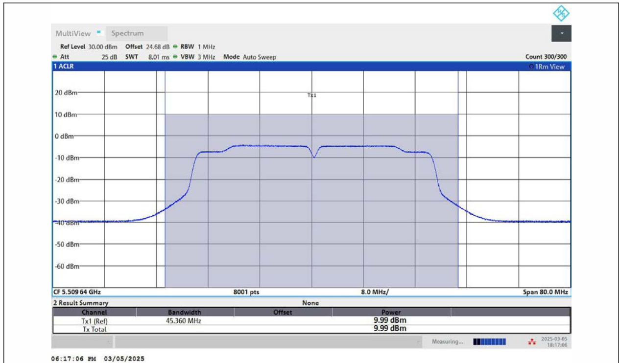
11AC40MIMO-Ant2-5510-PASS
