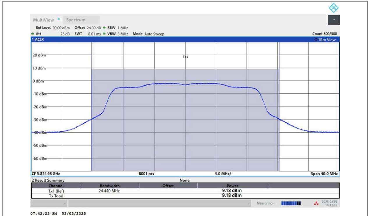
11AX20MIMO-Ant2-5825-PASS
