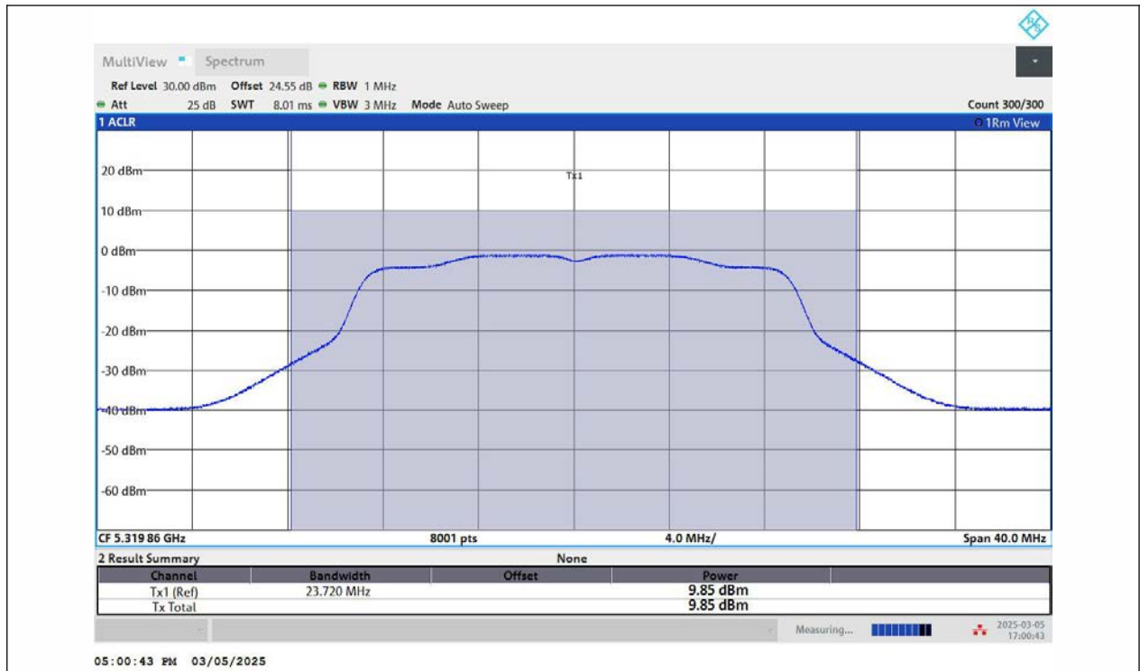
11AC20MIMO-Ant2-5320-PASS
