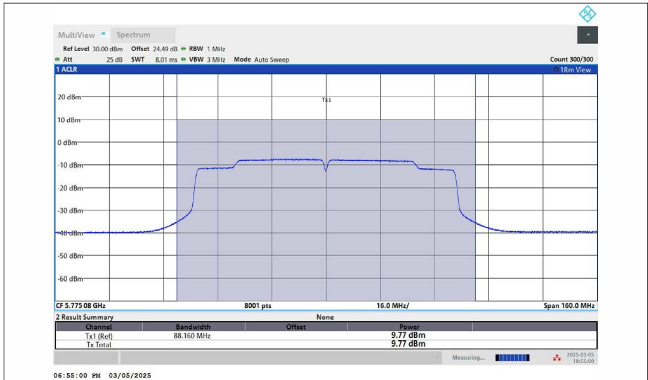
11AC80MIMO-Ant2-5775-PASS
