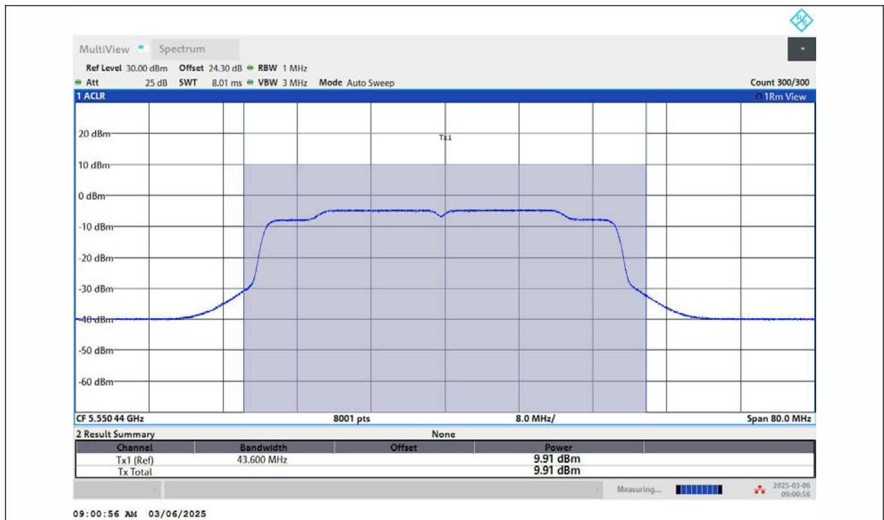
11AX40MIMO-Ant2-5550-PASS
