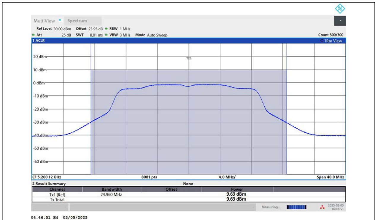
11AC20MIMO-Ant2-5200-PASS
