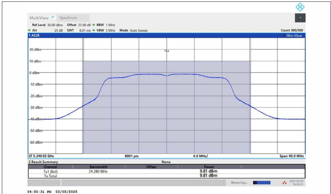
11AC20MIMO-Ant2-5240-PASS
