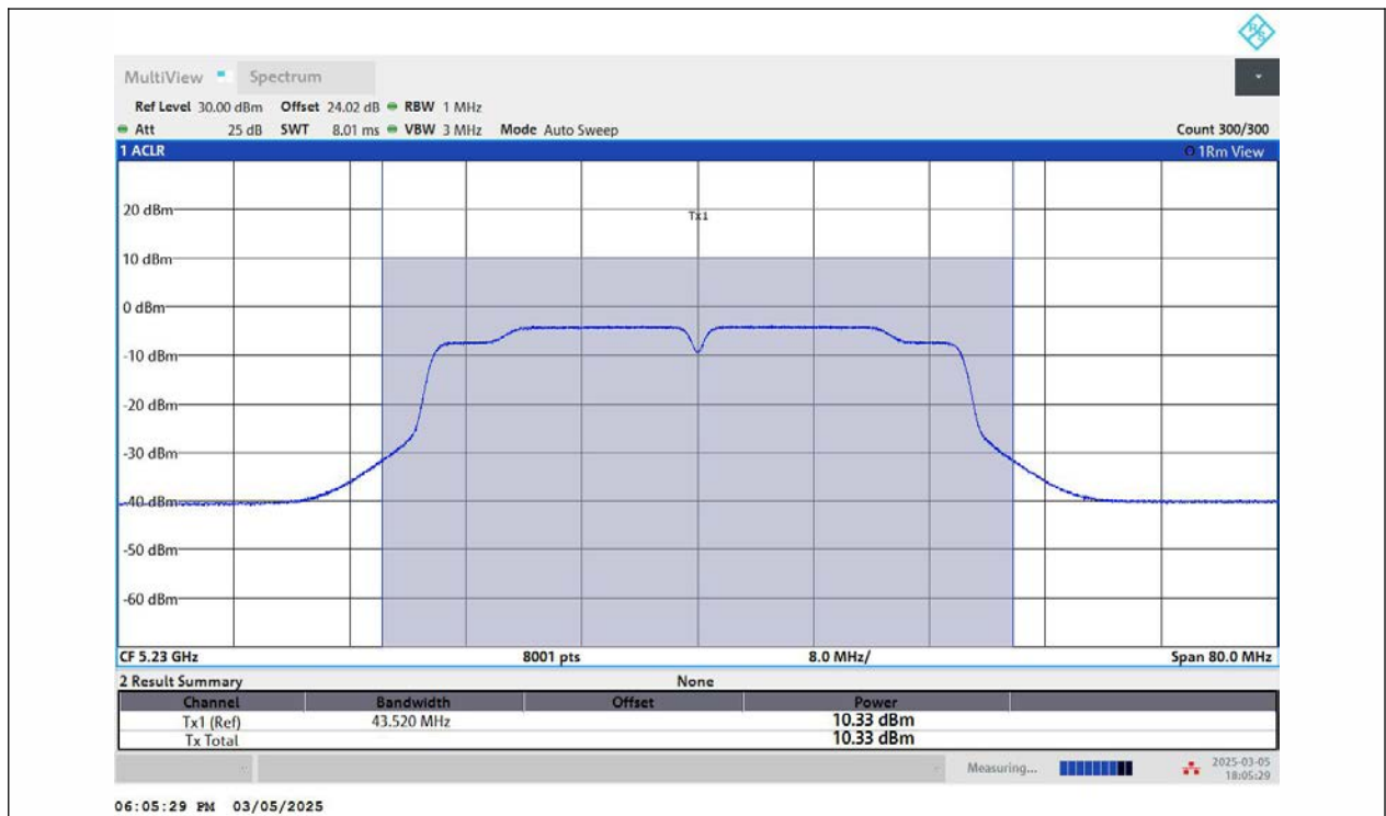
11AC40MIMO-Ant2-5230-PASS
