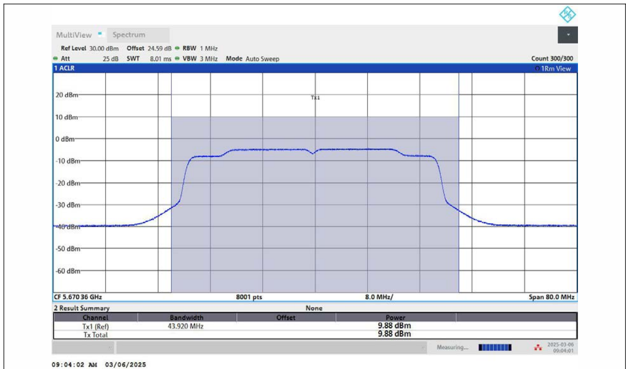
11AX40MIMO-Ant2-5670-PASS
