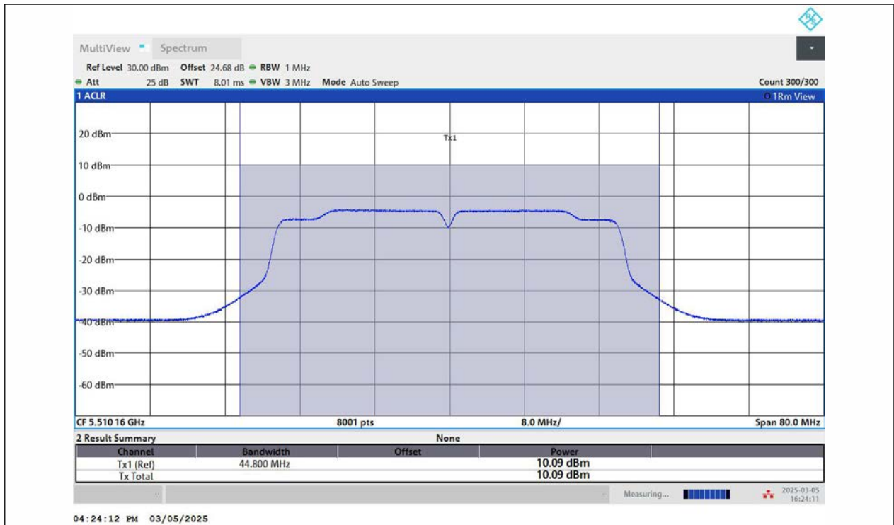
11N40MIMO-Ant2-5510-PASS
