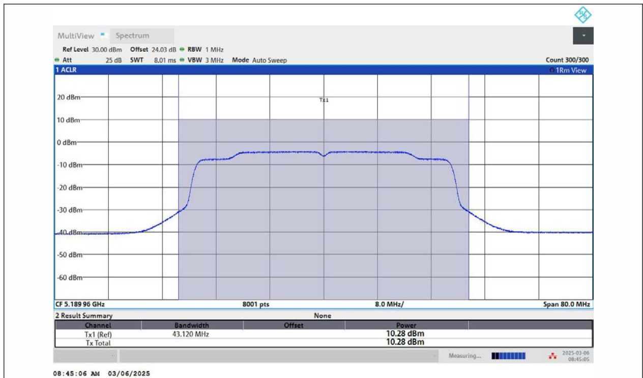
11AX40MIMO-Ant2-5190-PASS
