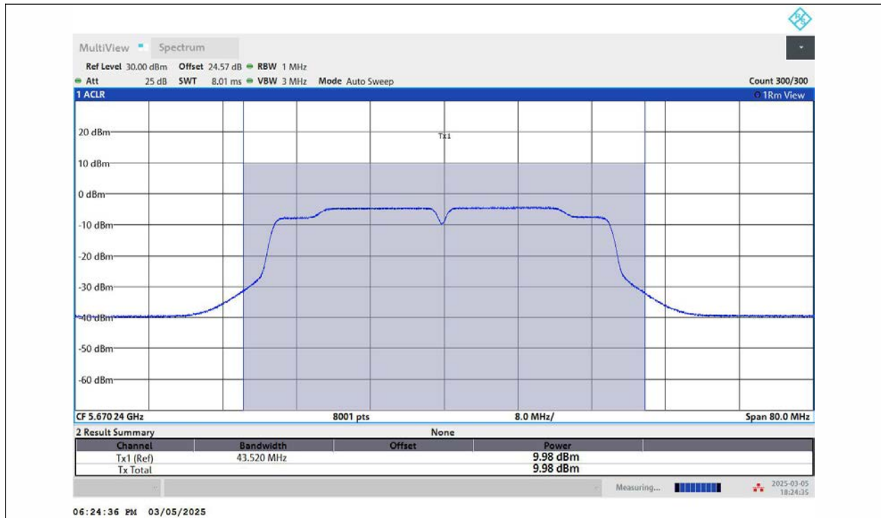
11AC40MIMO-Ant2-5670-PASS
