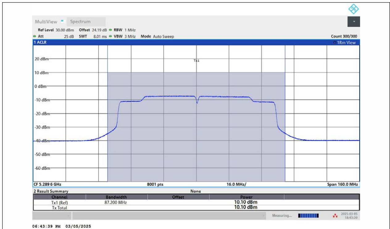
11AC80MIMO-Ant2-5290-PASS
