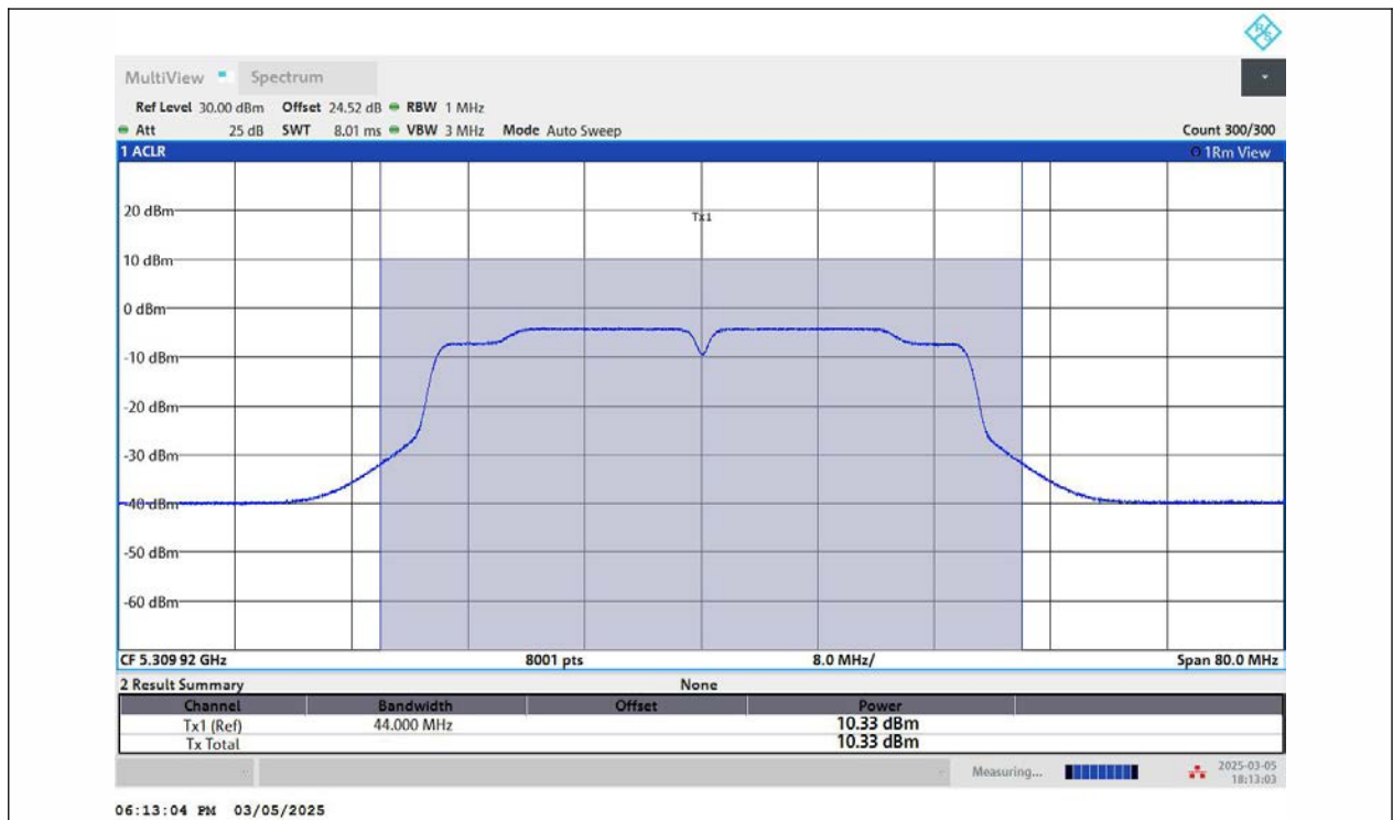
11AC40MIMO-Ant2-5310-PASS
