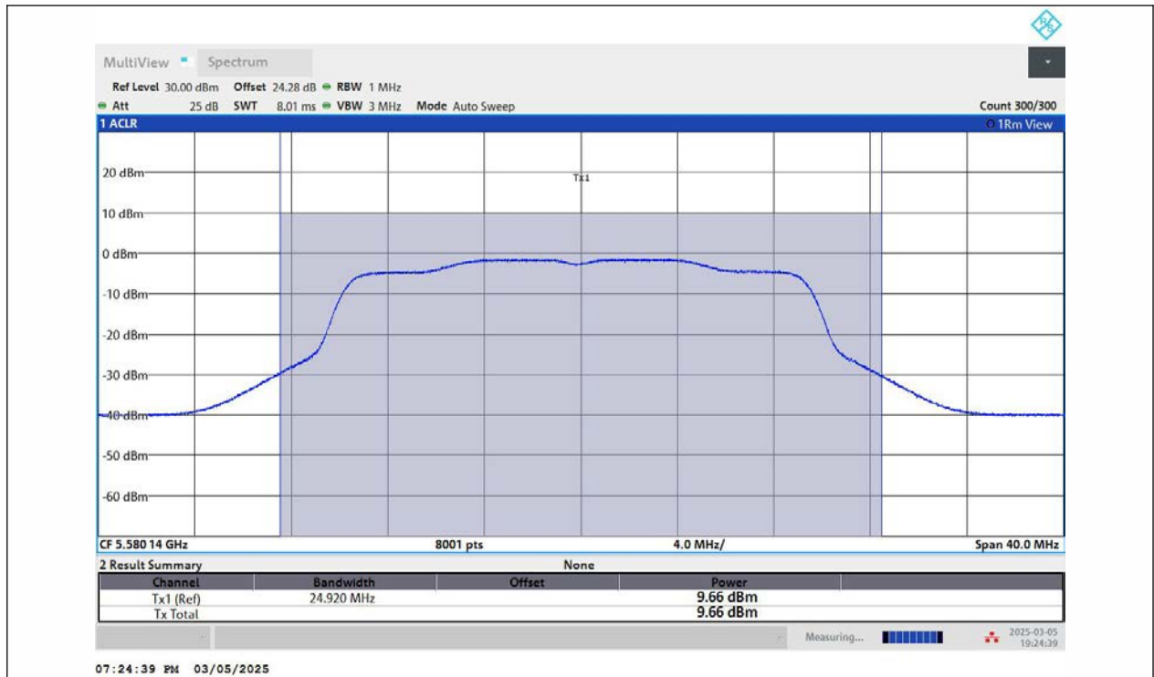
11AX20MIMO-Ant2-5580-PASS
