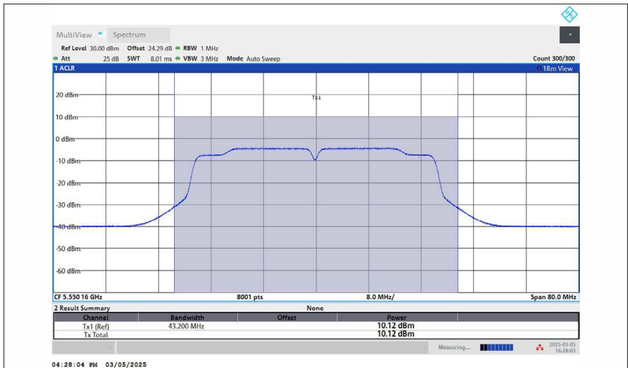
11N40MIMO-Ant2-5550-PASS
