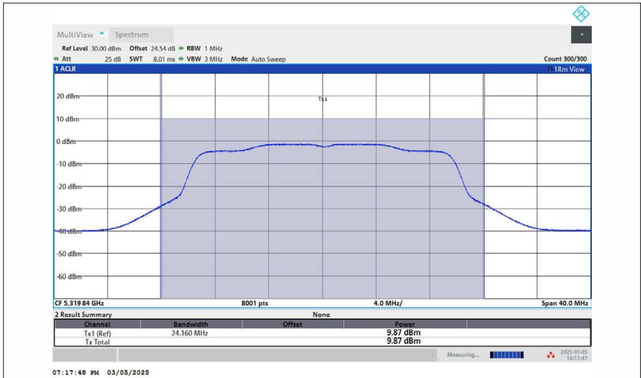
11AX20MIMO-Ant2-5320-PASS
