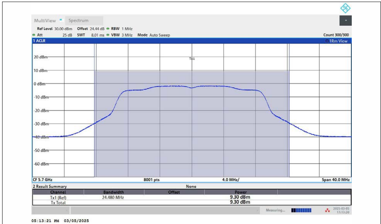
11AC20MIMO-Ant2-5700-PASS
