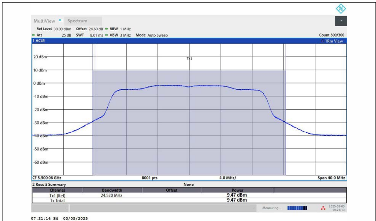
11AX20MIMO-Ant2-5500-PASS
