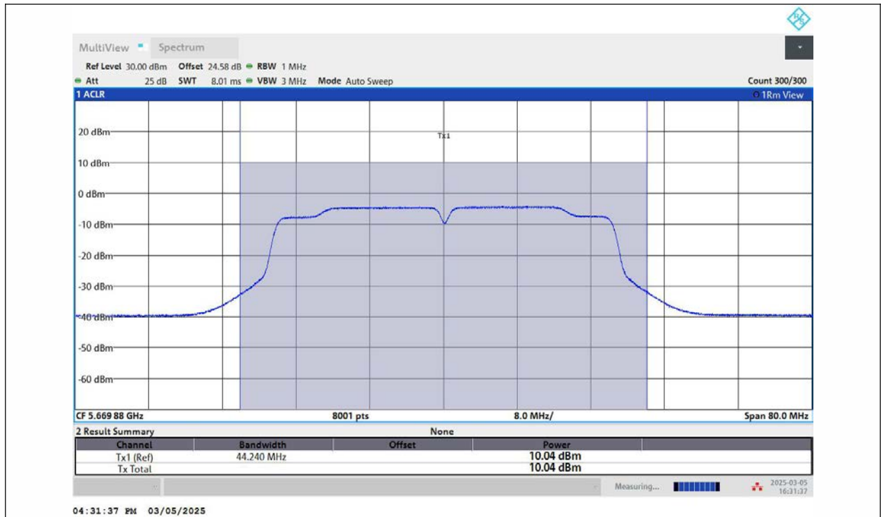
11N40MIMO-Ant2-5670-PASS
