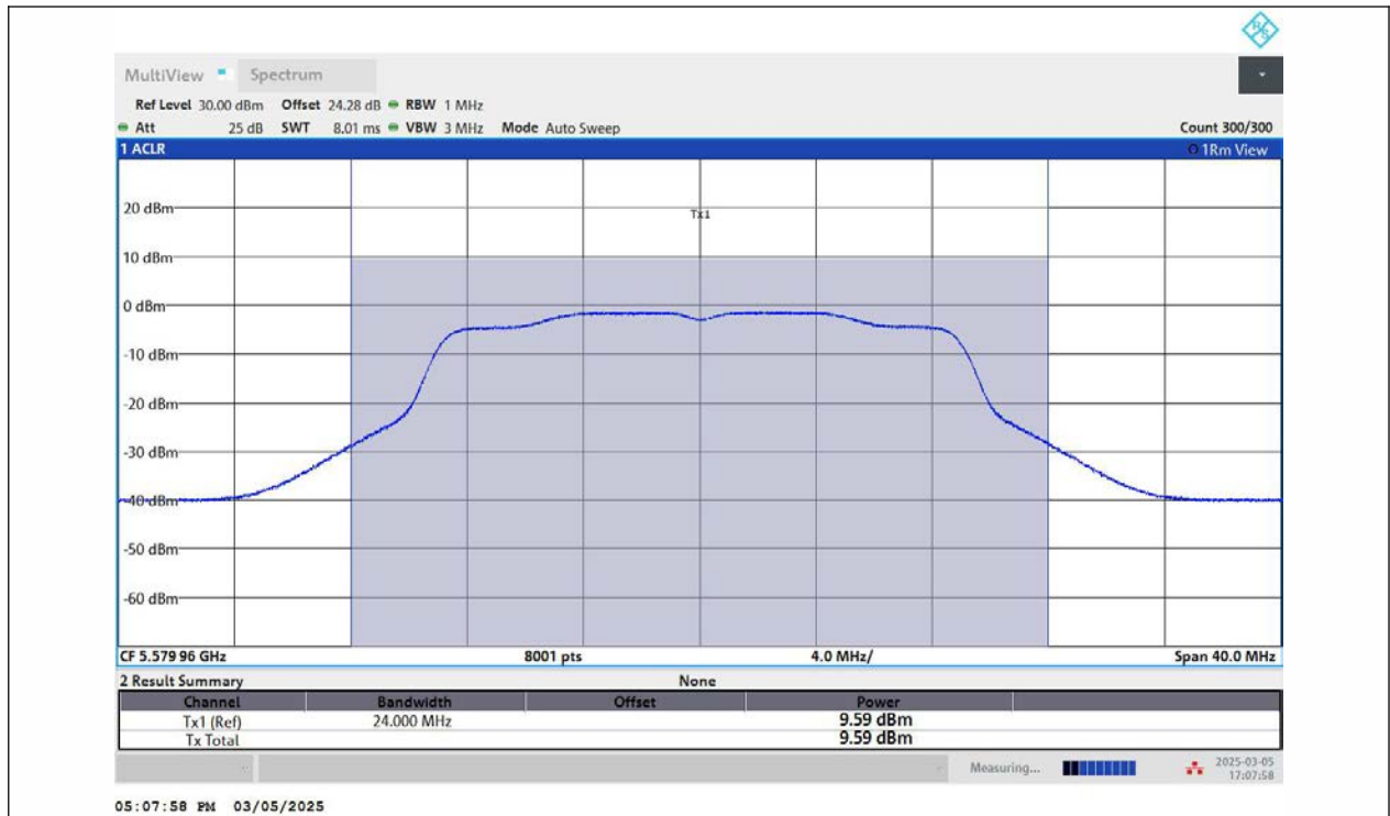
11AC20MIMO-Ant2-5580-PASS
