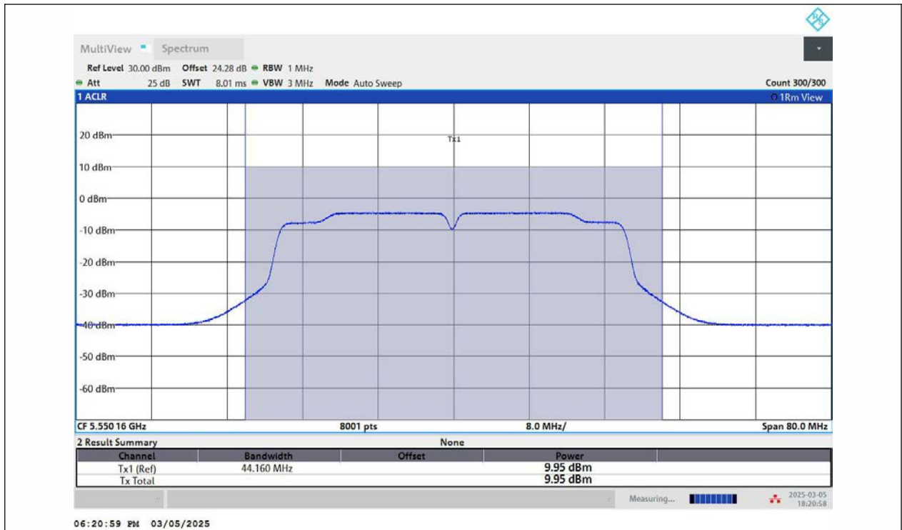
11AC40MIMO-Ant2-5550-PASS
