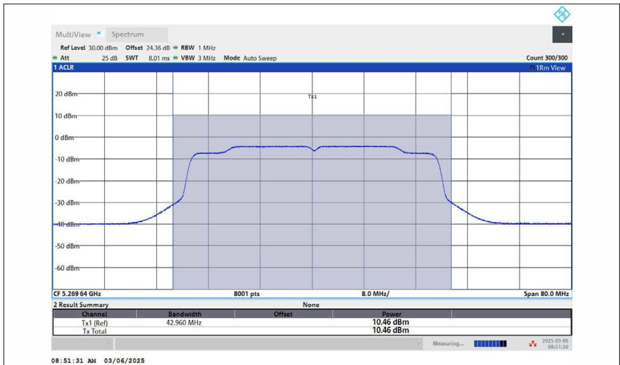
11AX40MIMO-Ant2-5270-PASS
