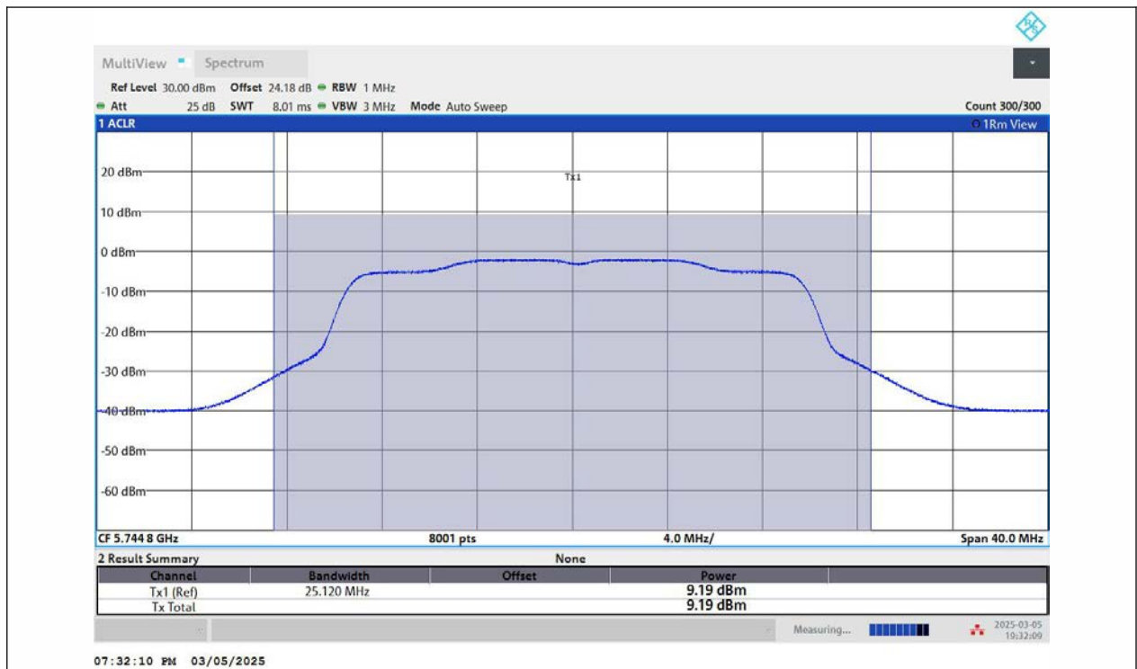
11AX20MIMO-Ant2-5745-PASS
