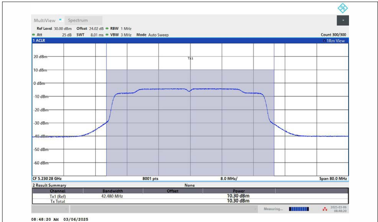
11AX40MIMO-Ant2-5230-PASS
