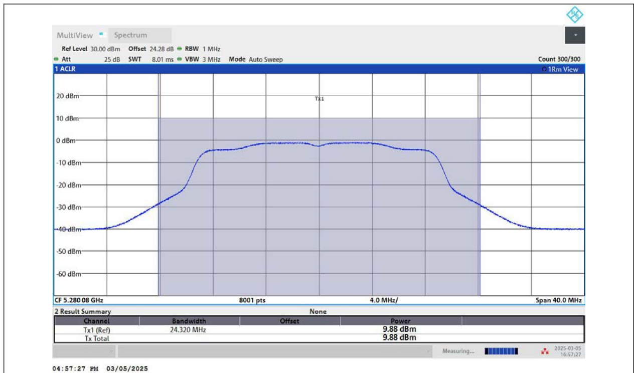
11AC20MIMO-Ant2-5280-PASS
