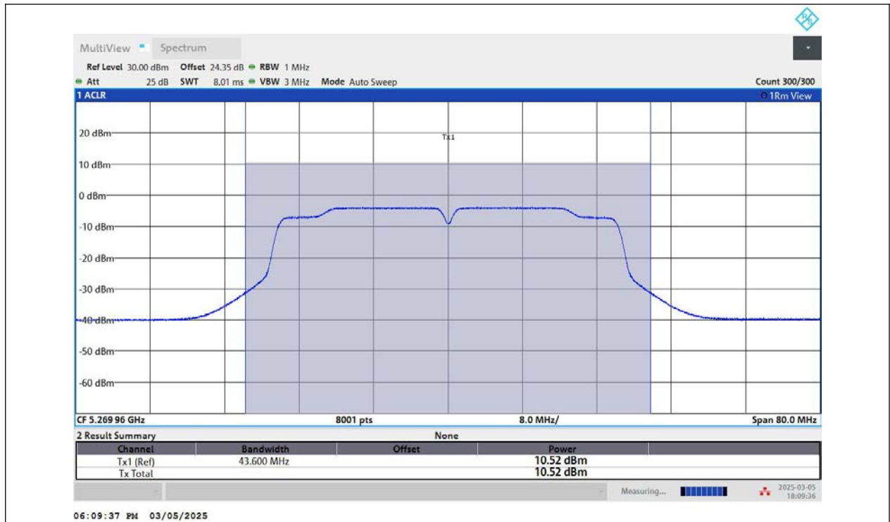
11AC40MIMO-Ant2-5270-PASS
