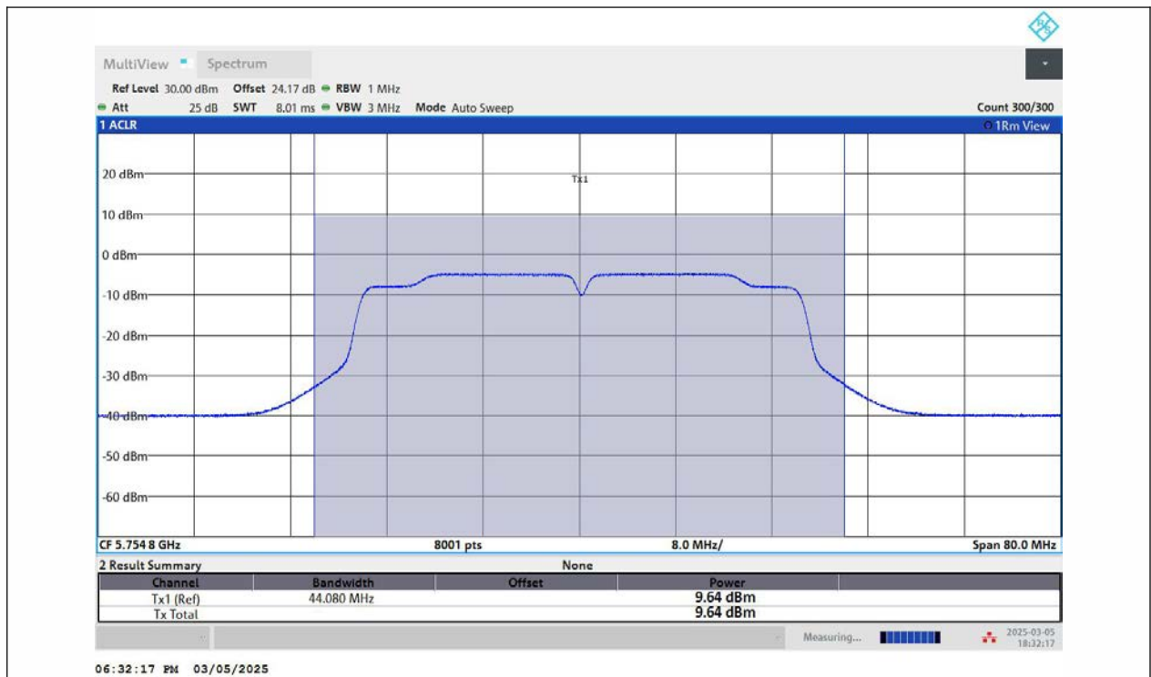
11AC40MIMO-Ant2-5755-PASS
