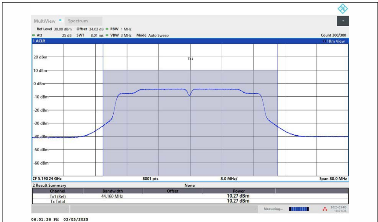
11AC40MIMO-Ant2-5190-PASS
