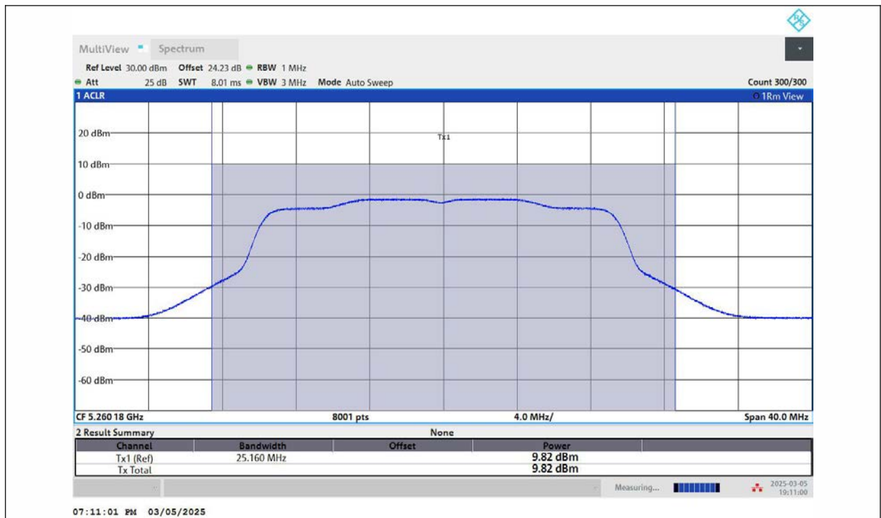
11AX20MIMO-Ant2-5260-PASS
