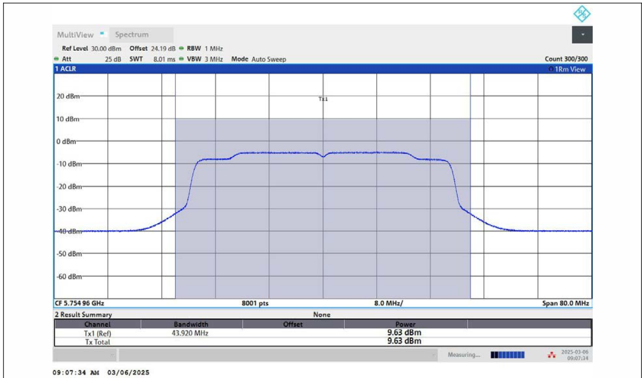
11AX40MIMO-Ant2-5755-PASS
