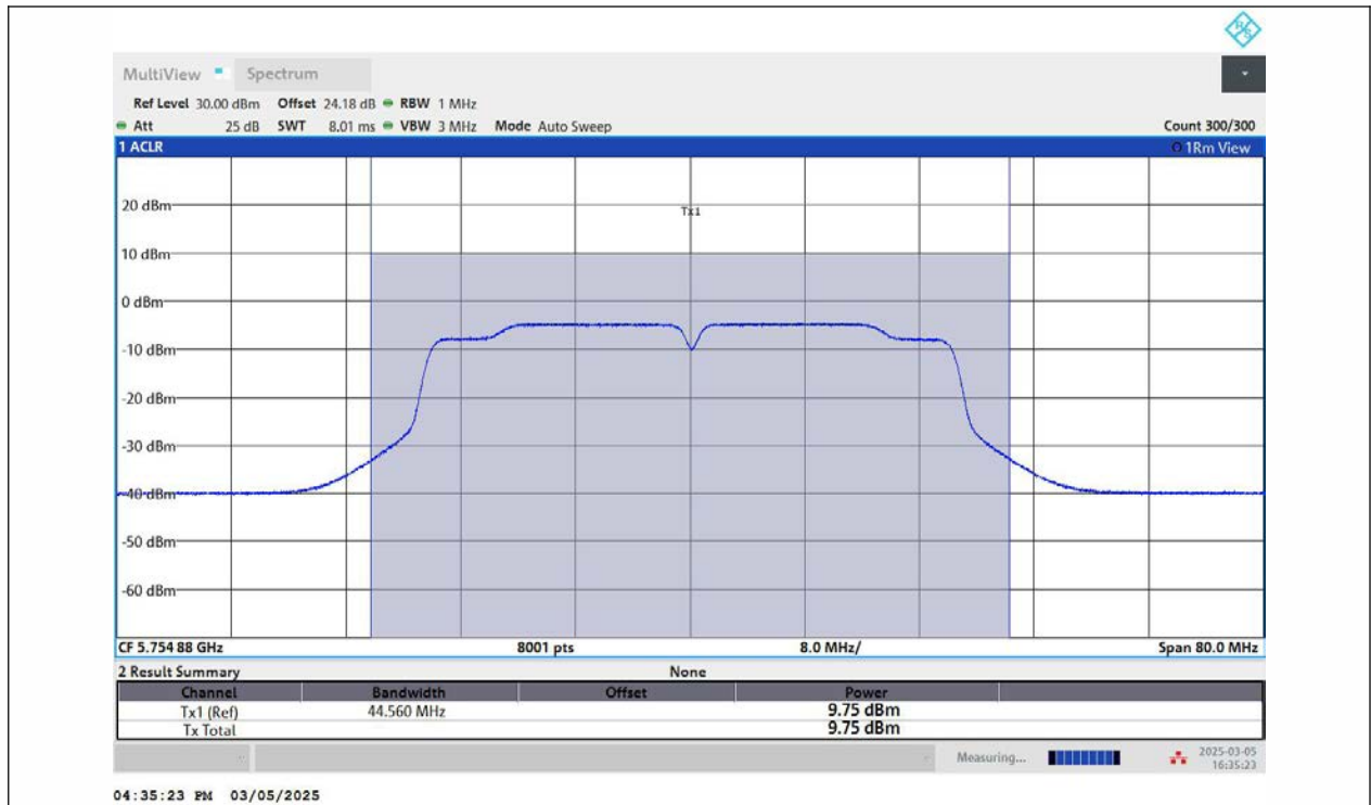
11N40MIMO-Ant2-5755-PASS
