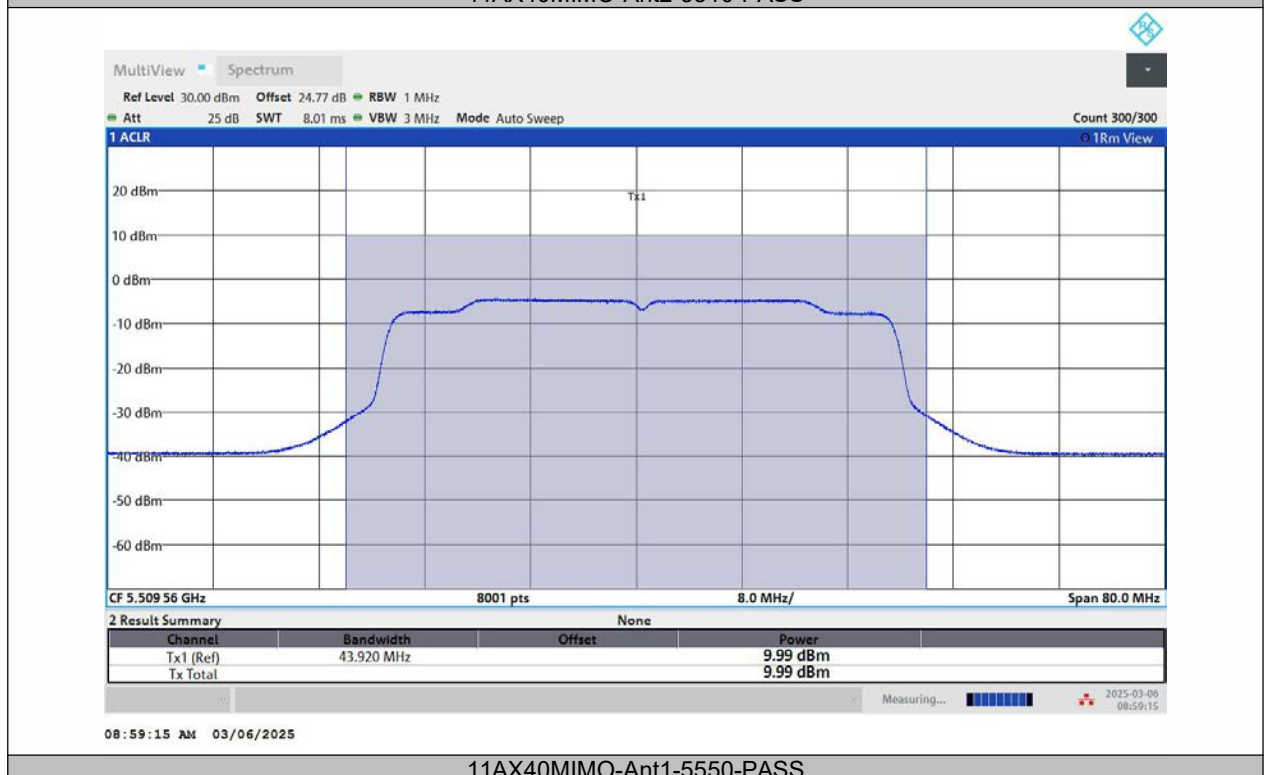
11AX40MIMO-Ant1-5550-PASS
