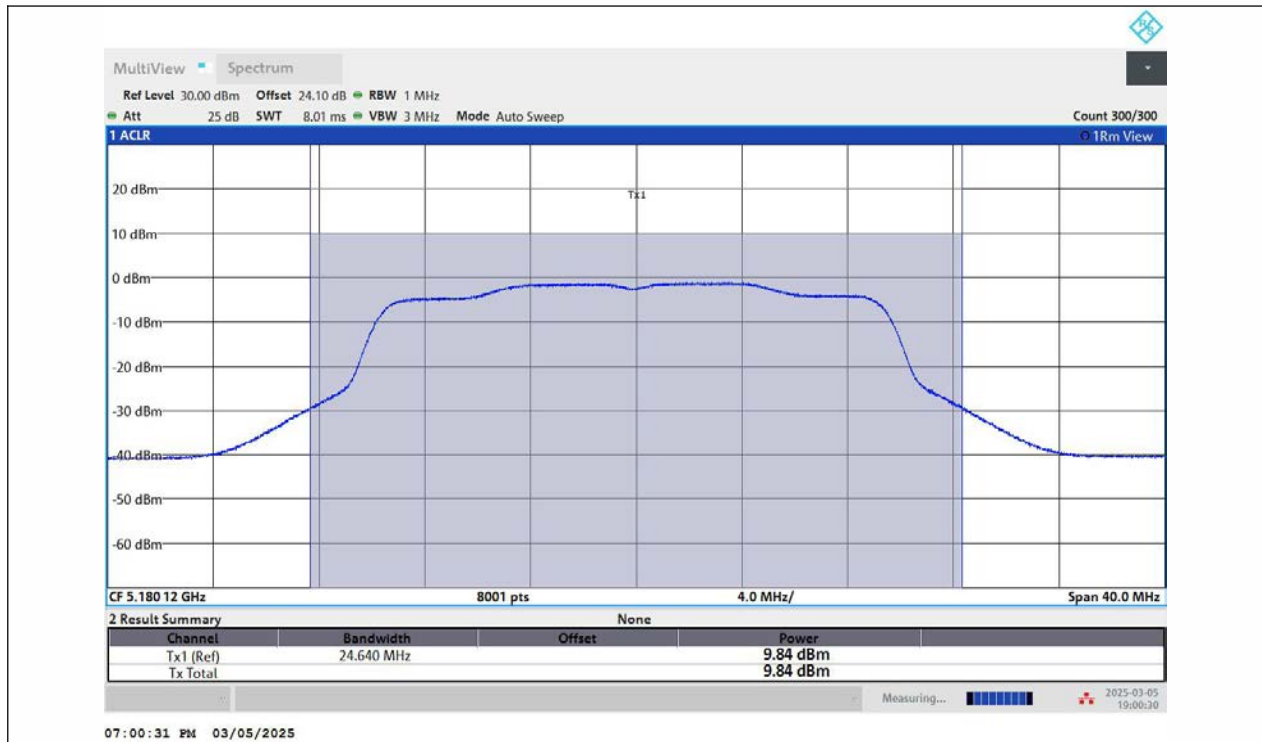
11AX20MIMO-Ant2-5180-PASS
