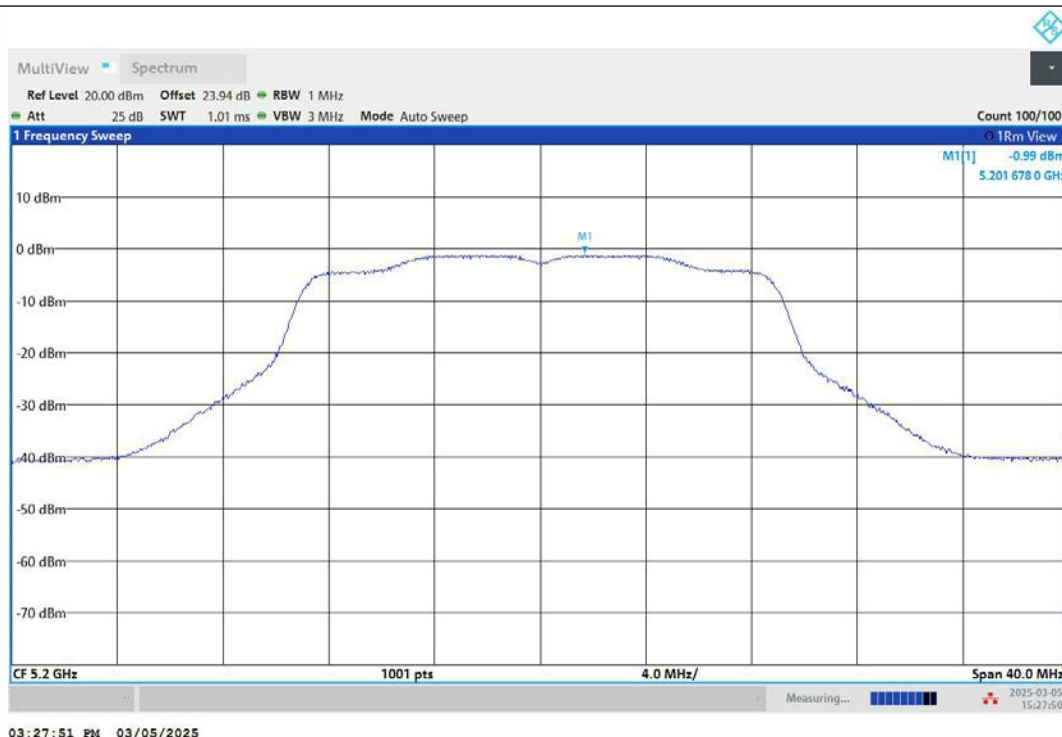
11N20MIMO-Ant2-5200-PASS
