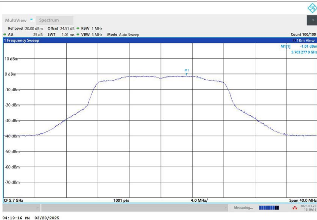
11A-Ant2-5700-PASS
