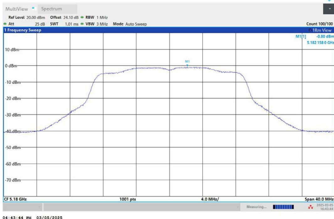
11AC20MIMO-Ant2-5180-PASS
