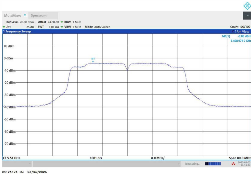
11N40MIMO-Ant2-5510-PASS
