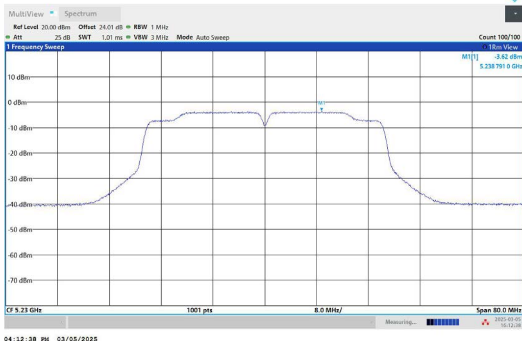
11N40MIMO-Ant2-5230-PASS
