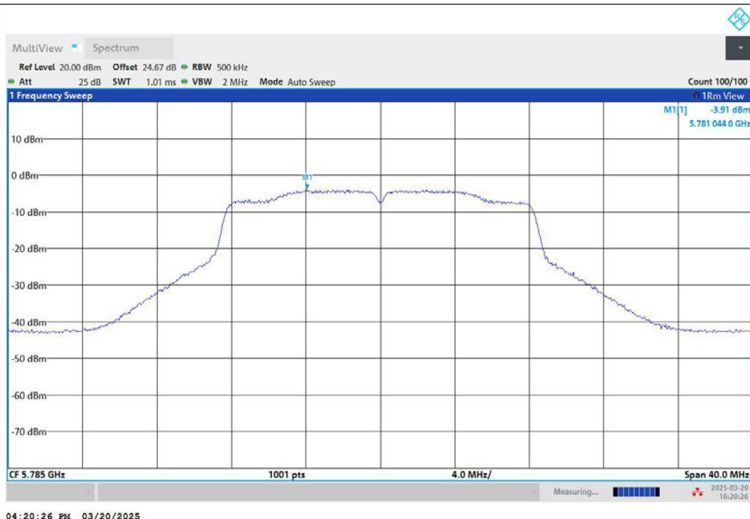
11A-Ant2-5785-PASS
