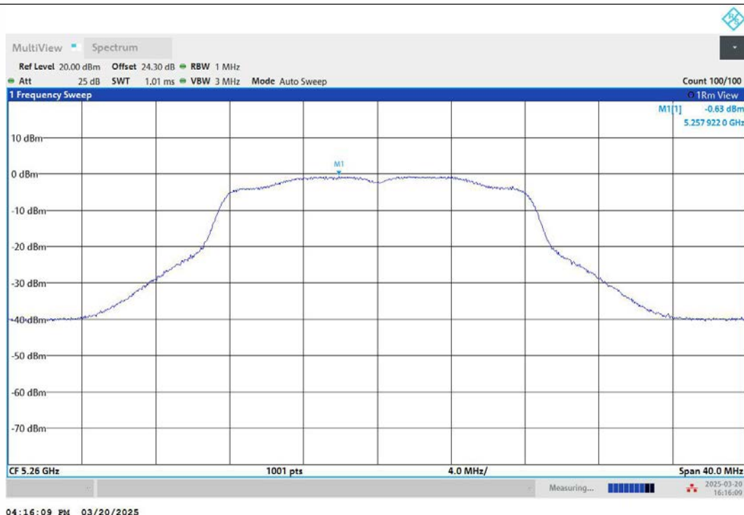
11A-Ant2-5260-PASS
