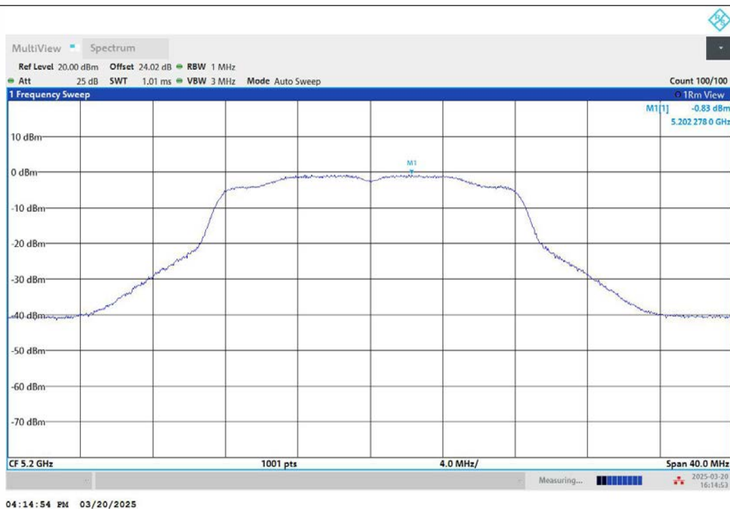
11A-Ant2-5200-PASS
