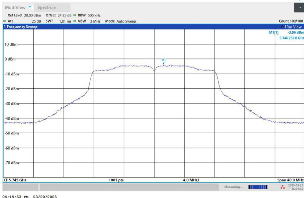
11A-Ant2-5745-PASS
