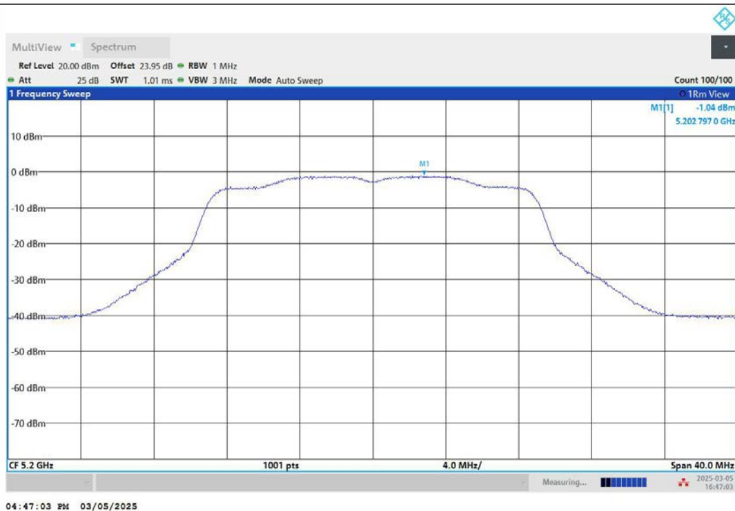
11AC20MIMO-Ant2-5200-PASS
