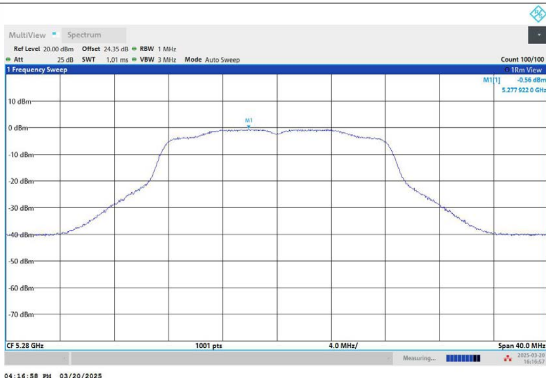
11A-Ant2-5280-PASS
