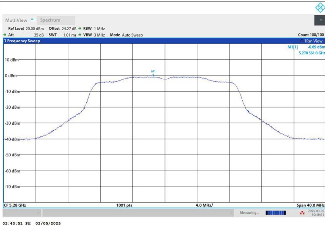
11N20MIMO-Ant2-5280-PASS
