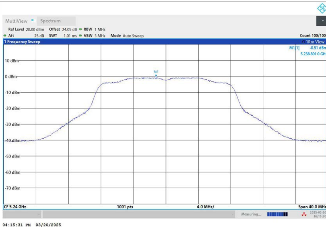
11A-Ant2-5240-PASS
