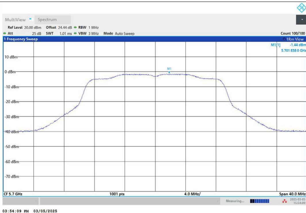
11N20MIMO-Ant2-5700-PASS
