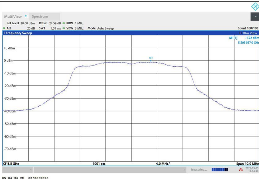
11AC20MIMO-Ant2-5500-PASS
