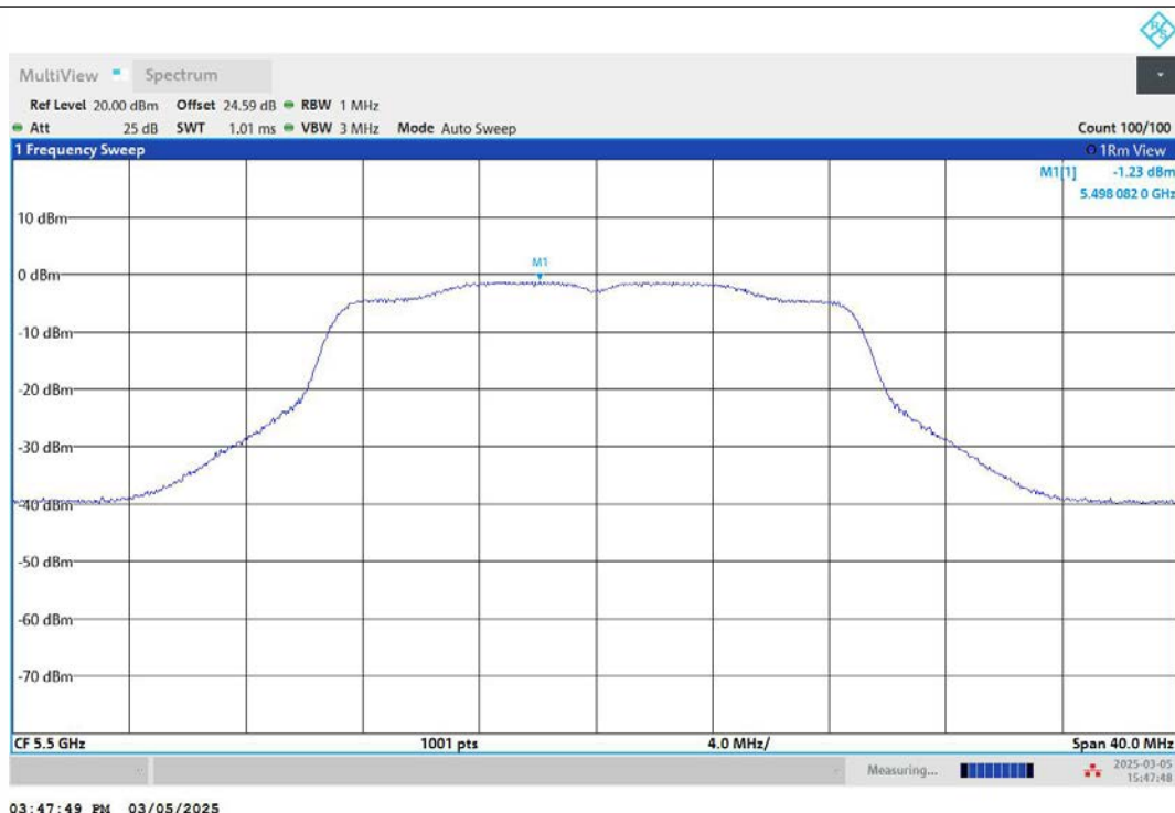
11N20MIMO-Ant2-5500-PASS
