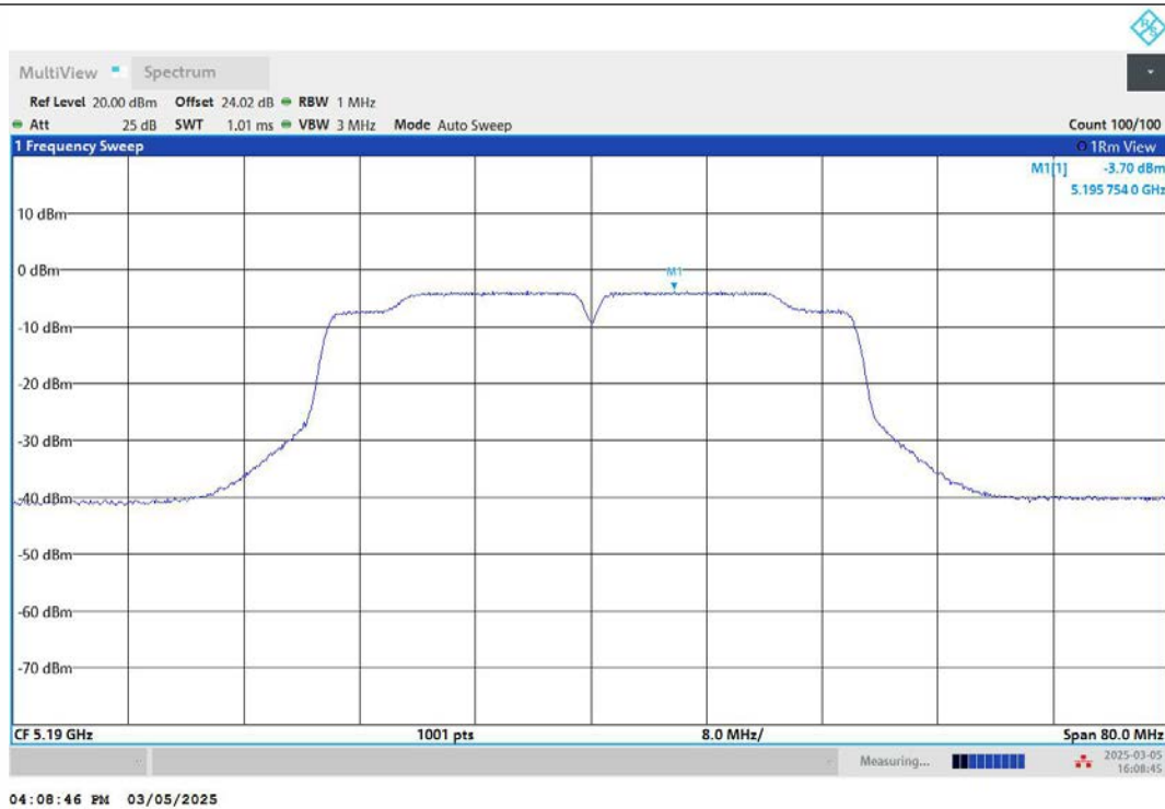
11N40MIMO-Ant2-5190-PASS
