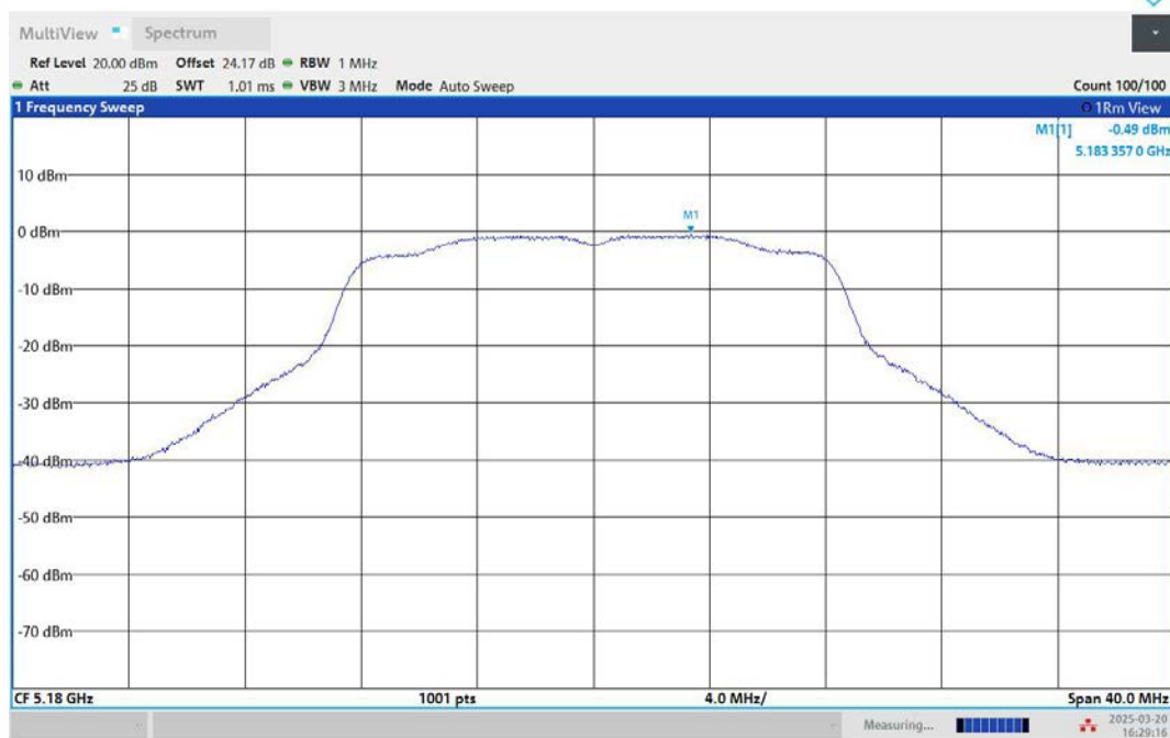
11A-Ant2-5180-PASS
