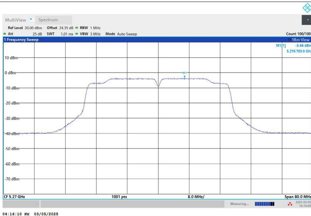
11N40MIMO-Ant2-5270-PASS
