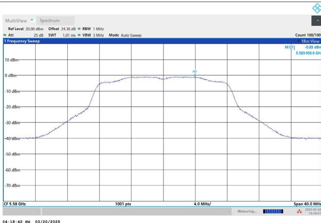
11A-Ant2-5580-PASS
