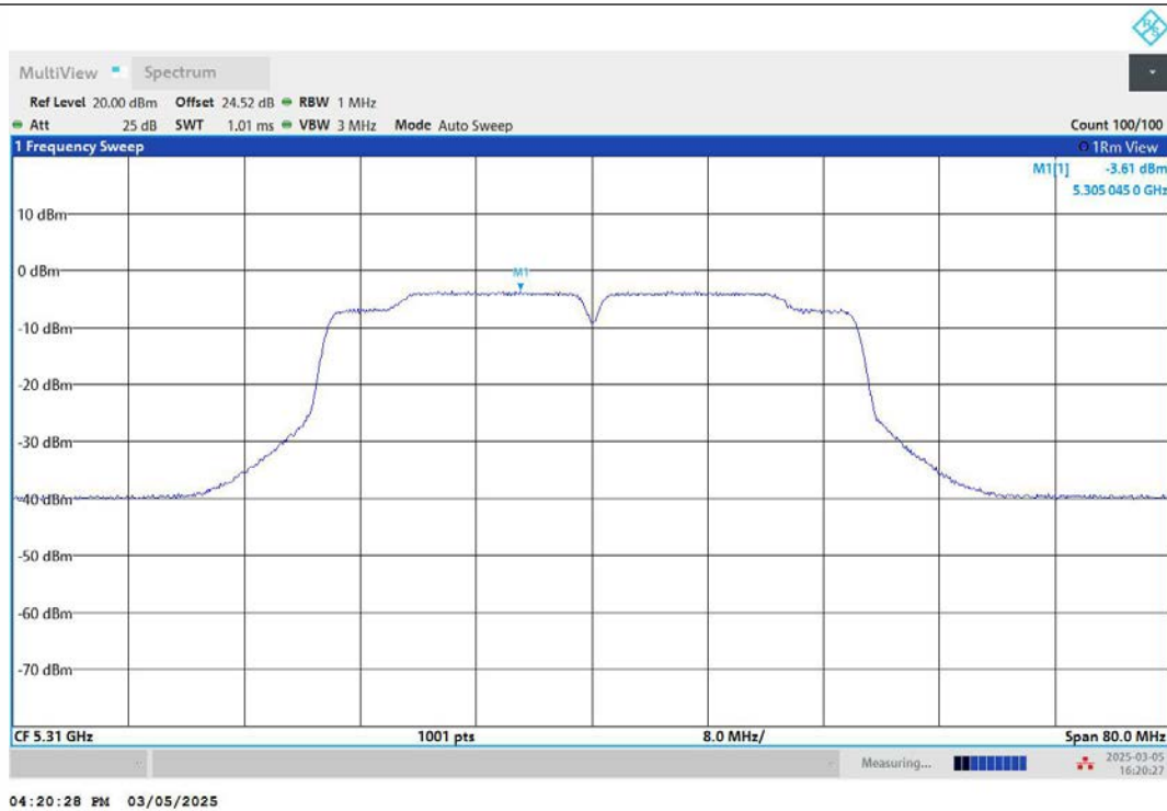
11N40MIMO-Ant2-5310-PASS
