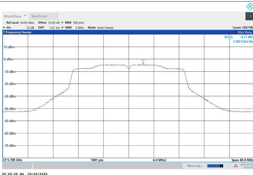
11AC20MIMO-Ant2-5785-PASS
