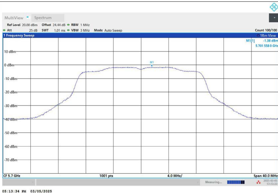
11AC20MIMO-Ant2-5700-PASS
