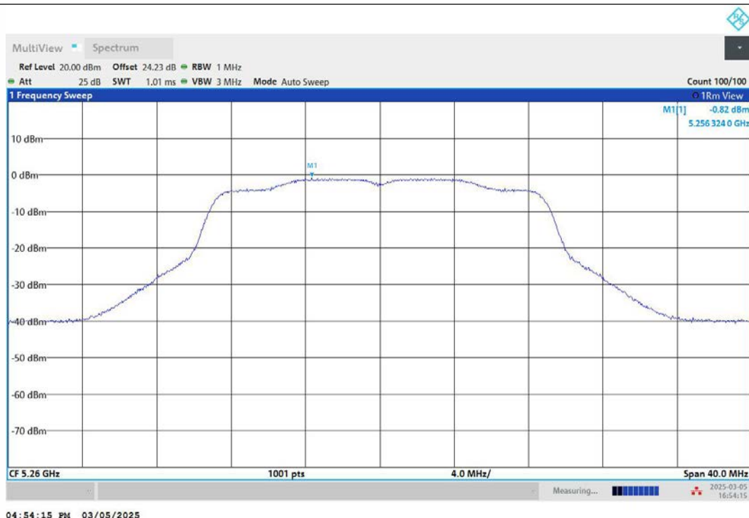
11AC20MIMO-Ant2-5260-PASS
