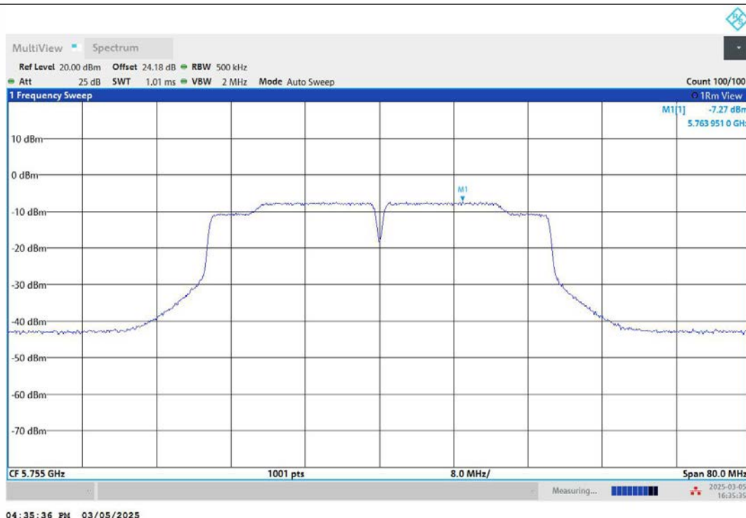
11N40MIMO-Ant2-5755-PASS
