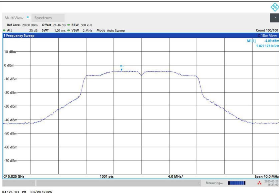
11A-Ant2-5825-PASS
