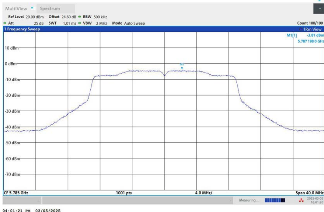
11N20MIMO-Ant2-5785-PASS
