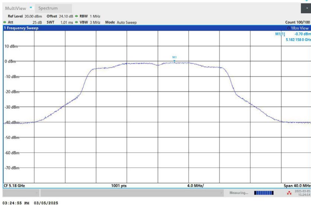
11N20MIMO-Ant2-5180-PASS
