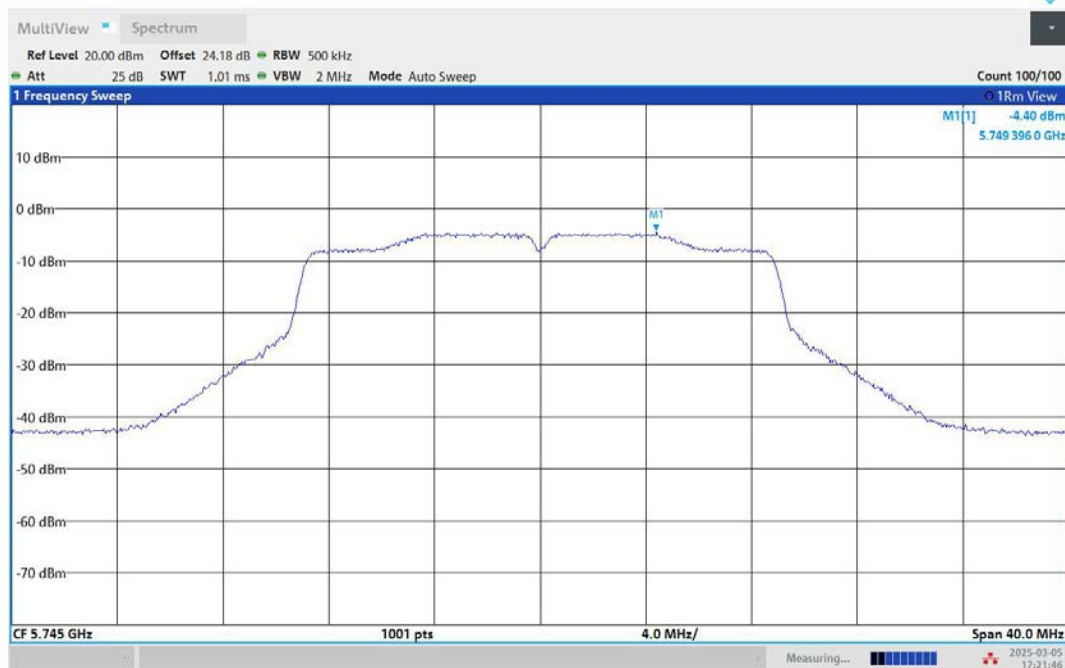
11AC20MIMO-Ant2-5745-PASS
