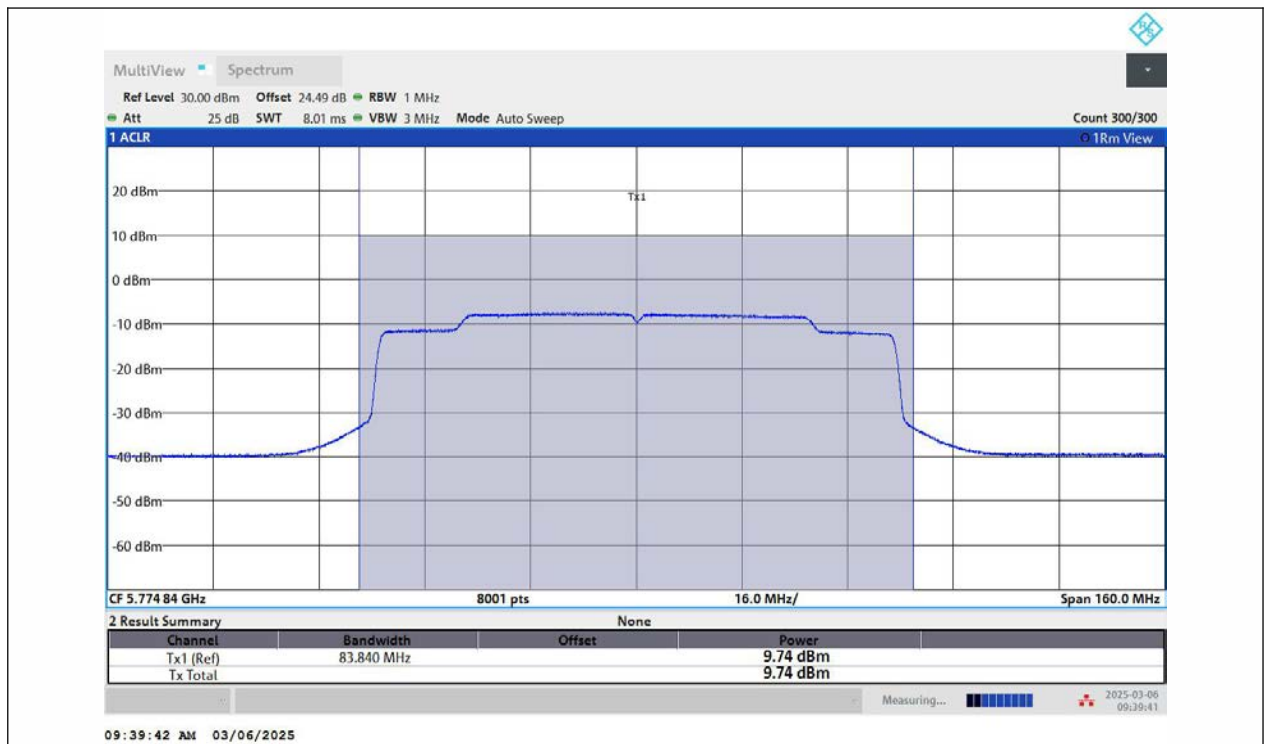
11AX80MIMO-Ant2-5775-PASS
