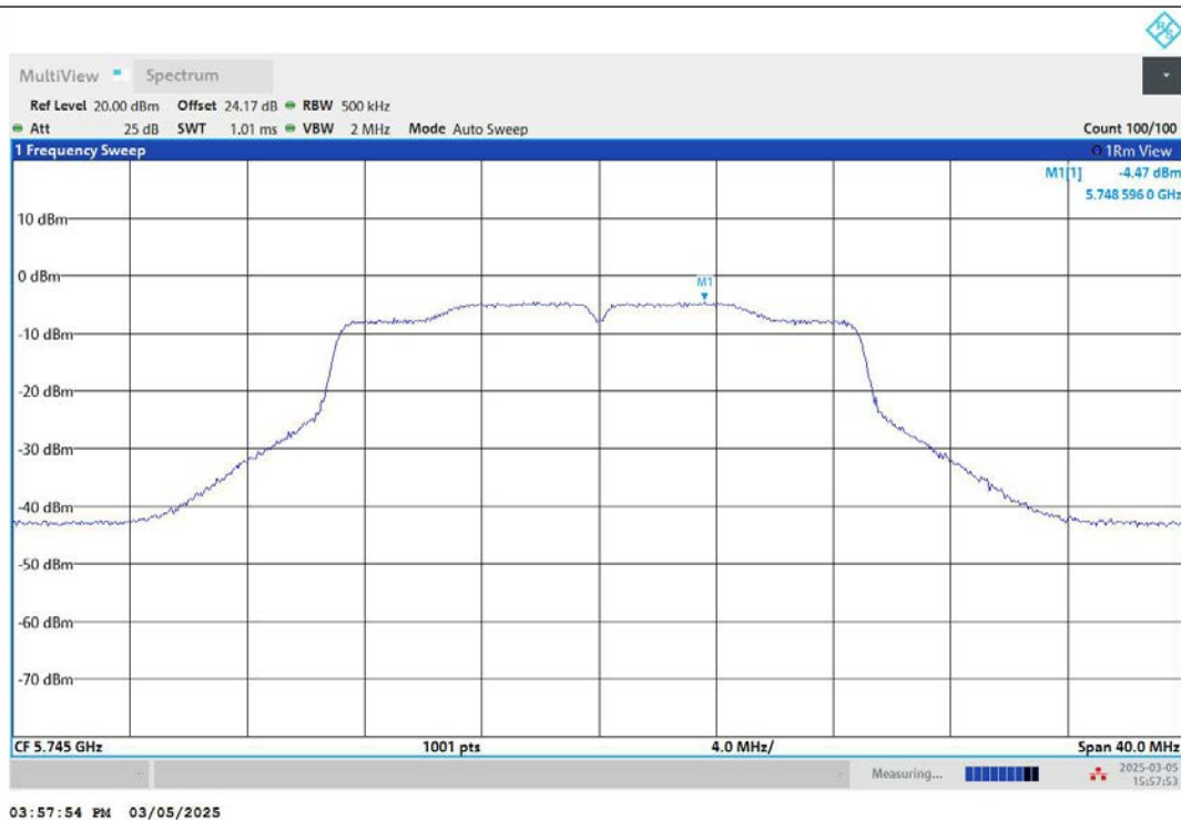
11N20MIMO-Ant2-5745-PASS
