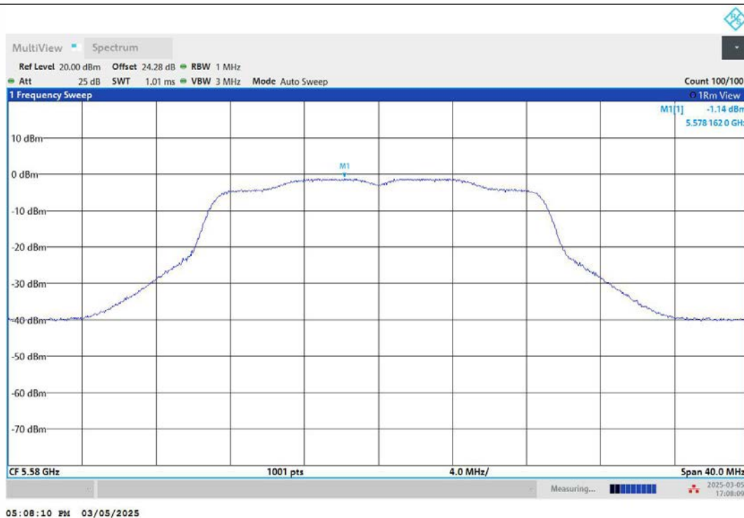
11AC20MIMO-Ant2-5580-PASS
