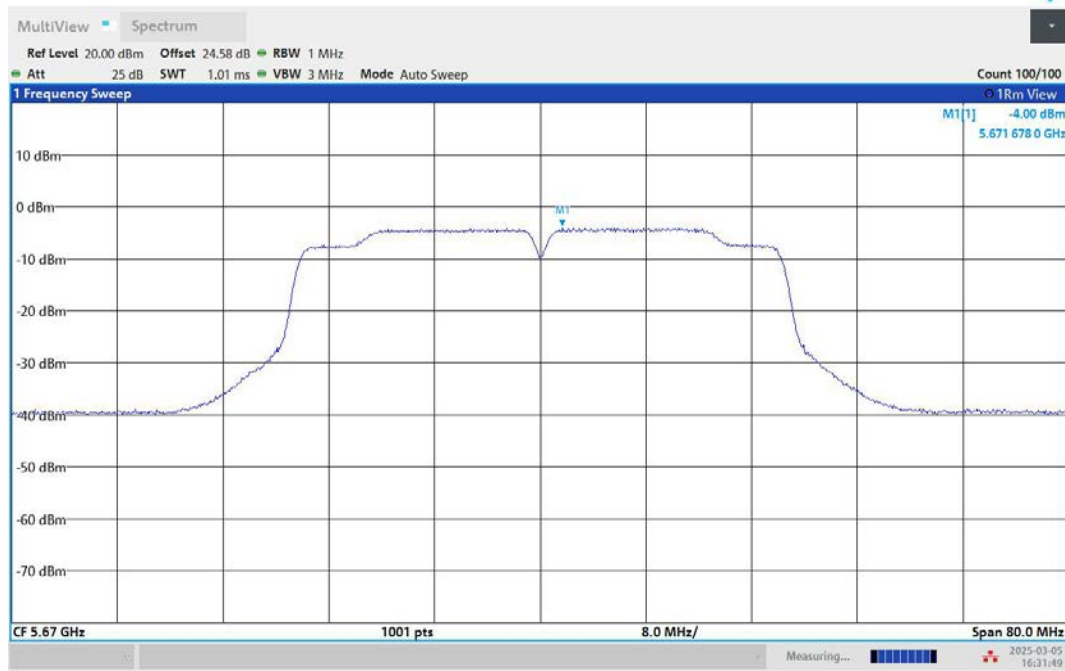
11N40MIMO-Ant2-5670-PASS
