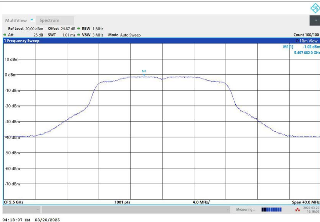
11A-Ant2-5500-PASS
