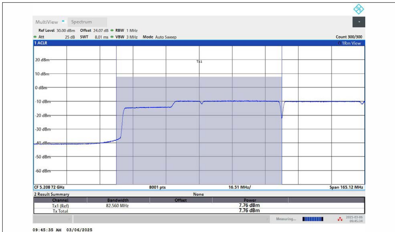
11AX160MIMO-Ant2-5250_UNII-1-PASS
