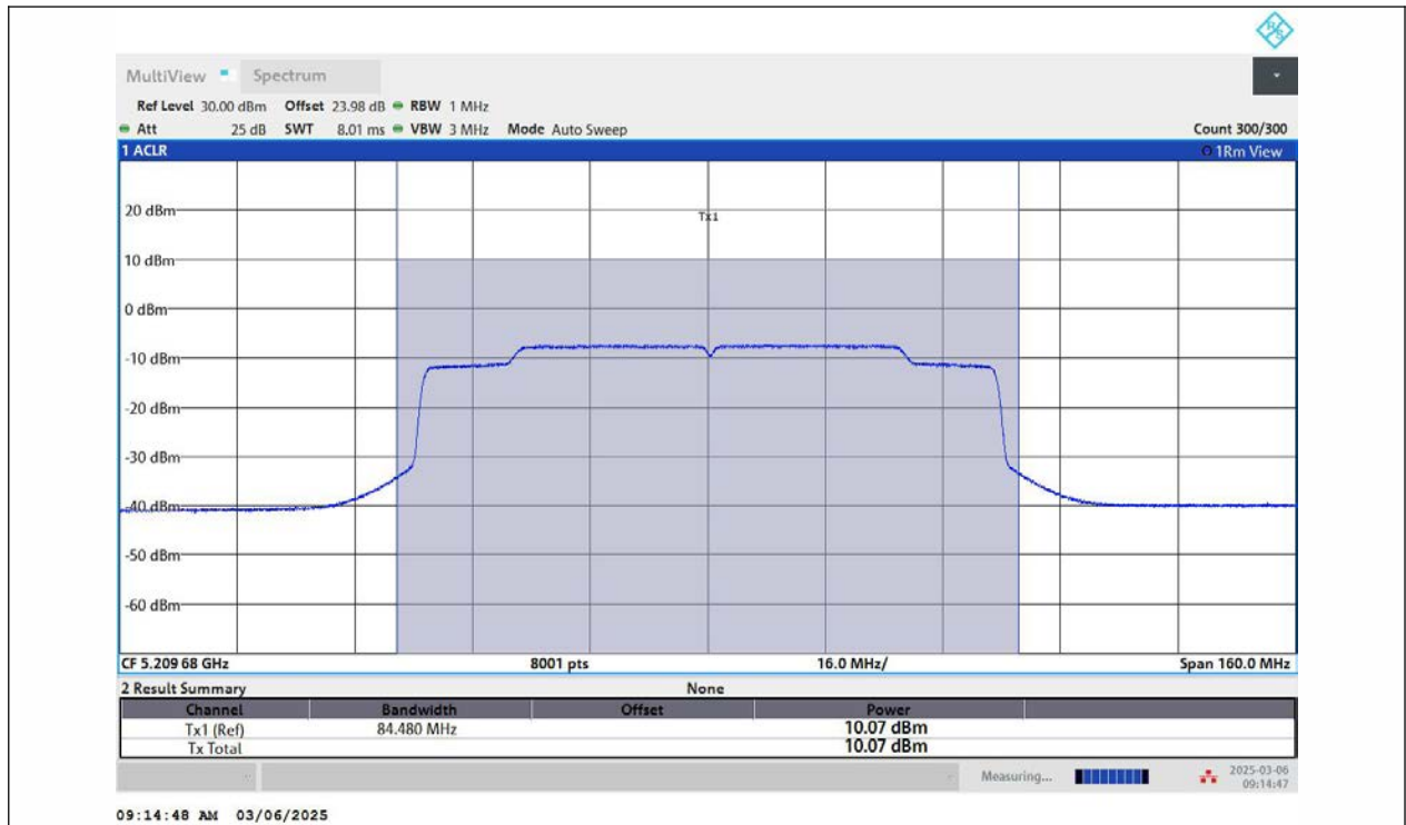
11AX80MIMO-Ant2-5210-PASS
