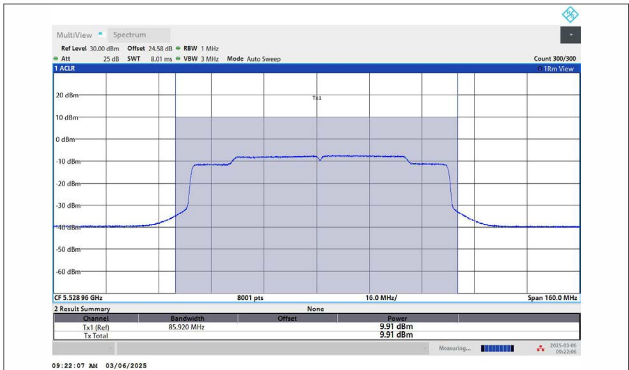
11AX80MIMO-Ant2-5530-PASS
