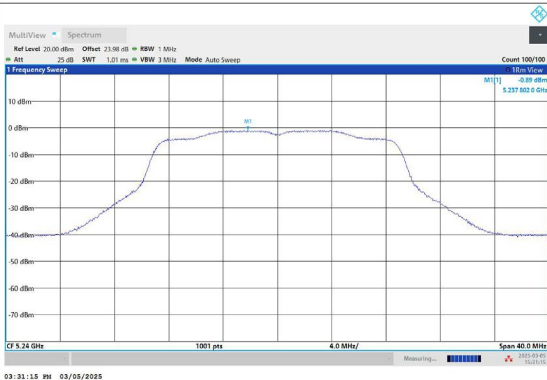
11N20MIMO-Ant2-5240-PASS
