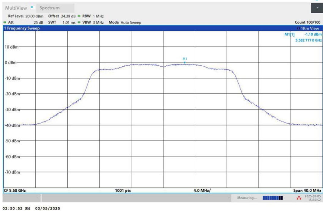
11N20MIMO-Ant2-5580-PASS
