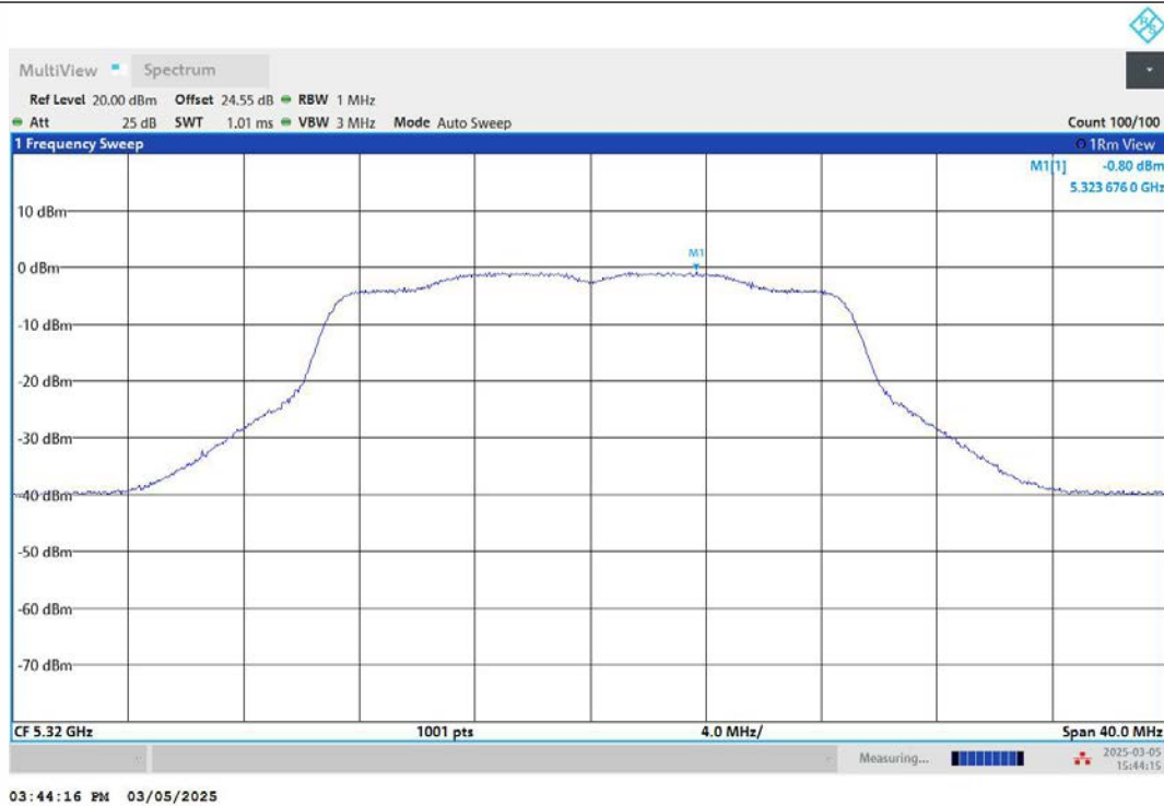
11N20MIMO-Ant2-5320-PASS
