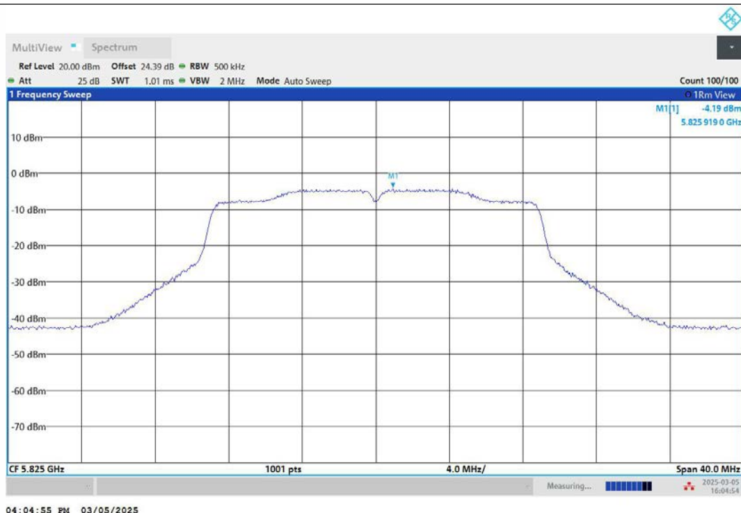
11N20MIMO-Ant2-5825-PASS
