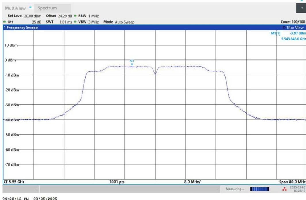
11N40MIMO-Ant2-5550-PASS
