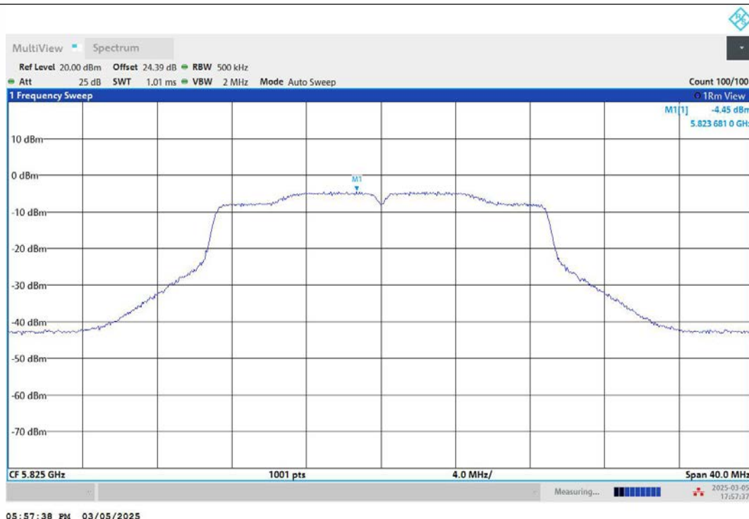
11AC20MIMO-Ant2-5825-PASS
