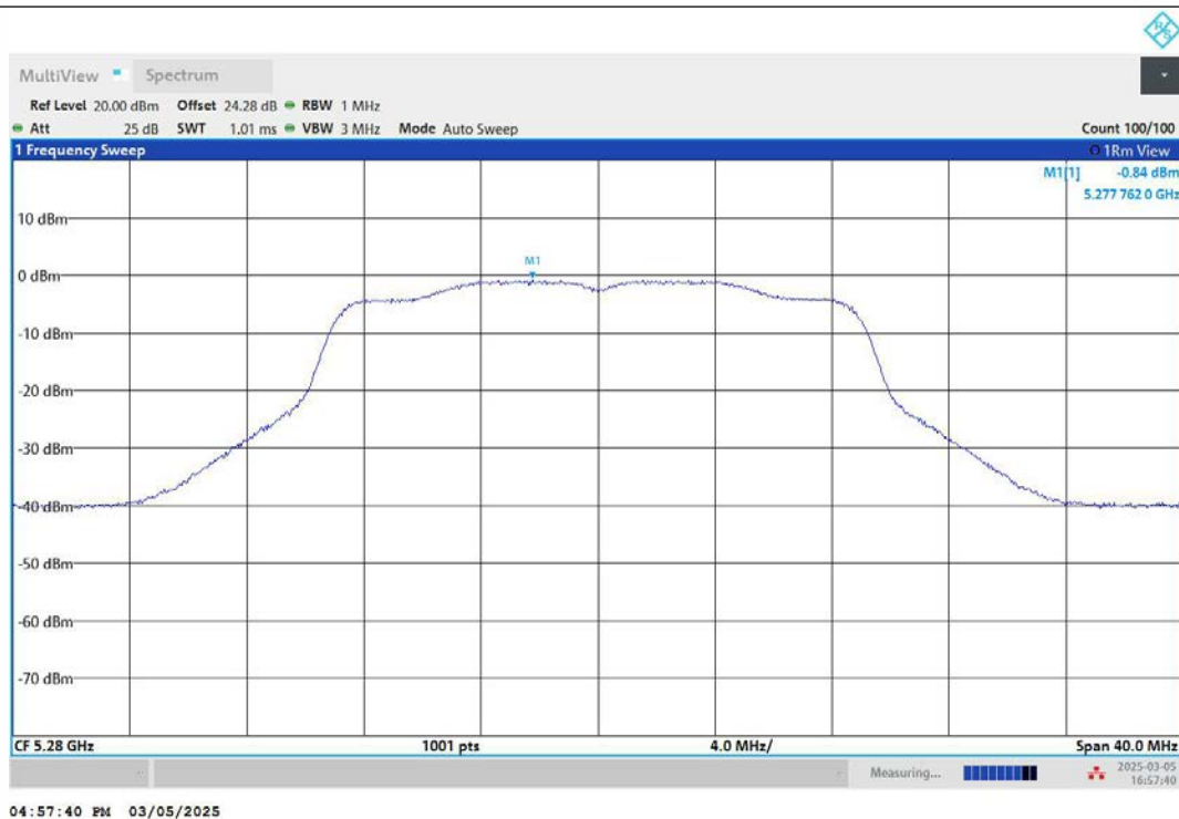
11AC20MIMO-Ant2-5280-PASS
