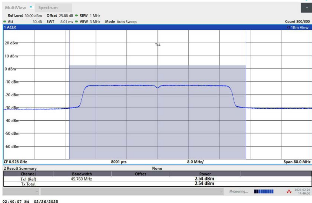
11AX40MIMO-Ant2-6925-PASS
