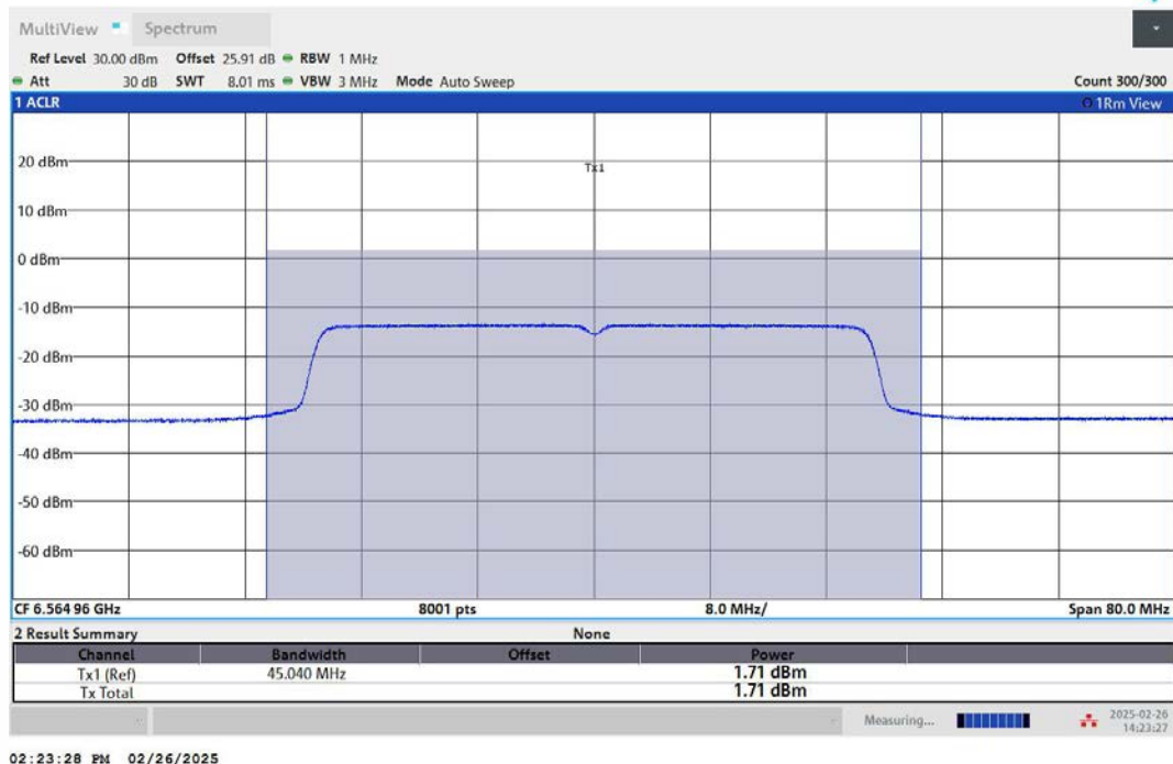
11AX40MIMO-Ant2-6565-PASS
