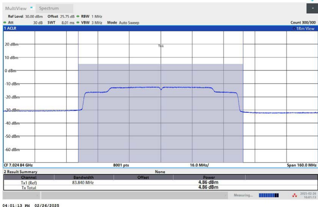
11AX80MIMO-Ant2-7025-PASS
