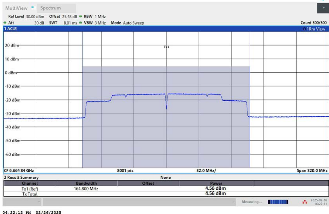
11AX160MIMO-Ant2-6665-PASS
