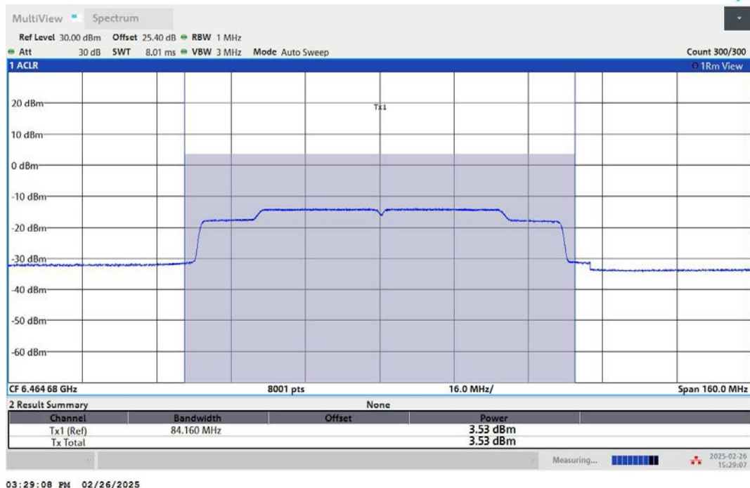
11AX80MIMO-Ant2-6465-PASS
