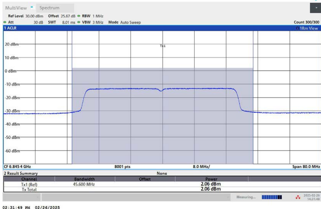
11AX40MIMO-Ant2-6845-PASS
