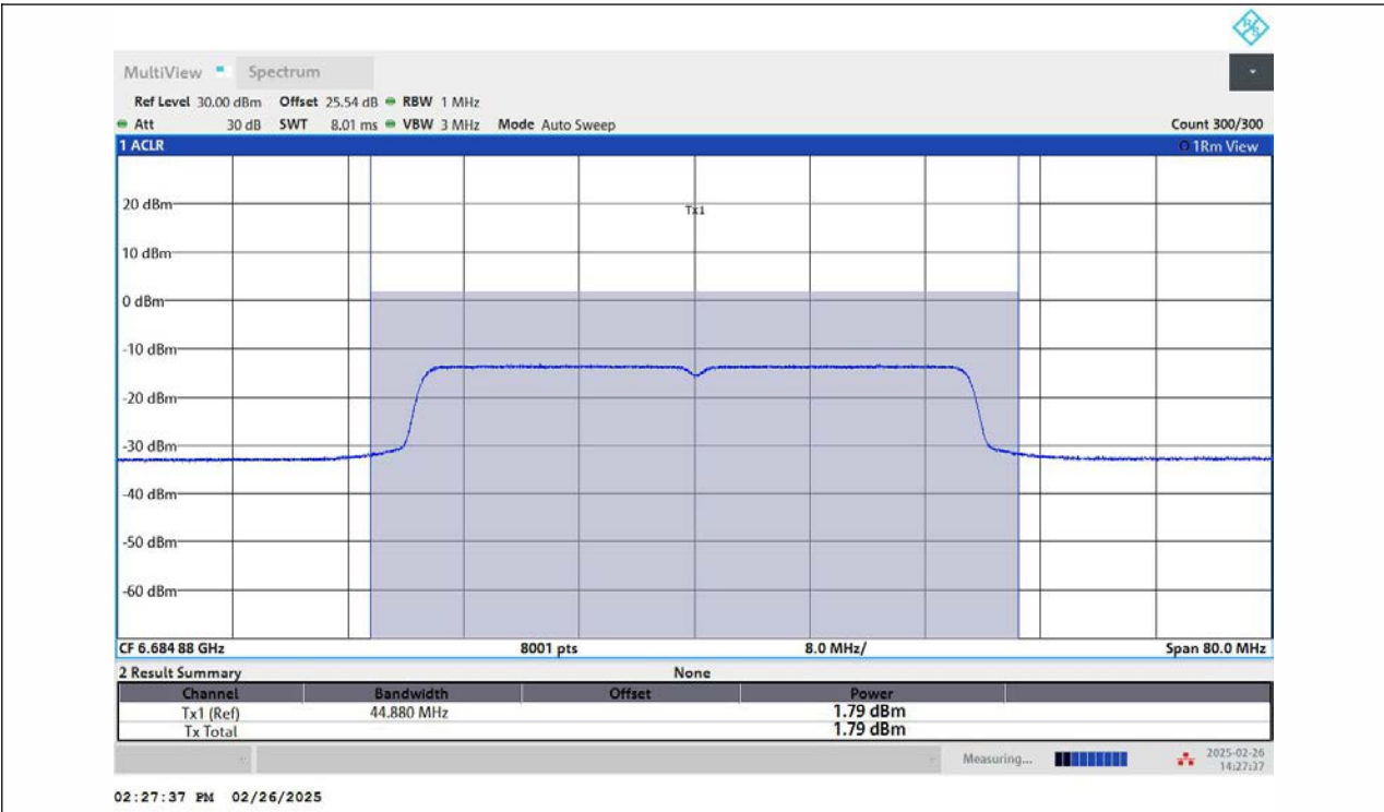
11AX40MIMO-Ant2-6685-PASS
