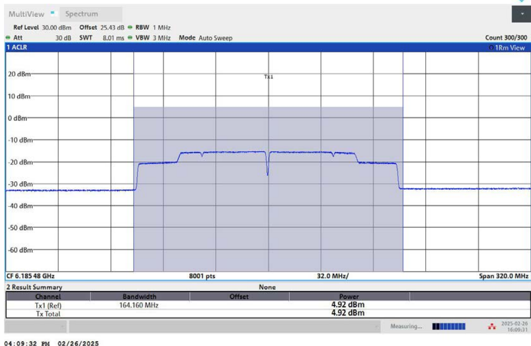
11AX160MIMO-Ant2-6185-PASS
