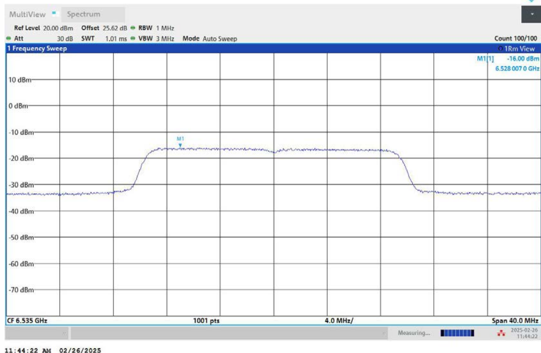
11AX20MIMO-Ant2-6535-PASS
