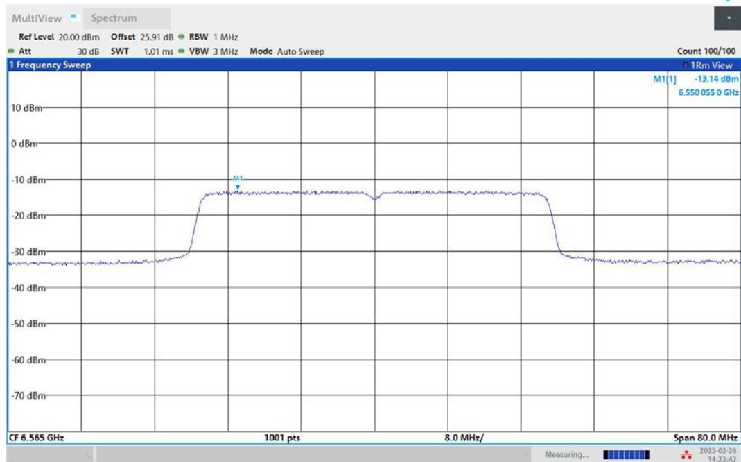
11AX40MIMO-Ant2-6565-PASS
