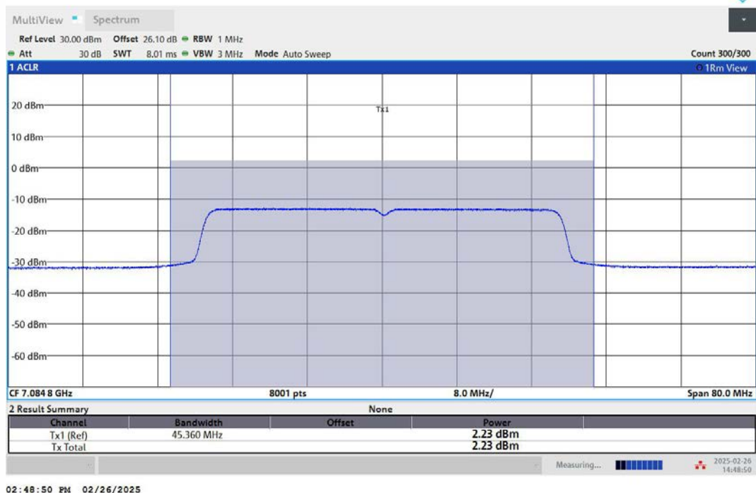
11AX40MIMO-Ant2-7085-PASS
