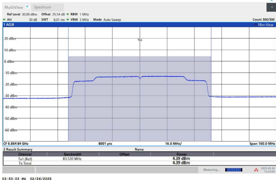
11AX80MIMO-Ant2-6865-PASS
