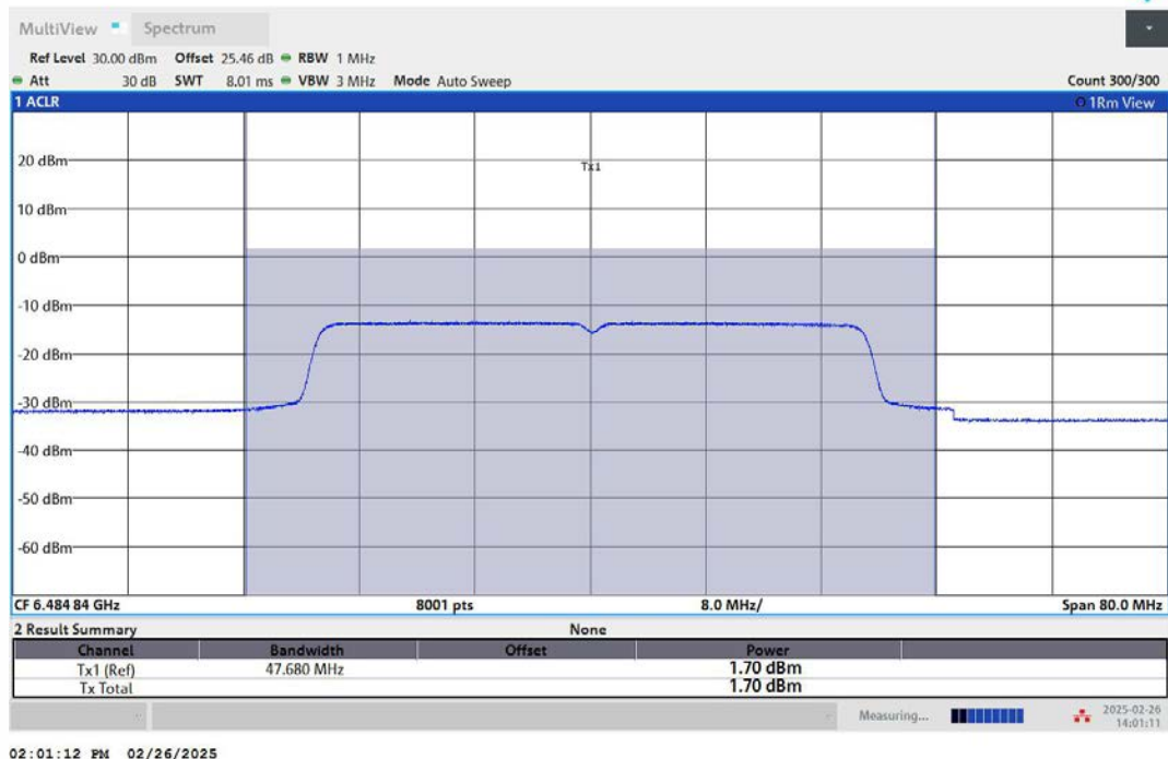
11AX40MIMO-Ant2-6485-PASS
