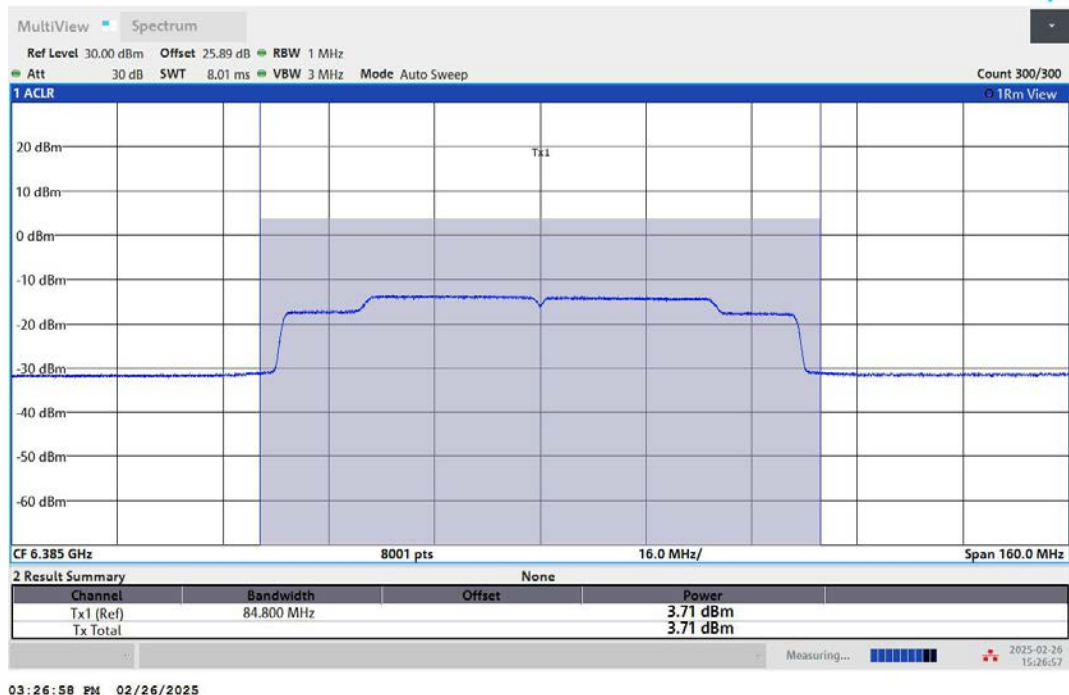
11AX80MIMO-Ant2-6385-PASS
