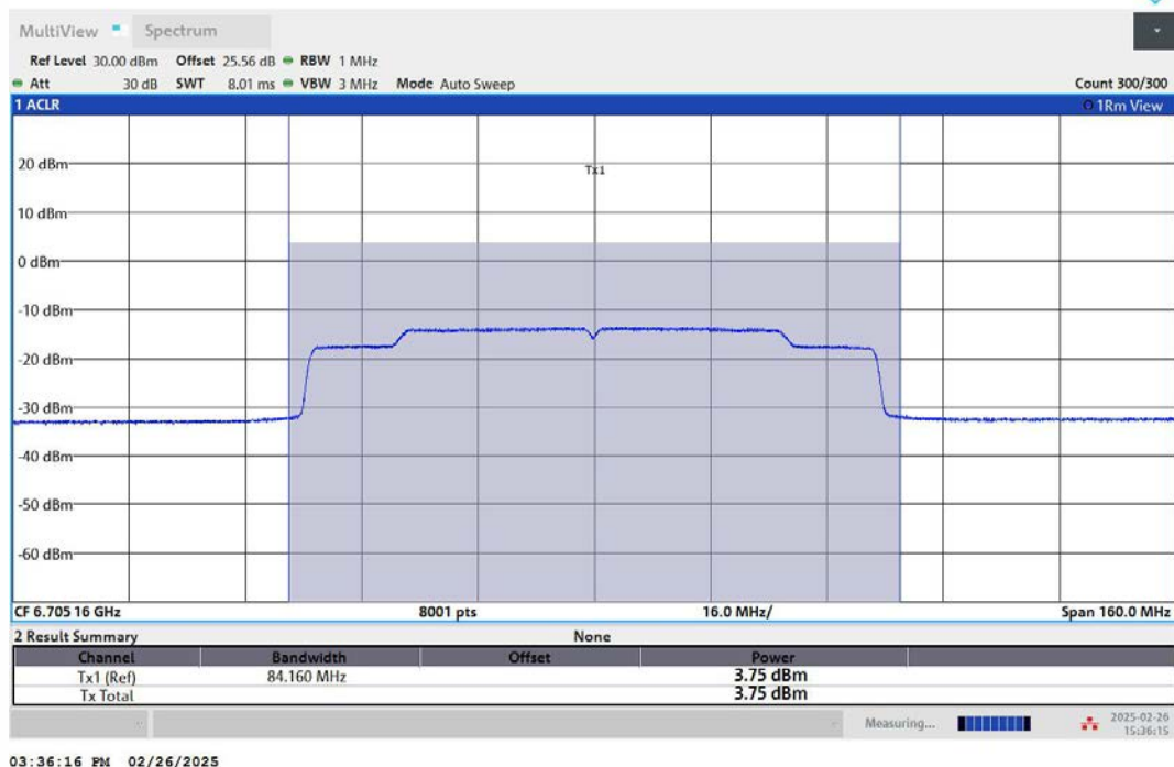
11AX80MIMO-Ant2-6705-PASS
