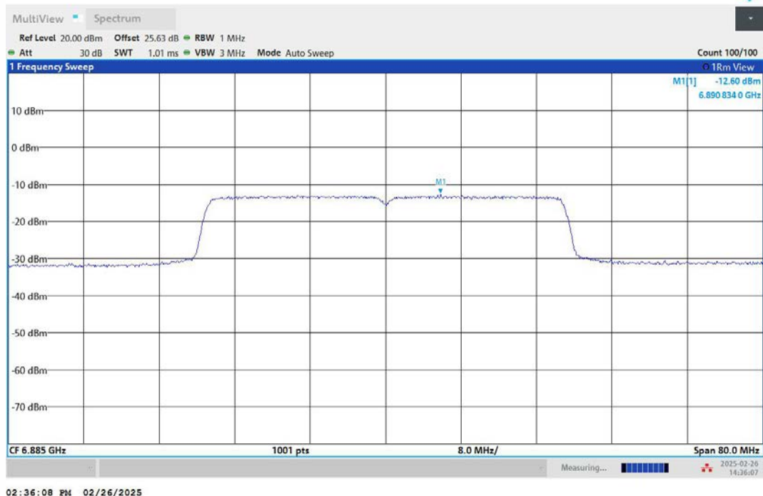
11AX40MIMO-Ant2-6885-PASS
