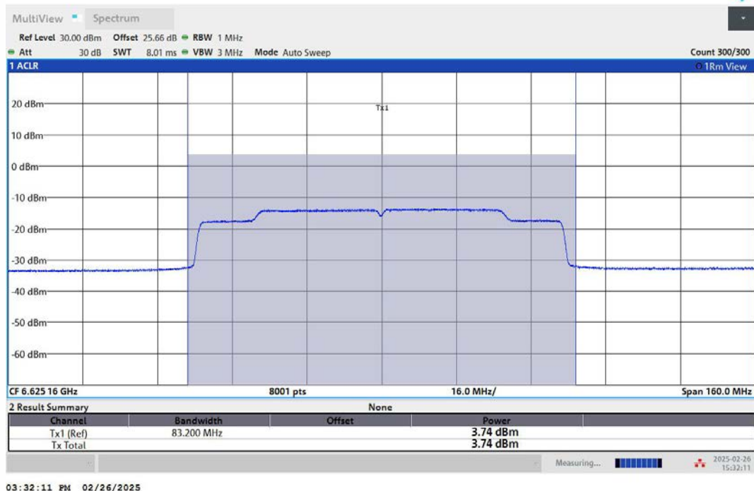
11AX80MIMO-Ant2-6625-PASS
