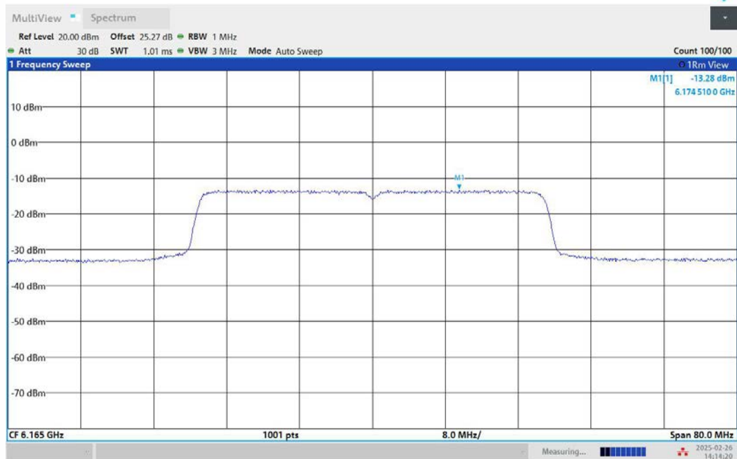
11AX40MIMO-Ant2-6165-PASS
