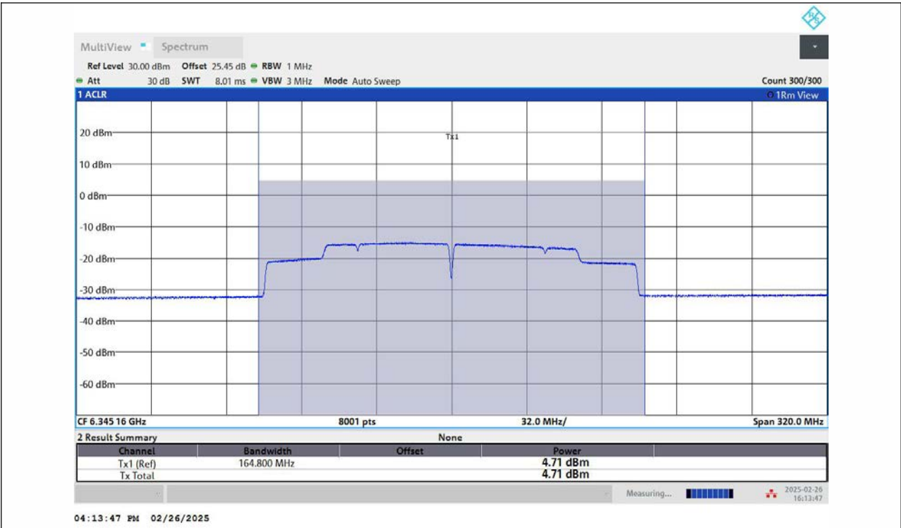
11AX160MIMO-Ant2-6345-PASS
