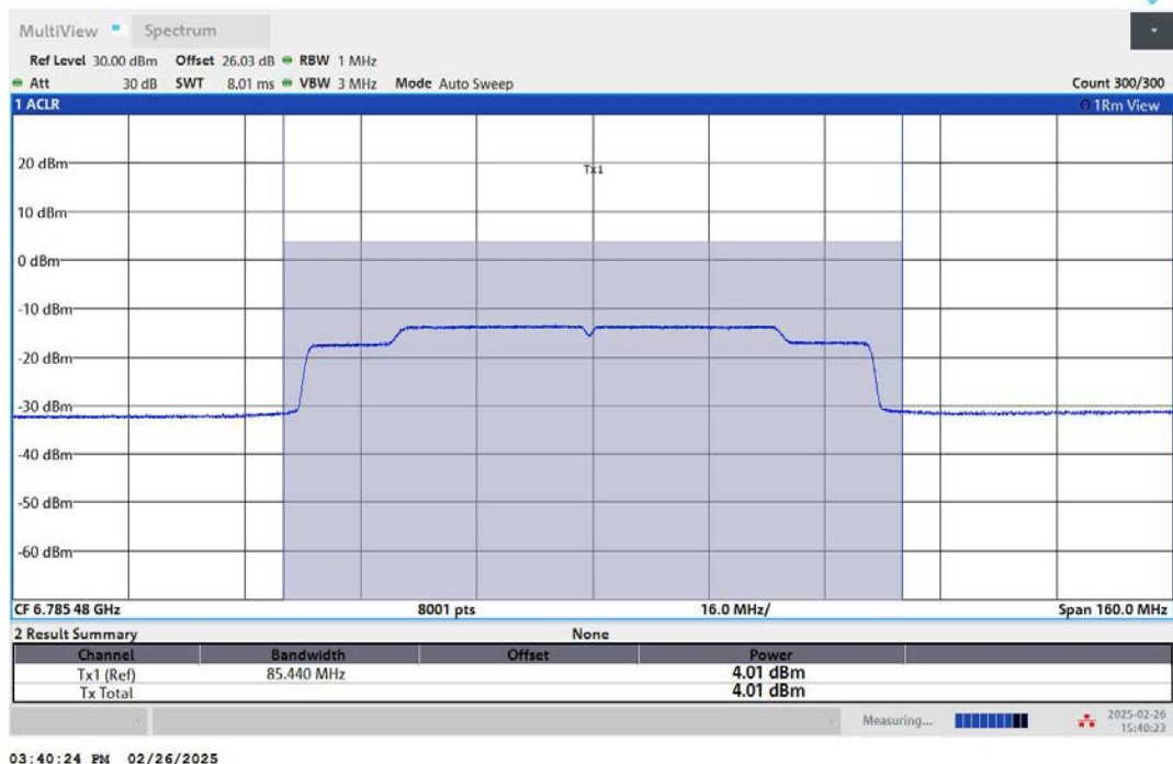
11AX80MIMO-Ant2-6785-PASS
