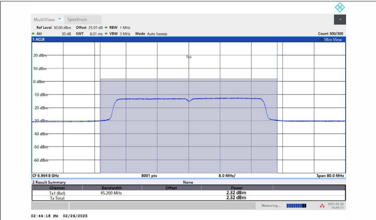
11AX40MIMO-Ant2-6965-PASS
