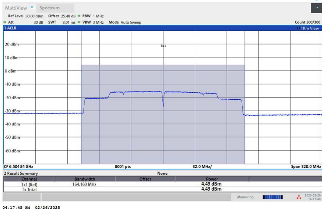
11AX160MIMO-Ant2-6505-PASS
