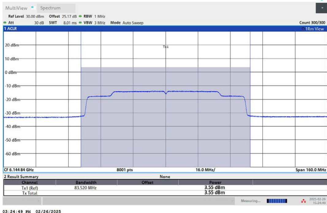
11AX80MIMO-Ant2-6145-PASS
