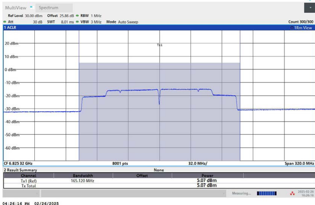
11AX160MIMO-Ant2-6825-PASS
