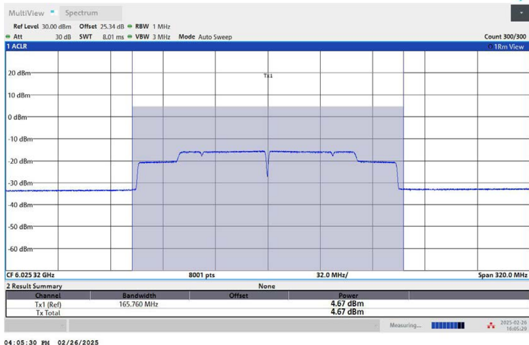
11AX160MIMO-Ant2-6025-PASS
