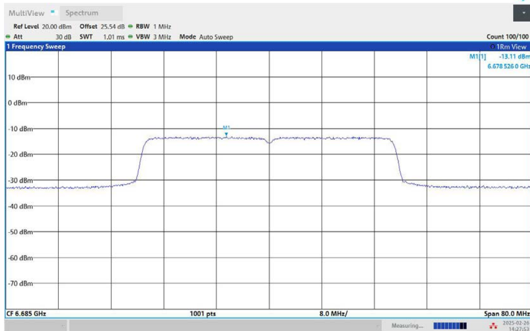
11AX40MIMO-Ant2-6685-PASS
