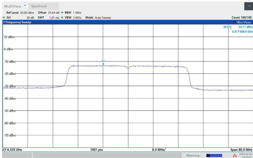
11AX40MIMO-Ant2-6525-PASS
