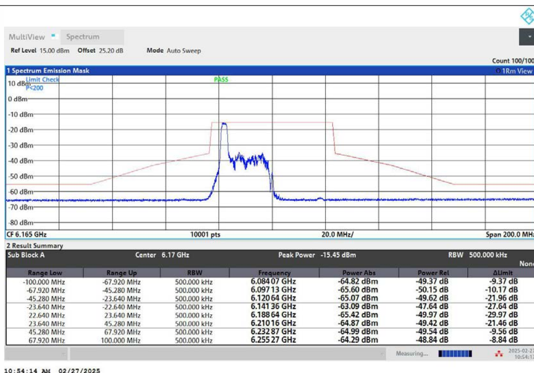
NTNV-11AX40MIMO-Ant2-6165-26Tone-RU0-PASS
