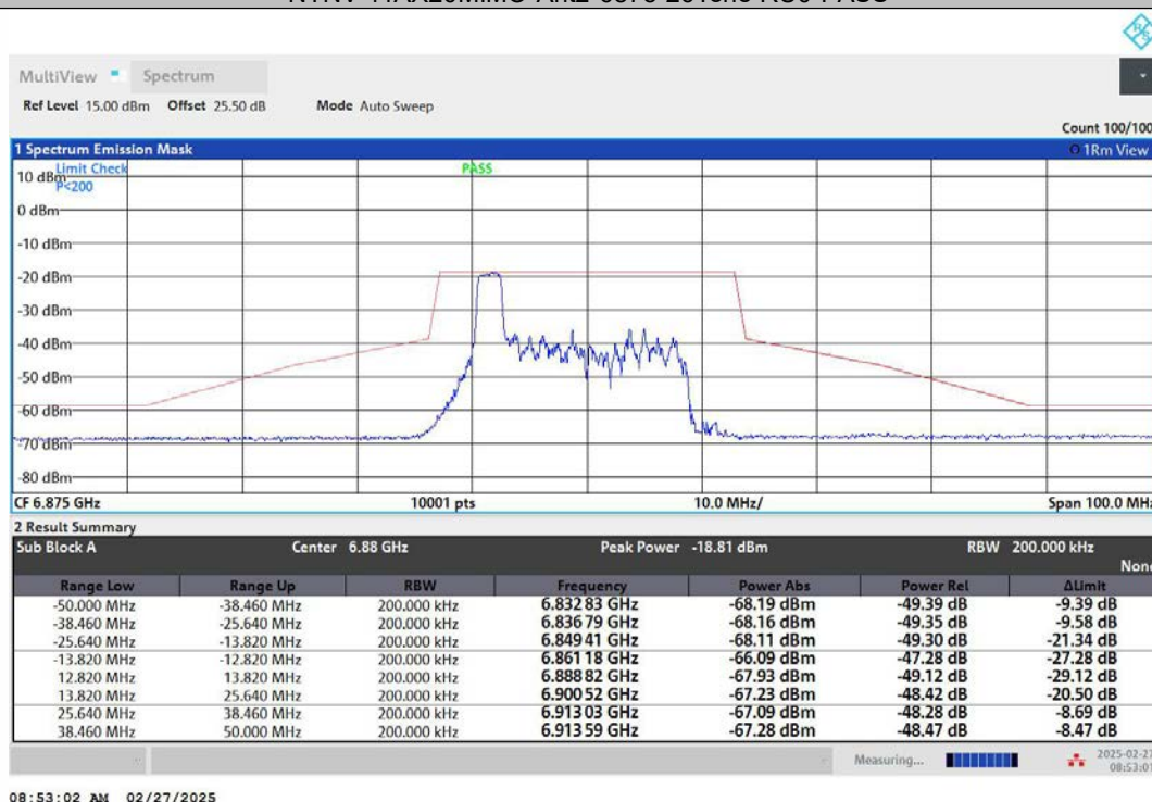
NTNV-11AX20MIMO-Ant1-6875-52Tone-RU37-PASS
