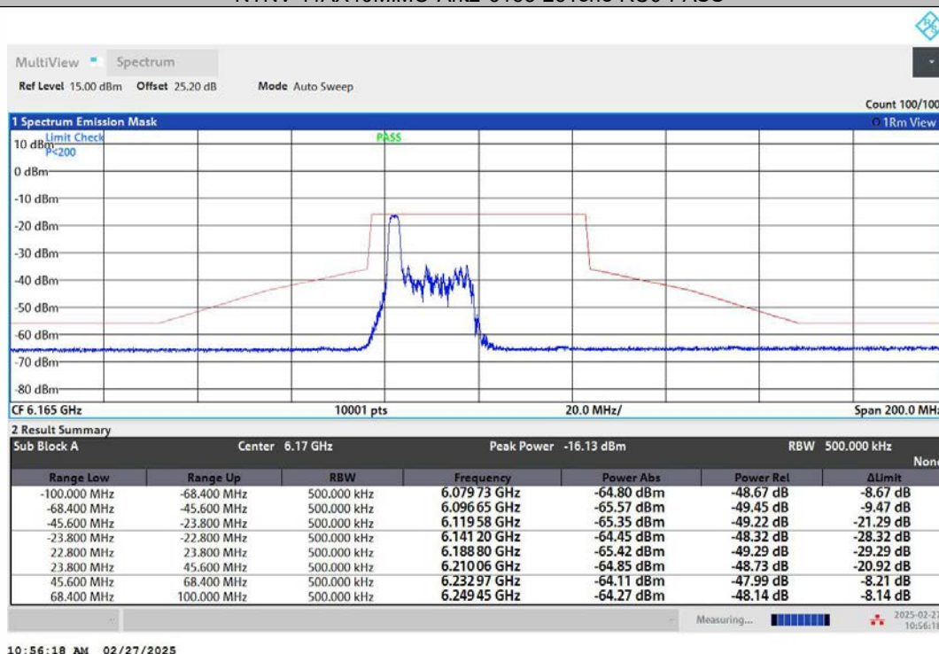
NTNV-11AX40MIMO-Ant1-6165-52Tone-RU37-PASS
