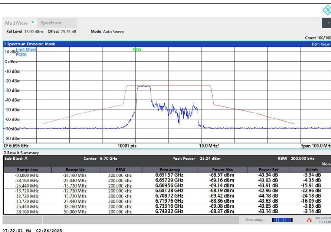
NTNV-11AX20MIMO-Ant2-6695-52Tone-RU37-PASS
