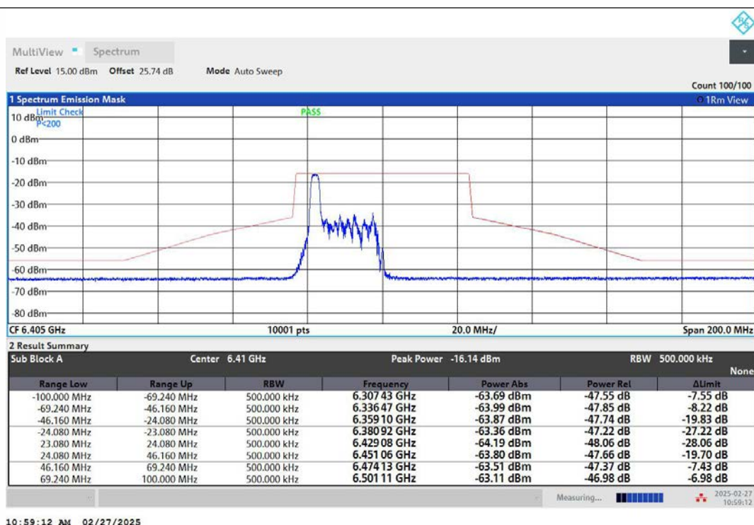
NTNV-11AX40MIMO-Ant2-6405-26Tone-RU0-PASS
