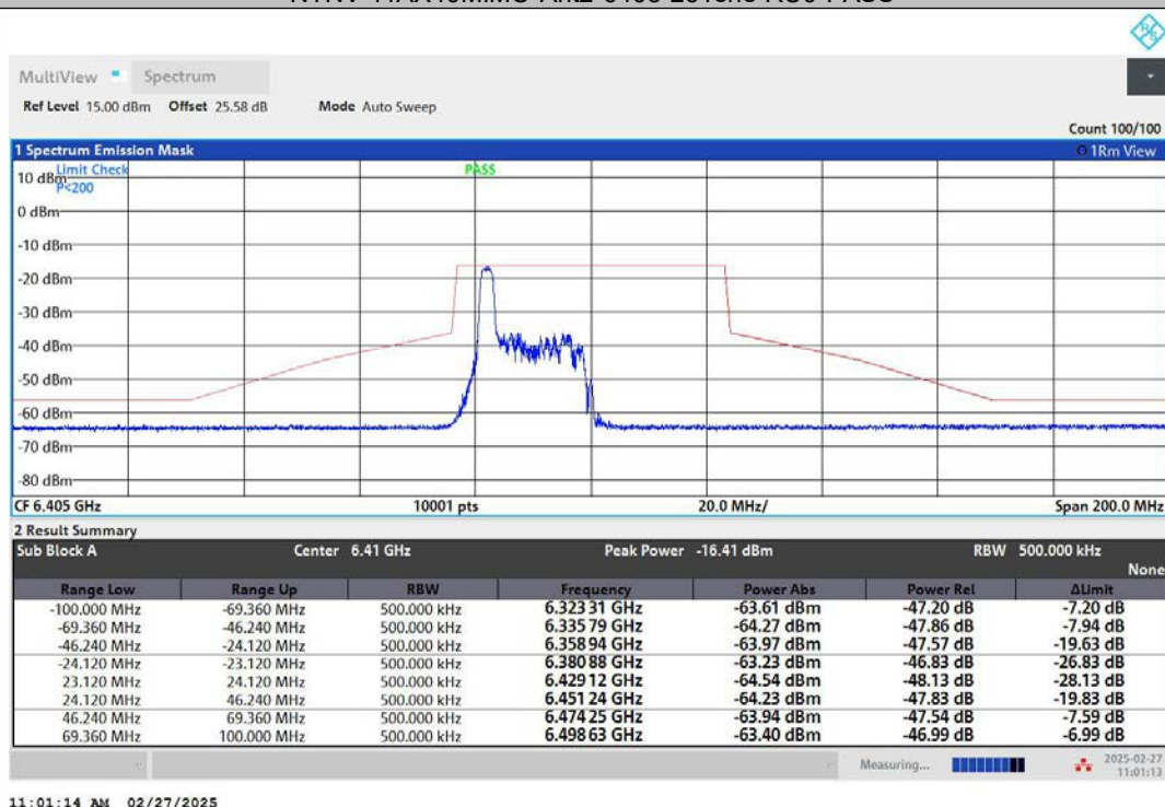
NTNV-11AX40MIMO-Ant1-6405-52Tone-RU37-PASS
