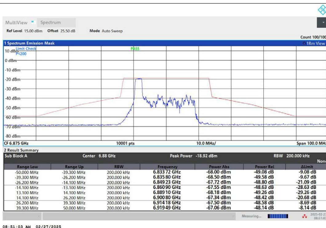
NTNV-11AX20MIMO-Ant2-6875-26Tone-RU0-PASS
