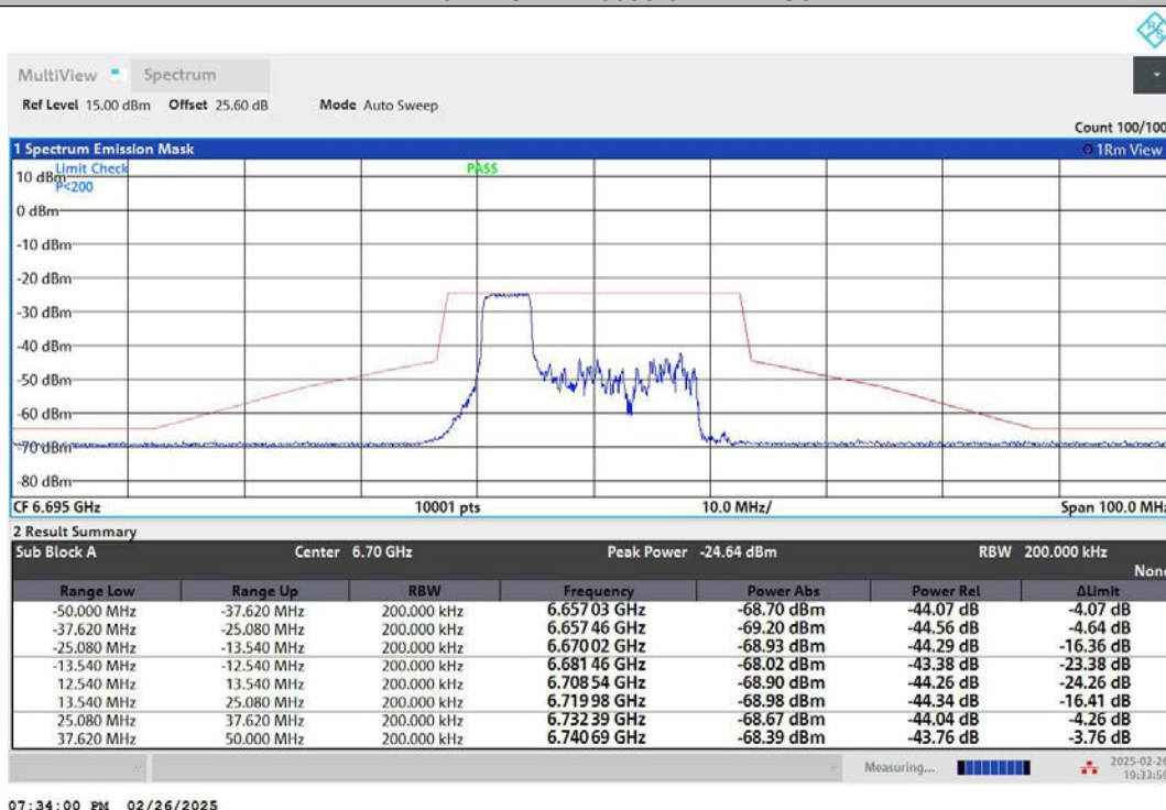
NTNV-11AX20MIMO-Ant1-6695-106Tone-RU53-PASS
