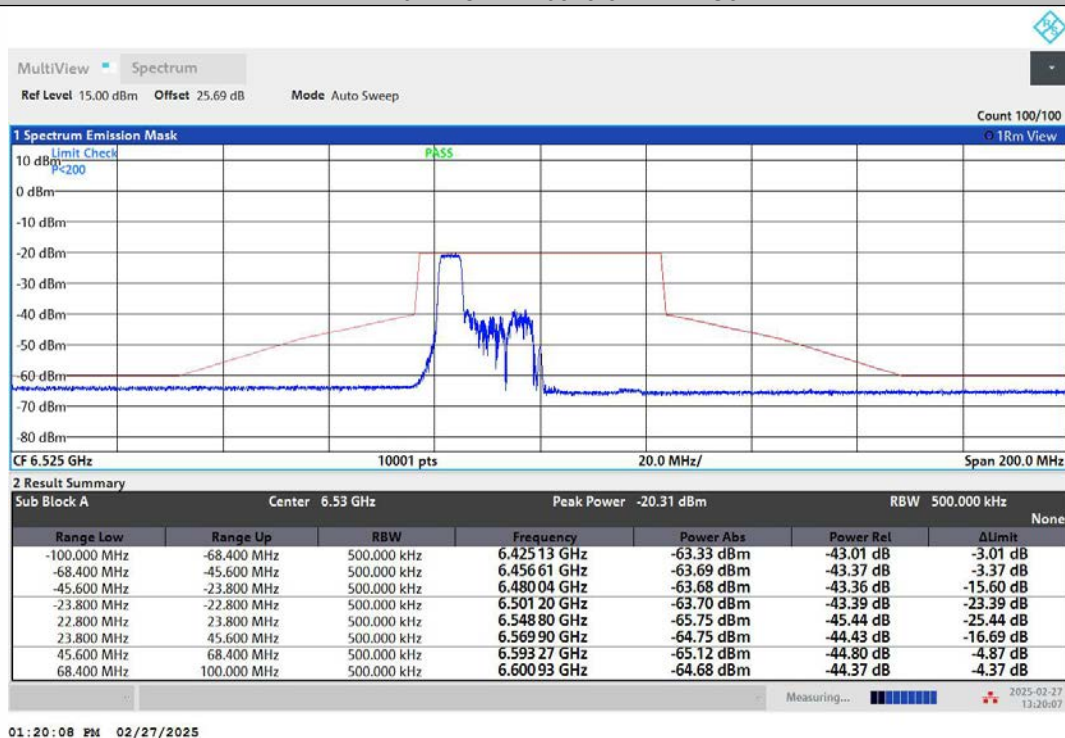
NTNV-11AX40MIMO-Ant1-6525-106Tone-RU53-PASS
