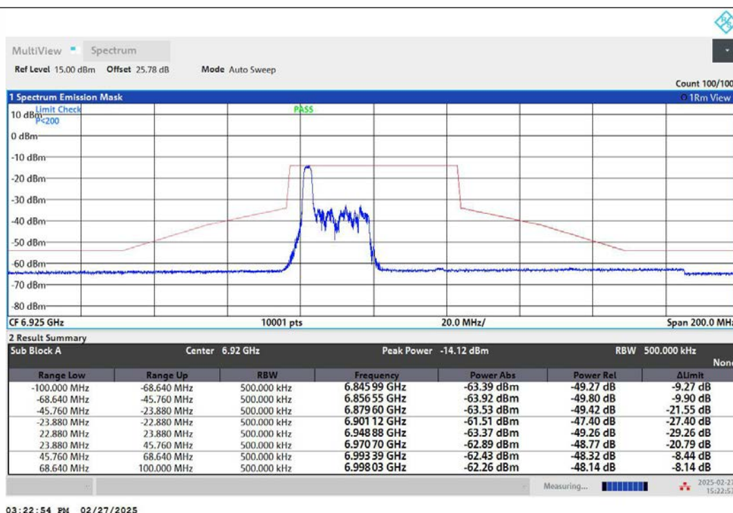
NTNV-11AX40MIMO-Ant2-6925-26Tone-RU0-PASS
