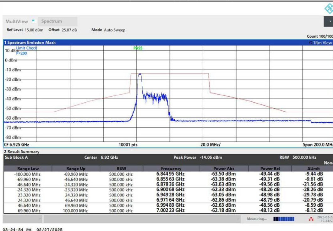
NTNV-11AX40MIMO-Ant1-6925-52Tone-RU37-PASS
