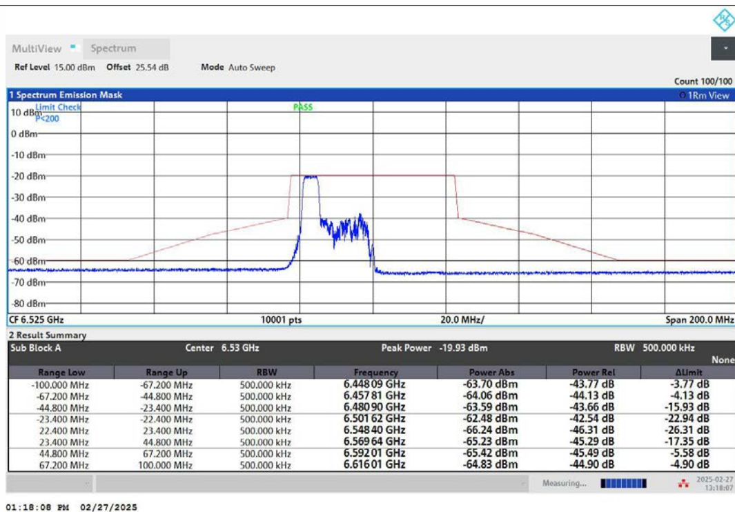
NTNV-11AX40MIMO-Ant2-6525-52Tone-RU37-PASS
