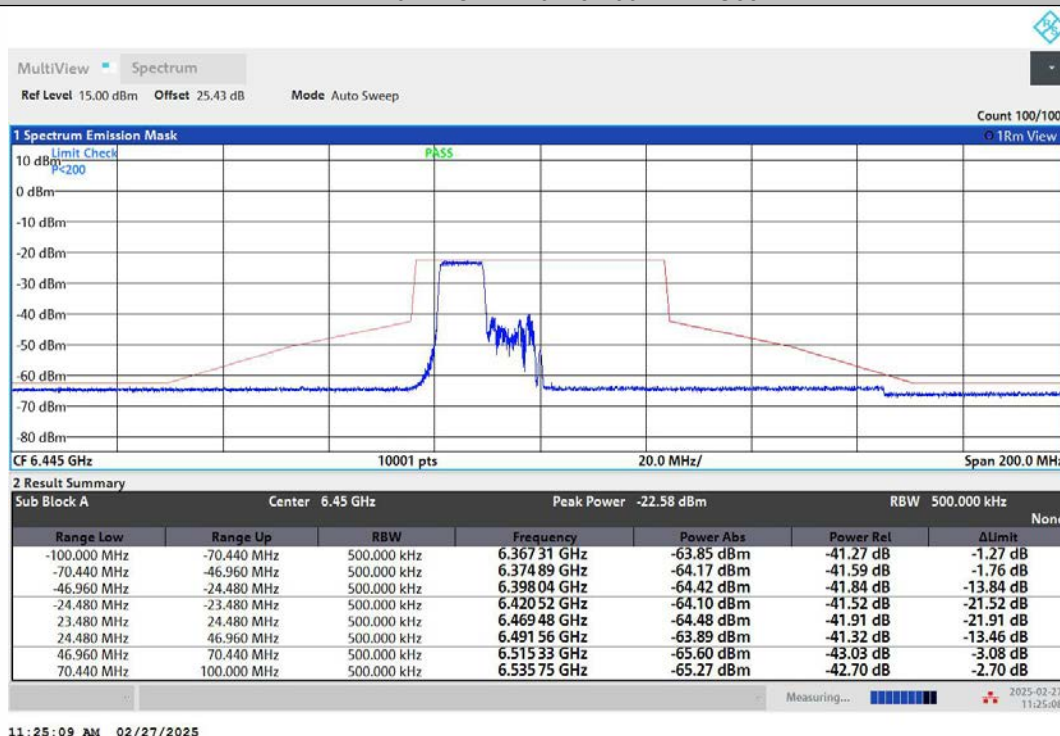
NTNV-11AX40MIMO-Ant1-6445-242Tone-RU61-PASS
