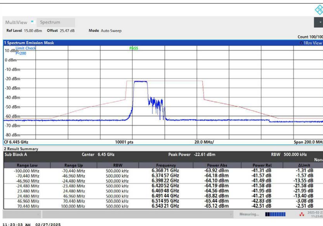
NTNV-11AX40MIMO-Ant2-6445-106Tone-RU53-PASS
