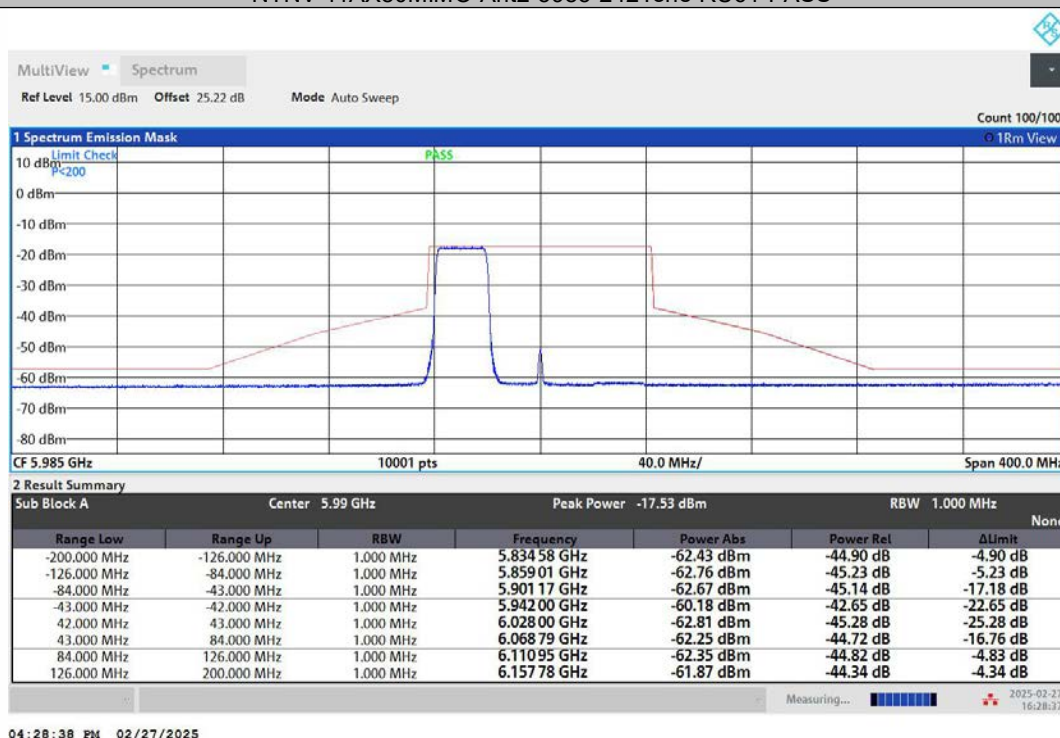
NTNV-11AX80MIMO-Ant1-5985-484Tone-RU65-PASS
