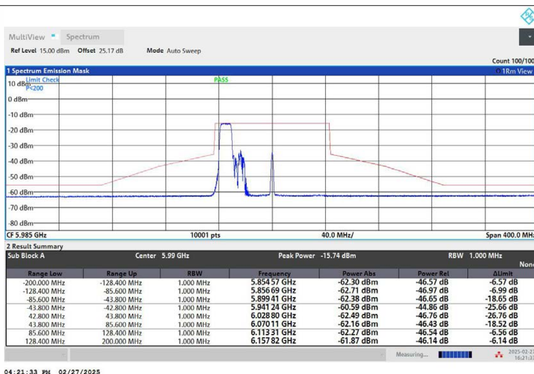
NTNV-11AX80MIMO-Ant2-5985-106Tone-RU53-PASS
