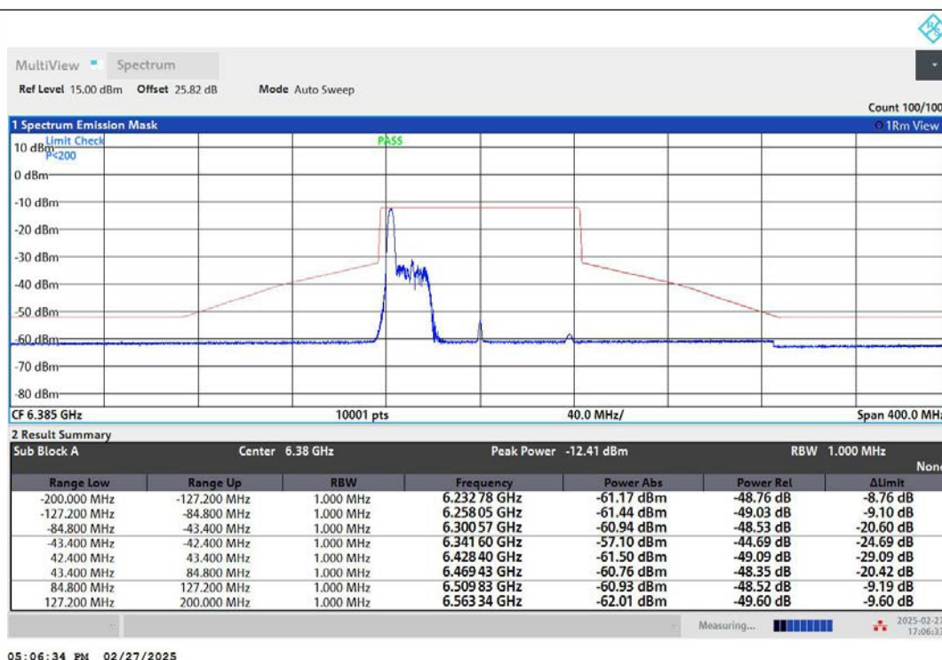
NTNV-11AX80MIMO-Ant2-6385-26Tone-RU0-PASS
