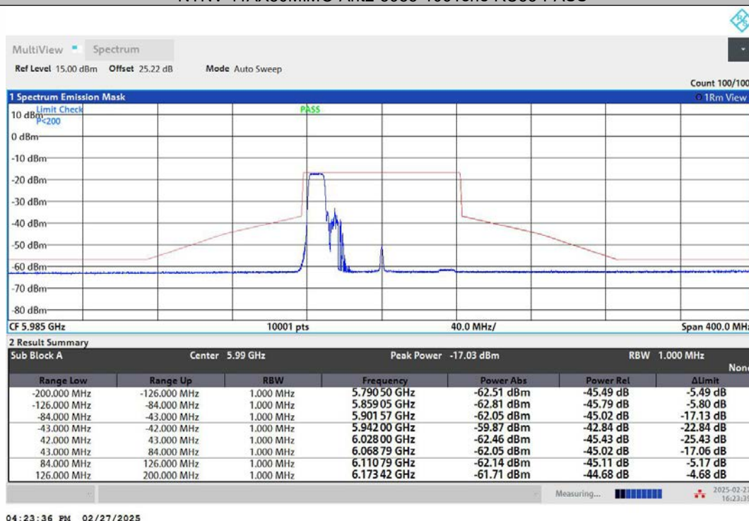
NTNV-11AX80MIMO-Ant1-5985-242Tone-RU61-PASS
