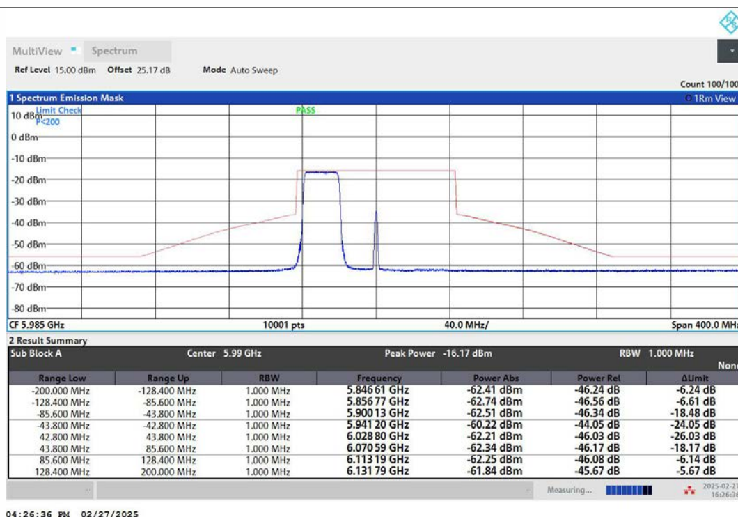
NTNV-11AX80MIMO-Ant2-5985-242Tone-RU61-PASS
