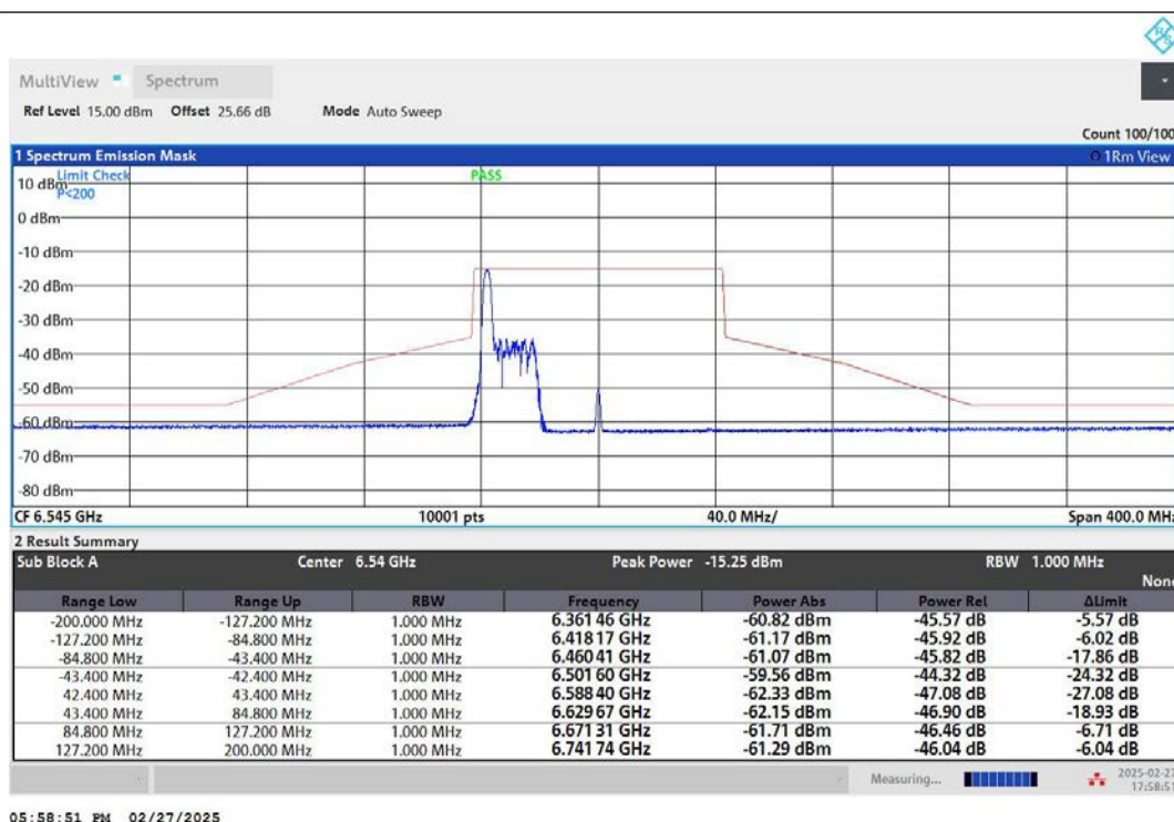
NTNV-11AX80MIMO-Ant2-6545-26Tone-RU0-PASS
