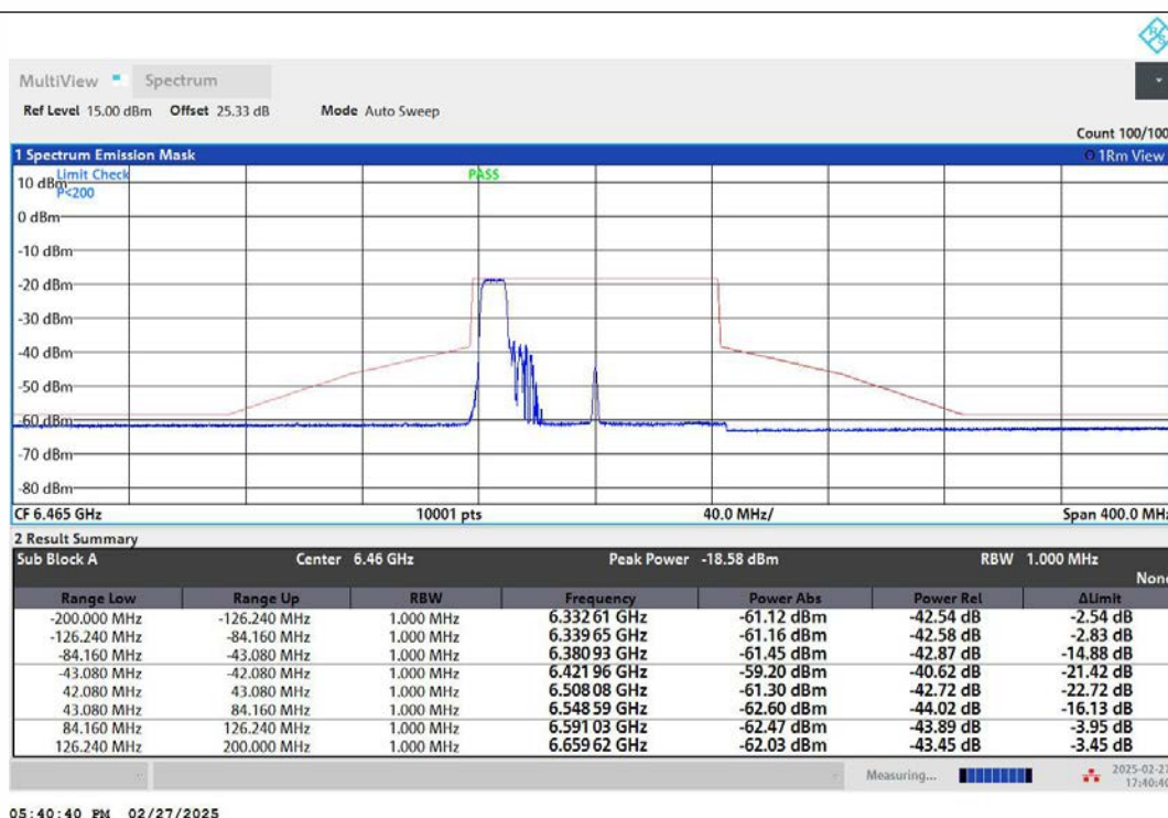
NTNV-11AX80MIMO-Ant2-6465-106Tone-RU53-PASS
