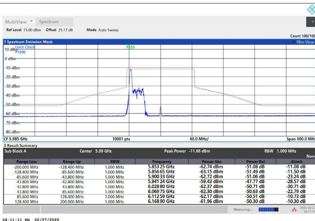
NTNV-11AX80MIMO-Ant2-5985-26Tone-RU0-PASS
