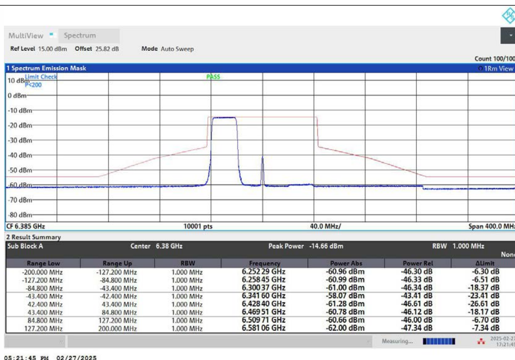
NTNV-11AX80MIMO-Ant2-6385-242Tone-RU61-PASS
