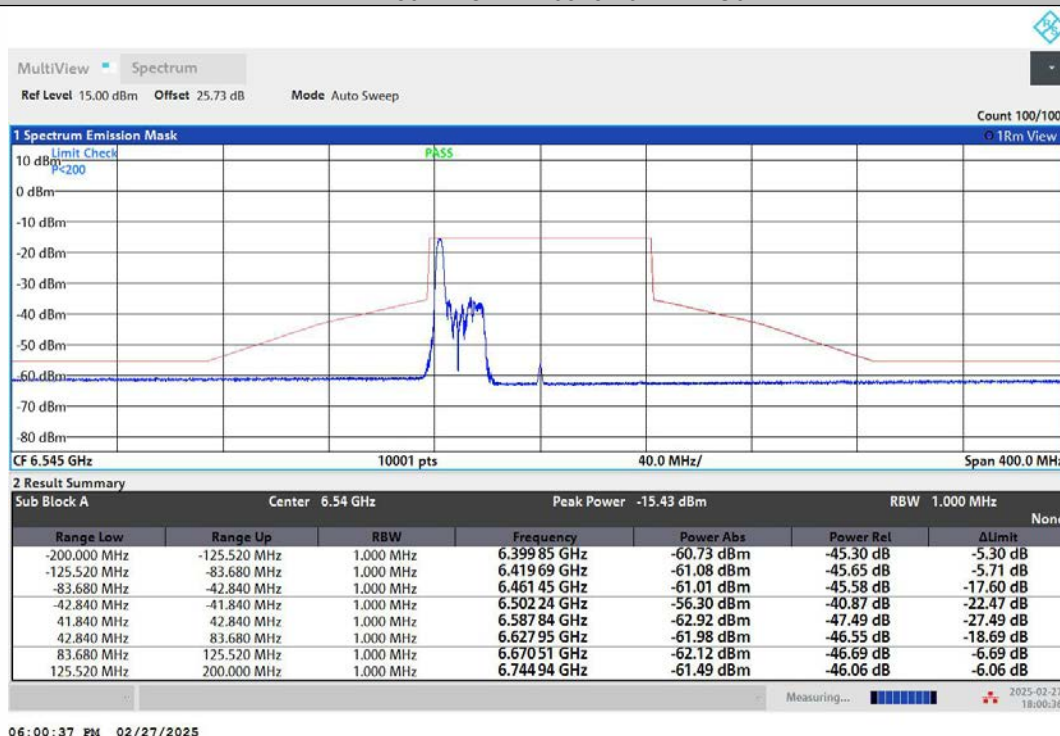
NTNV-11AX80MIMO-Ant1-6545-52Tone-RU37-PASS
