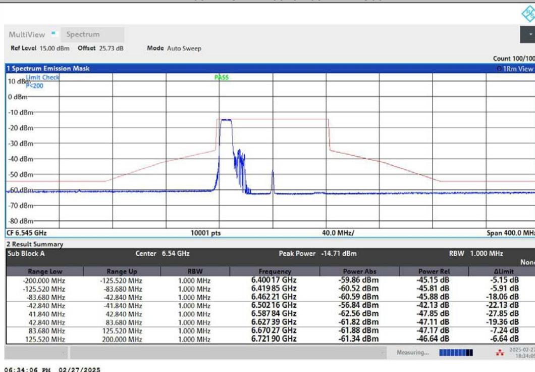
NTNV-11AX80MIMO-Ant1-6545-242Tone-RU61-PASS
