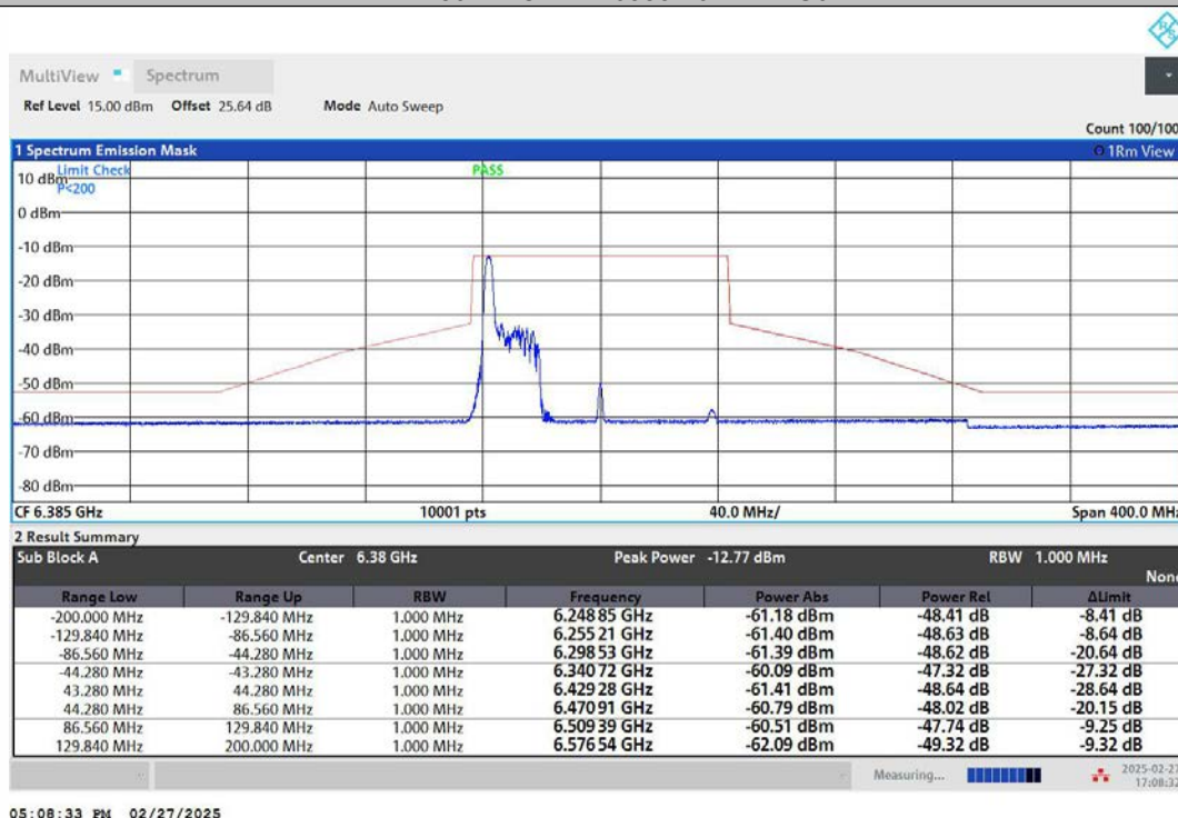
NTNV-11AX80MIMO-Ant1-6385-52Tone-RU37-PASS
