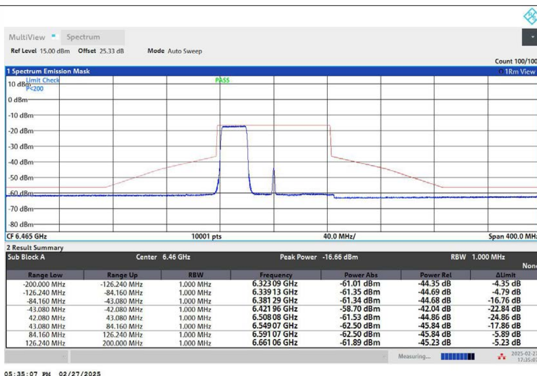
NTNV-11AX80MIMO-Ant2-6465-242Tone-RU61-PASS
