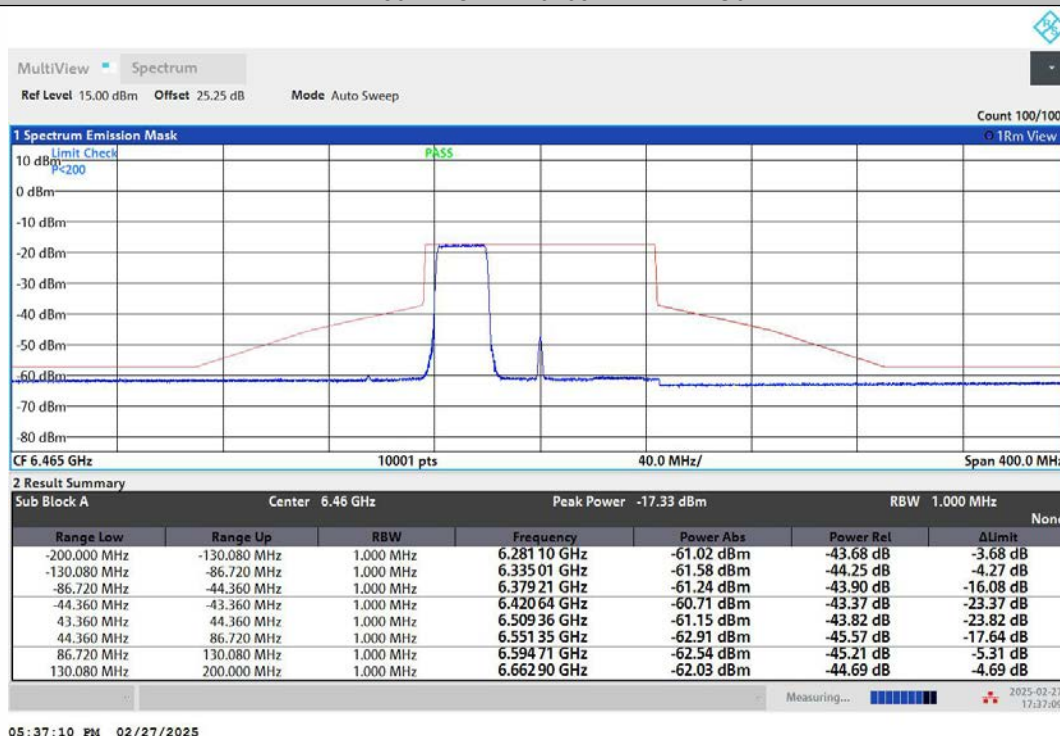
NTNV-11AX80MIMO-Ant1-6465-484Tone-RU65-PASS
