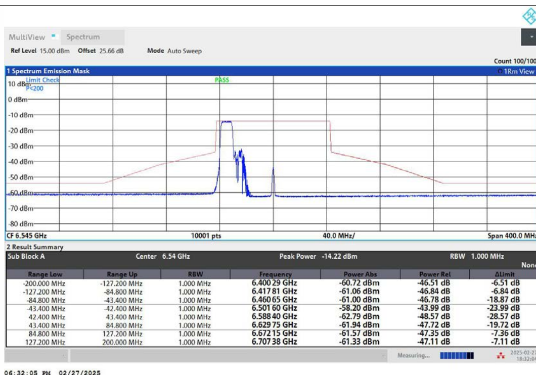
NTNV-11AX80MIMO-Ant2-6545-106Tone-RU53-PASS
