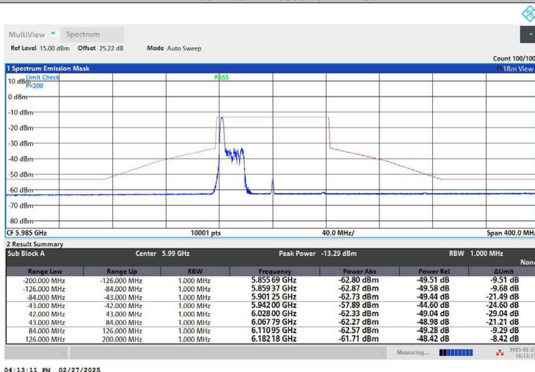
NTNV-11AX80MIMO-Ant1-5985-52Tone-RU37-PASS
