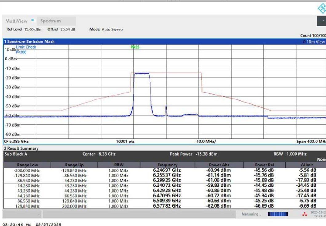
NTNV-11AX80MIMO-Ant1-6385-484Tone-RU65-PASS
