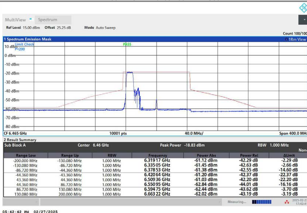
NTNV-11AX80MIMO-Ant1-6465-242Tone-RU61-PASS
