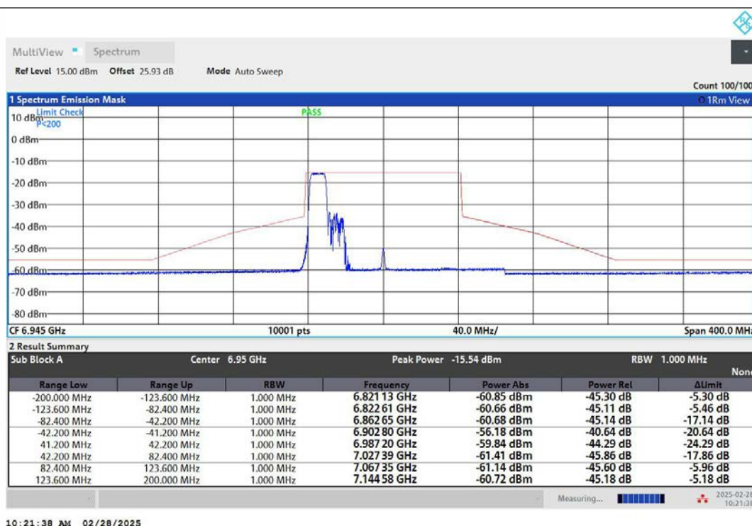
NTNV-11AX80MIMO-Ant2-6945-106Tone-RU53-PASS
