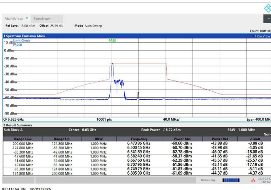
NTNV-11AX80MIMO-Ant2-6625-26Tone-RU0-PASS
