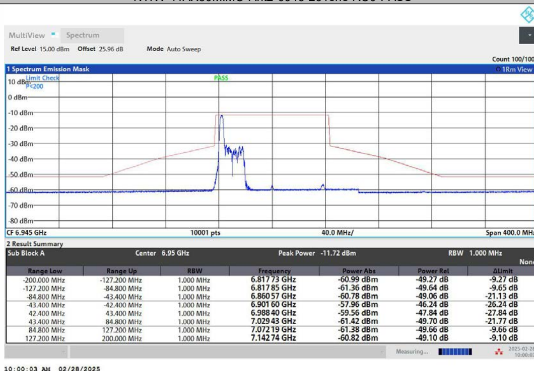
NTNV-11AX80MIMO-Ant1-6945-52Tone-RU37-PASS
