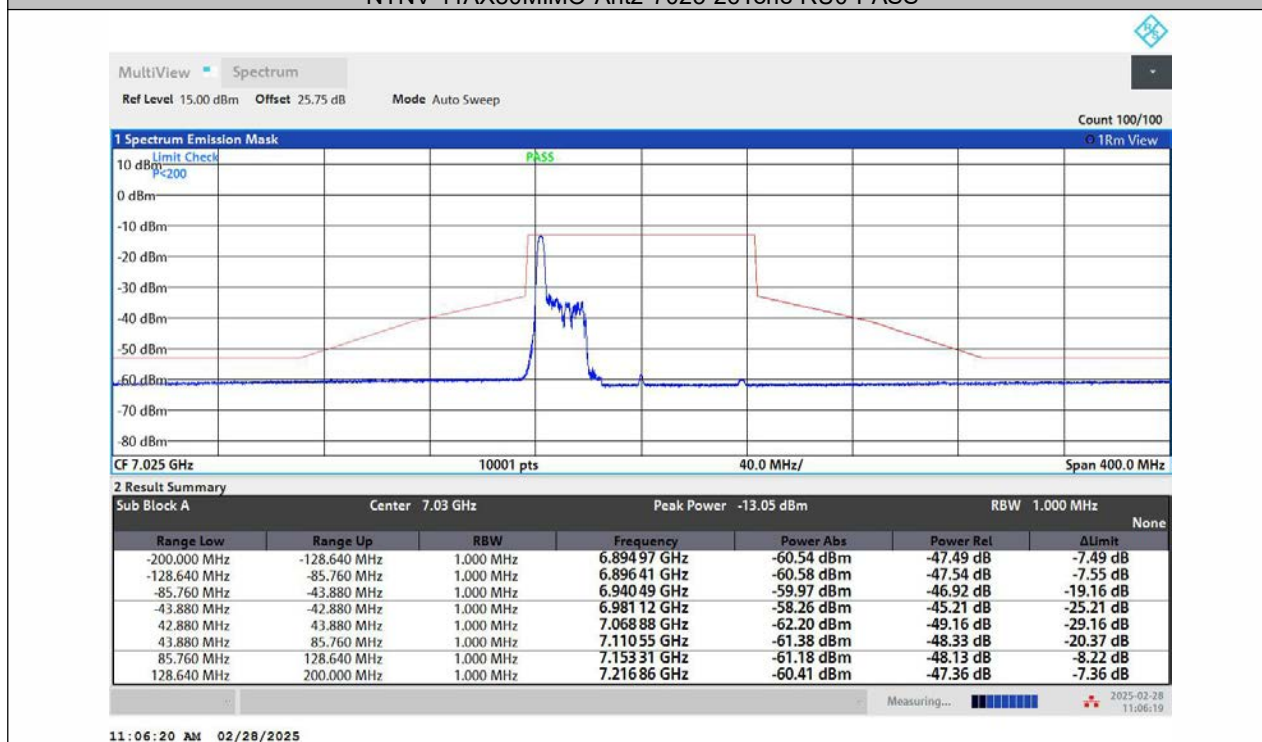
NTNV-11AX80MIMO-Ant1-7025-52Tone-RU37-PASS
