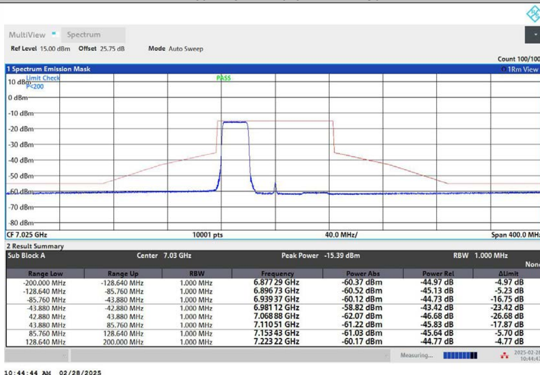
NTNV-11AX80MIMO-Ant1-7025-484Tone-RU65-PASS
