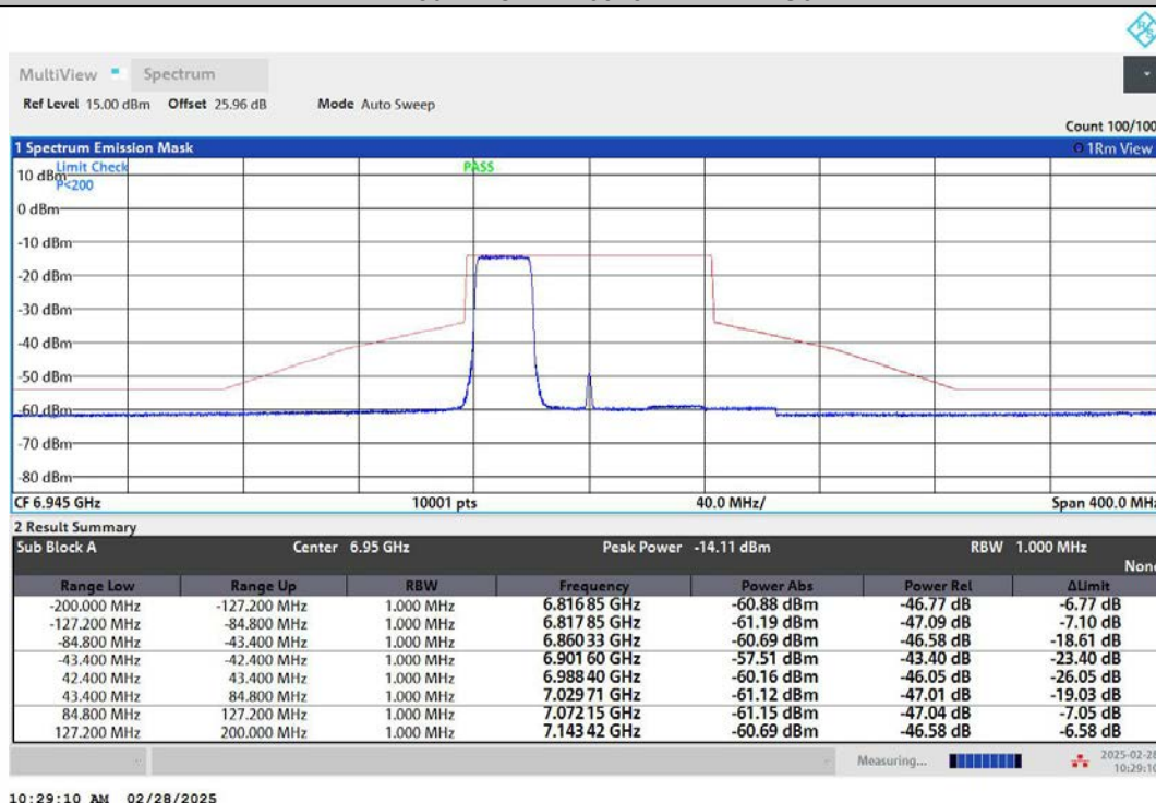
NTNV-11AX80MIMO-Ant1-6945-484Tone-RU65-PASS
