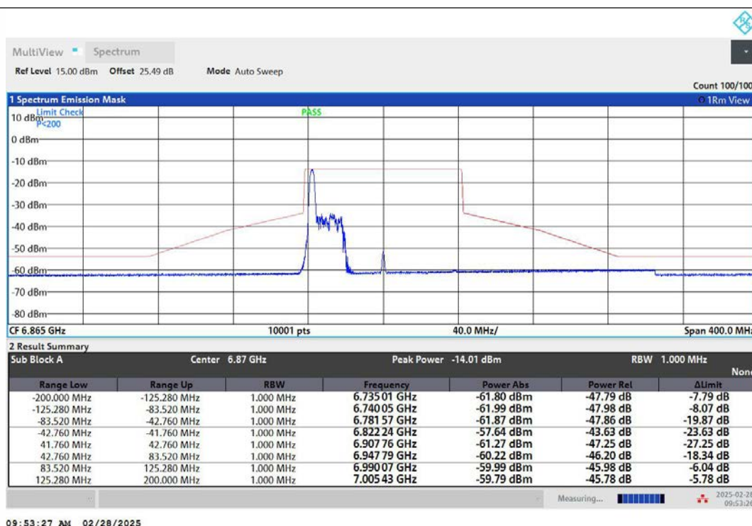
NTNV-11AX80MIMO-Ant2-6865-26Tone-RU0-PASS
