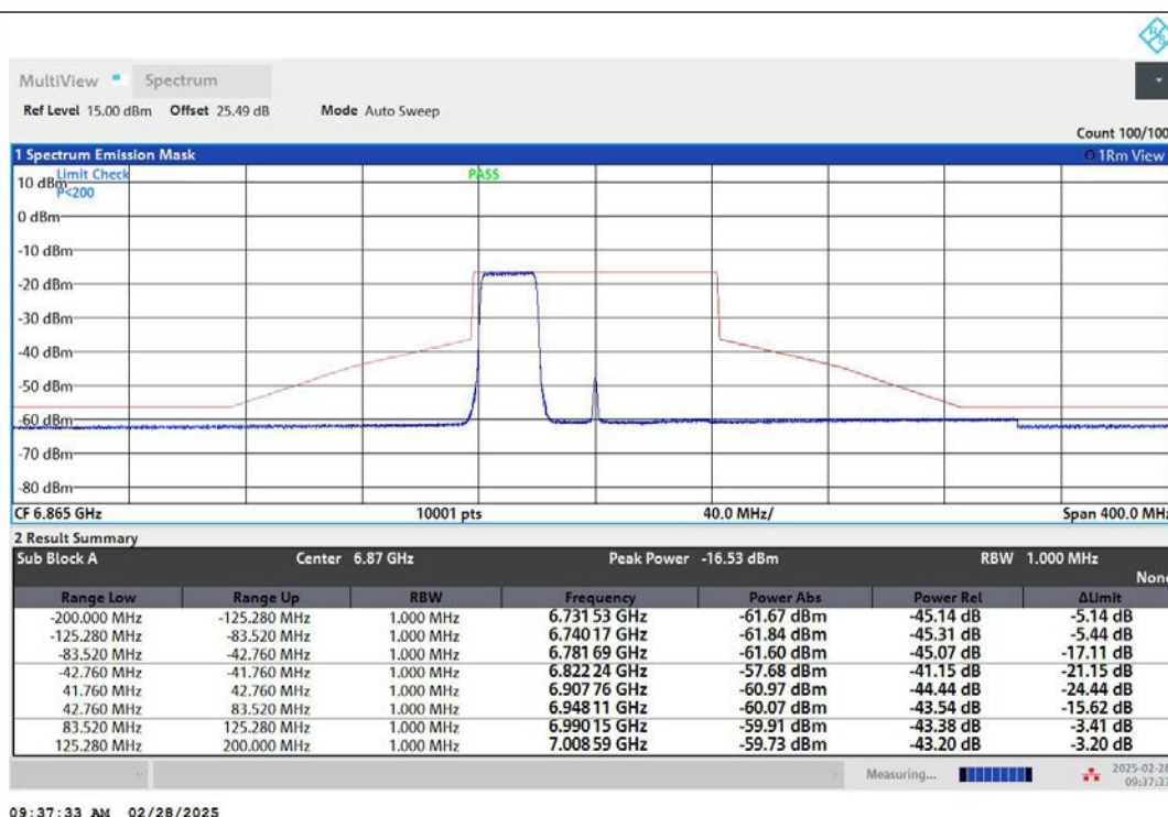
NTNV-11AX80MIMO-Ant2-6865-242Tone-RU61-PASS
