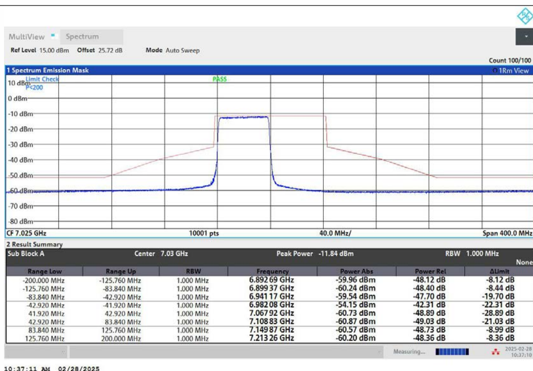
NTNV-11AX80MIMO-Ant2-7025-484Tone-RU65-PASS
