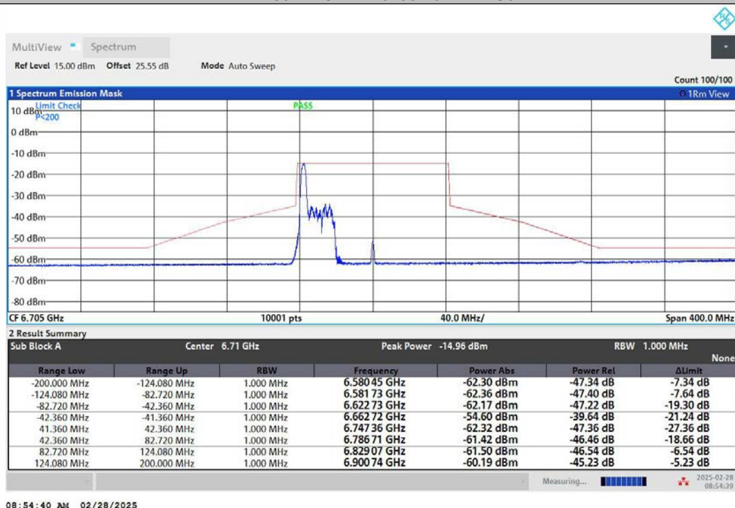
NTNV-11AX80MIMO-Ant1-6705-52Tone-RU37-PASS
