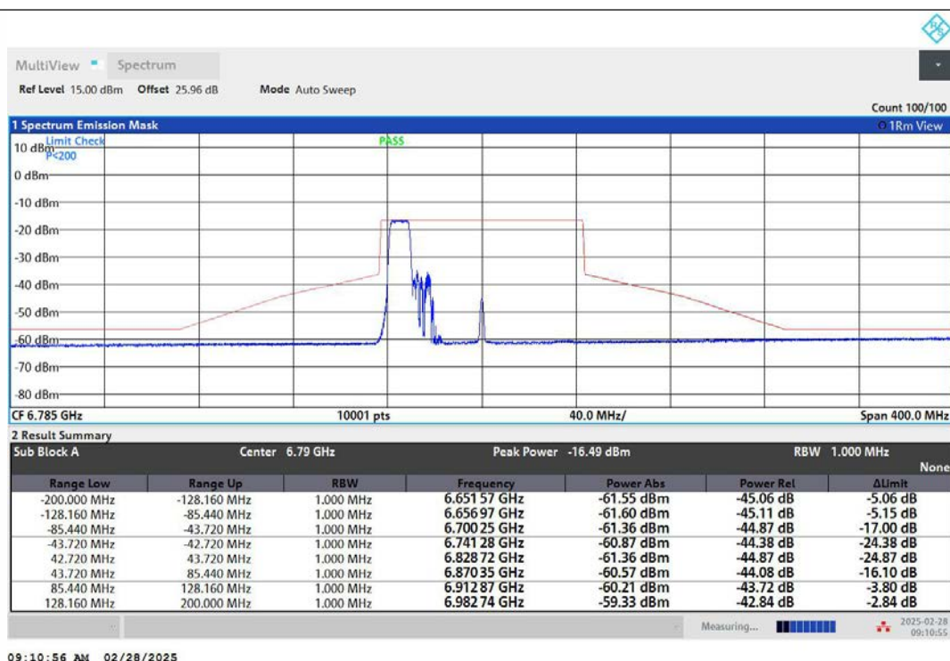
NTNV-11AX80MIMO-Ant2-6785-106Tone-RU53-PASS
