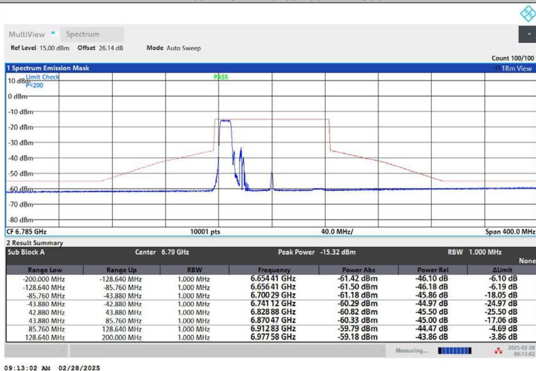
NTNV-11AX80MIMO-Ant1-6785-242Tone-RU61-PASS
