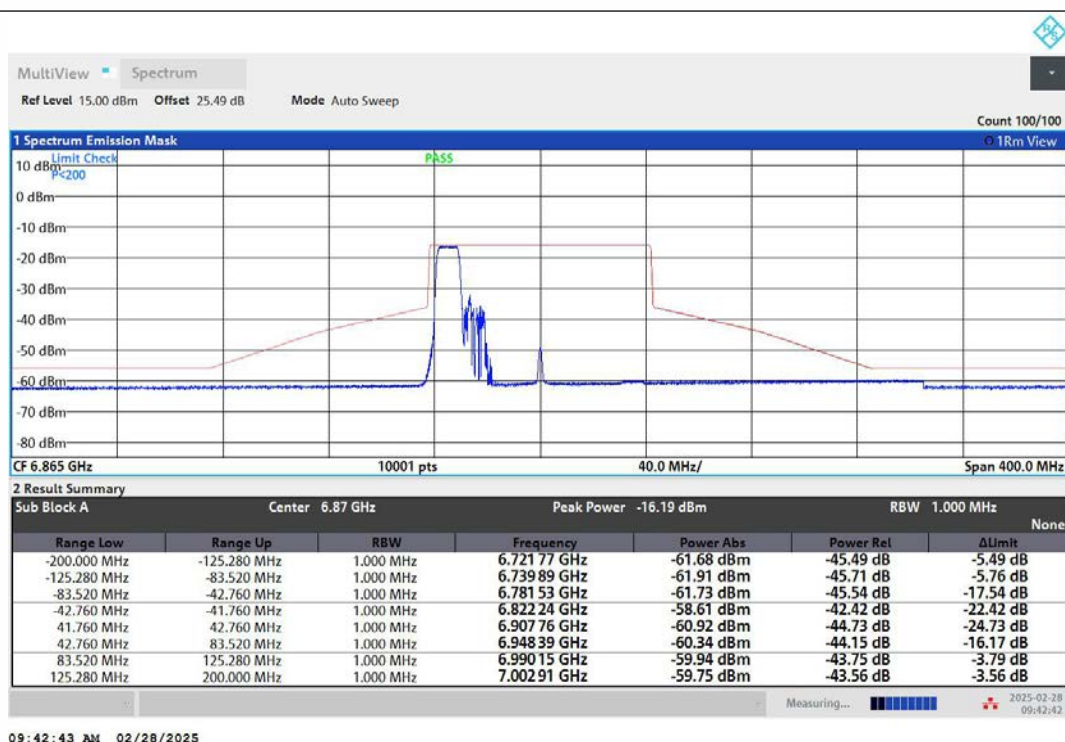
NTNV-11AX80MIMO-Ant2-6865-106Tone-RU53-PASS
