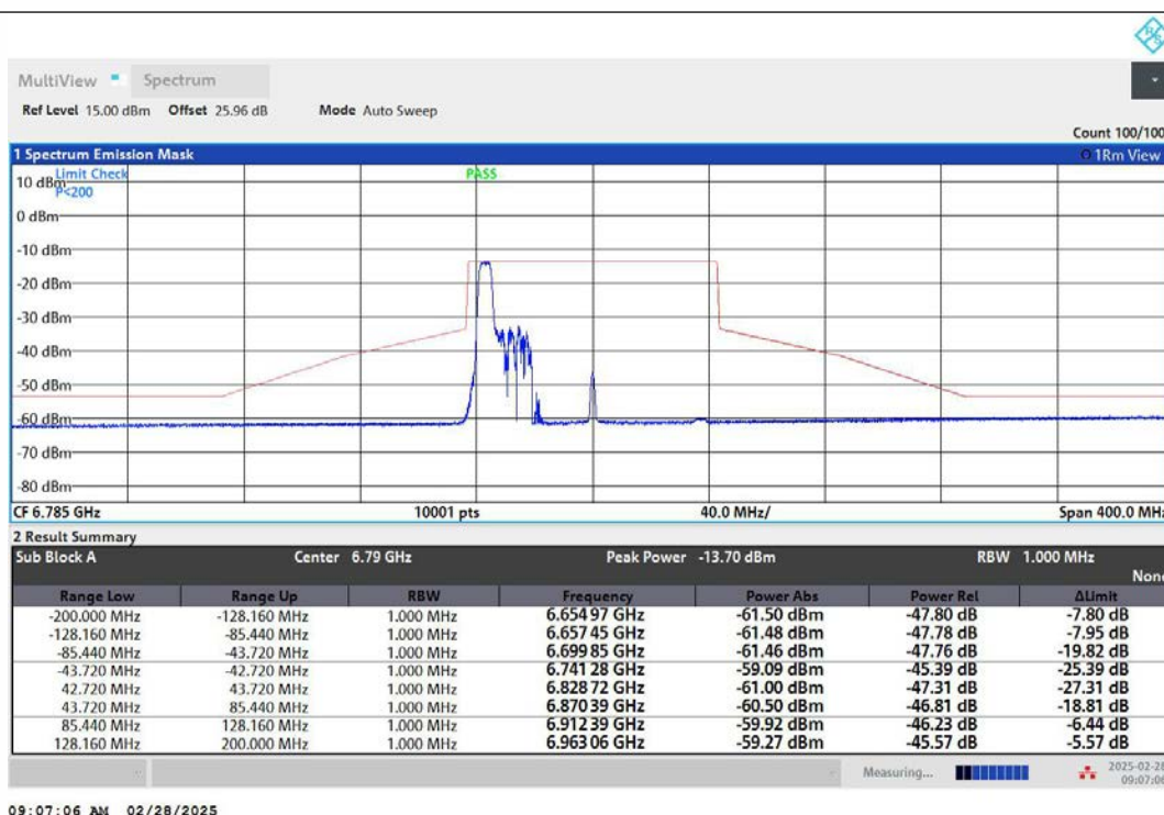
NTNV-11AX80MIMO-Ant2-6785-52Tone-RU37-PASS
