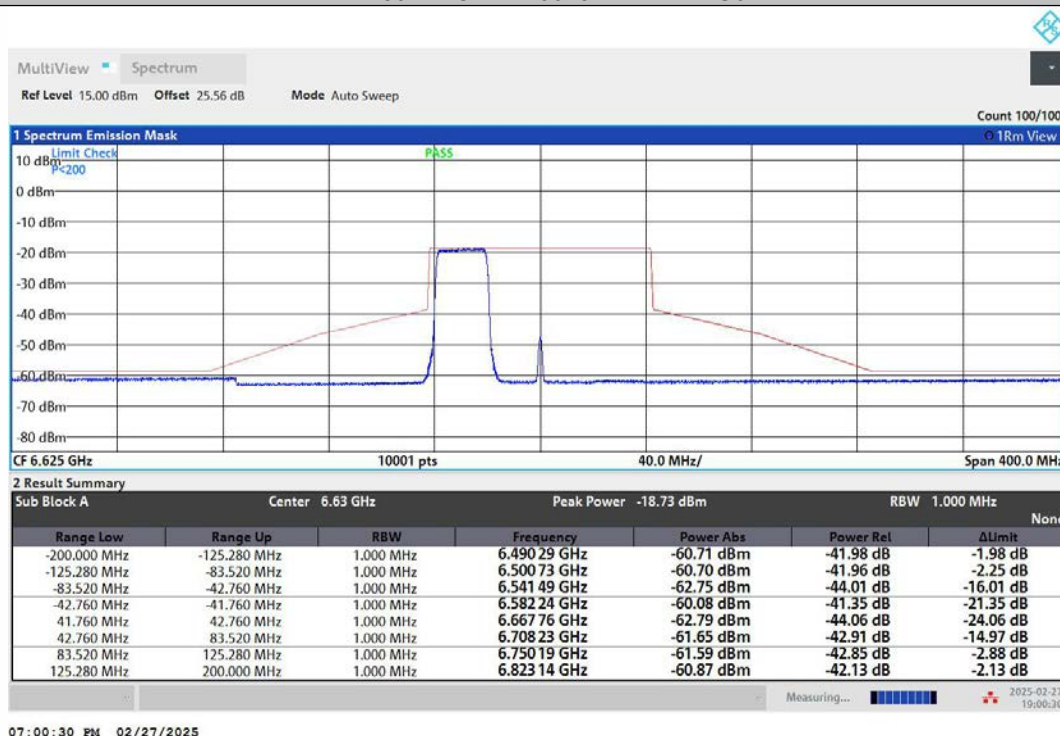
NTNV-11AX80MIMO-Ant1-6625-484Tone-RU65-PASS
