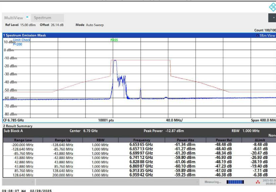
NTNV-11AX80MIMO-Ant1-6785-106Tone-RU53-PASS
