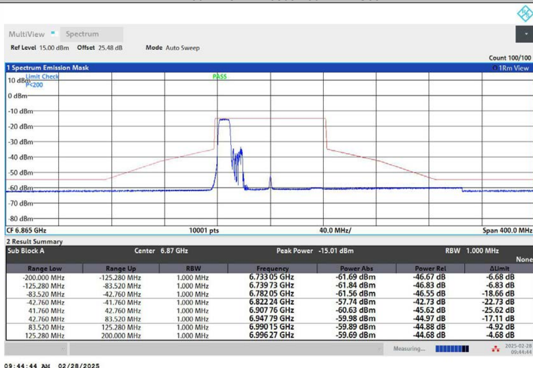
NTNV-11AX80MIMO-Ant1-6865-242Tone-RU61-PASS
