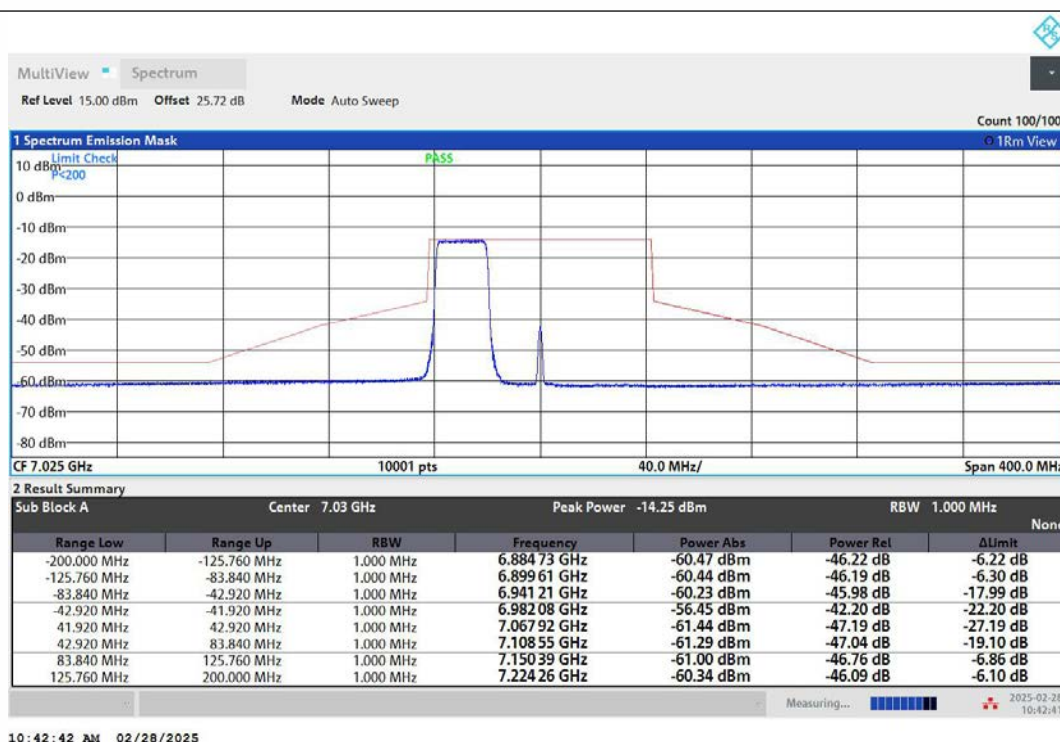
NTNV-11AX80MIMO-Ant2-7025-242Tone-RU61-PASS
