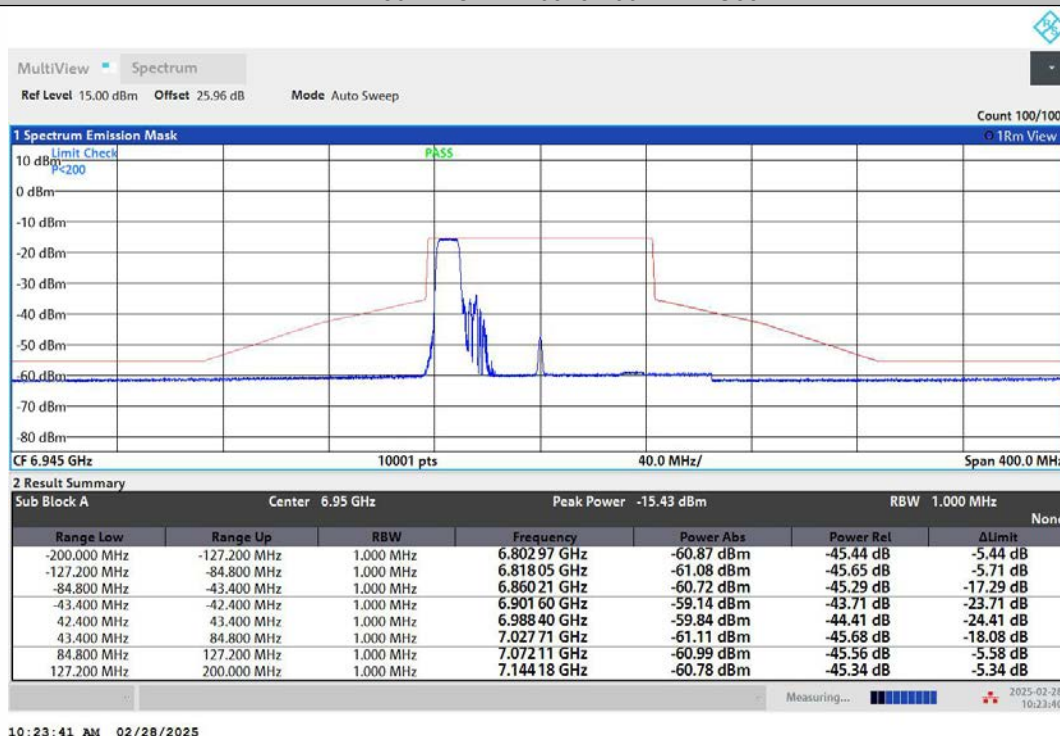
NTNV-11AX80MIMO-Ant1-6945-242Tone-RU61-PASS
