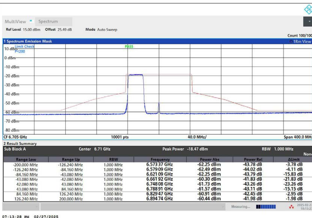
NTNV-11AX80MIMO-Ant2-6705-242Tone-RU61-PASS
