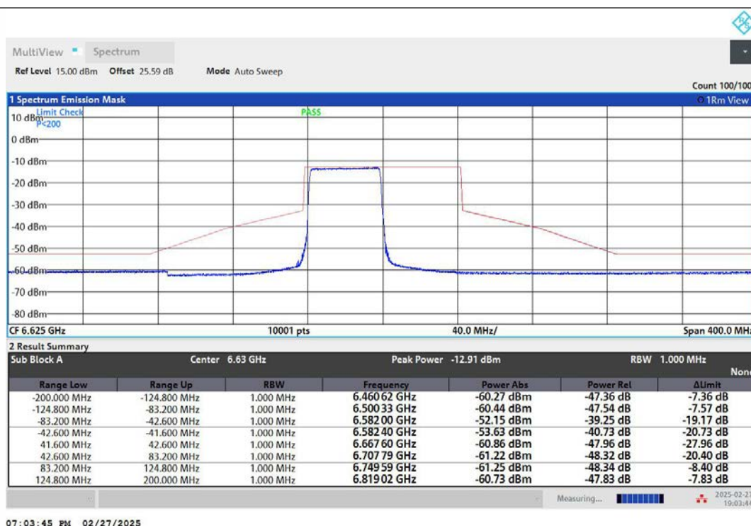
NTNV-11AX80MIMO-Ant2-6625-484Tone-RU65-PASS
