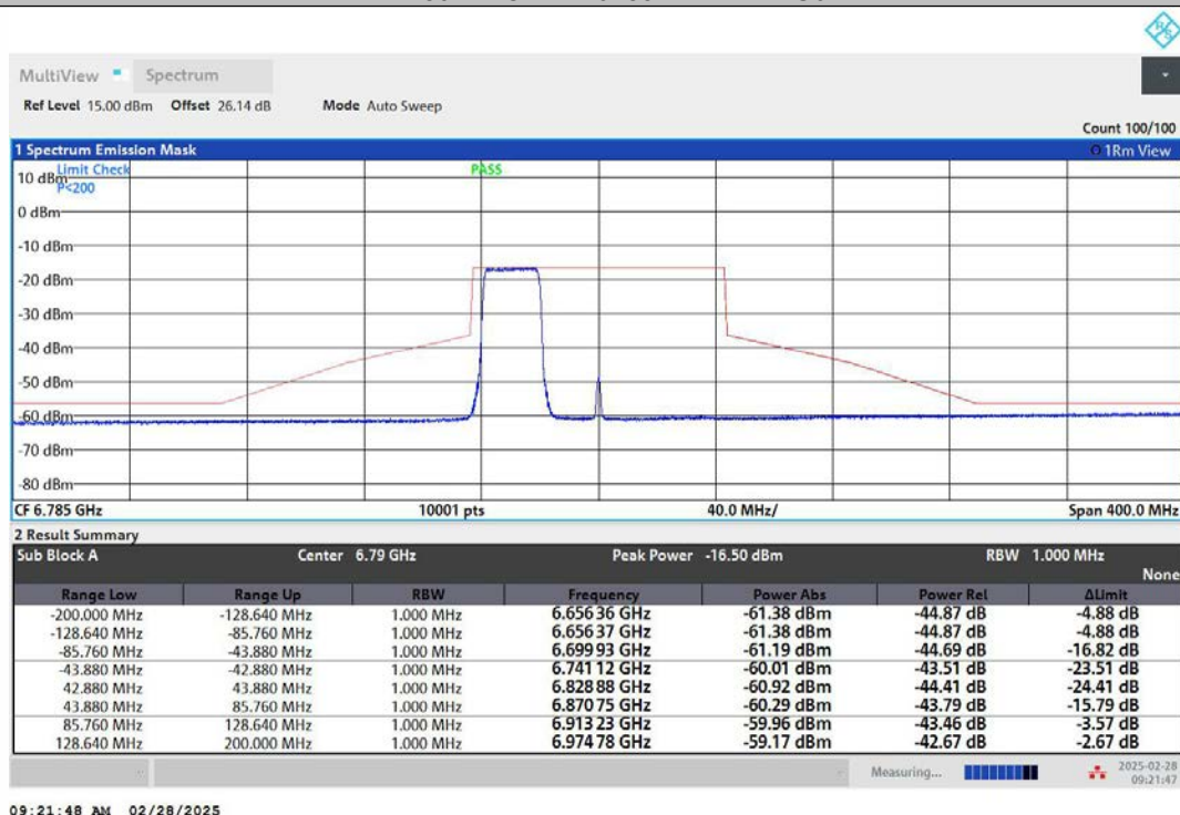
NTNV-11AX80MIMO-Ant1-6785-484Tone-RU65-PASS
