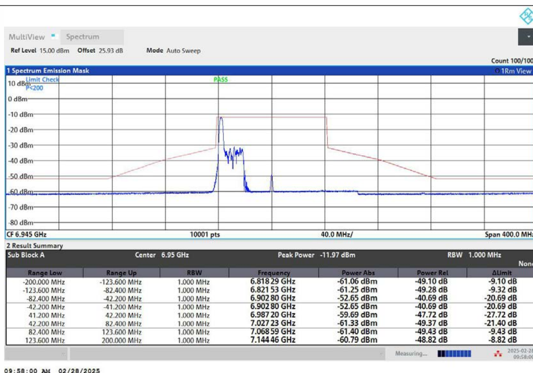
NTNV-11AX80MIMO-Ant2-6945-26Tone-RU0-PASS
