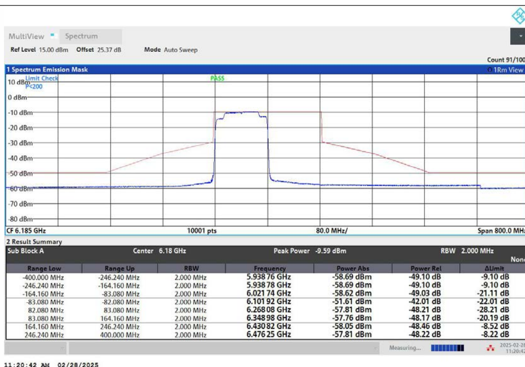
NTNV-11AX160MIMO-Ant2-6185-996Tone-RU67-PASS
