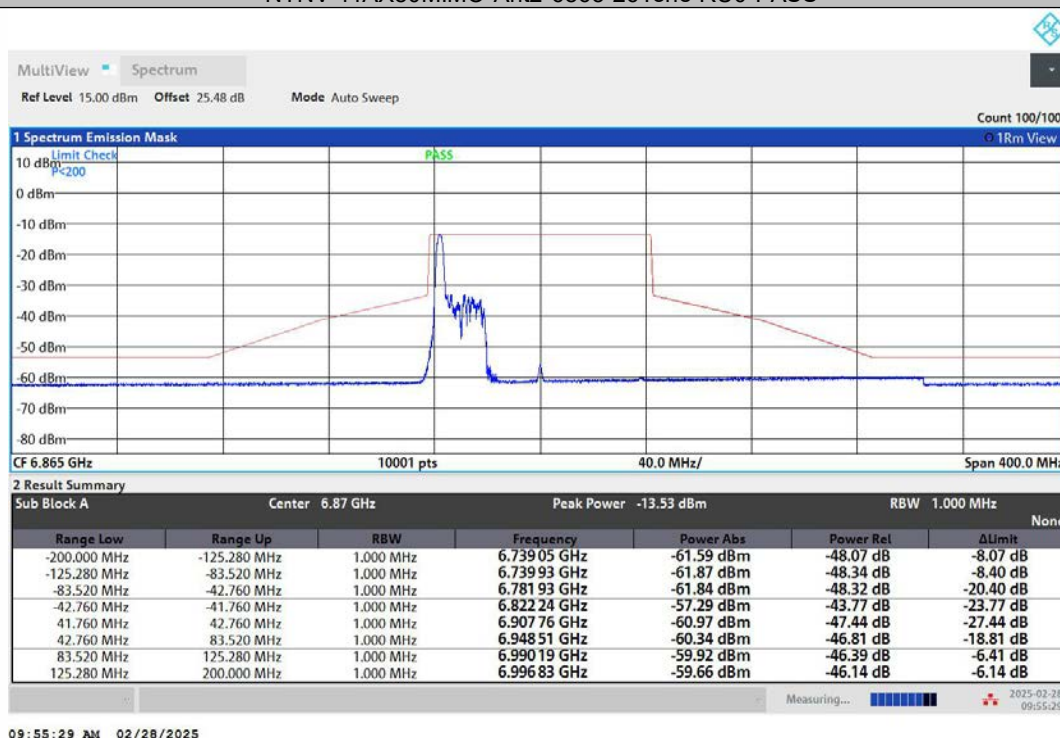
NTNV-11AX80MIMO-Ant1-6865-52Tone-RU37-PASS
