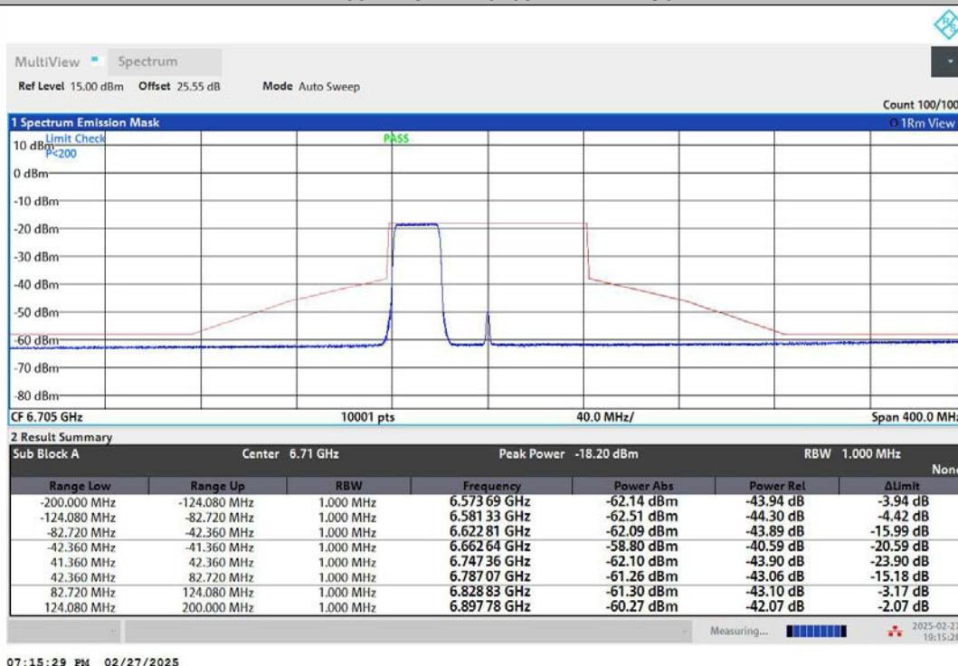
NTNV-11AX80MIMO-Ant1-6705-484Tone-RU65-PASS
