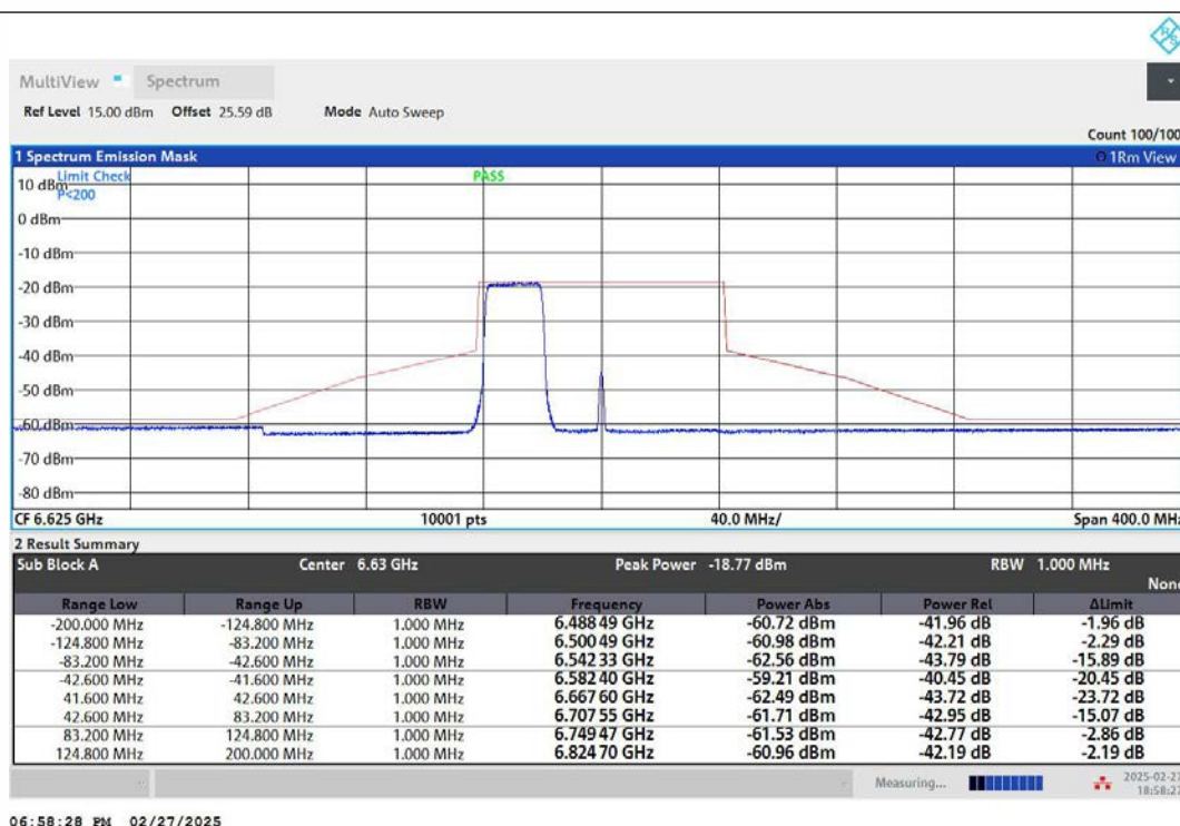
NTNV-11AX80MIMO-Ant2-6625-242Tone-RU61-PASS
