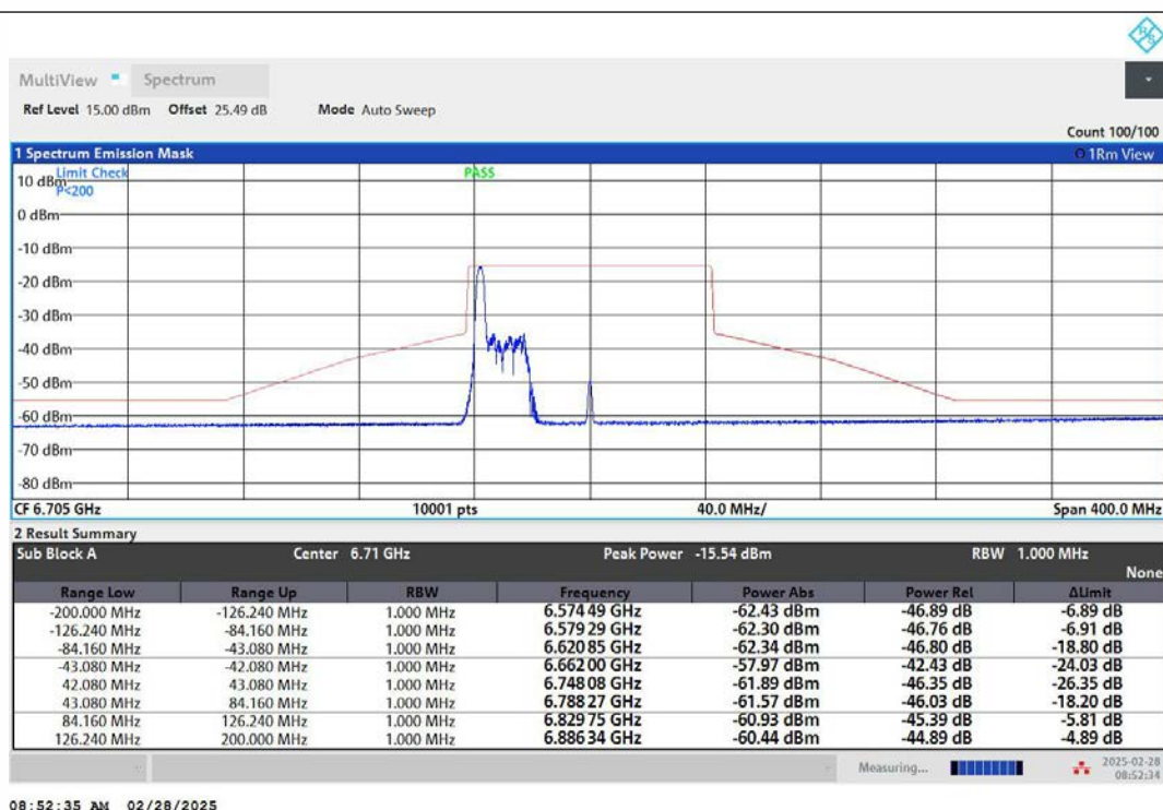
NTNV-11AX80MIMO-Ant2-6705-26Tone-RU0-PASS
