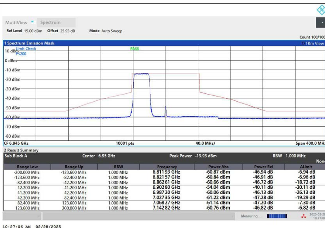
NTNV-11AX80MIMO-Ant2-6945-242Tone-RU61-PASS
