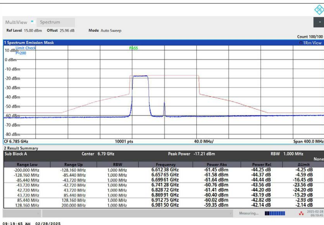
NTNV-11AX80MIMO-Ant2-6785-242Tone-RU61-PASS
