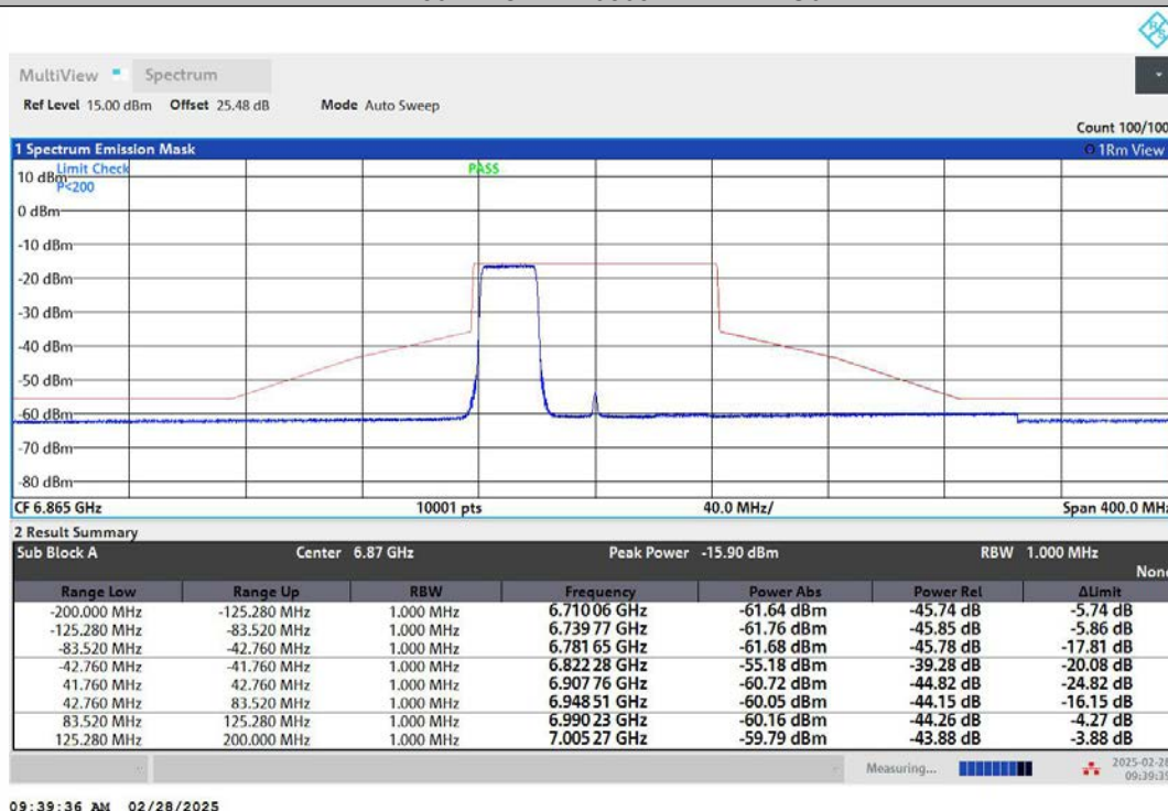
NTNV-11AX80MIMO-Ant1-6865-484Tone-RU65-PASS
