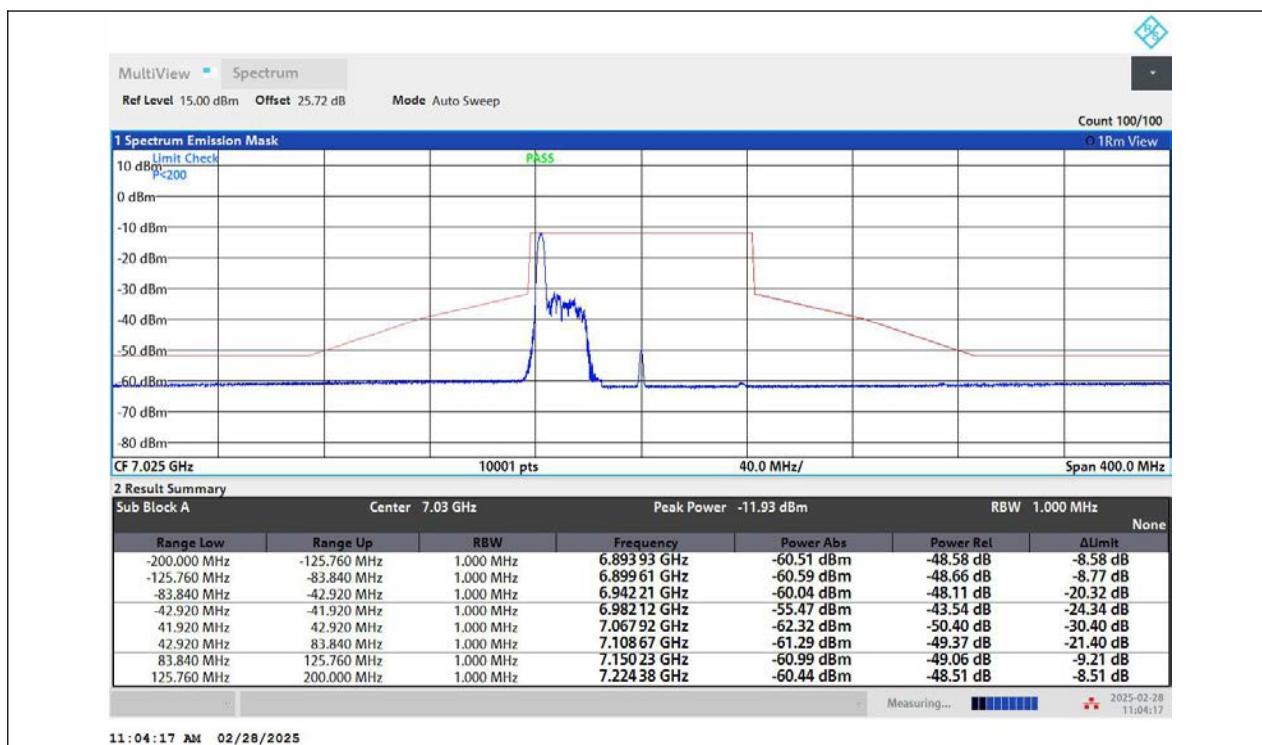
NTNV-11AX80MIMO-Ant2-7025-26Tone-RU0-PASS
