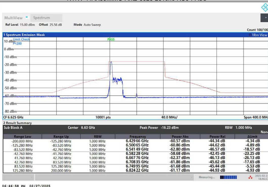
NTNV-11AX80MIMO-Ant1-6625-52Tone-RU37-PASS
