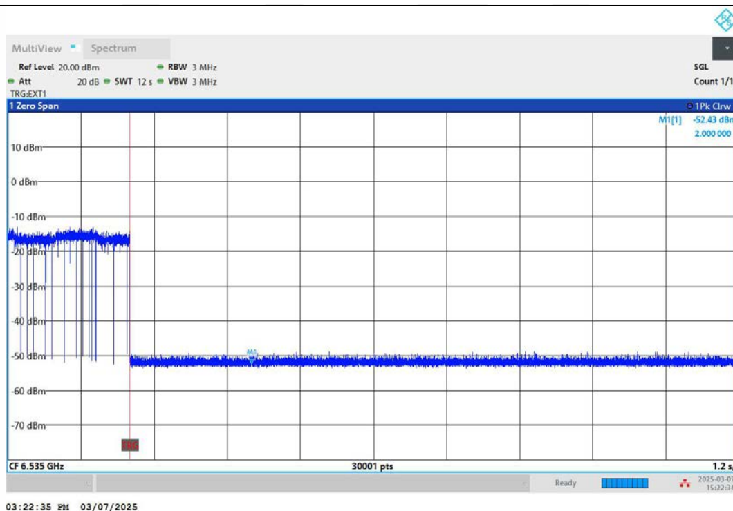
11AX20MIMO-Ant1-6535-Center-6535-Minimal
