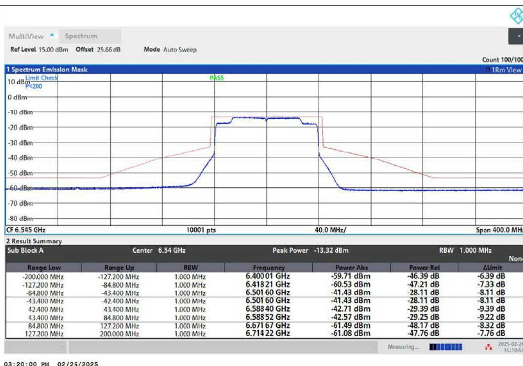
NTNV-11AX80MIMO-Ant2-6545-PASS
