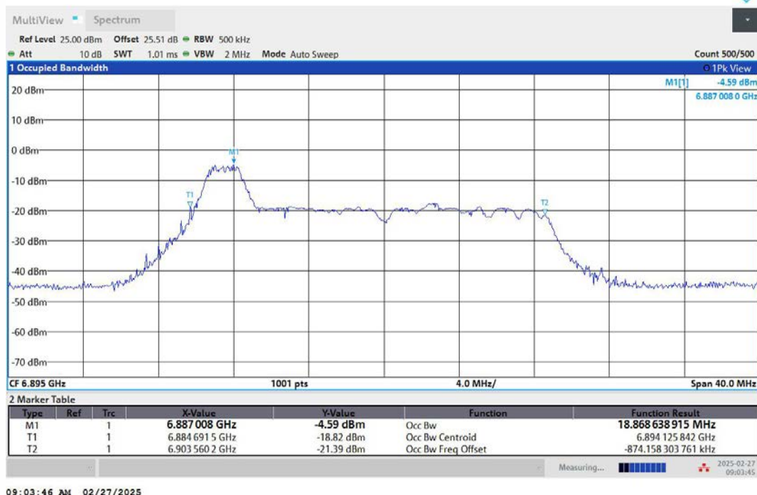
11AX20MIMO-Ant2-6895-26Tone-RU0-PASS
