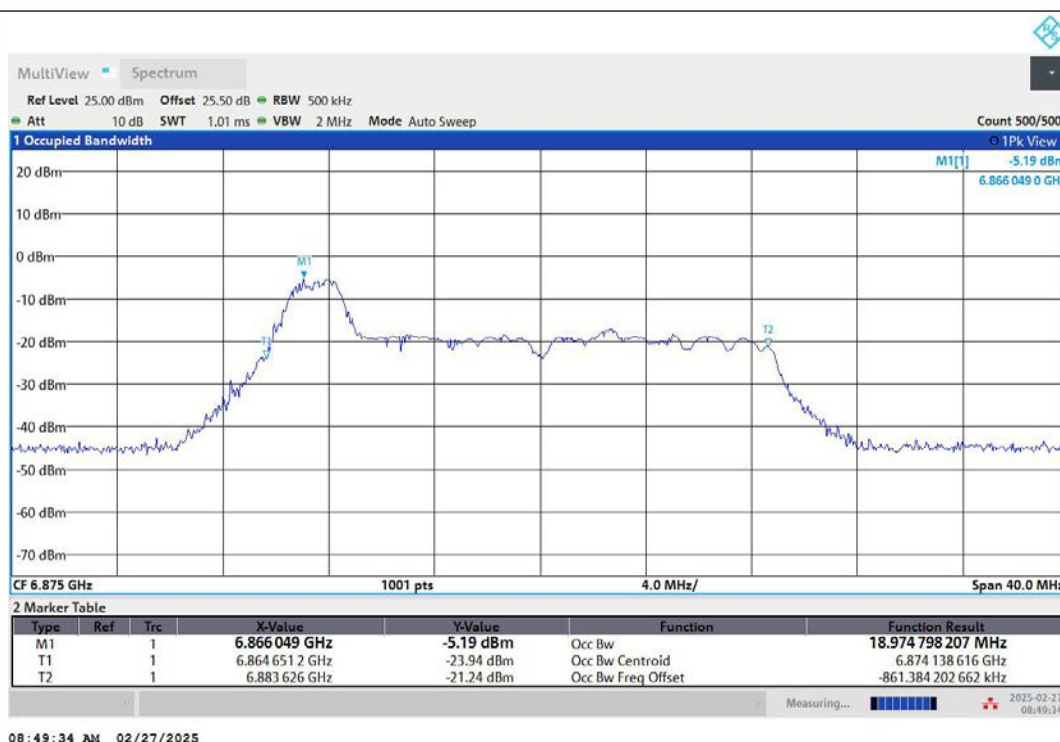
11AX20MIMO-Ant2-6875-26Tone-RU0-PASS
