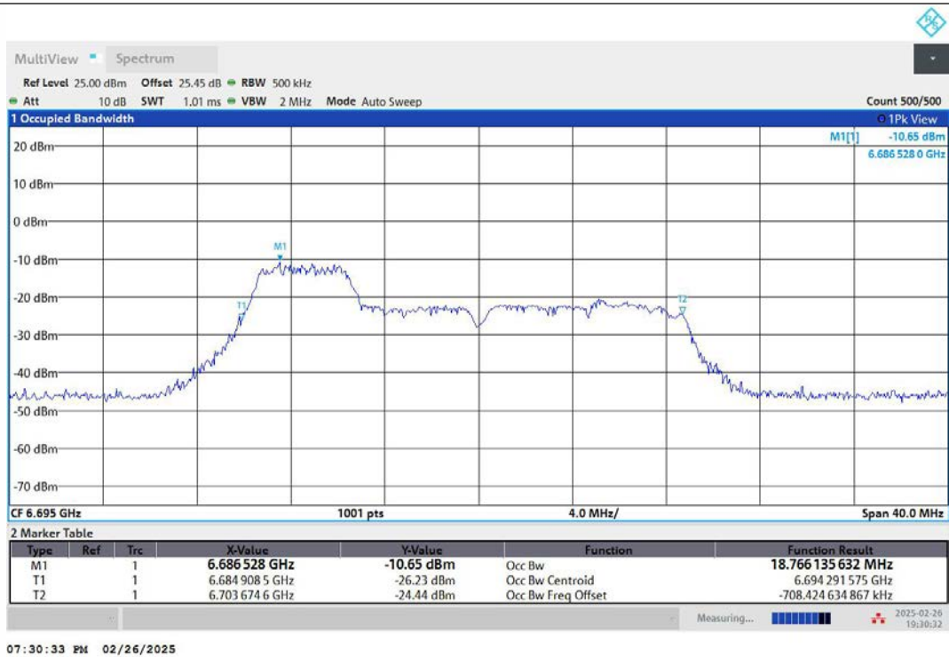
11AX20MIMO-Ant2-6695-52Tone-RU37-PASS
