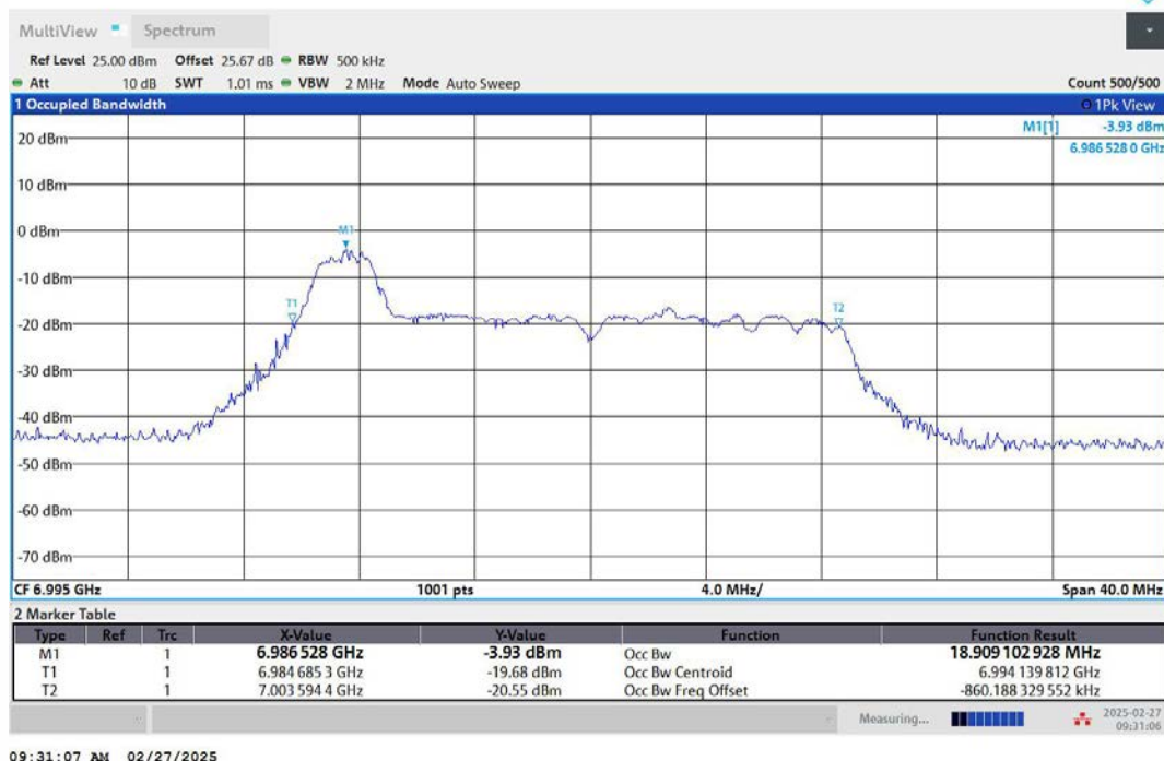
11AX20MIMO-Ant2-6995-26Tone-RU0-PASS
