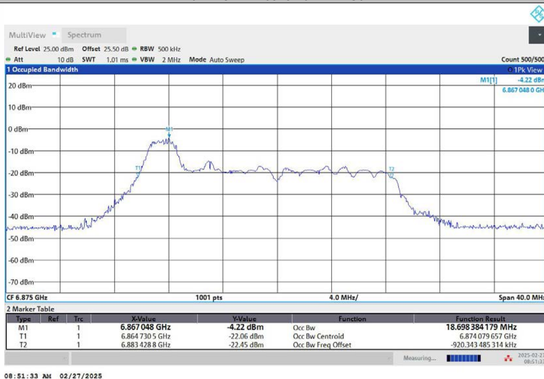
11AX20MIMO-Ant1-6875-52Tone-RU37-PASS
