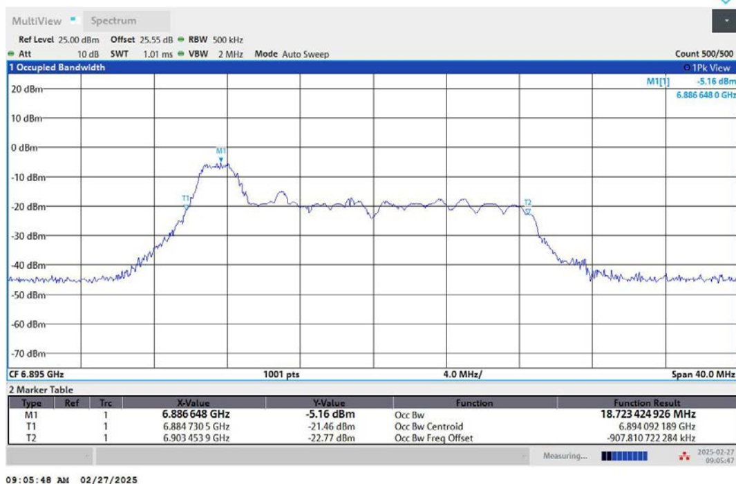
11AX20MIMO-Ant1-6895-52Tone-RU37-PASS
