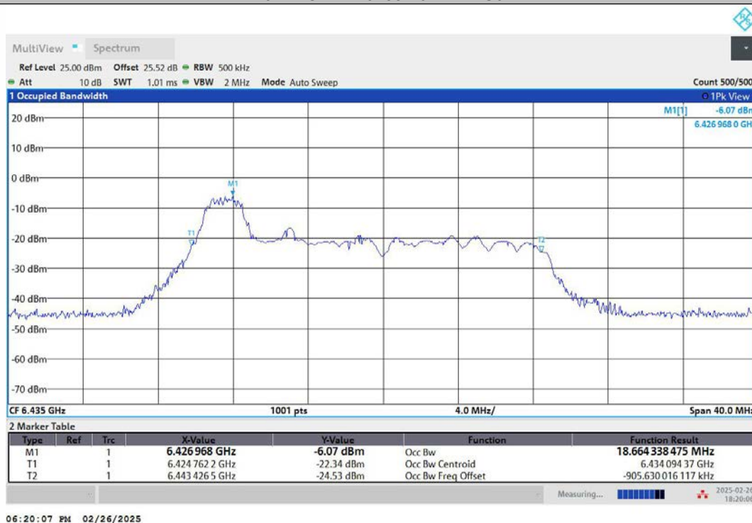
11AX20MIMO-Ant1-6435-52Tone-RU37-PASS
