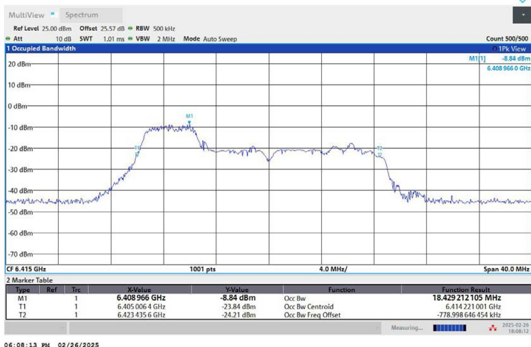
11AX20MIMO-Ant1-6415-106Tone-RU53-PASS
