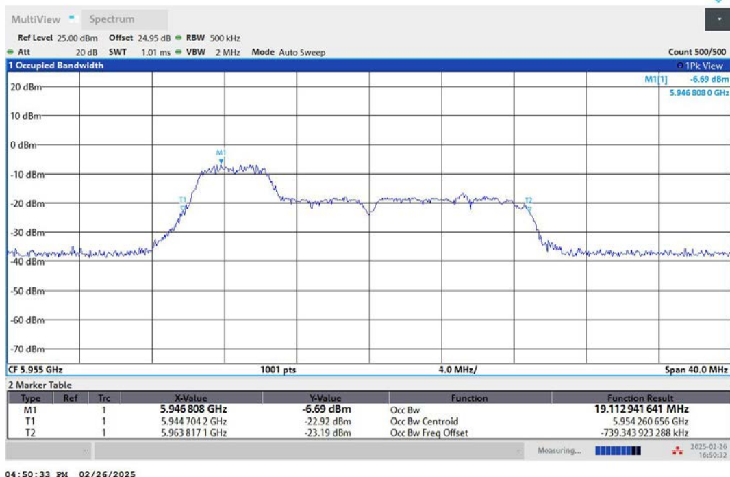
11AX20MIMO-Ant2-5955-52Tone-RU37-PASS
