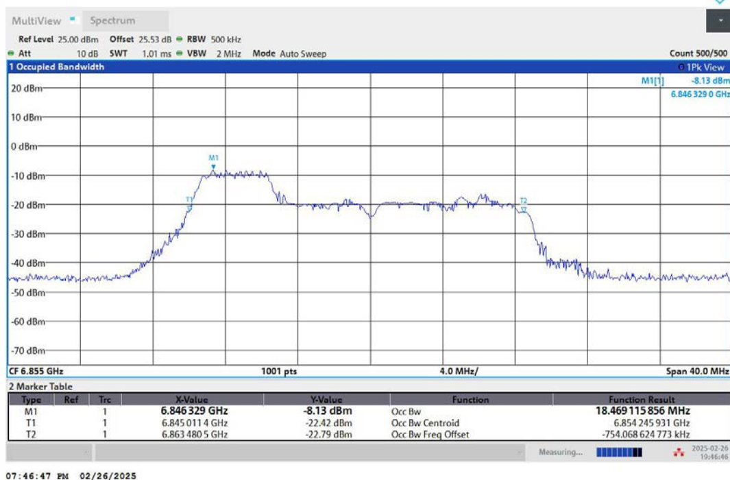
11AX20MIMO-Ant1-6855-106Tone-RU53-PASS
