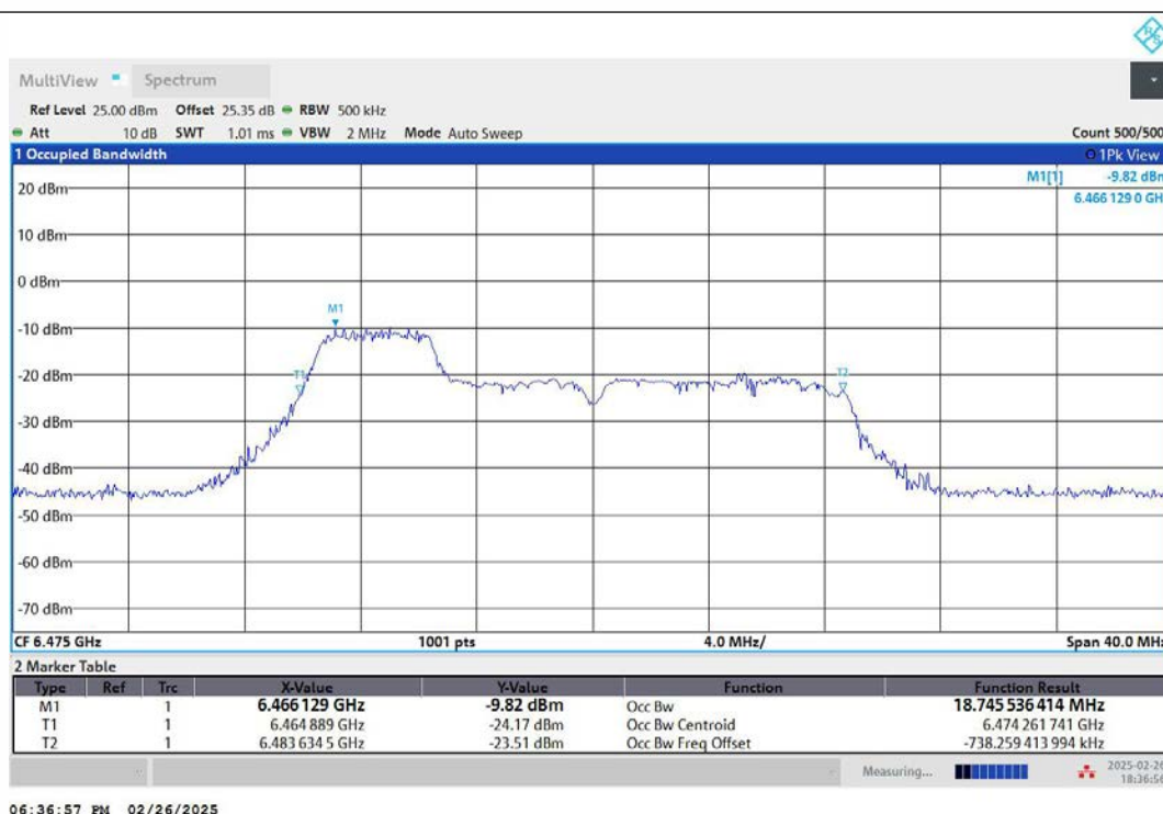
11AX20MIMO-Ant2-6475-52Tone-RU37-PASS
