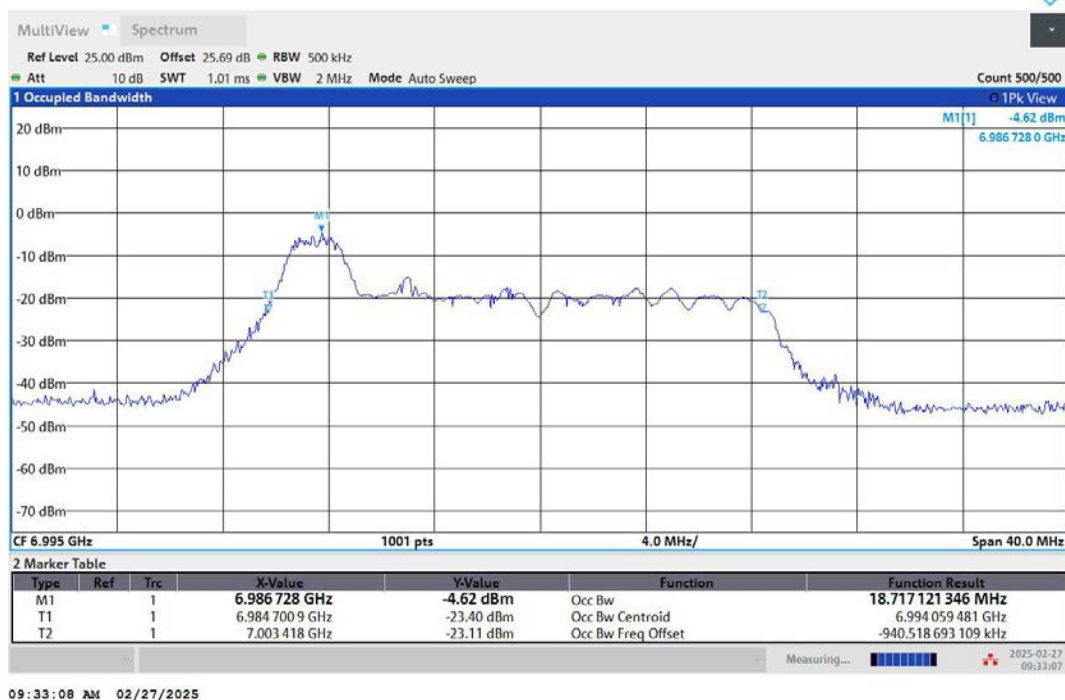
11AX20MIMO-Ant1-6995-52Tone-RU37-PASS
