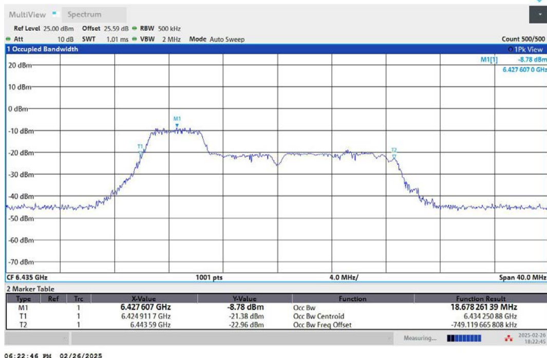
11AX20MIMO-Ant2-6435-52Tone-RU37-PASS
