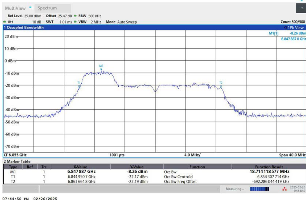
11AX20MIMO-Ant2-6855-52Tone-RU37-PASS
