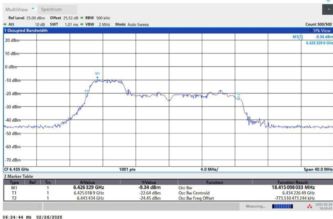
11AX20MIMO-Ant1-6435-106Tone-RU53-PASS
