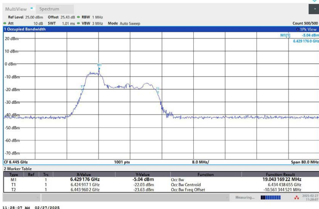
11AX40MIMO-Ant1-6445-106Tone-RU53-PASS
