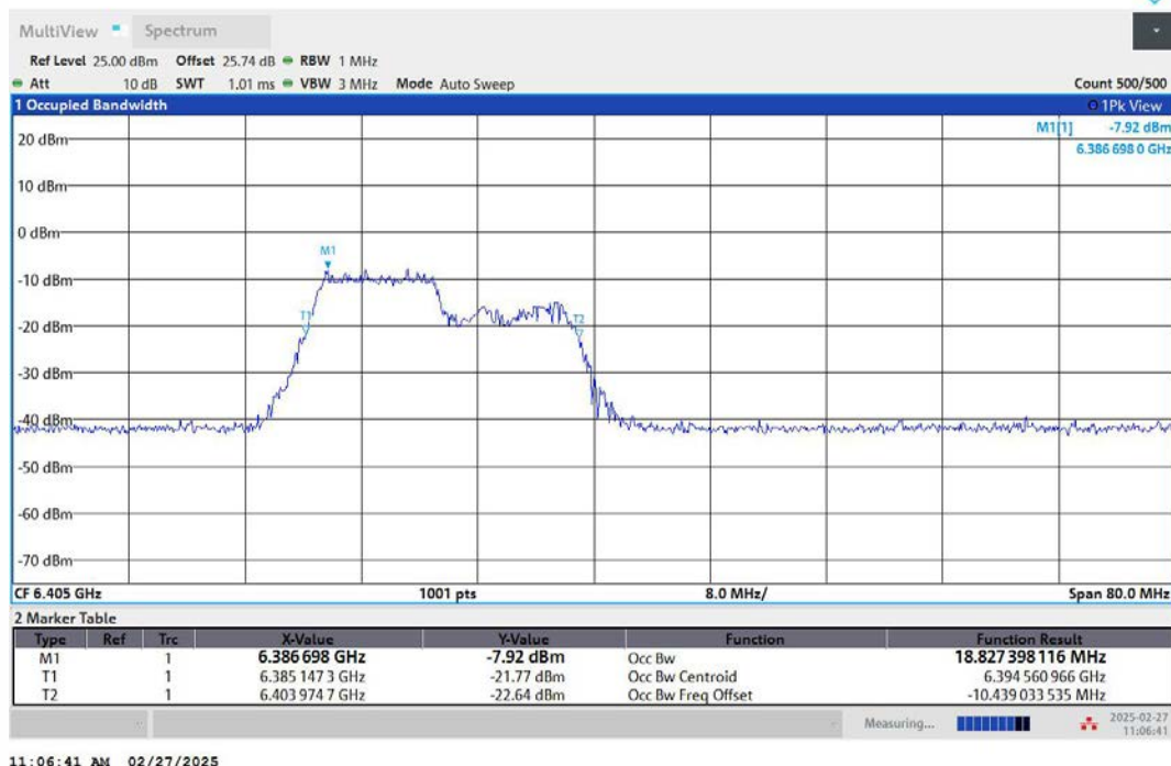
11AX40MIMO-Ant2-6405-106Tone-RU53-PASS
