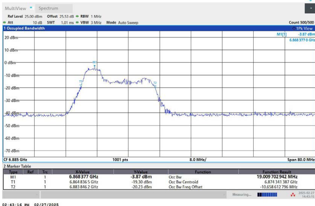
11AX40MIMO-Ant2-6885-52Tone-RU37-PASS
