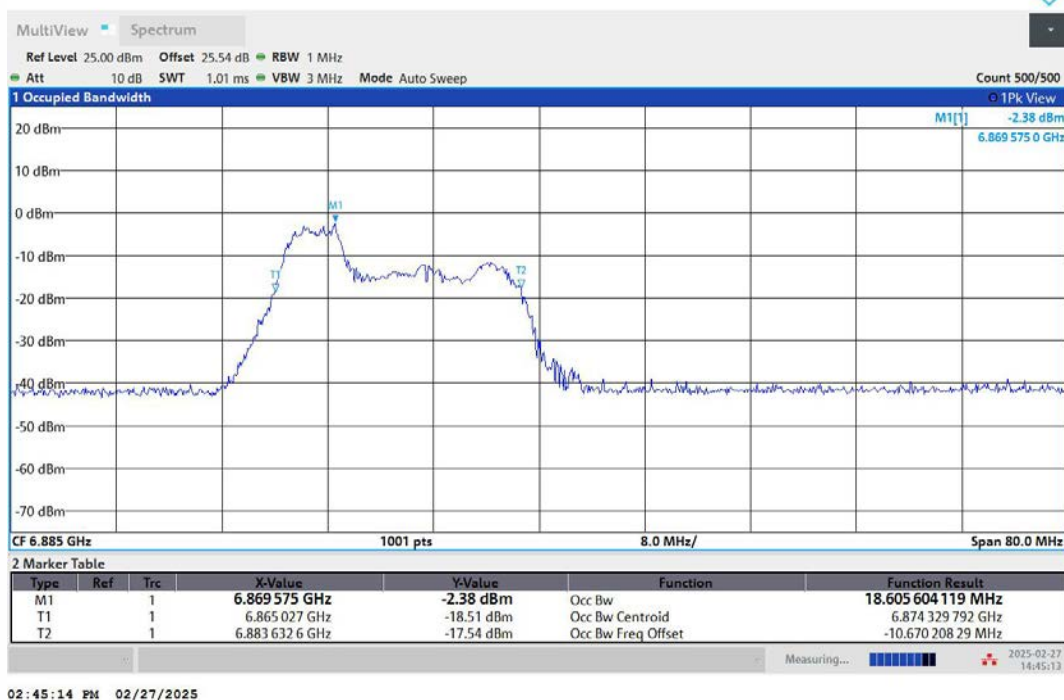
11AX40MIMO-Ant1-6885-106Tone-RU53-PASS
