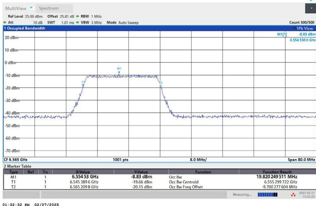
11AX40MIMO-Ant2-6565-242Tone-RU61-PASS
