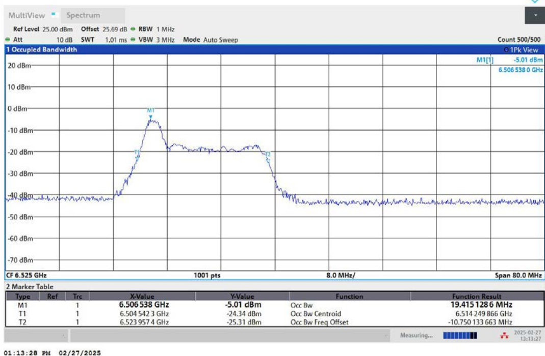
11AX40MIMO-Ant1-6525-52Tone-RU37-PASS
