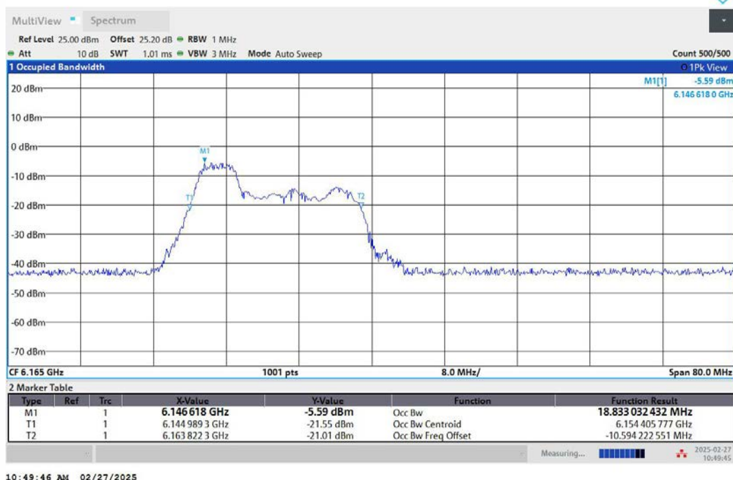
11AX40MIMO-Ant1-6165-106Tone-RU53-PASS
