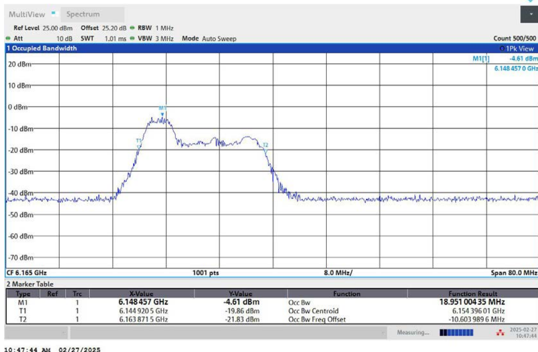
11AX40MIMO-Ant2-6165-52Tone-RU37-PASS
