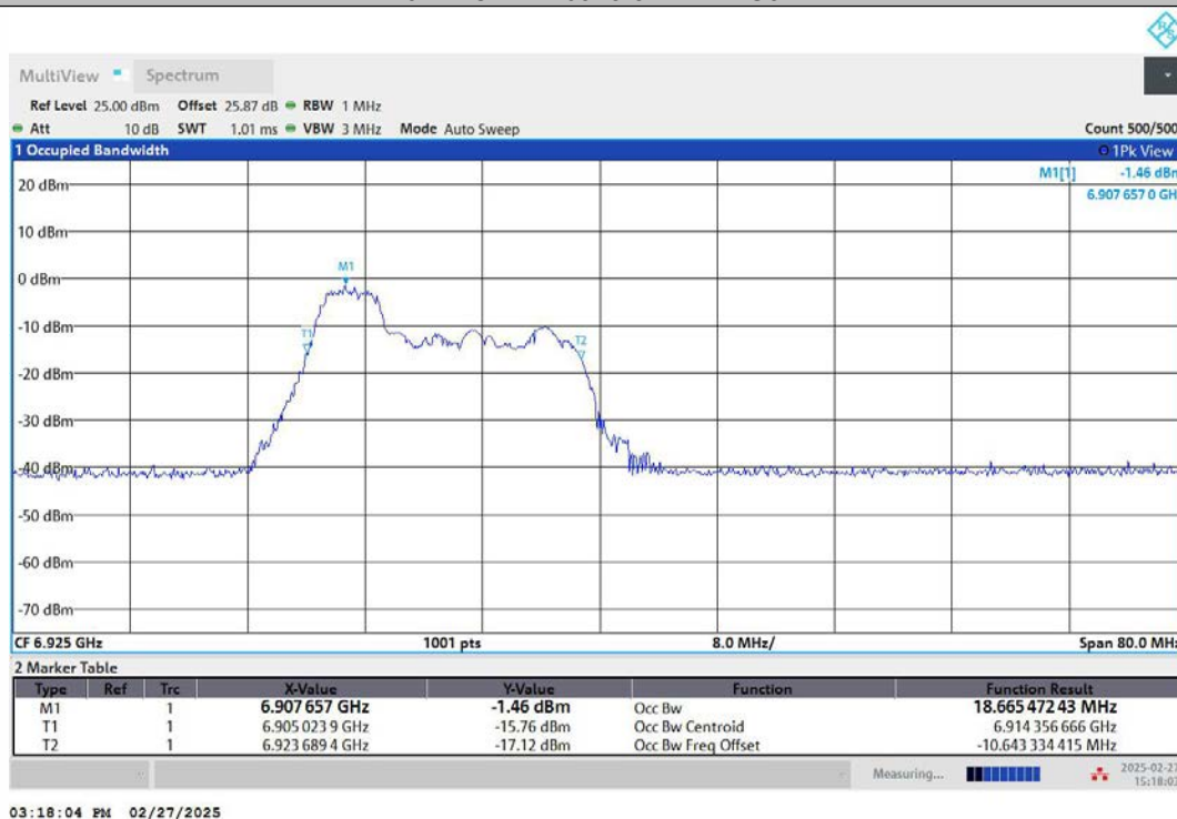
11AX40MIMO-Ant1-6925-106Tone-RU53-PASS
