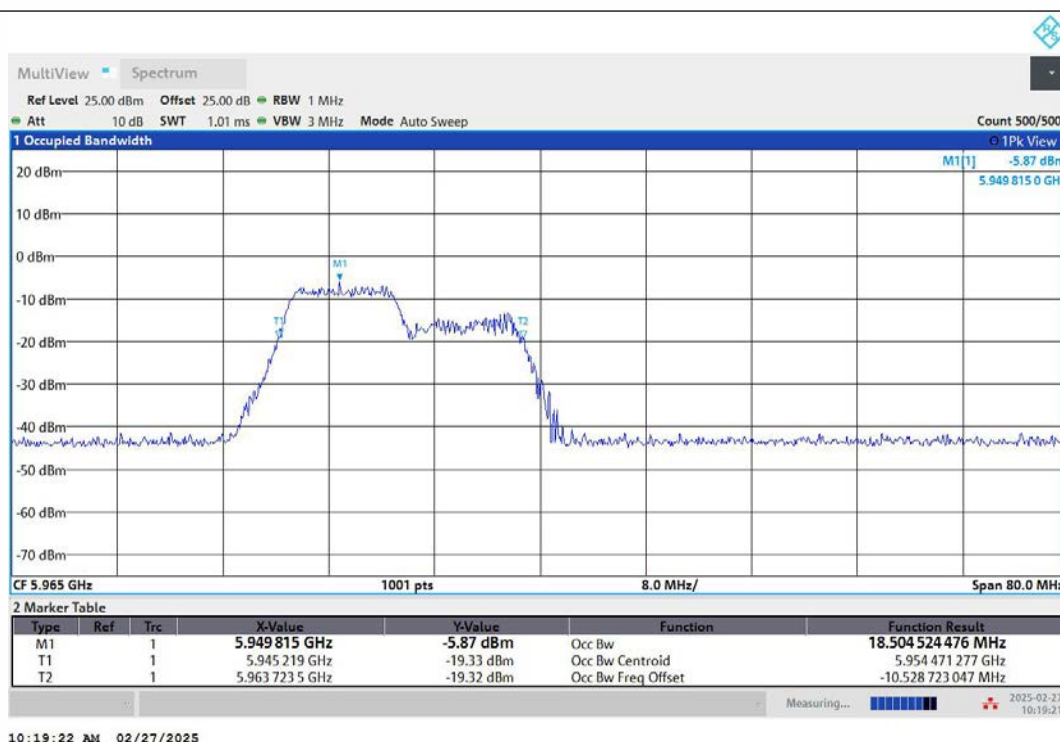
11AX40MIMO-Ant2-5965-106Tone-RU53-PASS
