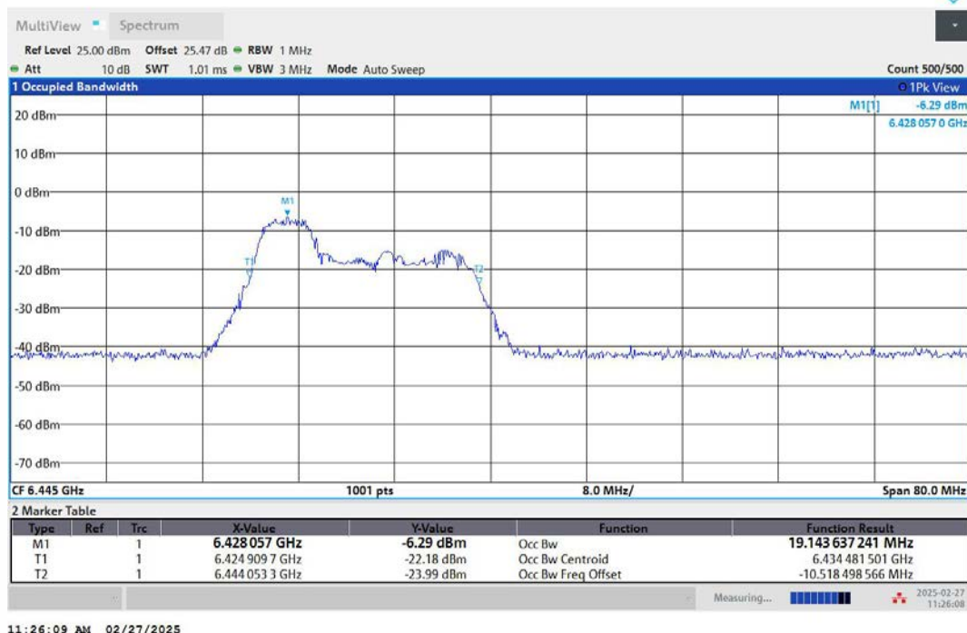
11AX40MIMO-Ant2-6445-52Tone-RU37-PASS
