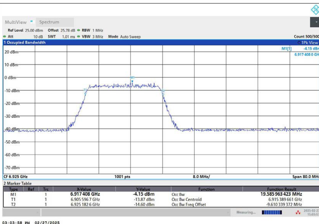
11AX40MIMO-Ant2-6925-242Tone-RU61-PASS
