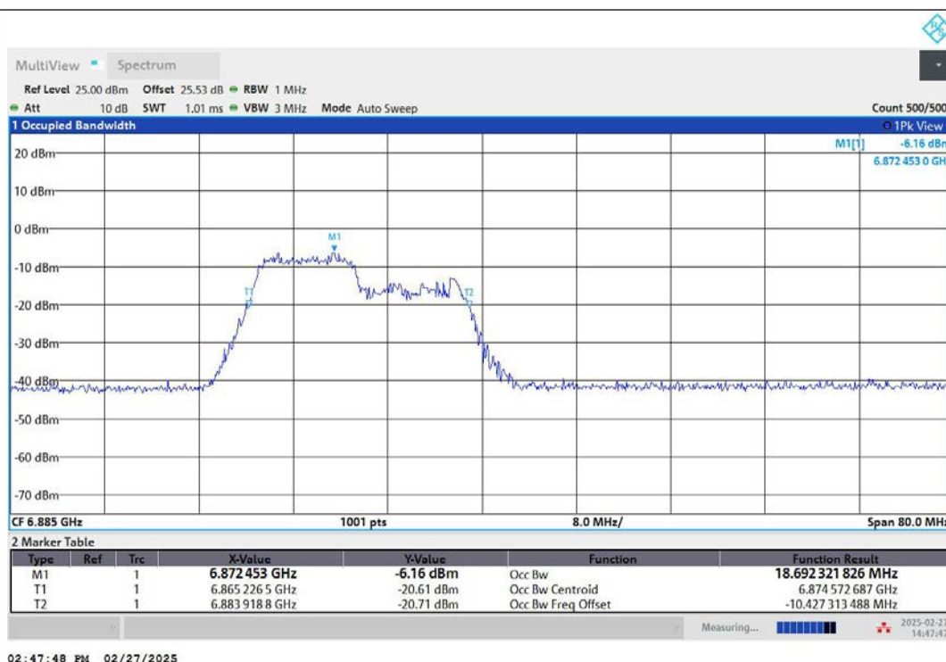
11AX40MIMO-Ant2-6885-106Tone-RU53-PASS
