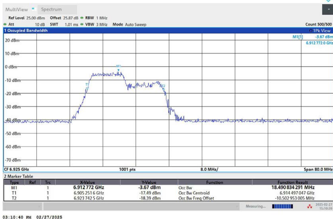
11AX40MIMO-Ant1-6925-242Tone-RU61-PASS
