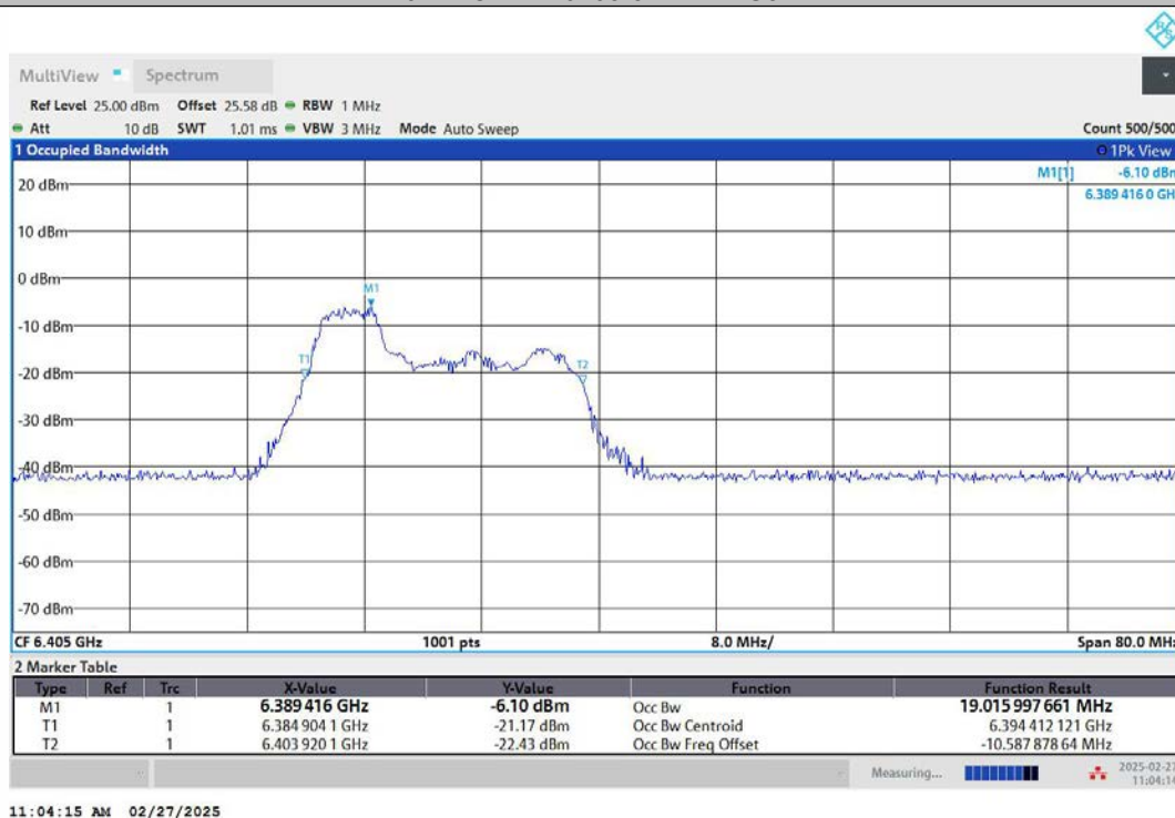
11AX40MIMO-Ant1-6405-106Tone-RU53-PASS
