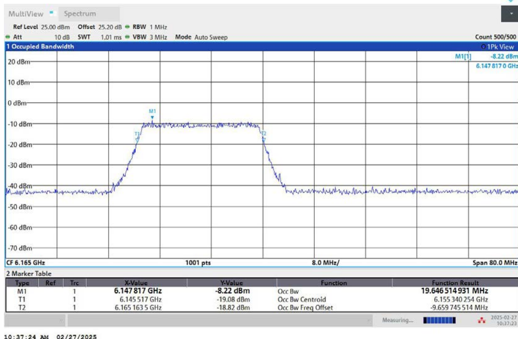
11AX40MIMO-Ant2-6165-242Tone-RU61-PASS
