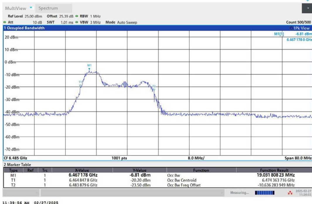
11AX40MIMO-Ant2-6485-52Tone-RU37-PASS
