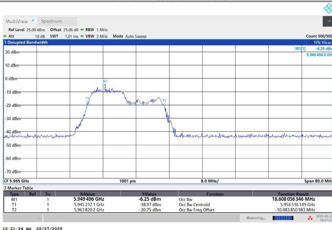
11AX40MIMO-Ant1-5965-242Tone-RU61-PASS
