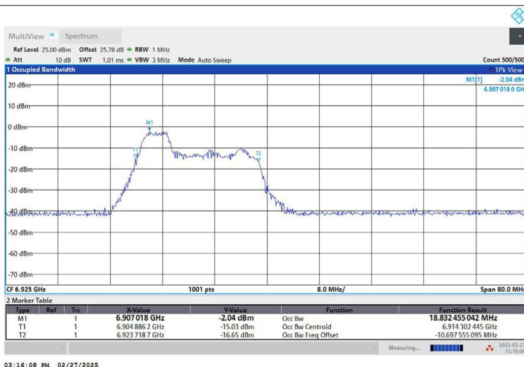
11AX40MIMO-Ant2-6925-52Tone-RU37-PASS
