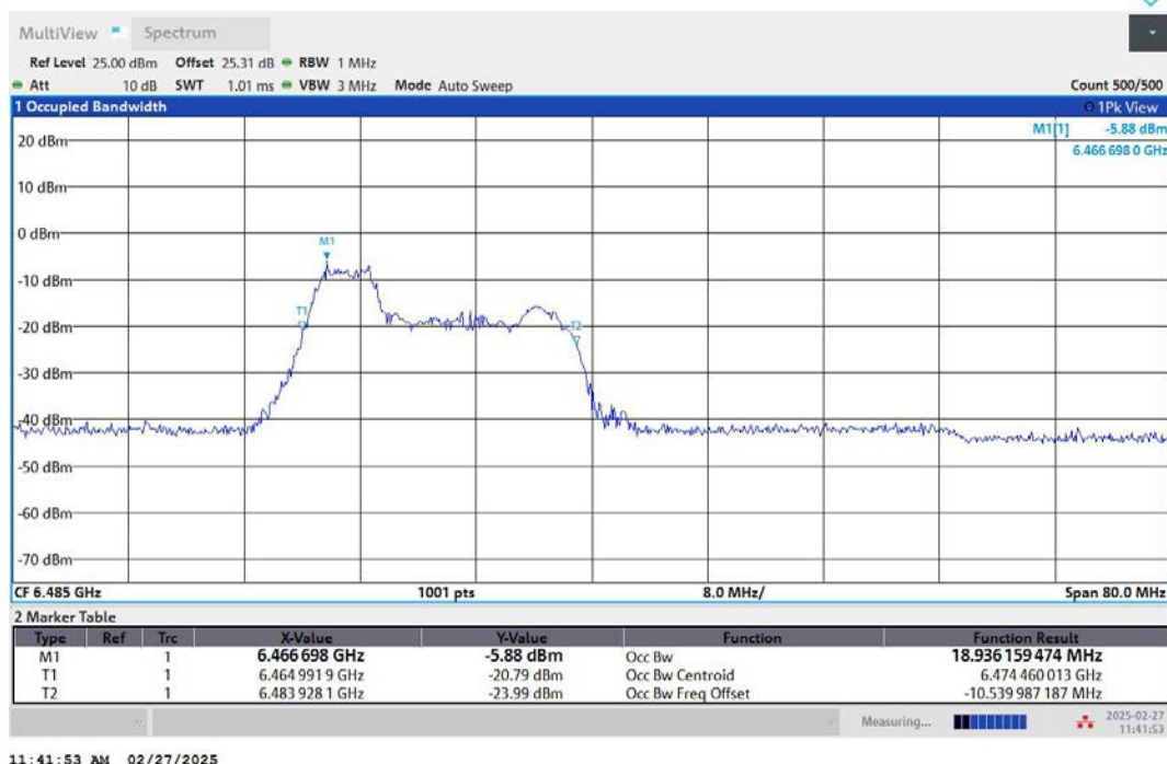
11AX40MIMO-Ant1-6485-106Tone-RU53-PASS
