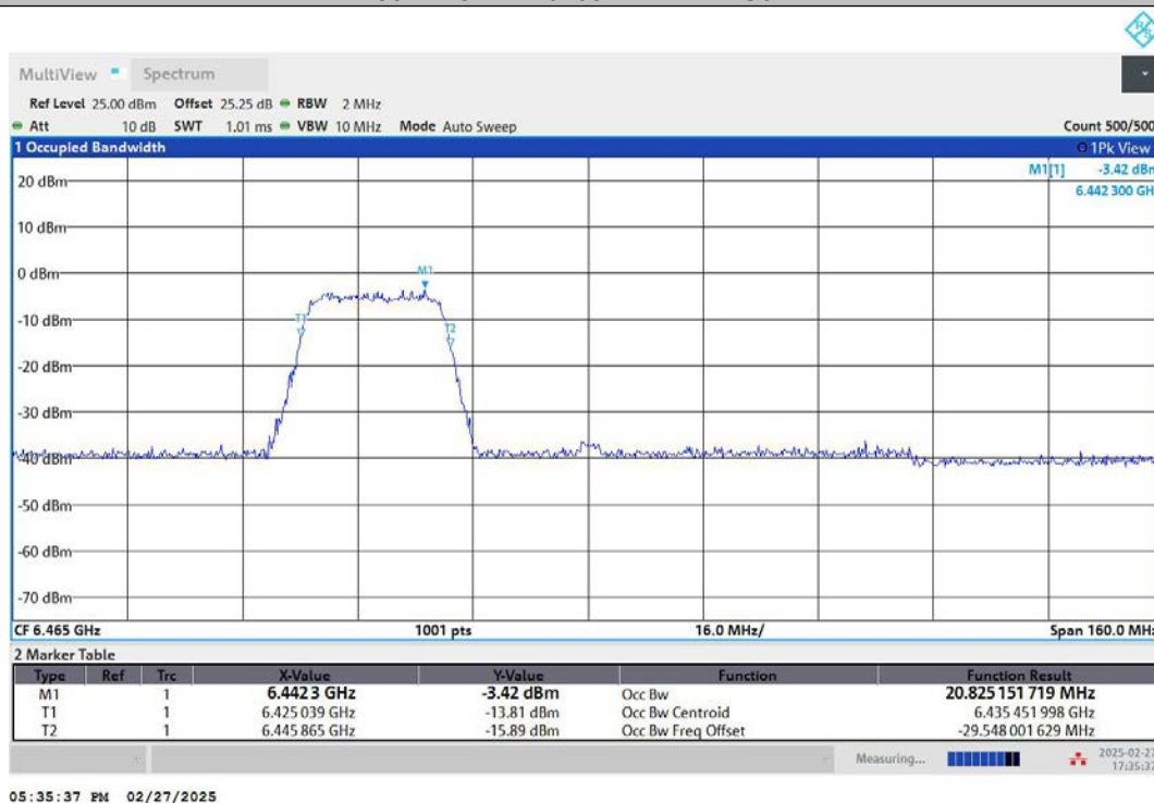
11AX80MIMO-Ant1-6465-484Tone-RU65-PASS
