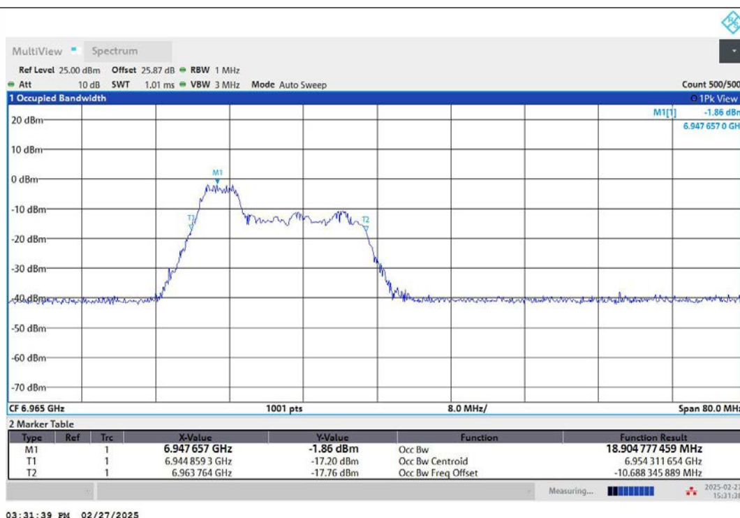
11AX40MIMO-Ant2-6965-52Tone-RU37-PASS
