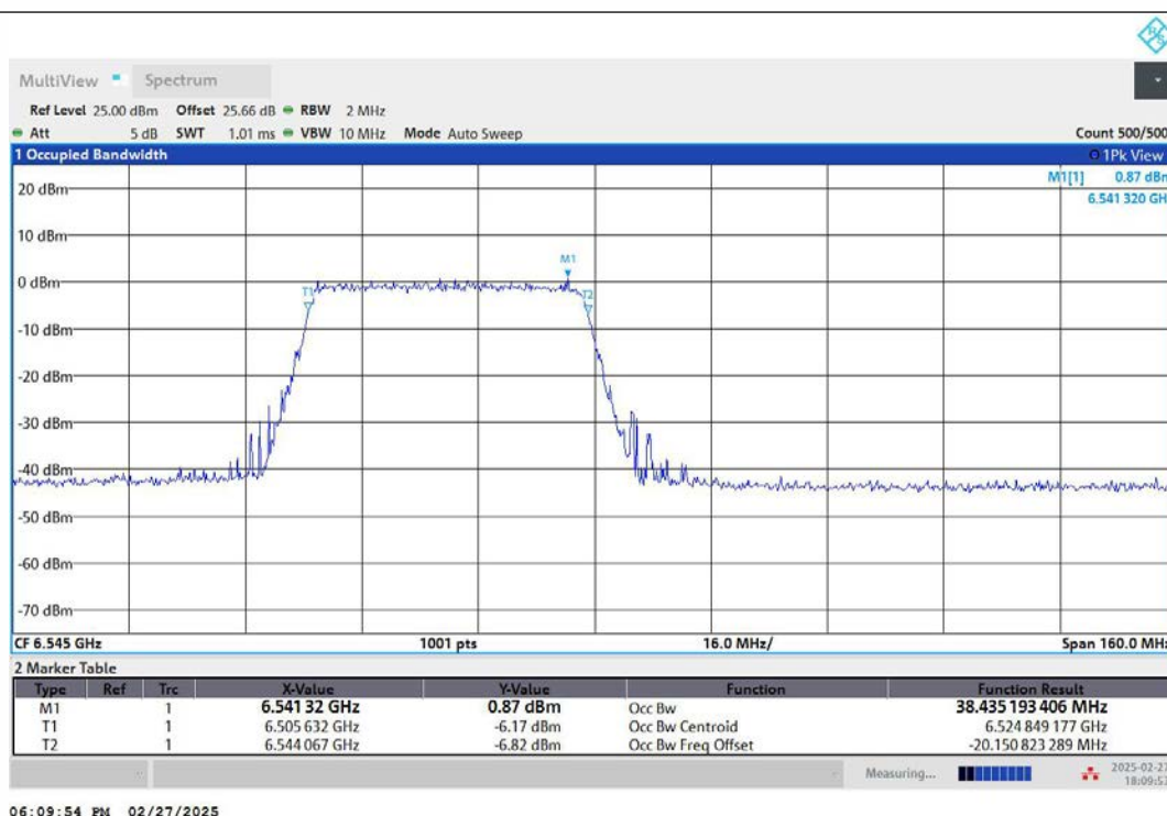
11AX80MIMO-Ant2-6545-484Tone-RU65-PASS
