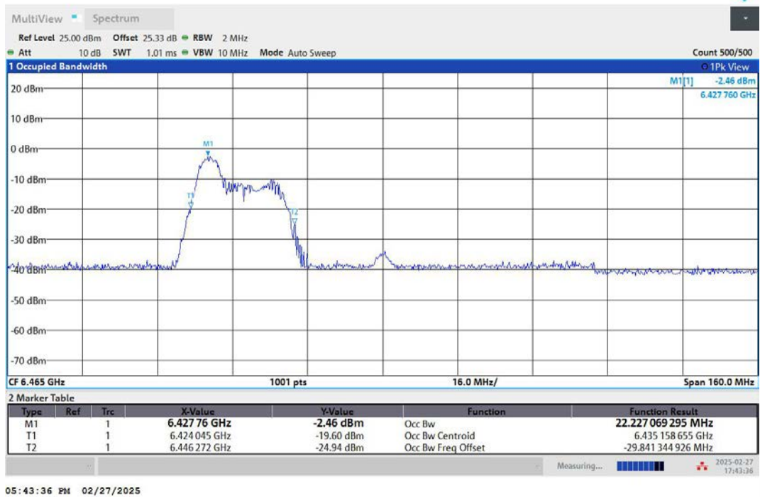
11AX80MIMO-Ant2-6465-52Tone-RU37-PASS
