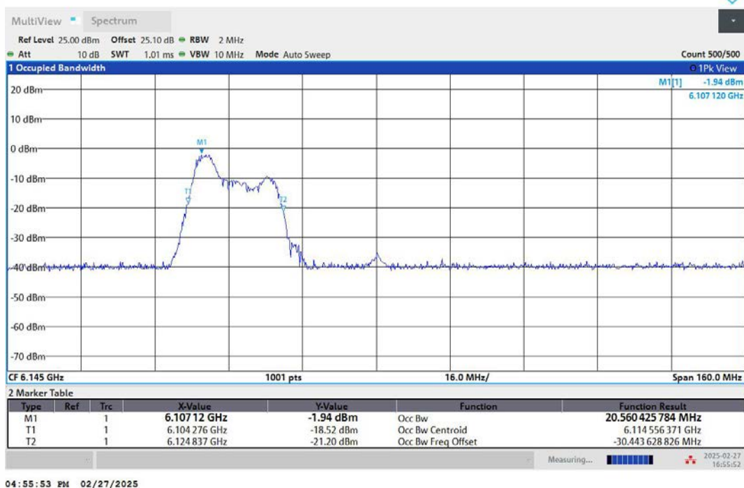
11AX80MIMO-Ant1-6145-106Tone-RU53-PASS
