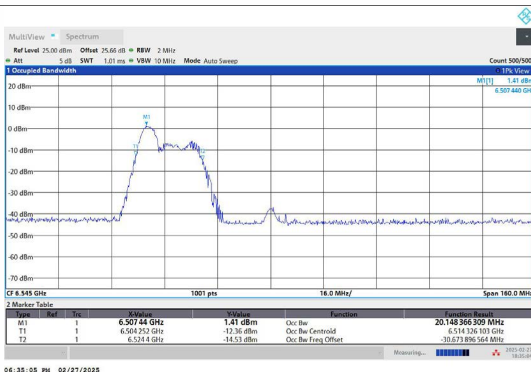
11AX80MIMO-Ant2-6545-52Tone-RU37-PASS
