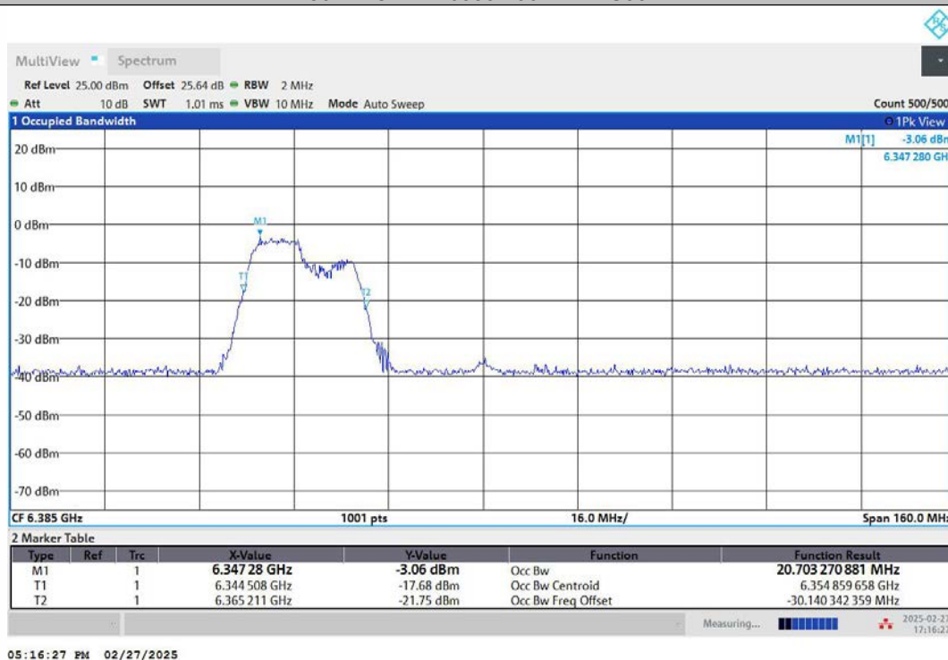
11AX80MIMO-Ant1-6385-242Tone-RU61-PASS
