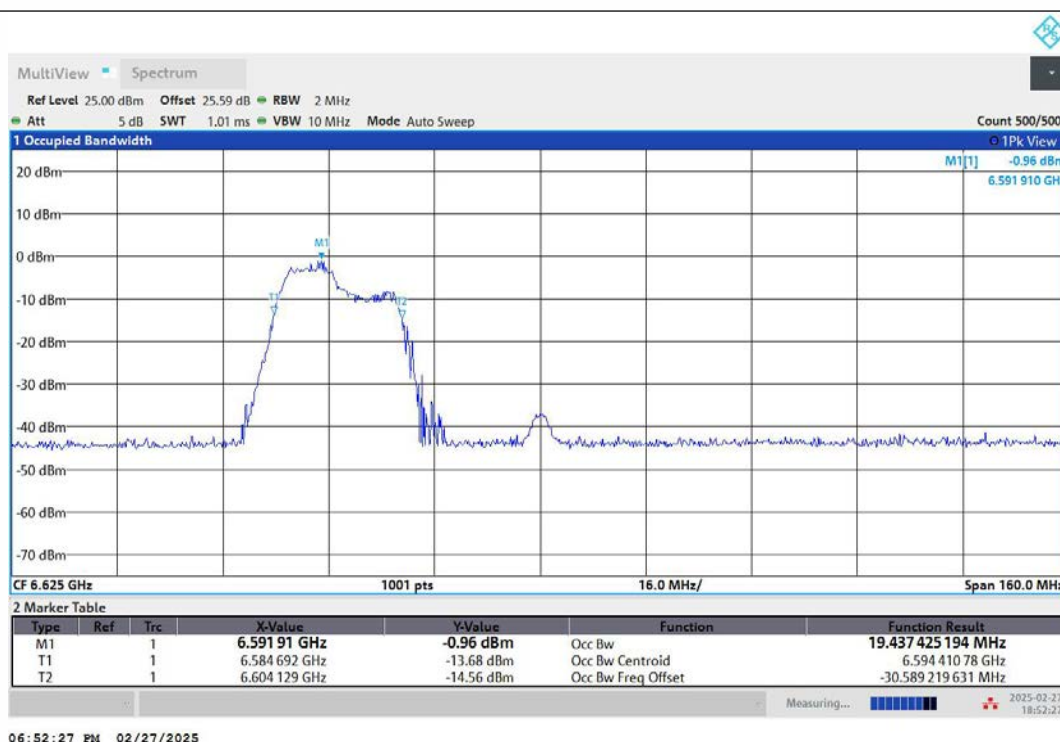
11AX80MIMO-Ant2-6625-106Tone-RU53-PASS
