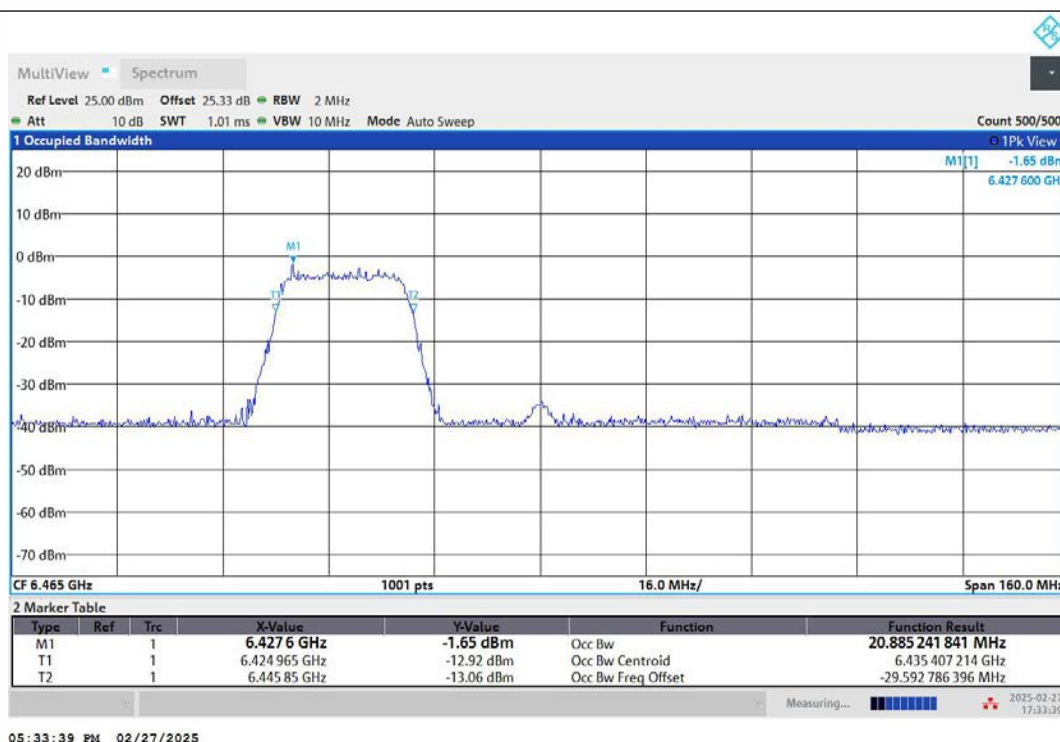
11AX80MIMO-Ant2-6465-242Tone-RU61-PASS
