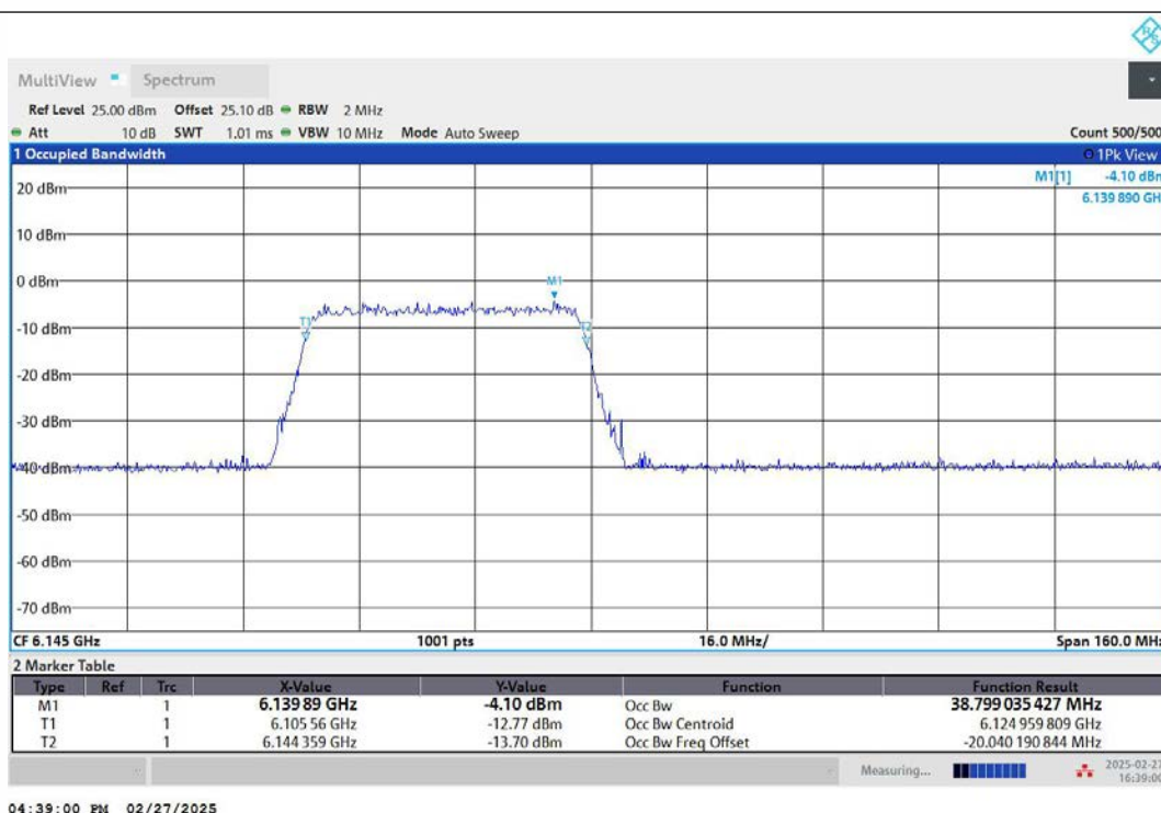
11AX80MIMO-Ant2-6145-484Tone-RU65-PASS
