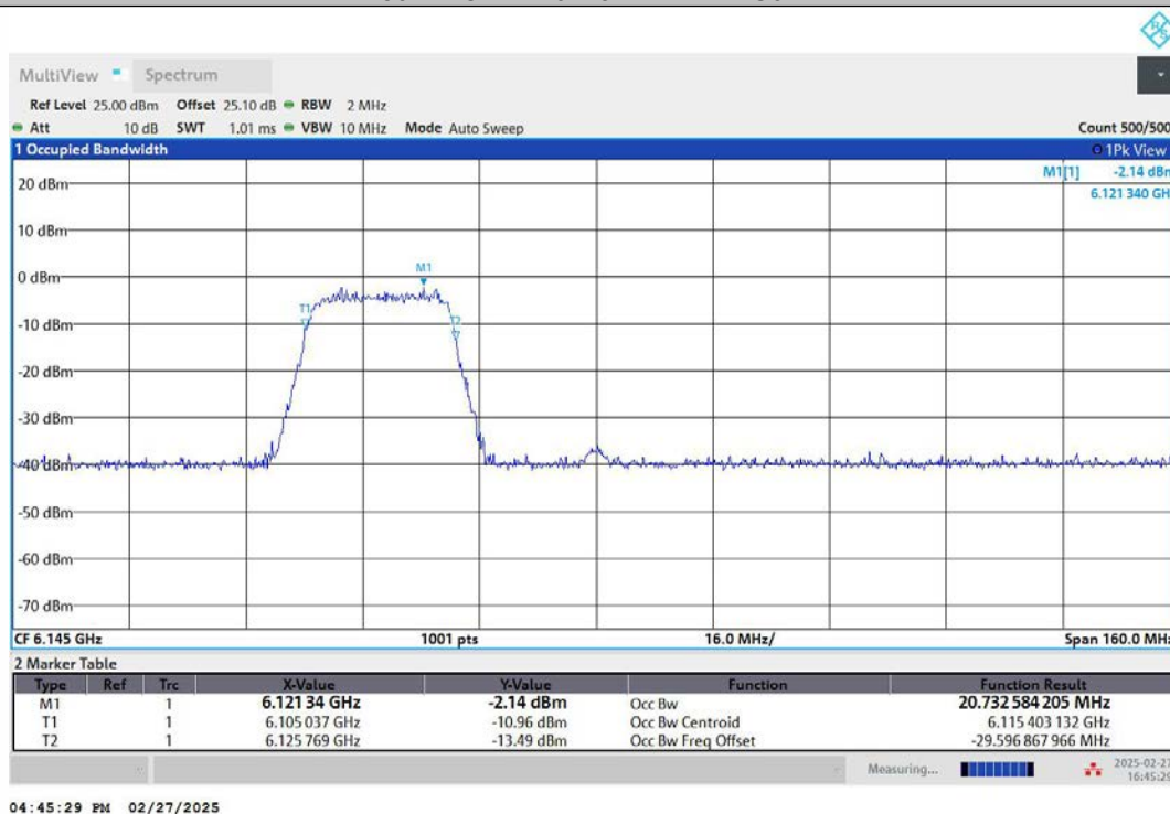
11AX80MIMO-Ant1-6145-484Tone-RU65-PASS
