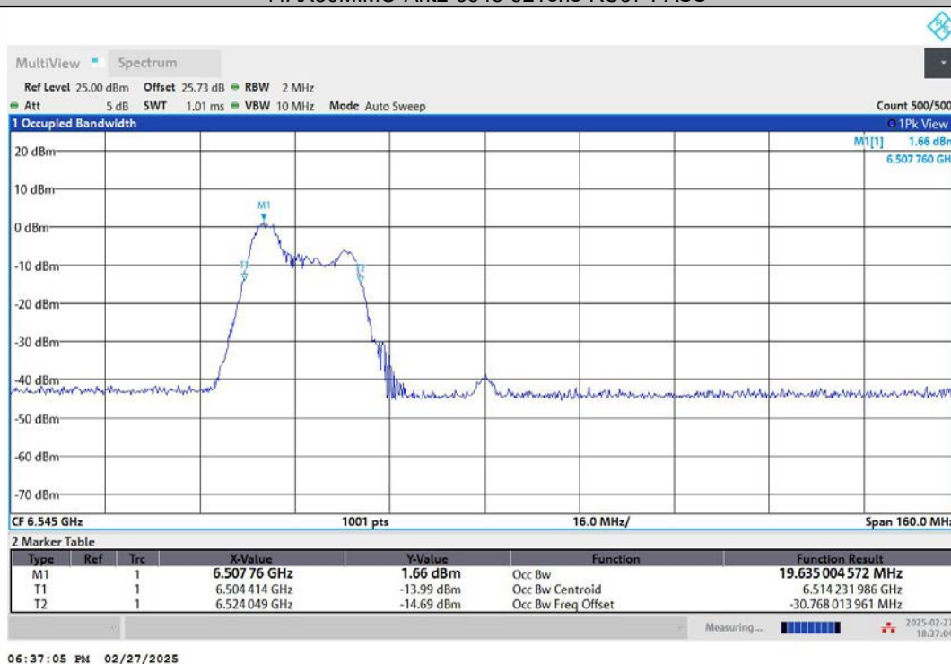
11AX80MIMO-Ant1-6545-106Tone-RU53-PASS
