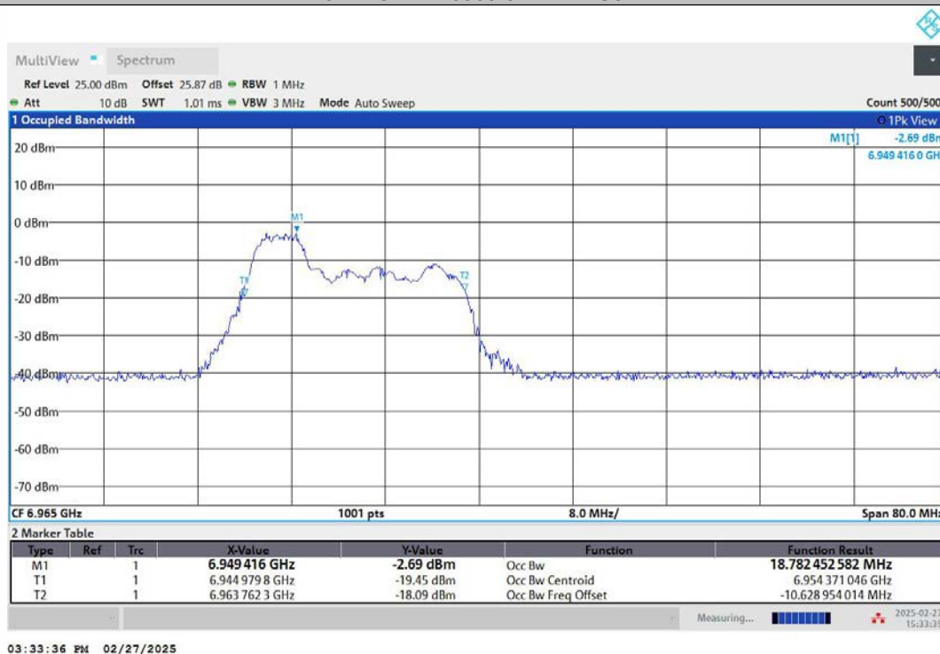
11AX40MIMO-Ant1-6965-106Tone-RU53-PASS
