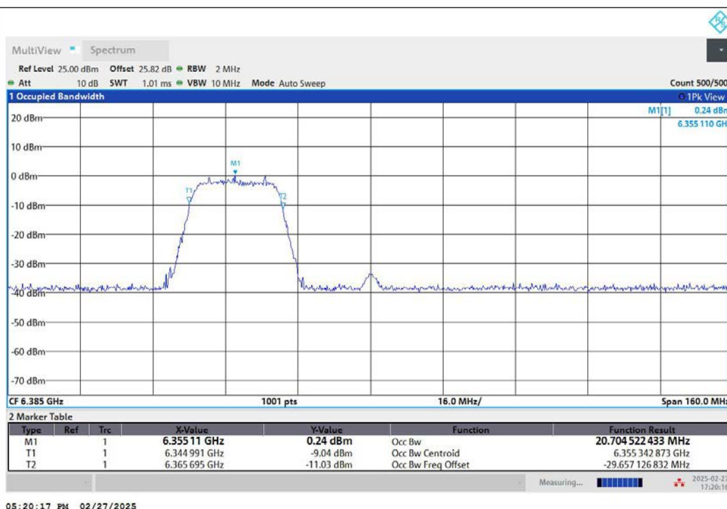
11AX80MIMO-Ant2-6385-242Tone-RU61-PASS
