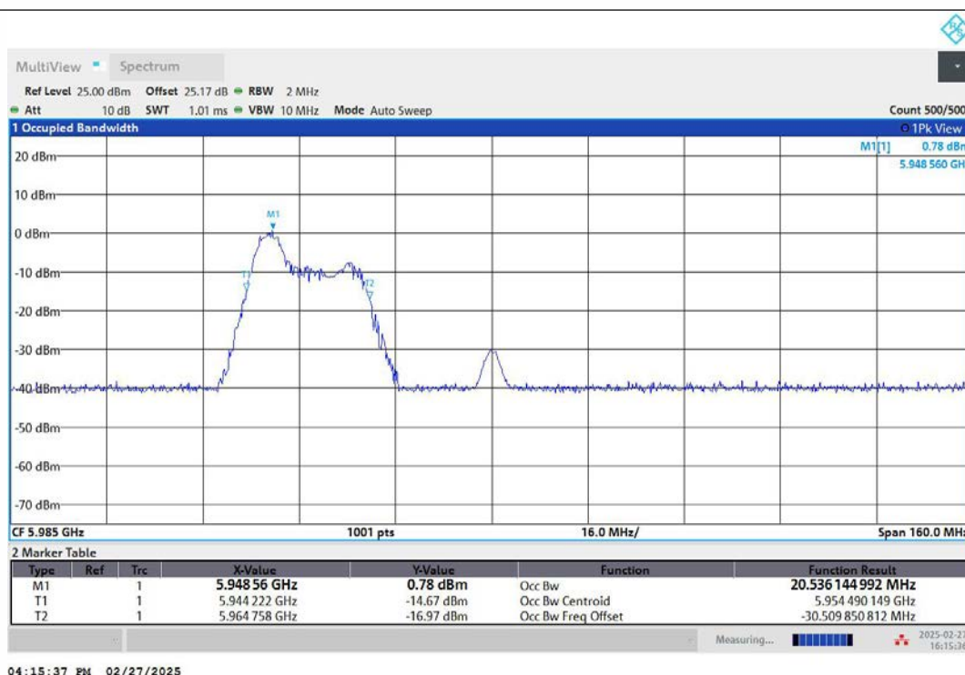
11AX80MIMO-Ant2-5985-52Tone-RU37-PASS
