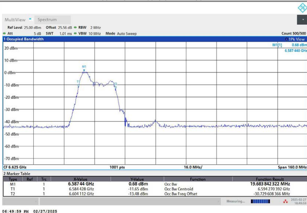
11AX80MIMO-Ant1-6625-106Tone-RU53-PASS
