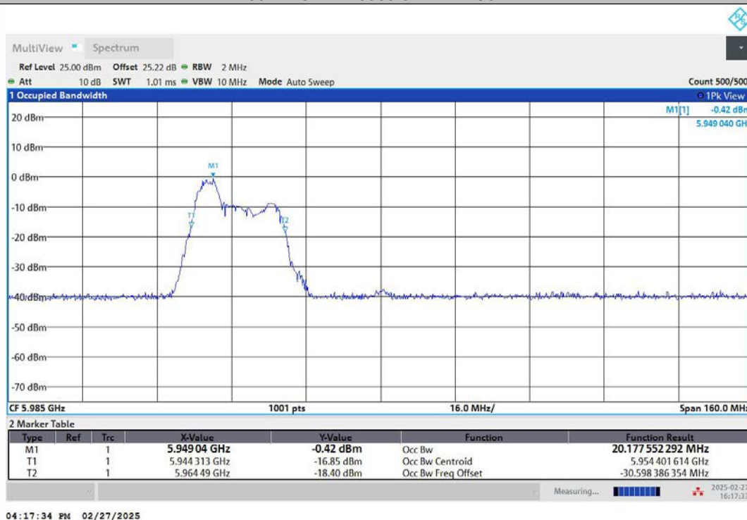
11AX80MIMO-Ant1-5985-106Tone-RU53-PASS
