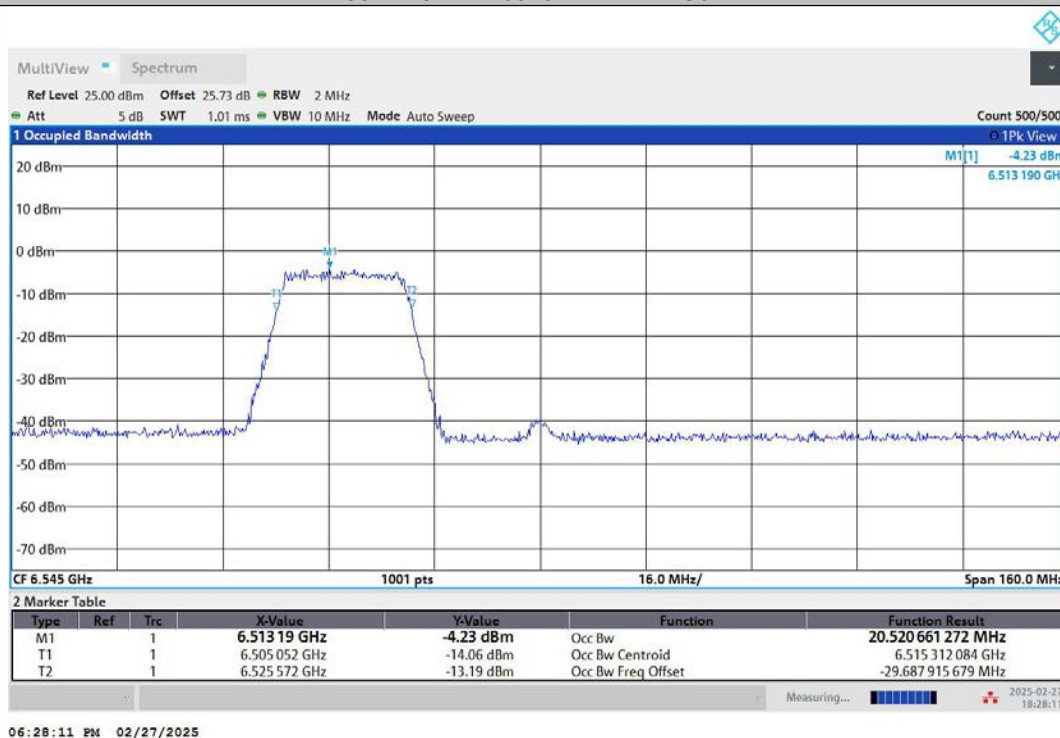
11AX80MIMO-Ant1-6545-484Tone-RU65-PASS
