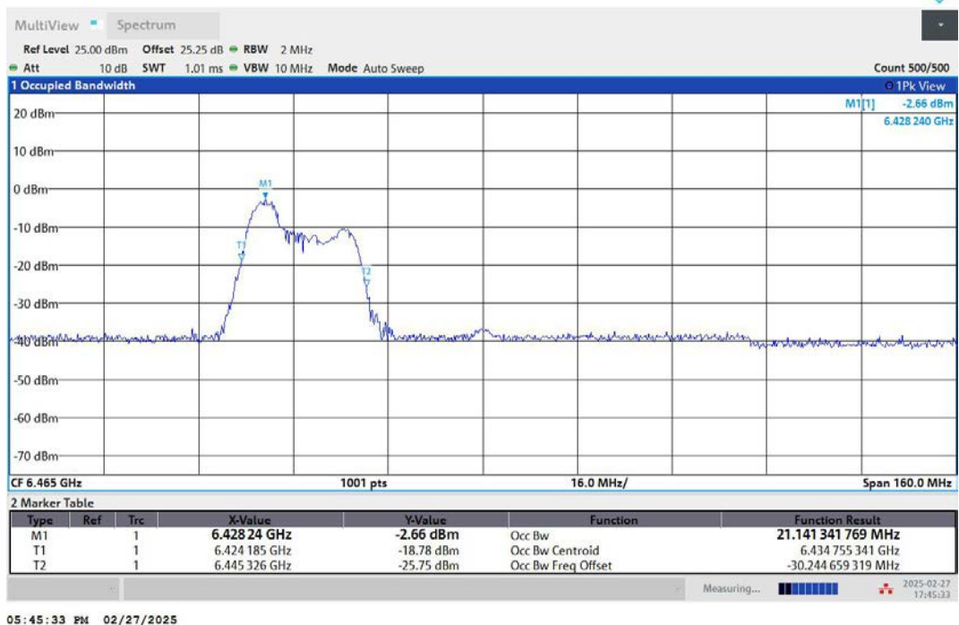
11AX80MIMO-Ant1-6465-106Tone-RU53-PASS
