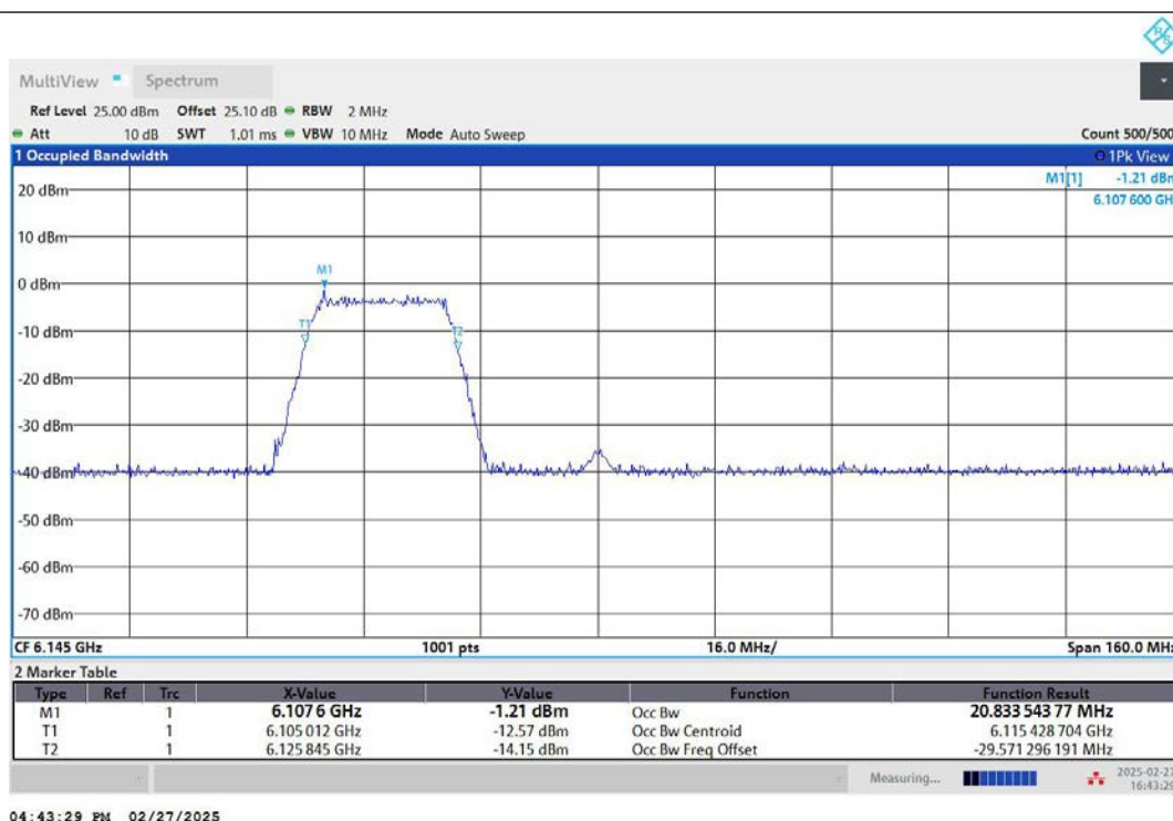
11AX80MIMO-Ant2-6145-242Tone-RU61-PASS
