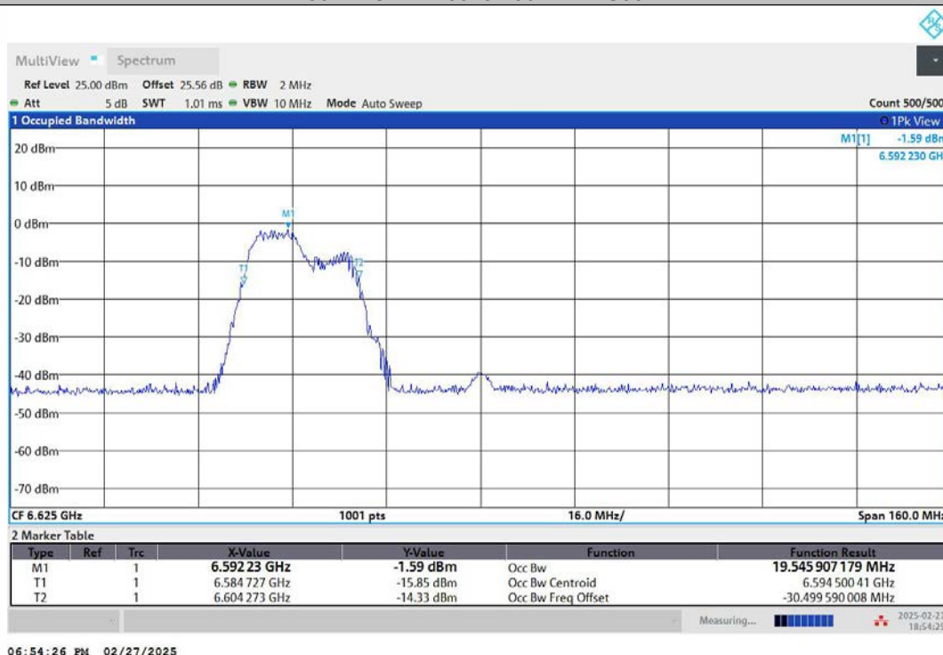
11AX80MIMO-Ant1-6625-242Tone-RU61-PASS
