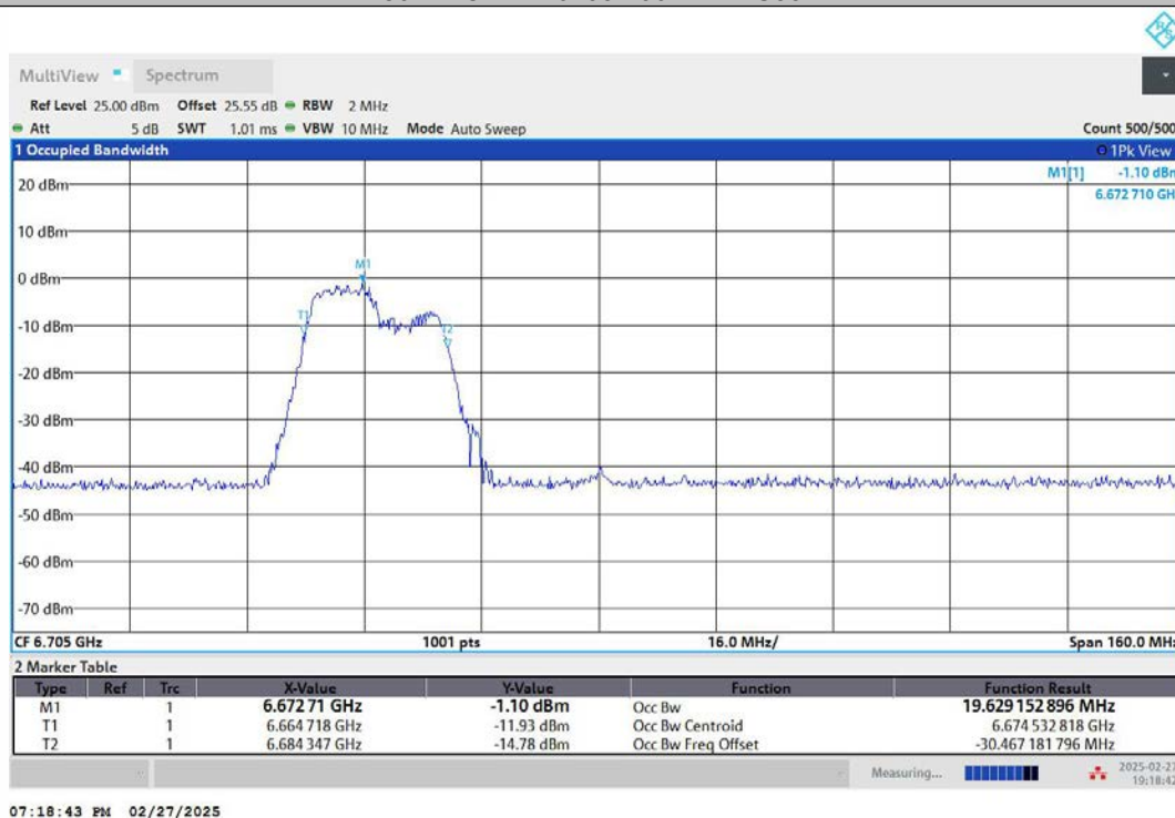
11AX80MIMO-Ant1-6705-242Tone-RU61-PASS
