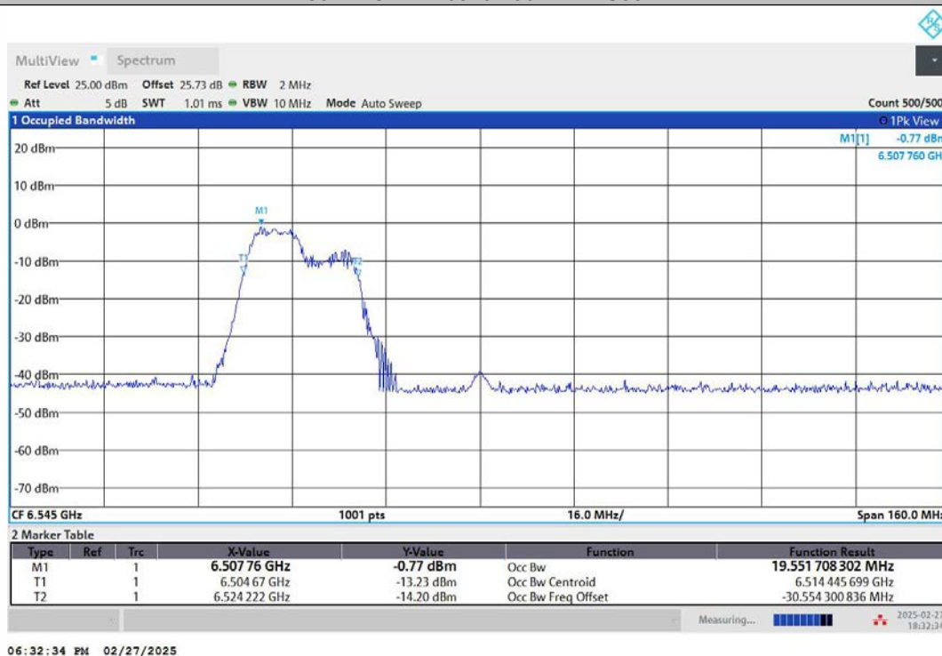
11AX80MIMO-Ant1-6545-242Tone-RU61-PASS
