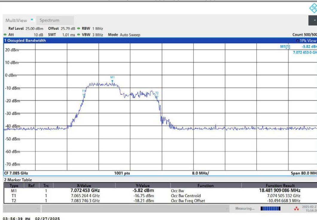
11AX40MIMO-Ant1-7085-242Tone-RU61-PASS
