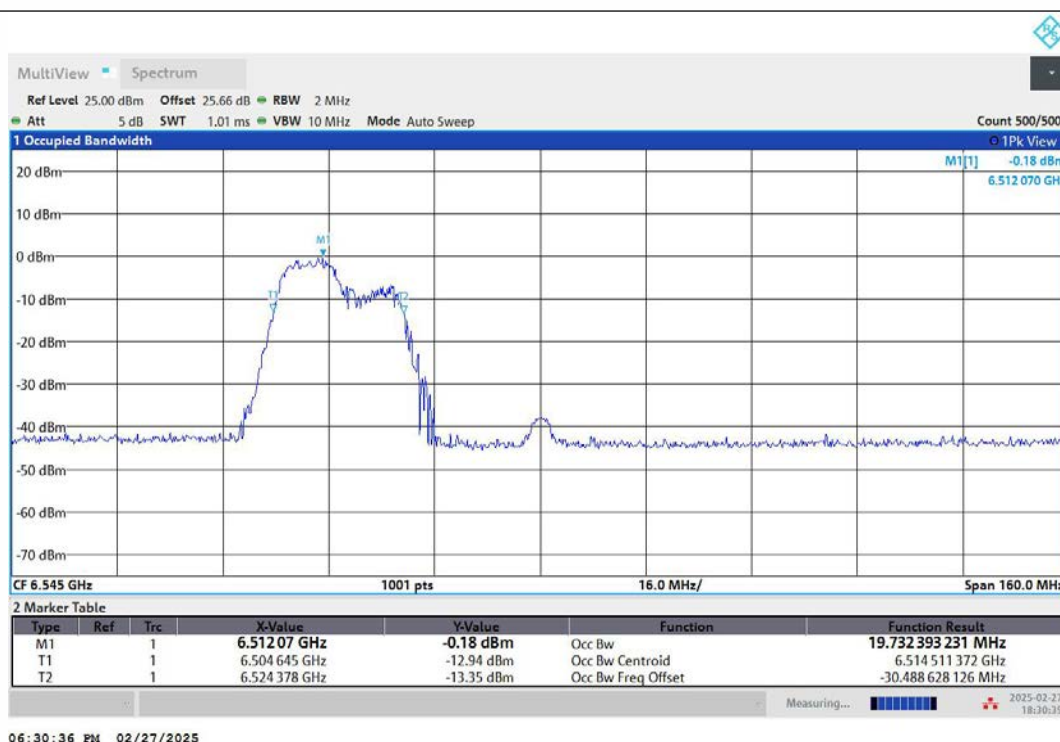
11AX80MIMO-Ant2-6545-106Tone-RU53-PASS
