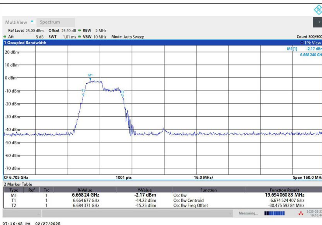
11AX80MIMO-Ant2-6705-106Tone-RU53-PASS
