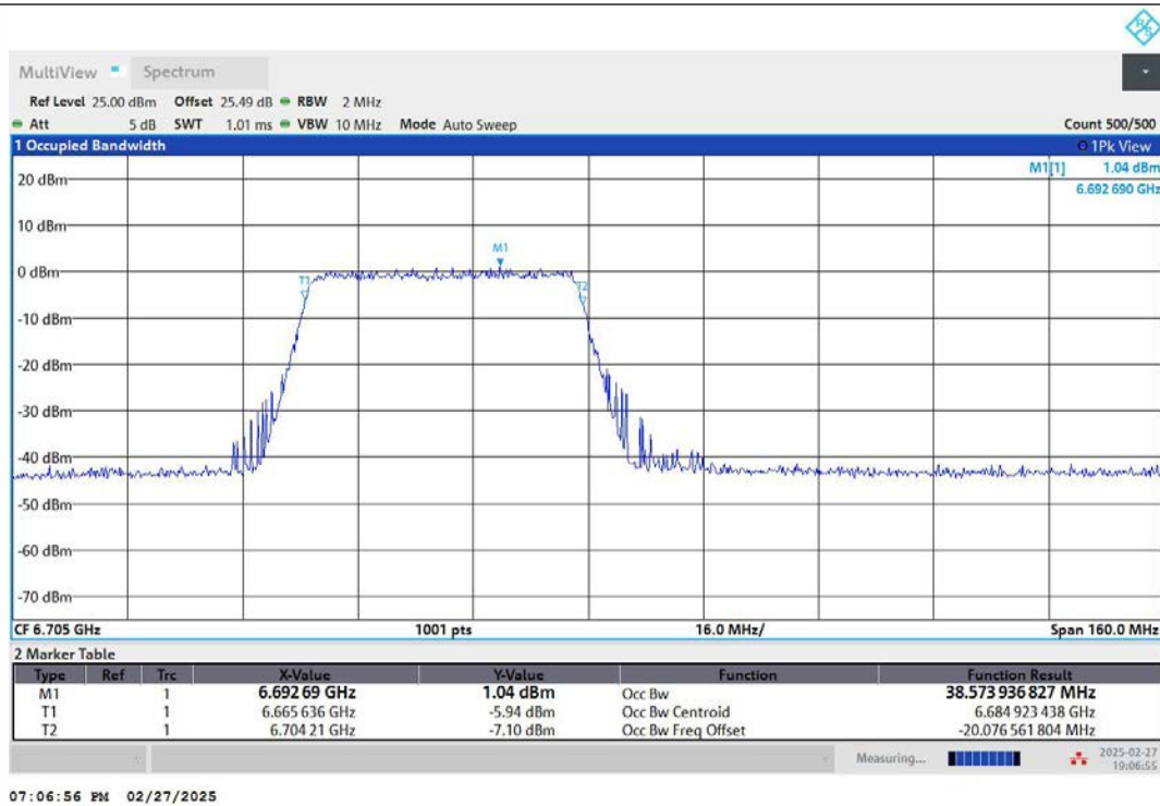
11AX80MIMO-Ant2-6705-484Tone-RU65-PASS
