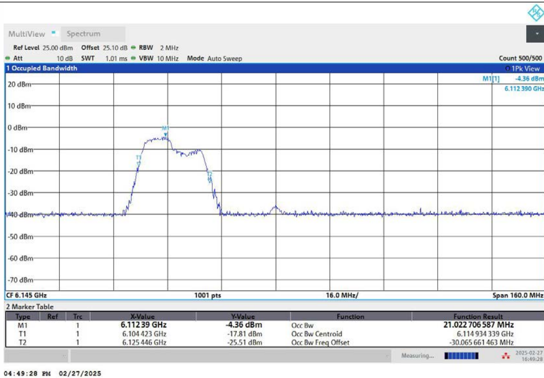
11AX80MIMO-Ant2-6145-106Tone-RU53-PASS
