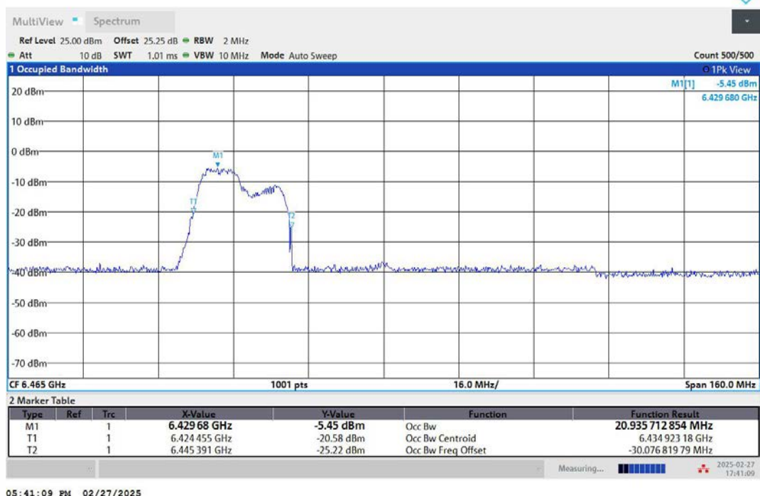
11AX80MIMO-Ant1-6465-242Tone-RU61-PASS
