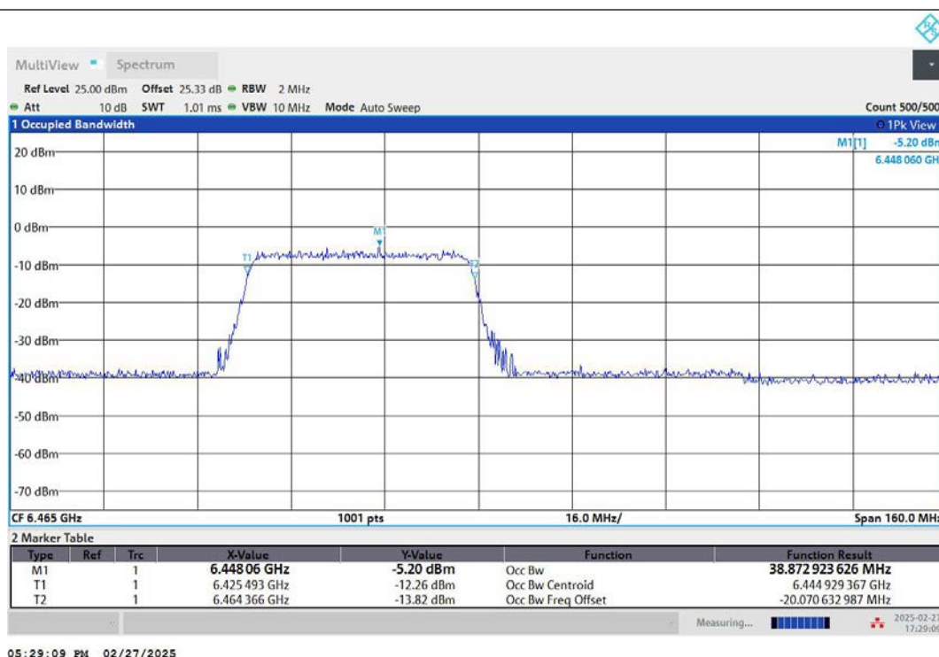
11AX80MIMO-Ant2-6465-484Tone-RU65-PASS
