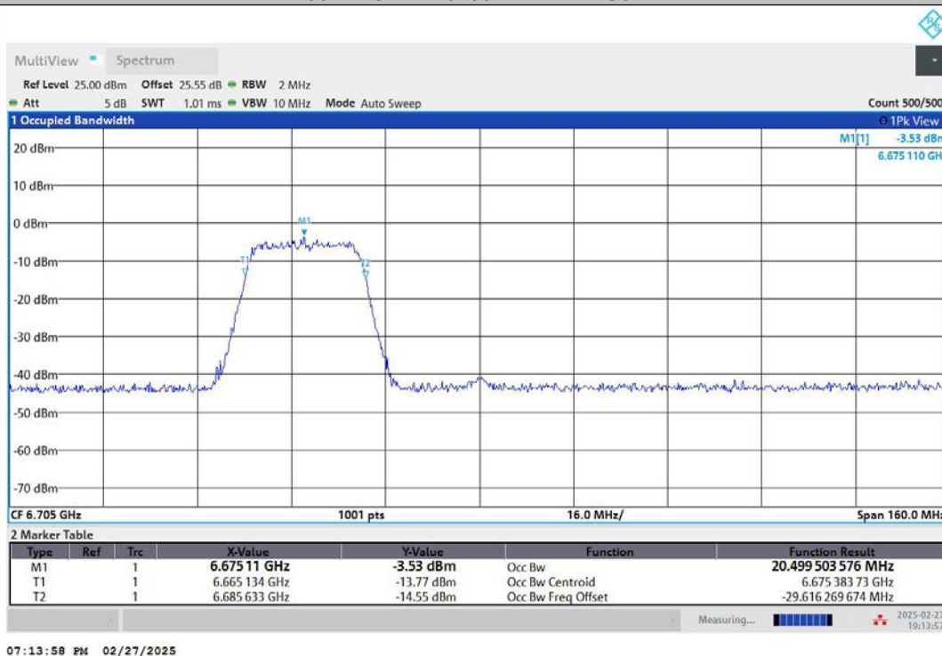
11AX80MIMO-Ant1-6705-484Tone-RU65-PASS
