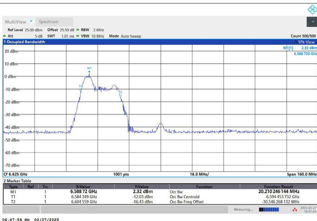
11AX80MIMO-Ant2-6625-52Tone-RU37-PASS
