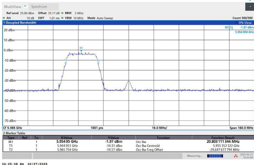
11AX80MIMO-Ant2-5985-242Tone-RU61-PASS
