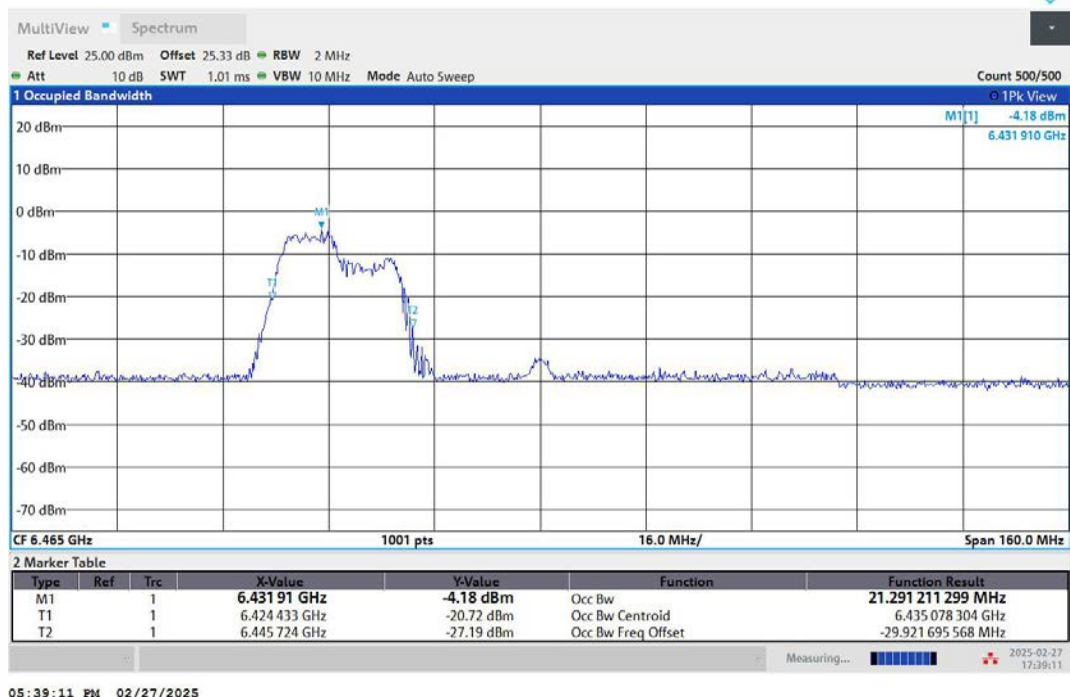
11AX80MIMO-Ant2-6465-106Tone-RU53-PASS
