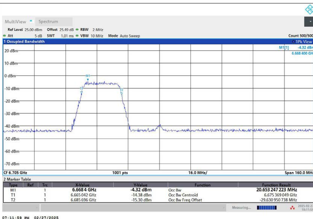
11AX80MIMO-Ant2-6705-242Tone-RU61-PASS
