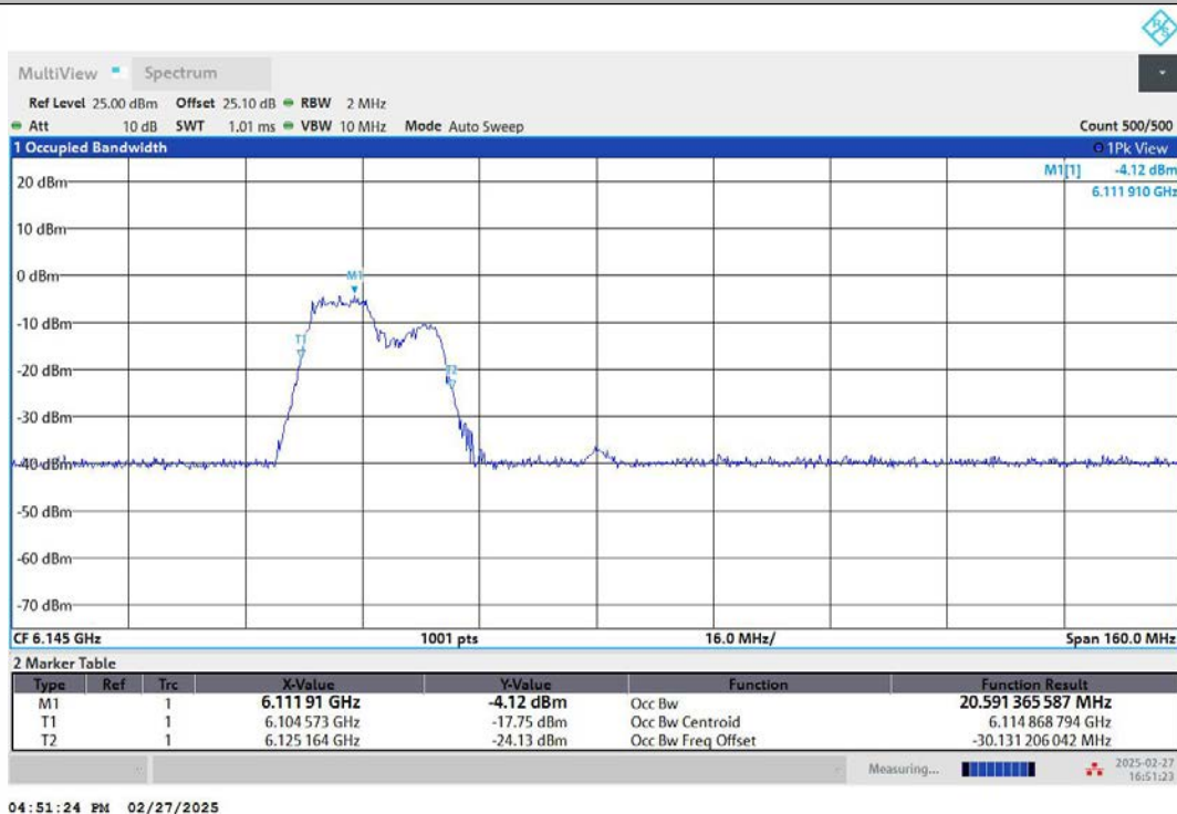
11AX80MIMO-Ant1-6145-242Tone-RU61-PASS
