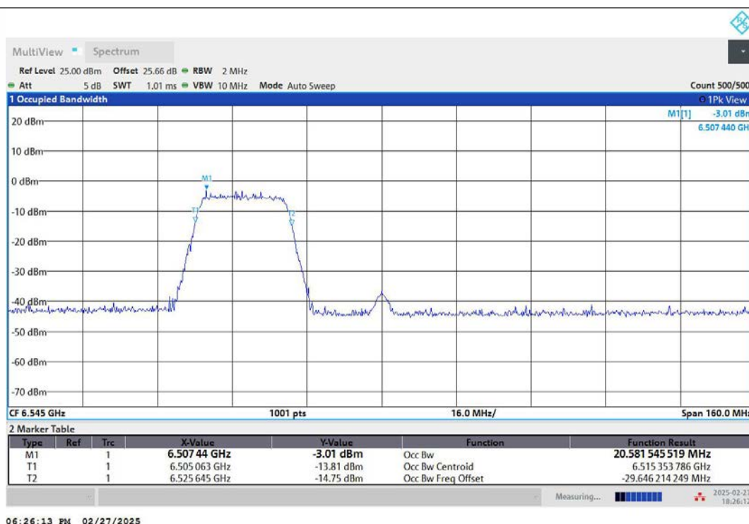
11AX80MIMO-Ant2-6545-242Tone-RU61-PASS
