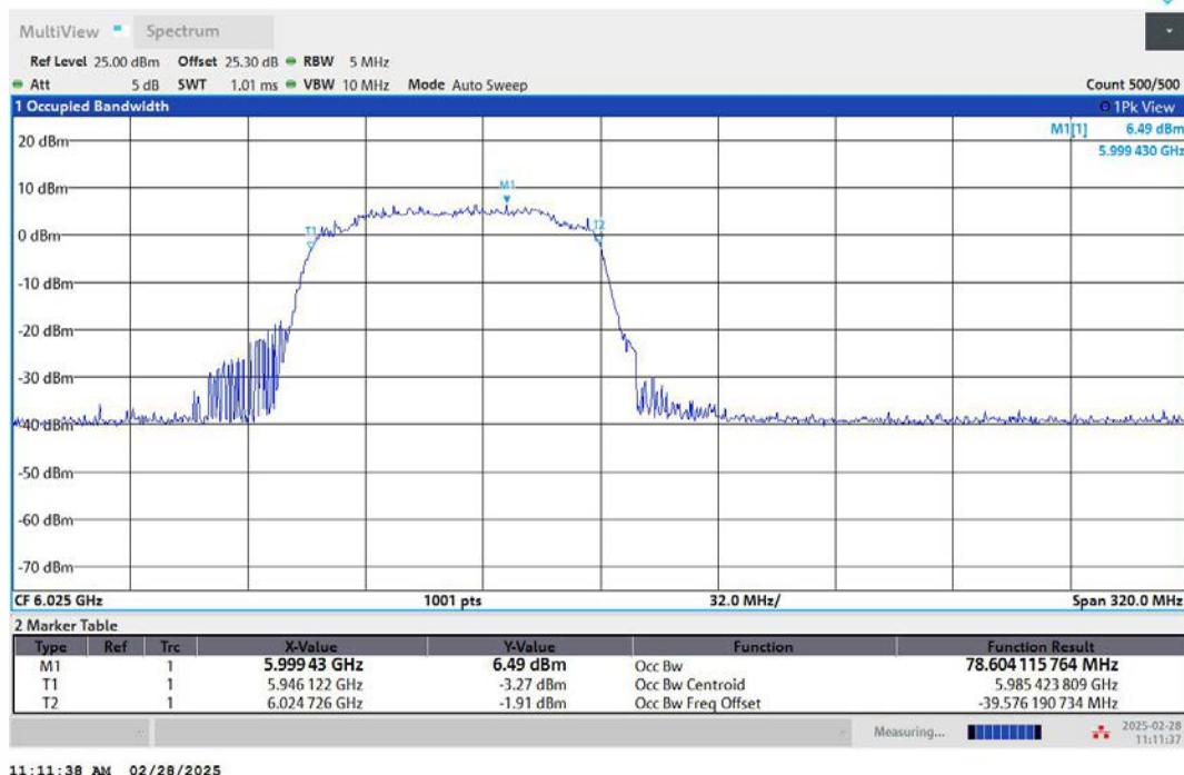
11AX160MIMO-Ant2-6025-996Tone-RU67-PASS
