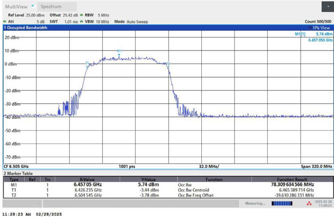
11AX160MIMO-Ant2-6505-996Tone-RU67-PASS
