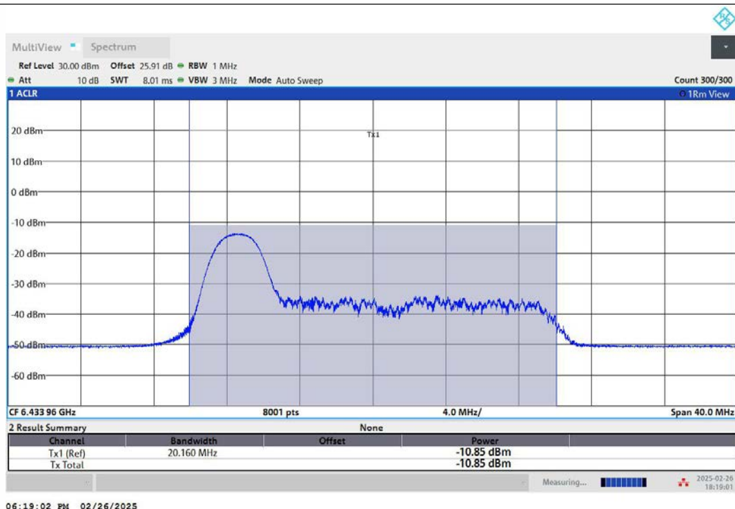
11AX20MIMO-Ant2-6435-26Tone-RU0-PASS
