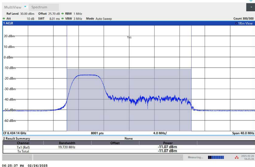
11AX20MIMO-Ant1-6435-106Tone-RU53-PASS
