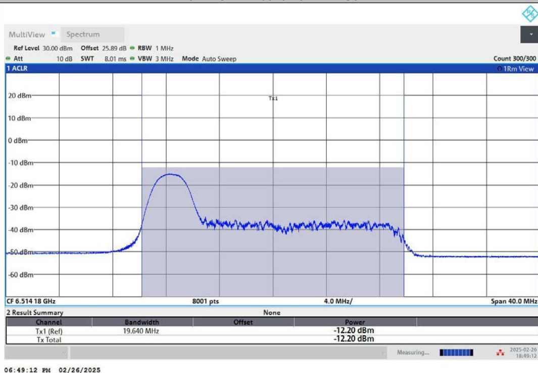
11AX20MIMO-Ant1-6515-52Tone-RU37-PASS
