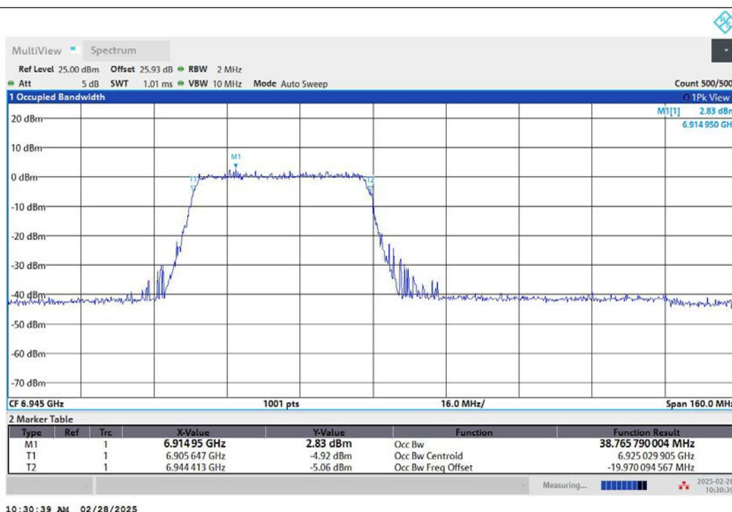
11AX80MIMO-Ant2-6945-484Tone-RU65-PASS
