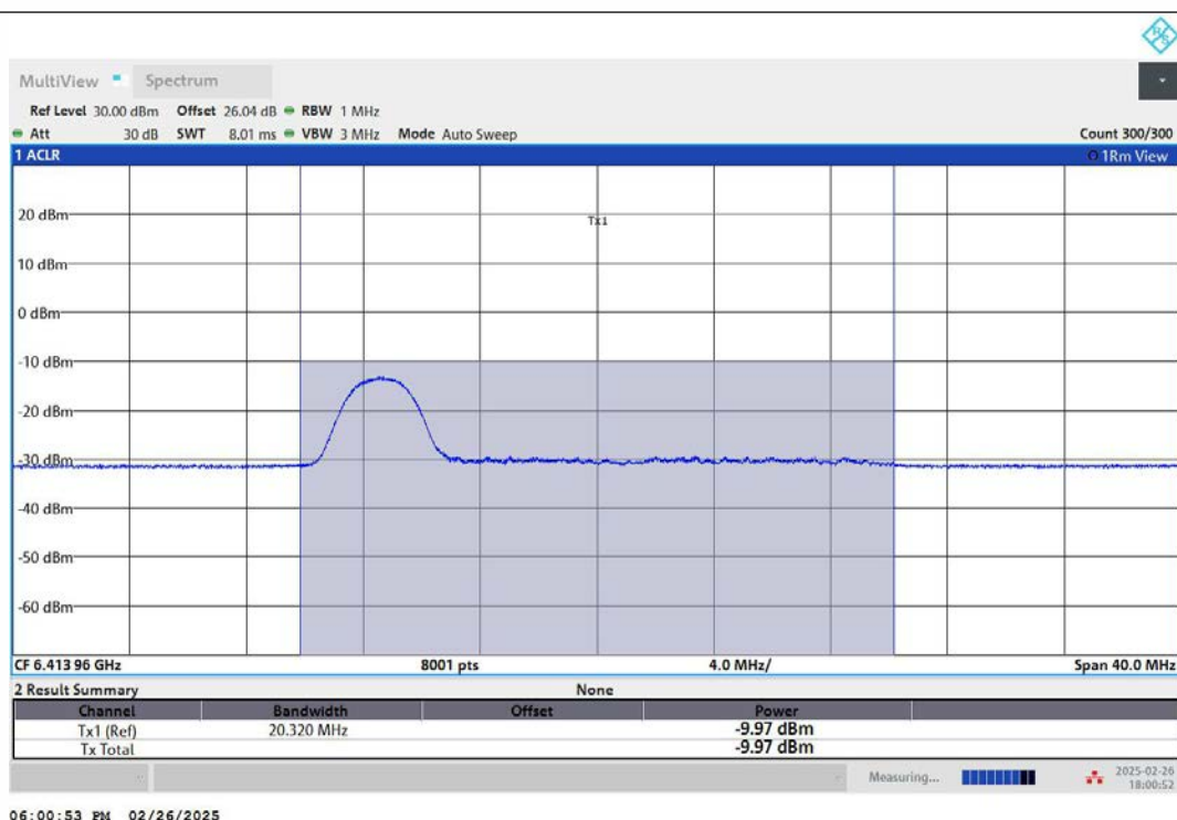
11AX20MIMO-Ant2-6415-26Tone-RU0-PASS
