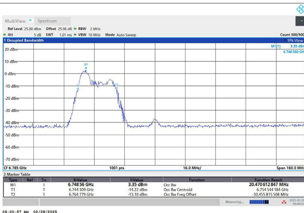
11AX80MIMO-Ant2-6785-52Tone-RU37-PASS
