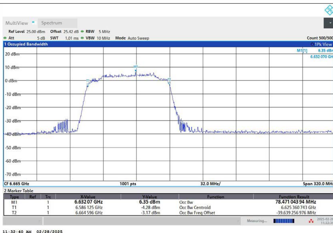
11AX160MIMO-Ant2-6665-996Tone-RU67-PASS
