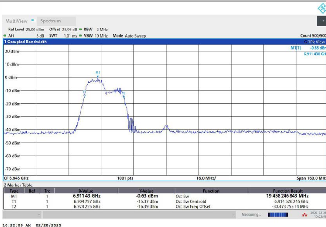
11AX80MIMO-Ant1-6945-242Tone-RU61-PASS
