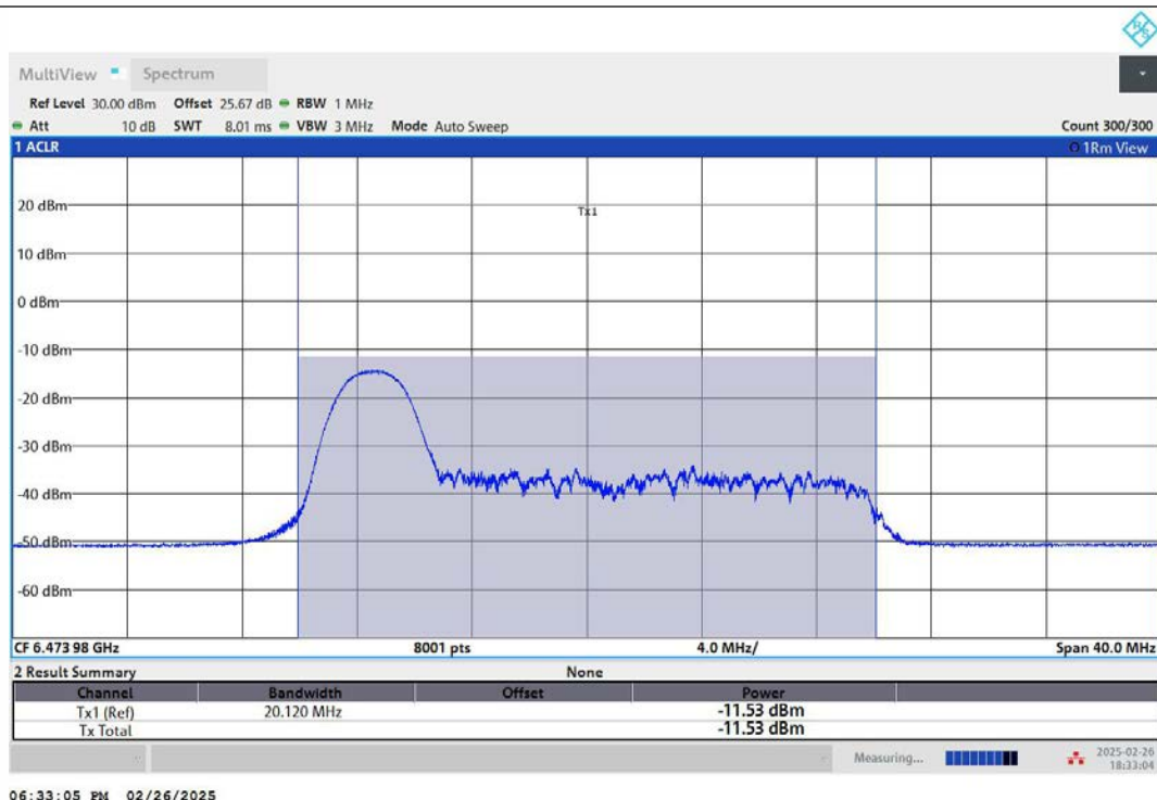
11AX20MIMO-Ant2-6475-26Tone-RU0-PASS
