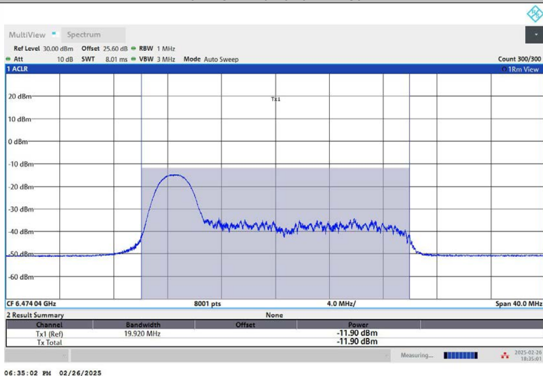
11AX20MIMO-Ant1-6475-52Tone-RU37-PASS
