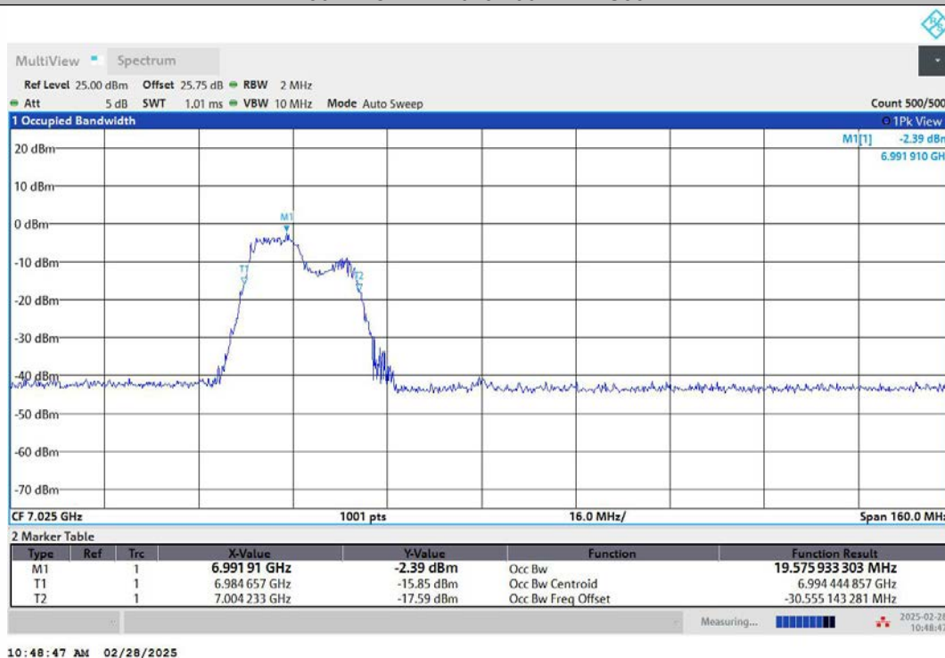
11AX80MIMO-Ant1-7025-242Tone-RU61-PASS
