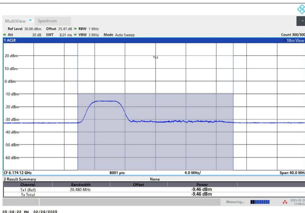
11AX20MIMO-Ant2-6175-52Tone-RU37-PASS
