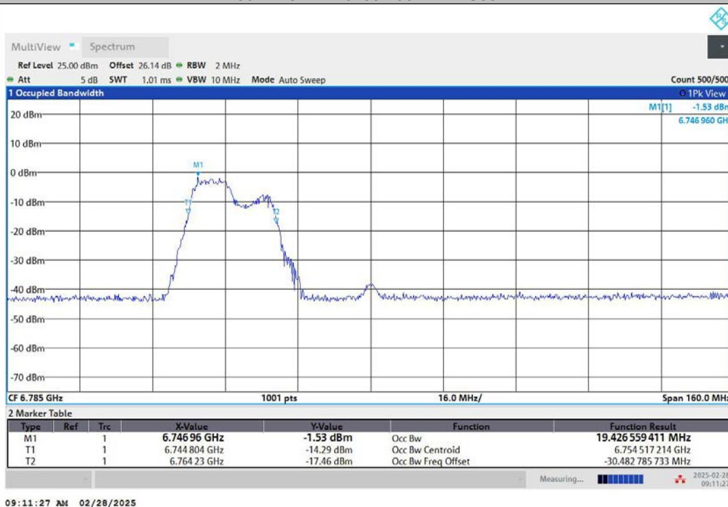
11AX80MIMO-Ant1-6785-242Tone-RU61-PASS
