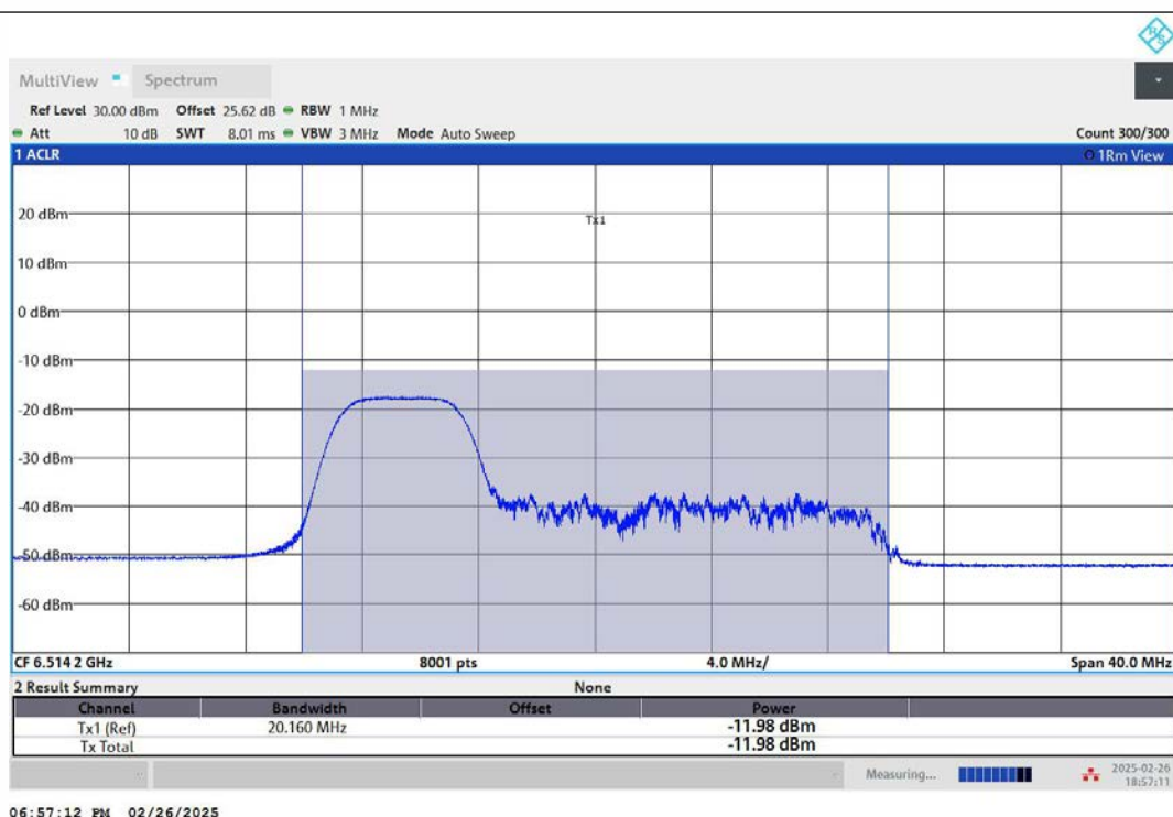
11AX20MIMO-Ant2-6515-52Tone-RU37-PASS
