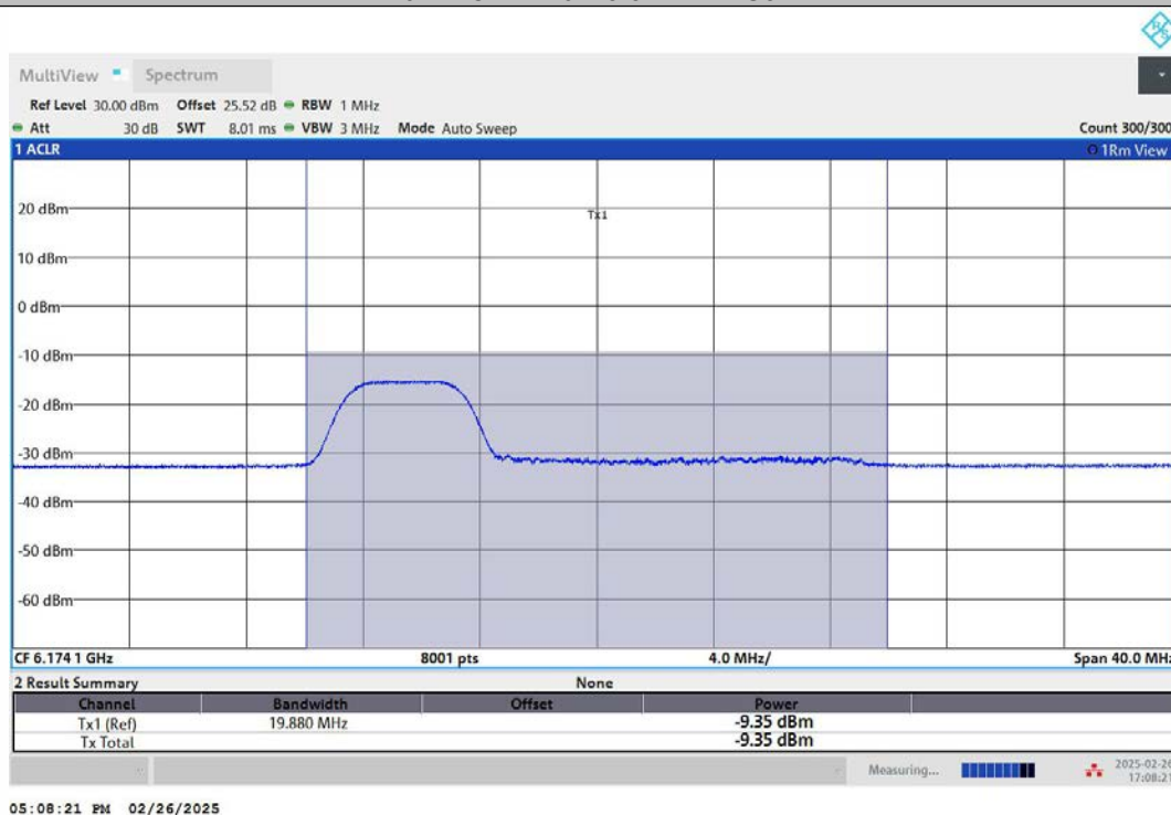
11AX20MIMO-Ant1-6175-106Tone-RU53-PASS
