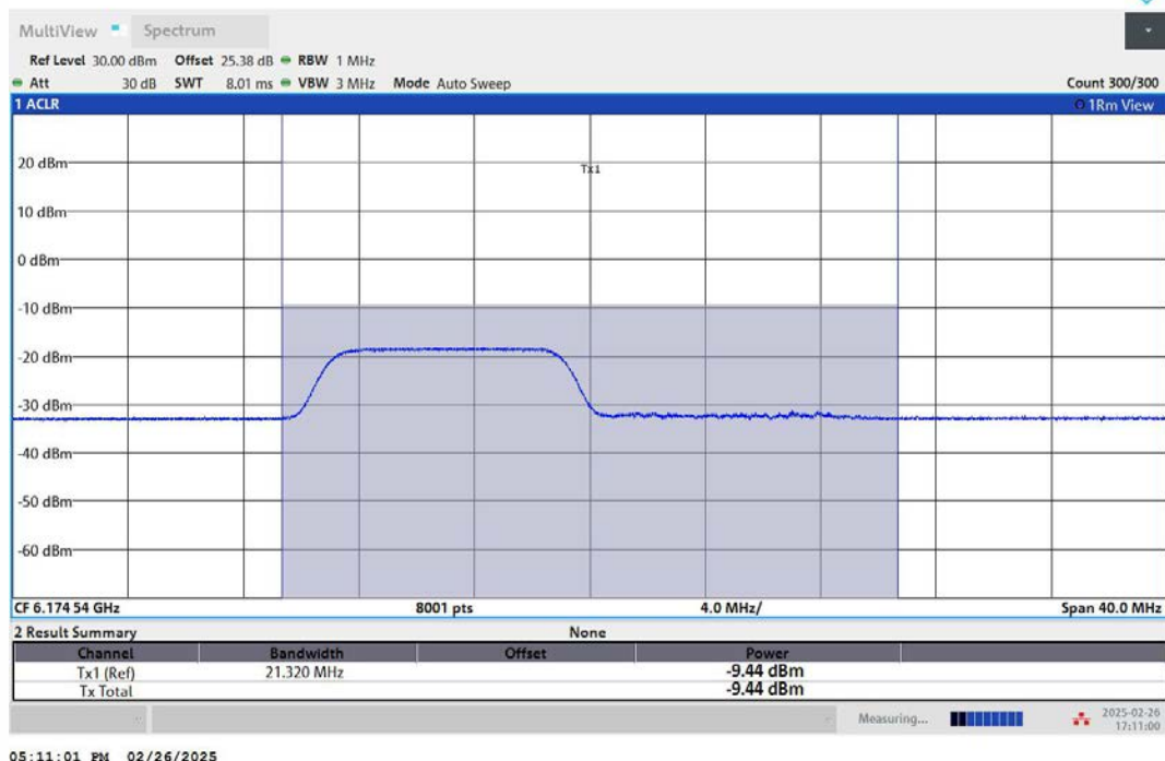
11AX20MIMO-Ant2-6175-106Tone-RU53-PASS
