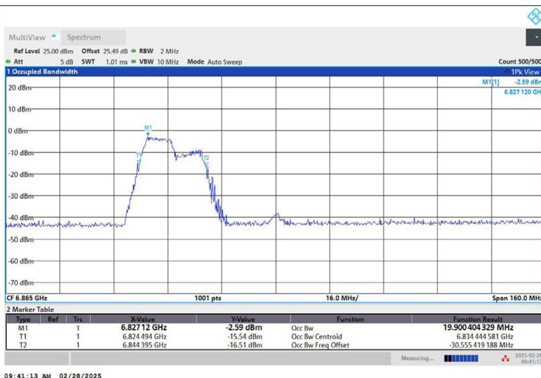
11AX80MIMO-Ant2-6865-106Tone-RU53-PASS
