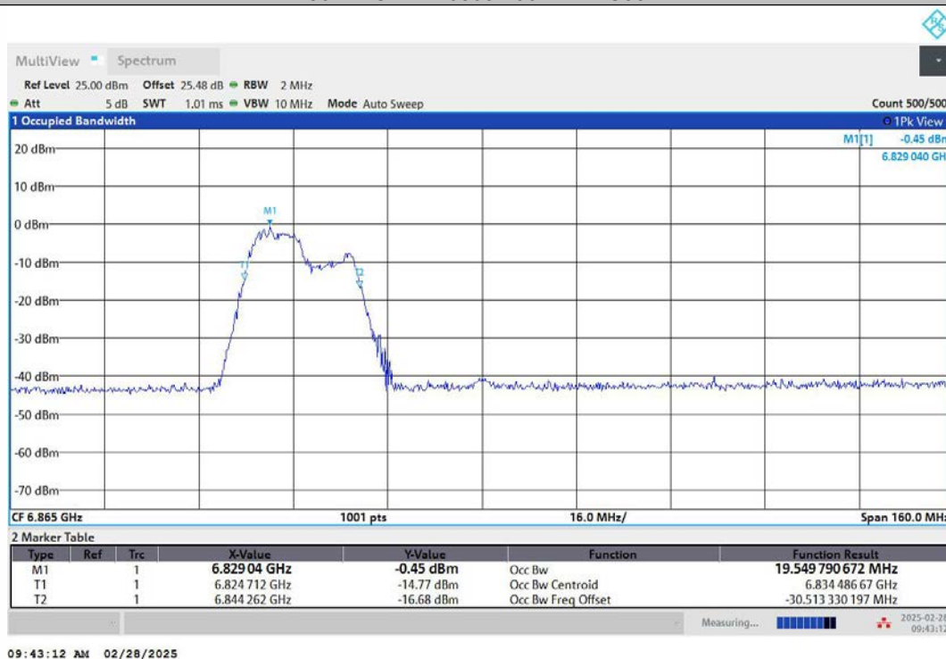
11AX80MIMO-Ant1-6865-242Tone-RU61-PASS
