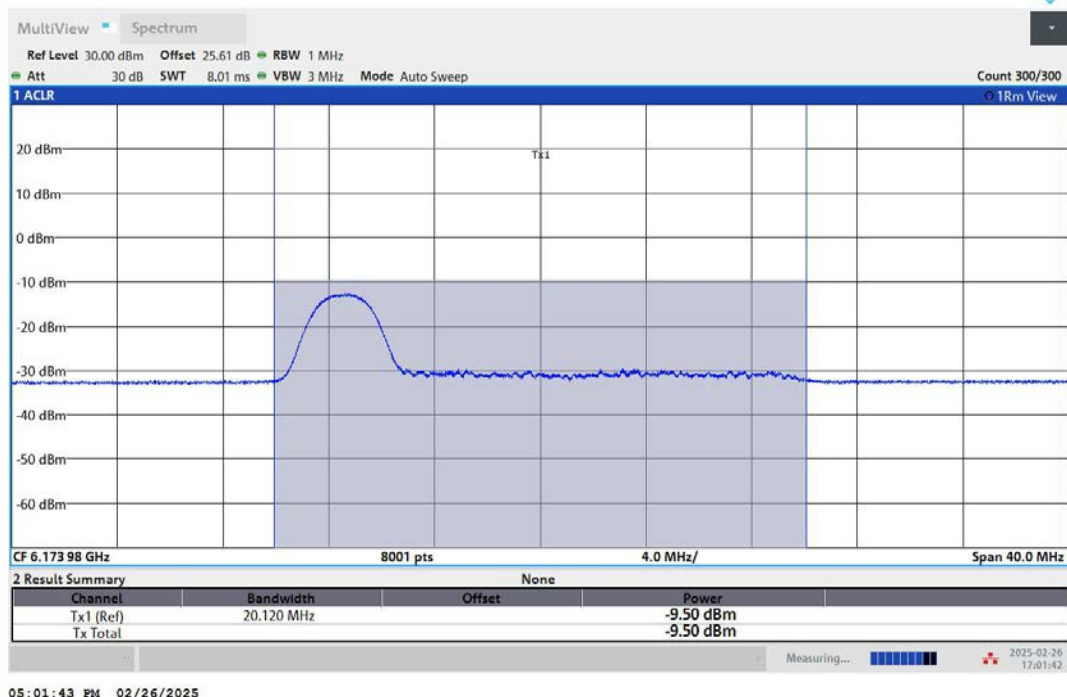
11AX20MIMO-Ant2-6175-26Tone-RU0-PASS
