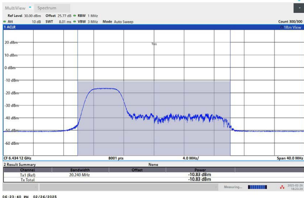
11AX20MIMO-Ant2-6435-52Tone-RU37-PASS
