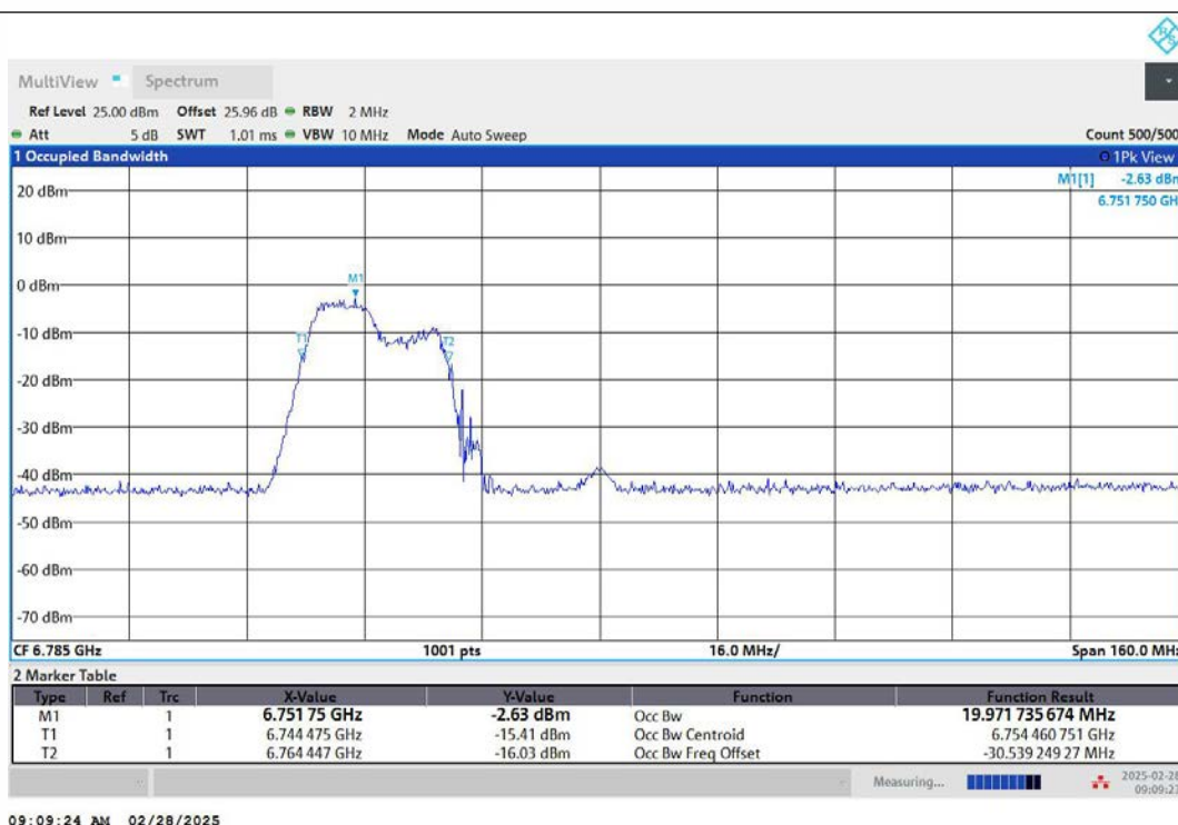
11AX80MIMO-Ant2-6785-106Tone-RU53-PASS
