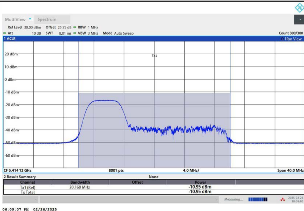
11AX20MIMO-Ant1-6415-106Tone-RU53-PASS
