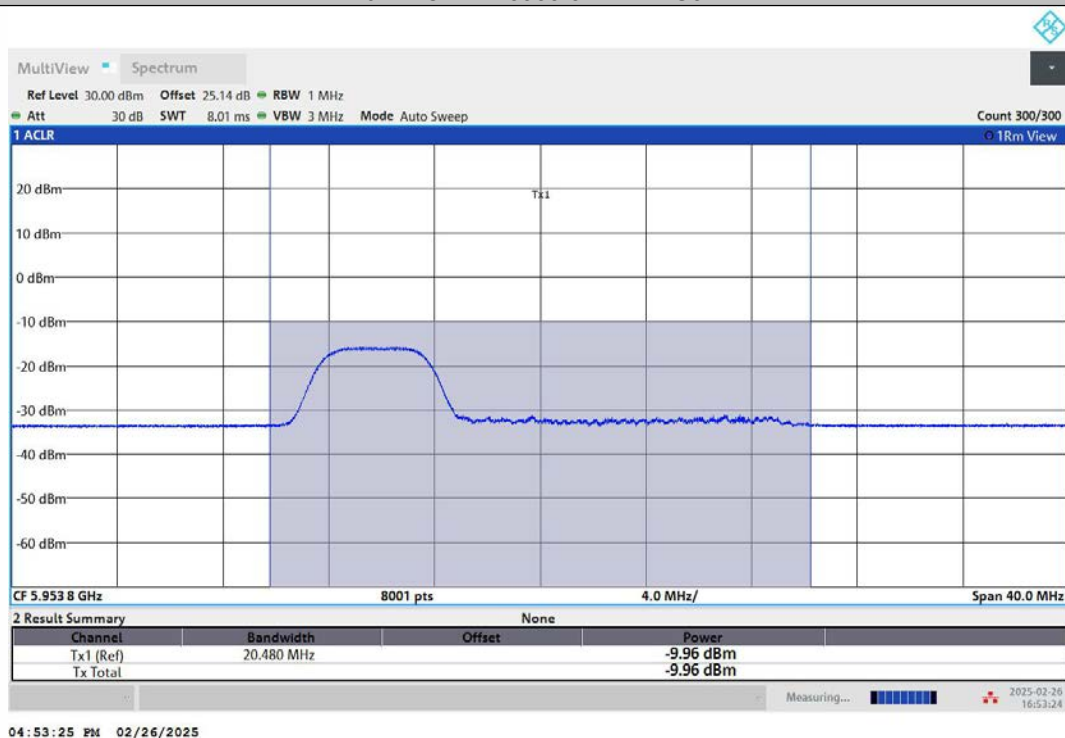
11AX20MIMO-Ant1-5955-106Tone-RU53-PASS
