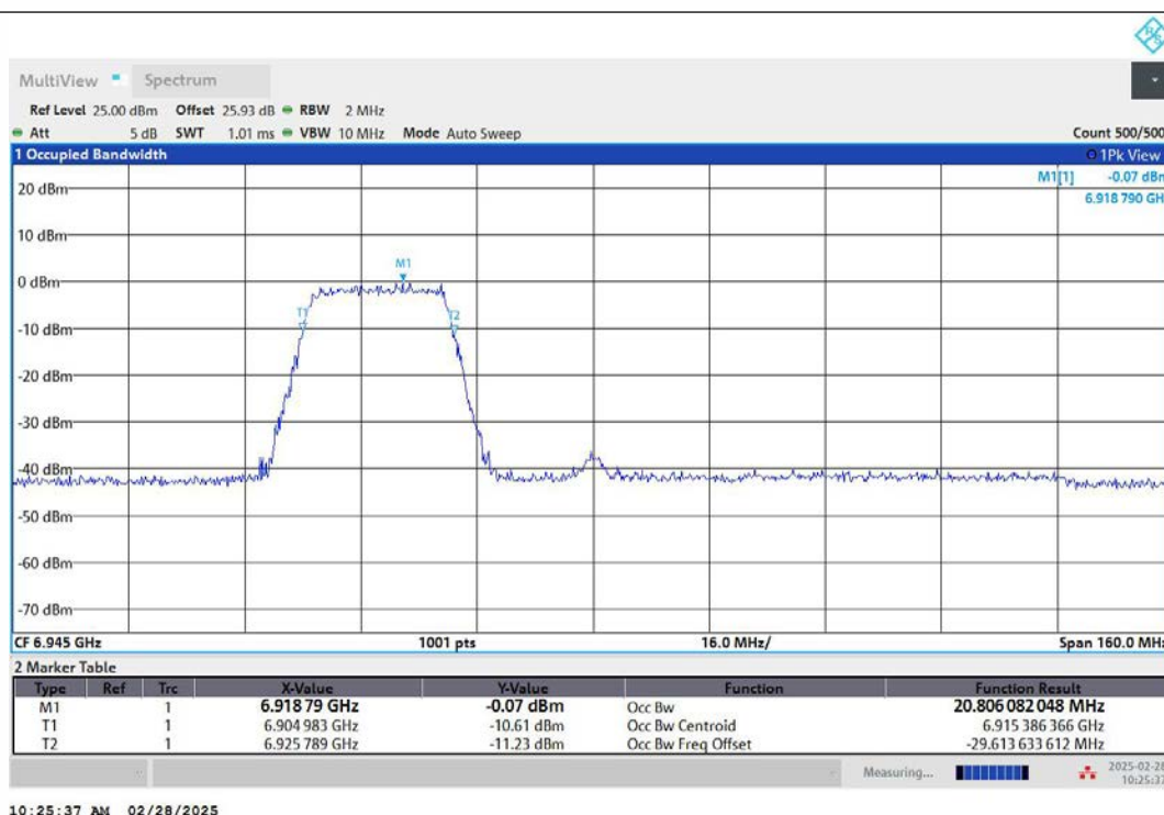
11AX80MIMO-Ant2-6945-242Tone-RU61-PASS
