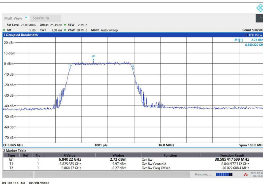
11AX80MIMO-Ant2-6865-484Tone-RU65-PASS
