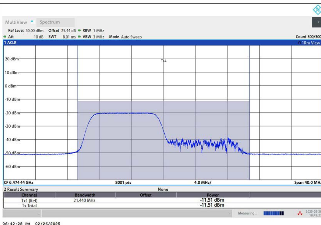
11AX20MIMO-Ant2-6475-106Tone-RU53-PASS
