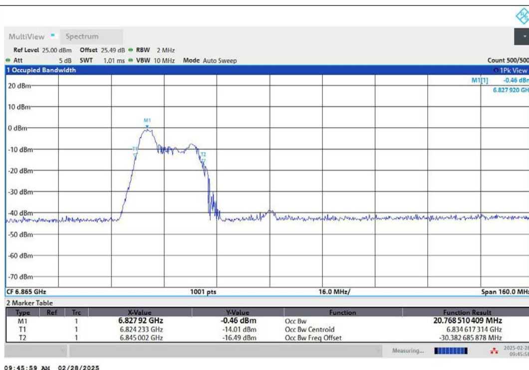
11AX80MIMO-Ant2-6865-52Tone-RU37-PASS
