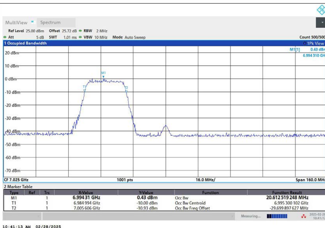
11AX80MIMO-Ant2-7025-242Tone-RU61-PASS
