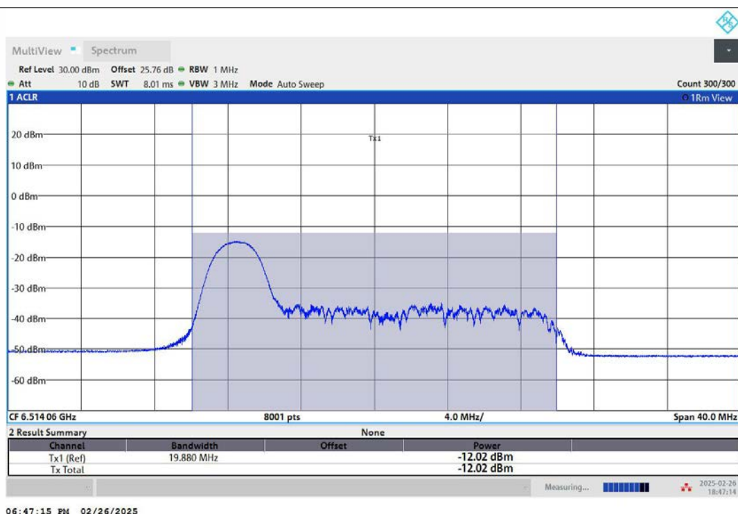
11AX20MIMO-Ant2-6515-26Tone-RU0-PASS
