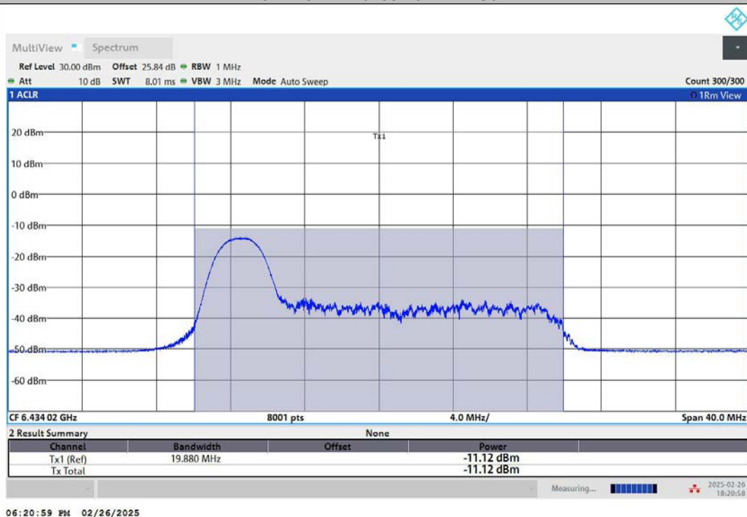
11AX20MIMO-Ant1-6435-52Tone-RU37-PASS
