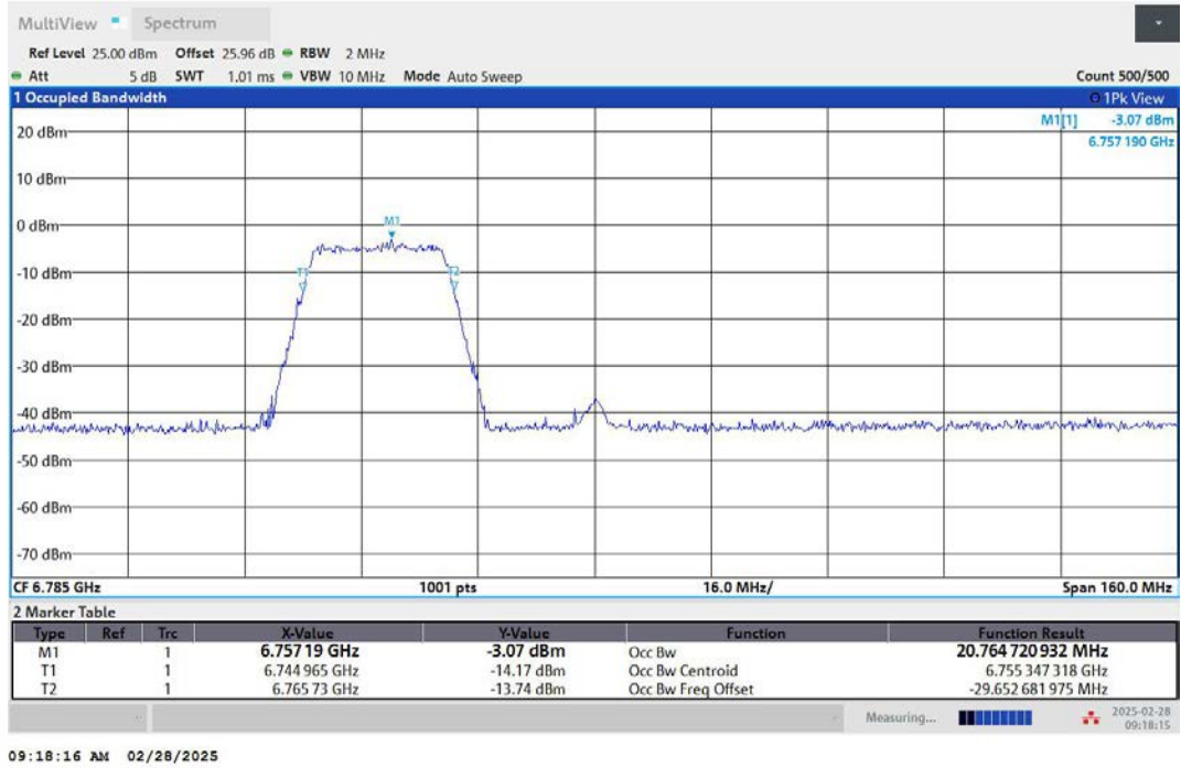
11AX80MIMO-Ant2-6785-242Tone-RU61-PASS
