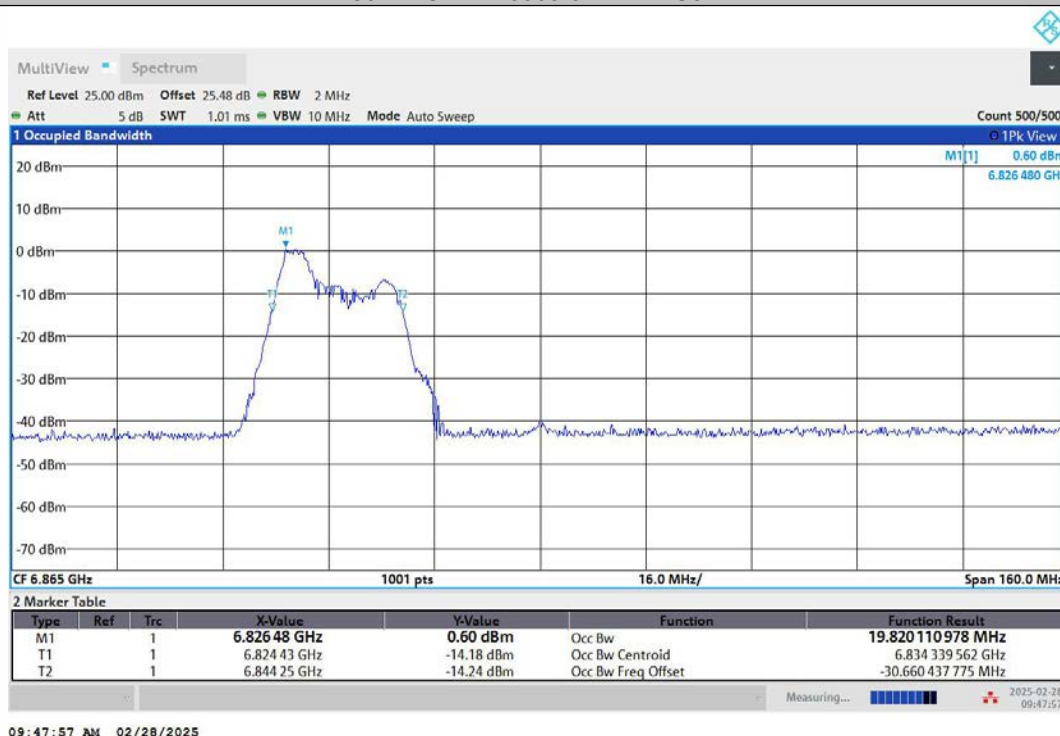
11AX80MIMO-Ant1-6865-106Tone-RU53-PASS
