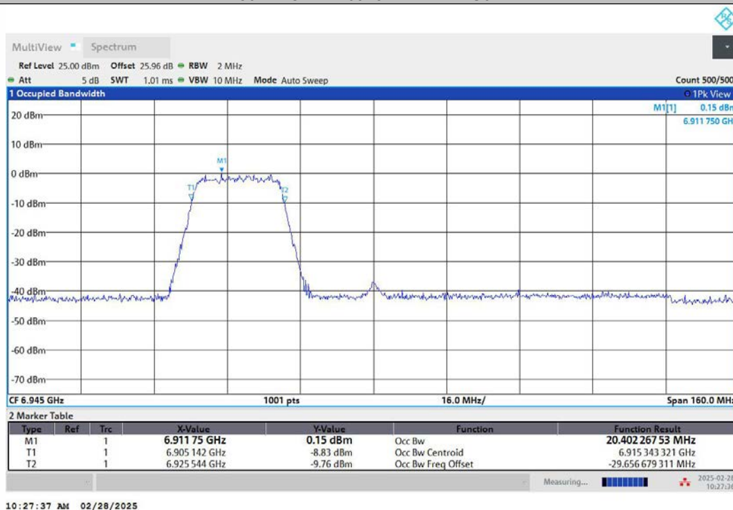
11AX80MIMO-Ant1-6945-484Tone-RU65-PASS
