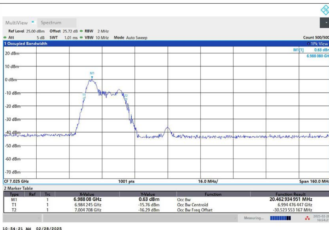
11AX80MIMO-Ant2-7025-52Tone-RU37-PASS
