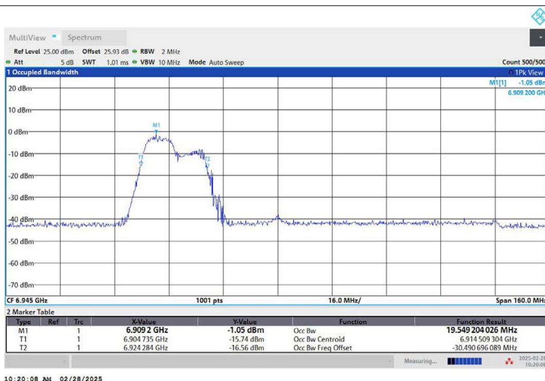
11AX80MIMO-Ant2-6945-106Tone-RU53-PASS
