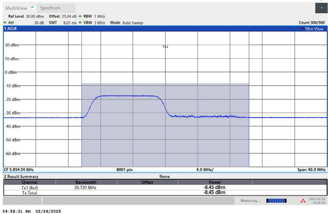
11AX20MIMO-Ant2-5955-106Tone-RU53-PASS
