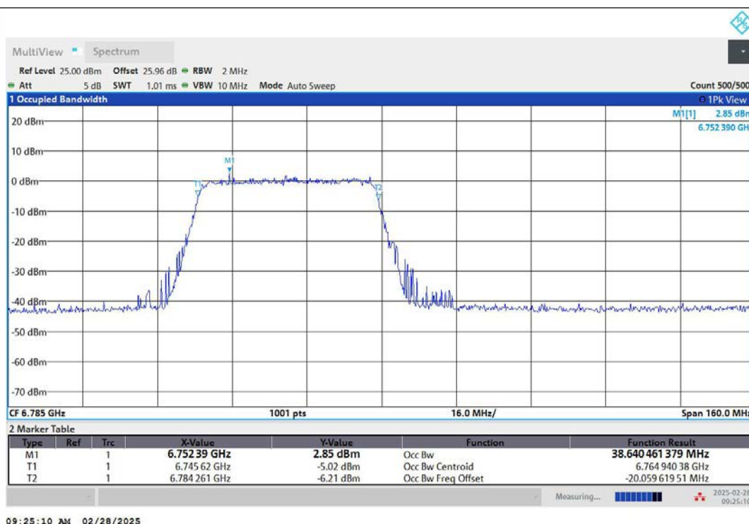
11AX80MIMO-Ant2-6785-484Tone-RU65-PASS
