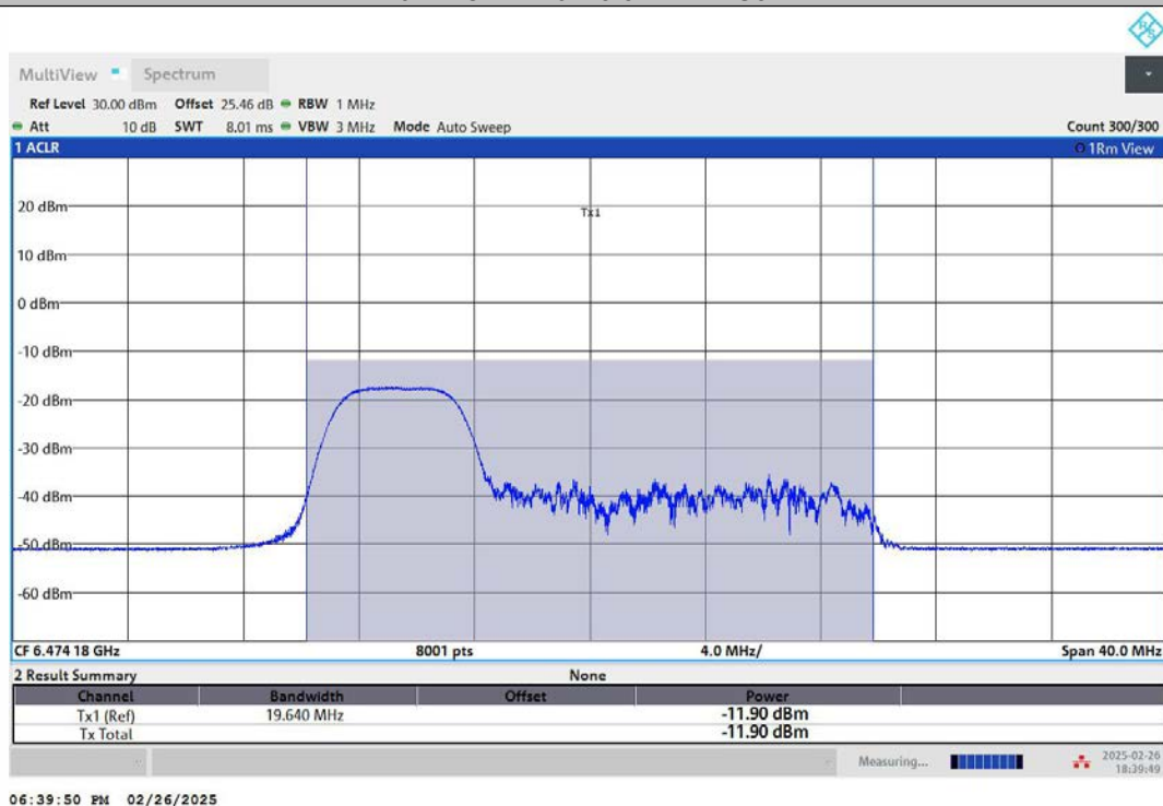
11AX20MIMO-Ant1-6475-106Tone-RU53-PASS
