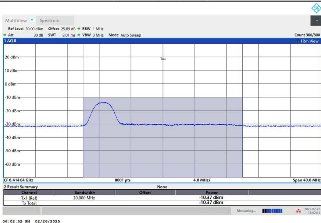
11AX20MIMO-Ant1-6415-52Tone-RU37-PASS
