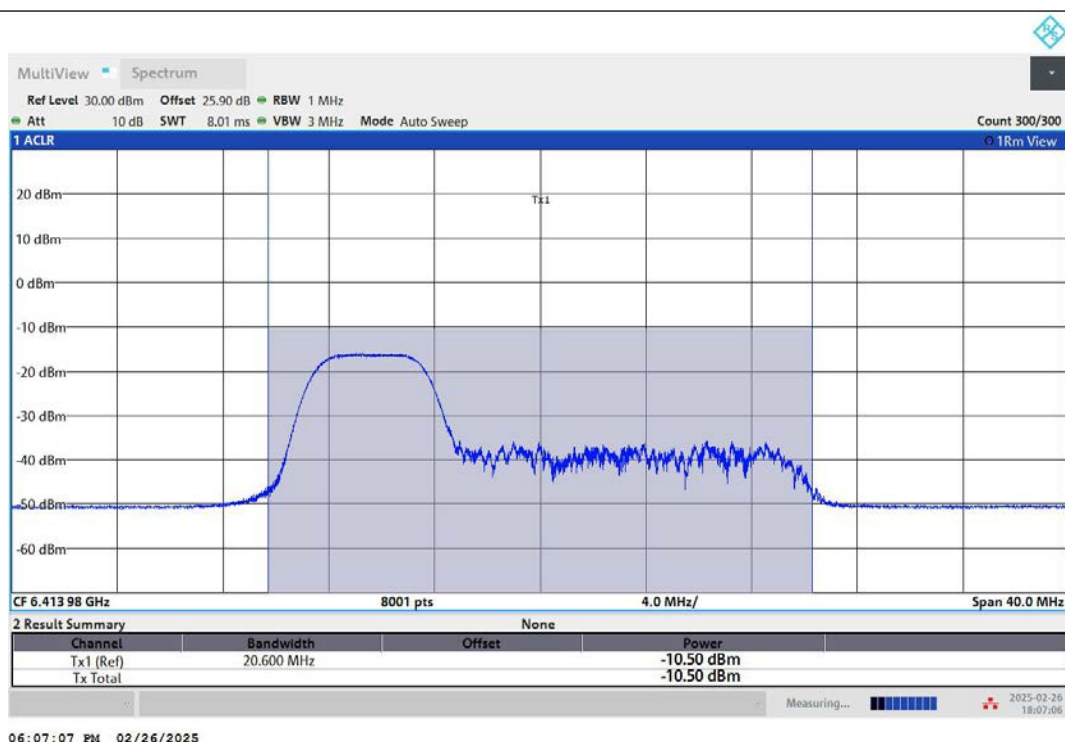
11AX20MIMO-Ant2-6415-52Tone-RU37-PASS
