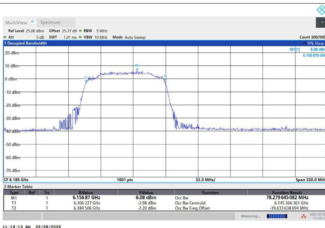
11AX160MIMO-Ant2-6185-996Tone-RU67-PASS
