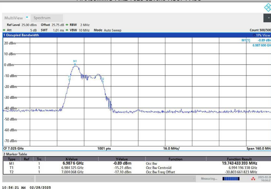
11AX80MIMO-Ant1-7025-106Tone-RU53-PASS
