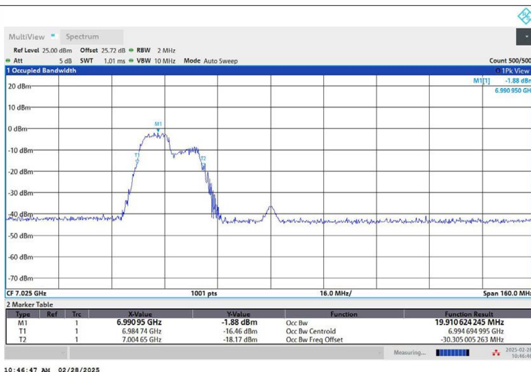
11AX80MIMO-Ant2-7025-106Tone-RU53-PASS
