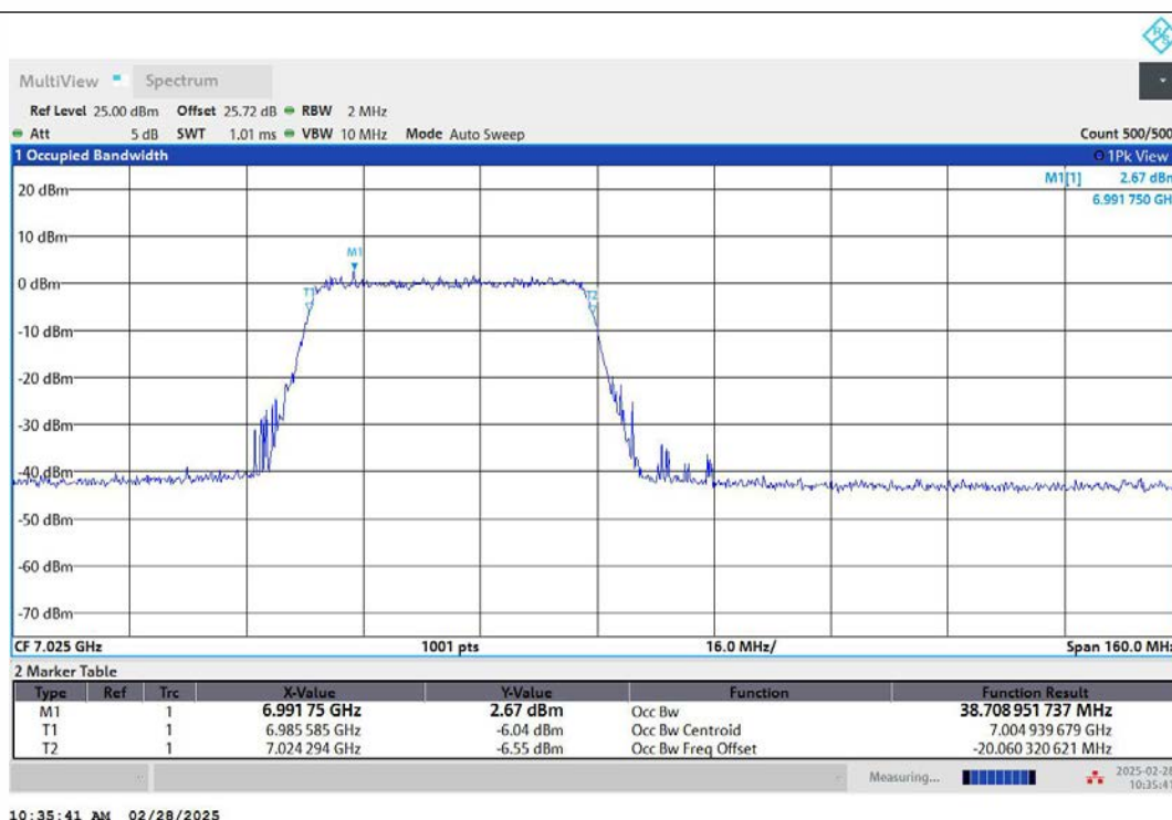
11AX80MIMO-Ant2-7025-484Tone-RU65-PASS
