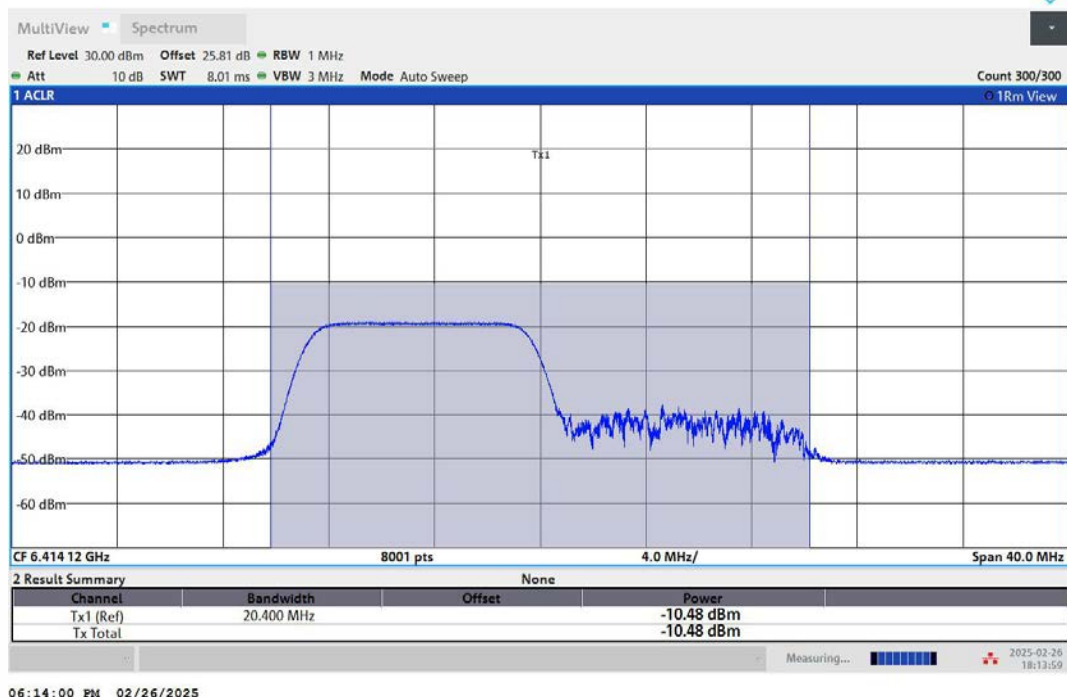
11AX20MIMO-Ant2-6415-106Tone-RU53-PASS
