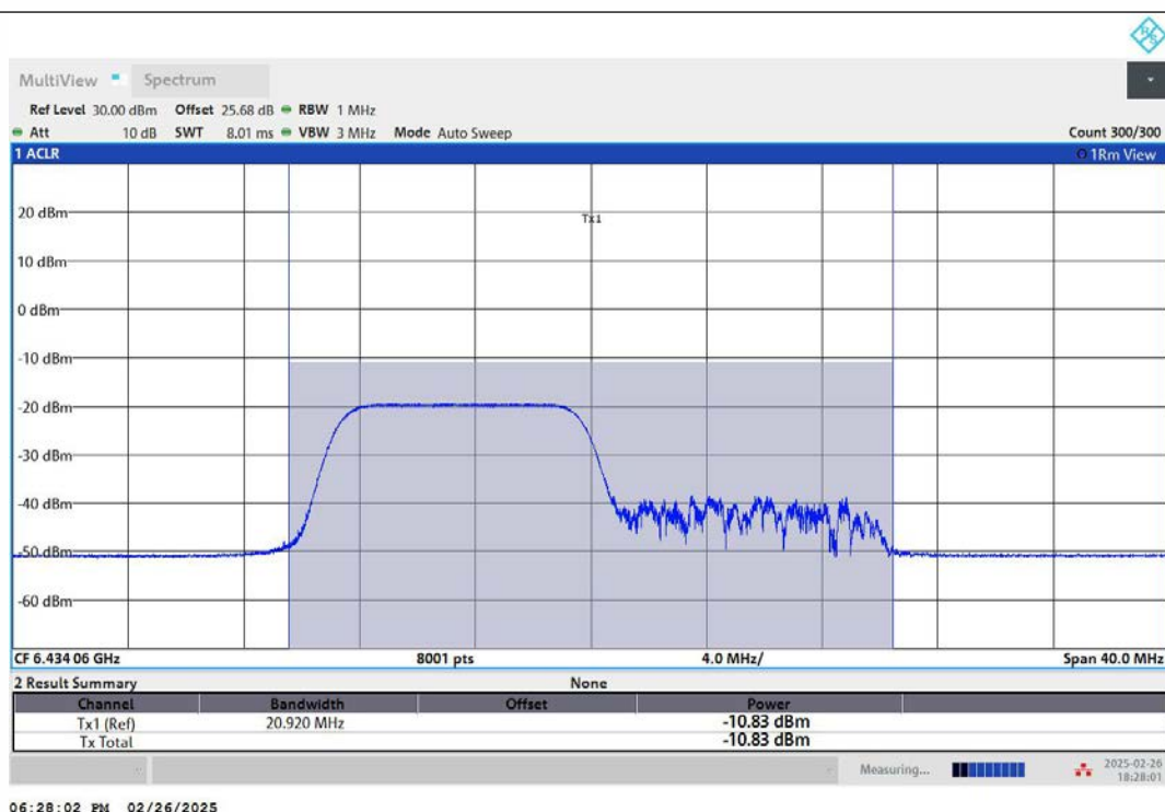
11AX20MIMO-Ant2-6435-106Tone-RU53-PASS
