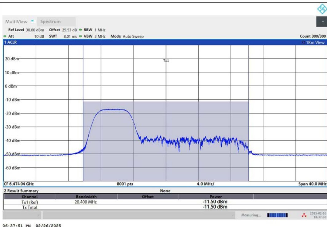
11AX20MIMO-Ant2-6475-52Tone-RU37-PASS
