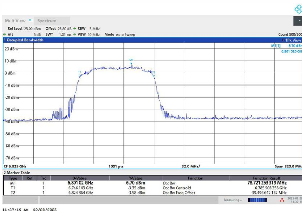
11AX160MIMO-Ant2-6825-996Tone-RU67-PASS
