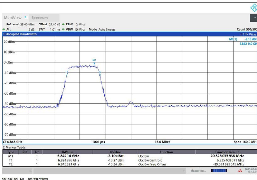
11AX80MIMO-Ant2-6865-242Tone-RU61-PASS
