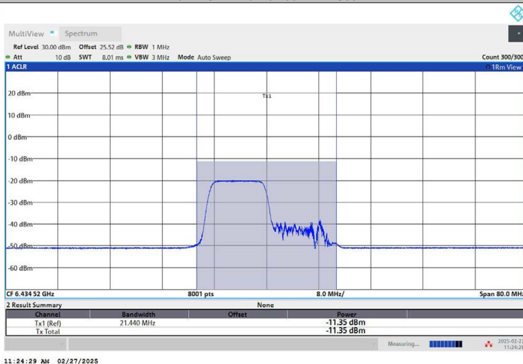
11AX40MIMO-Ant1-6445-242Tone-RU61-PASS
