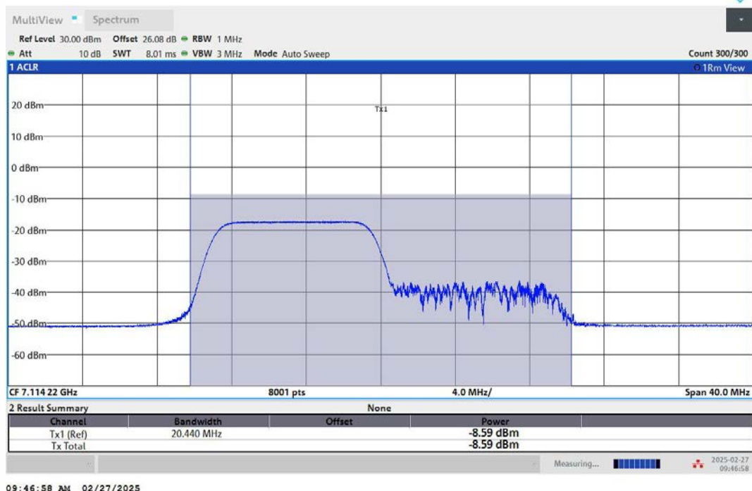
11AX20MIMO-Ant2-7115-106Tone-RU53-PASS
