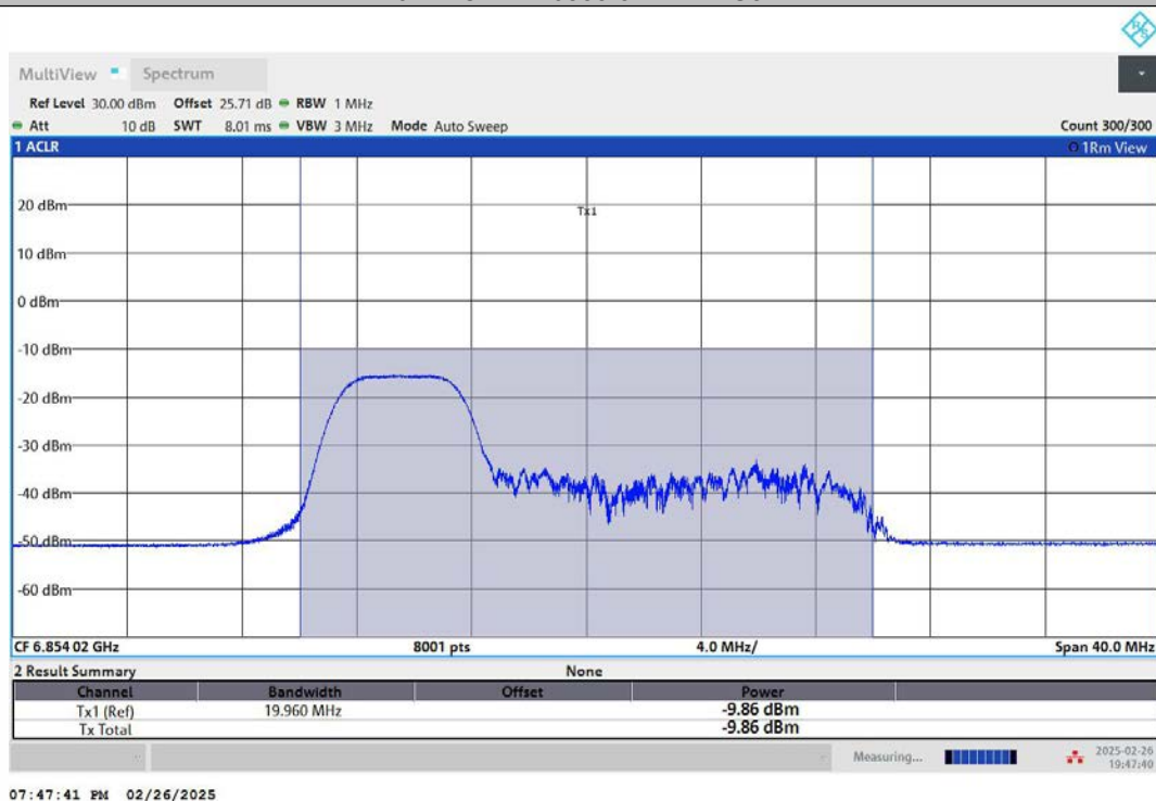
11AX20MIMO-Ant1-6855-106Tone-RU53-PASS
