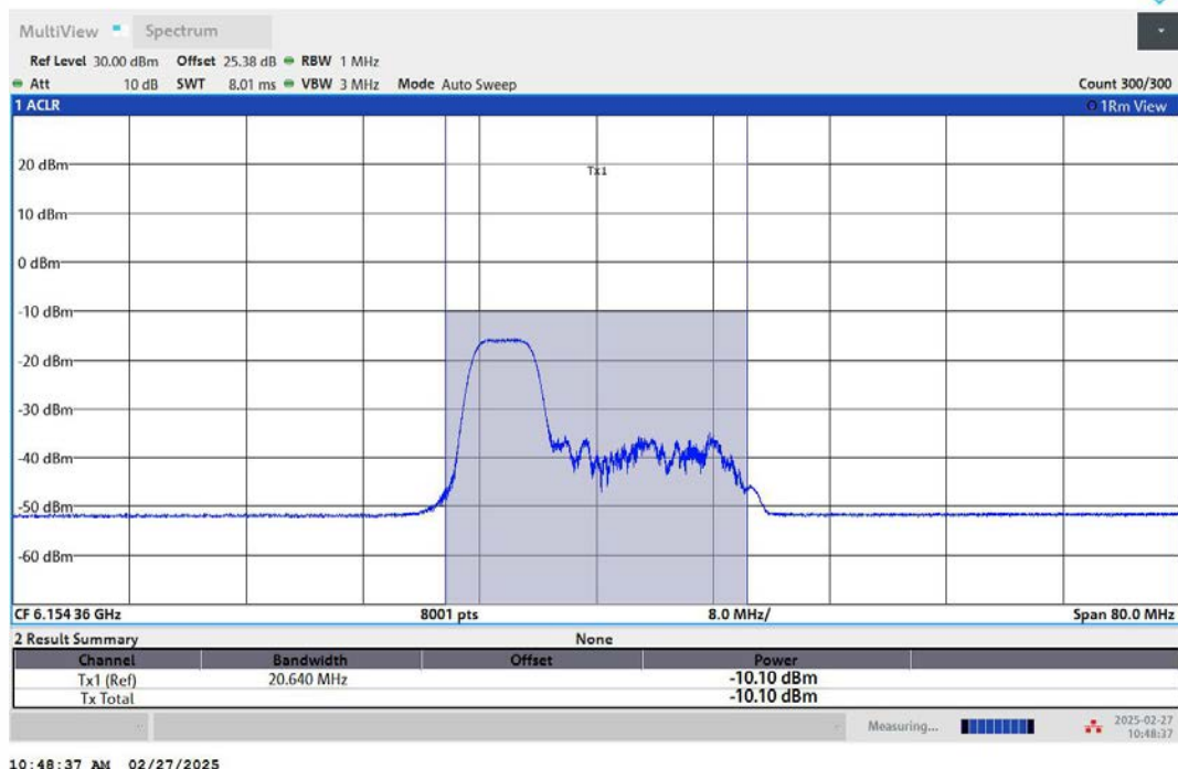
11AX40MIMO-Ant2-6165-52Tone-RU37-PASS
