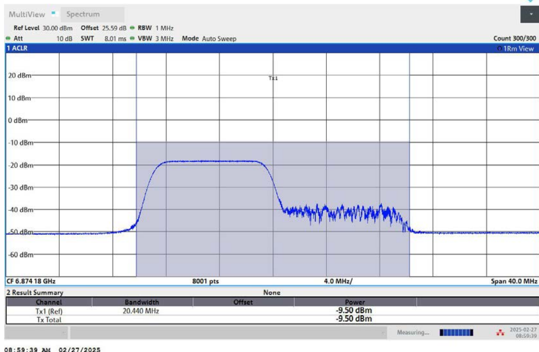
11AX20MIMO-Ant2-6875-106Tone-RU53-PASS
