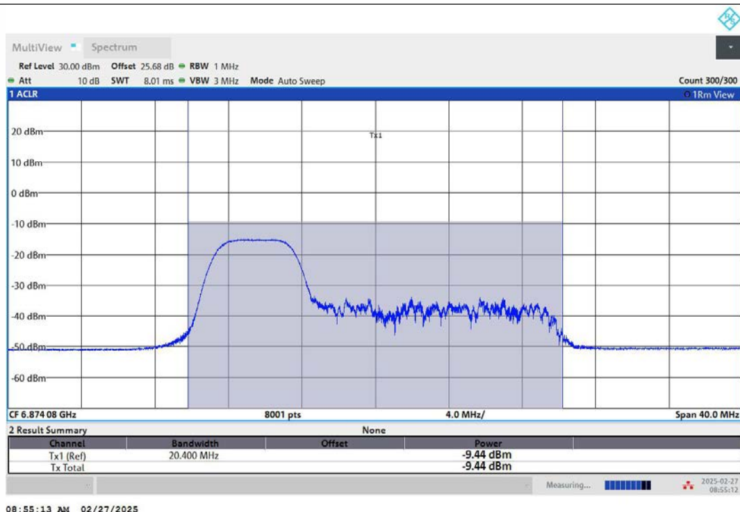
11AX20MIMO-Ant2-6875-52Tone-RU37-PASS
