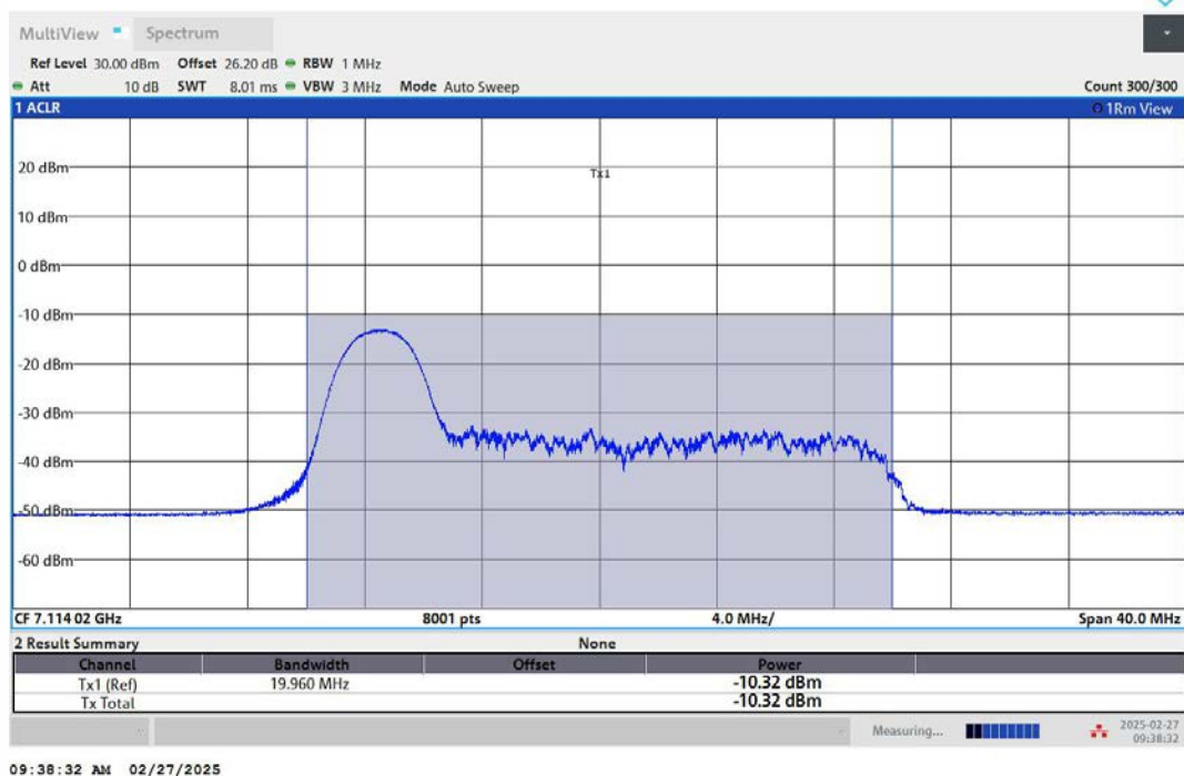
11AX20MIMO-Ant1-7115-52Tone-RU37-PASS
