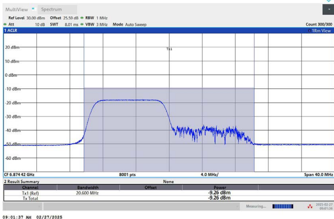
11AX20MIMO-Ant1-6895-26Tone-RU0-PASS
