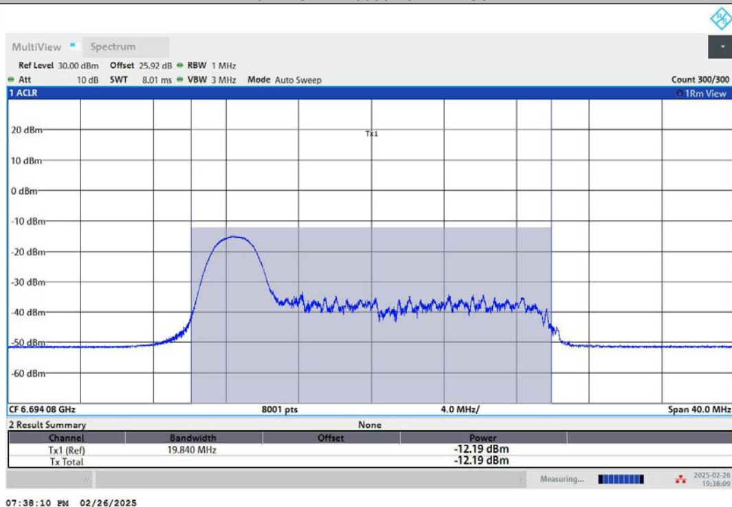
11AX20MIMO-Ant1-6695-52Tone-RU37-PASS
