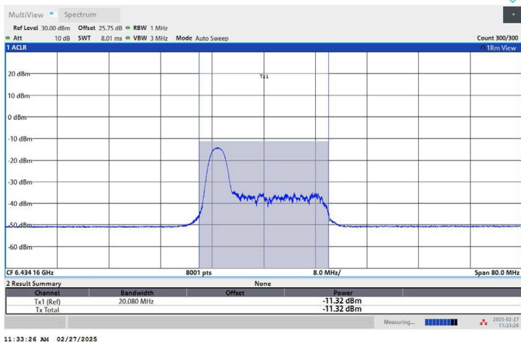
11AX40MIMO-Ant1-6445-52Tone-RU37-PASS
