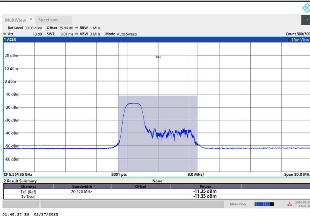
11AX40MIMO-Ant1-6565-106Tone-RU53-PASS
