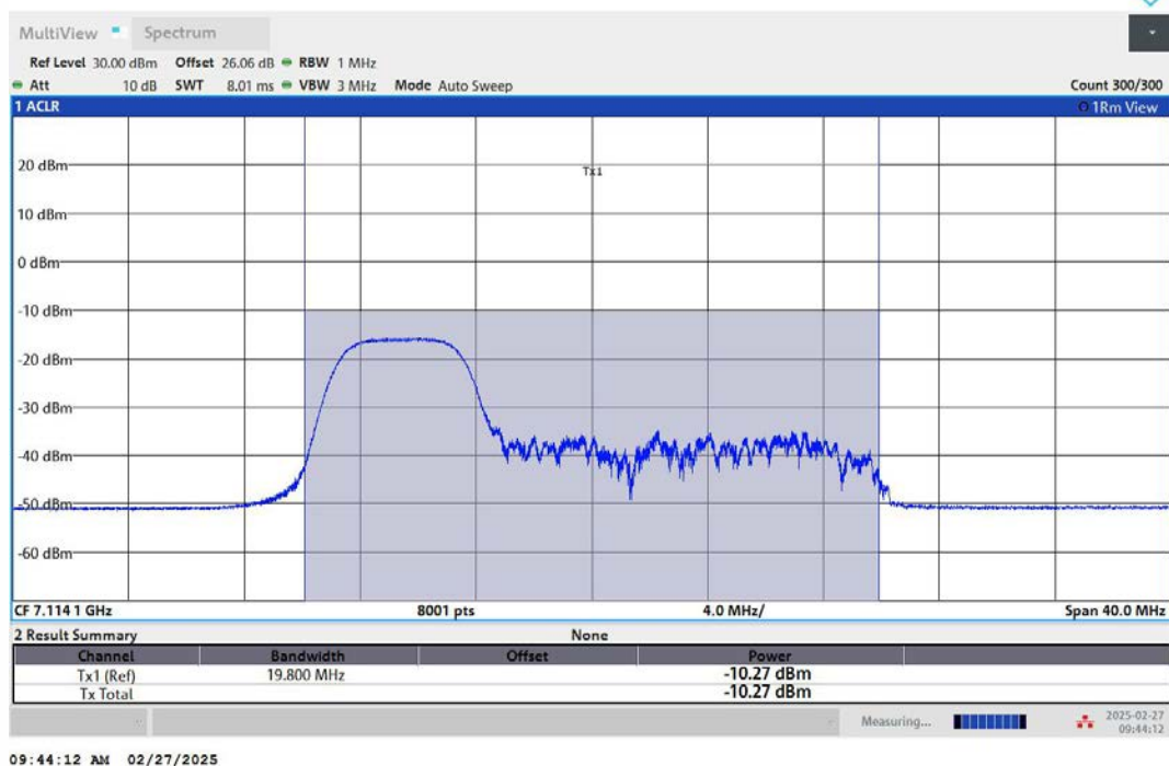
11AX20MIMO-Ant1-7115-106Tone-RU53-PASS
