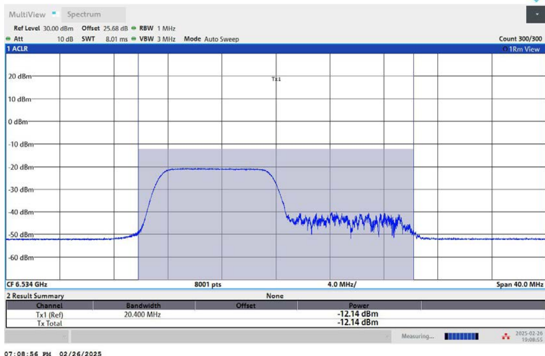
11AX20MIMO-Ant2-6535-106Tone-RU53-PASS
