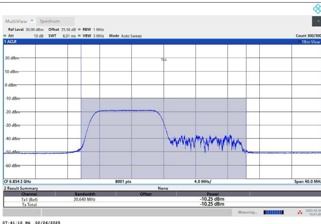
11AX20MIMO-Ant2-6855-106Tone-RU53-PASS
