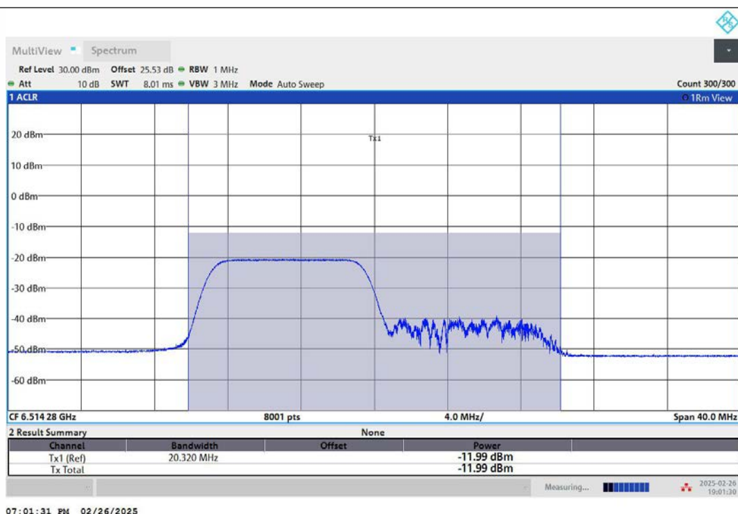
11AX20MIMO-Ant2-6515-106Tone-RU53-PASS
