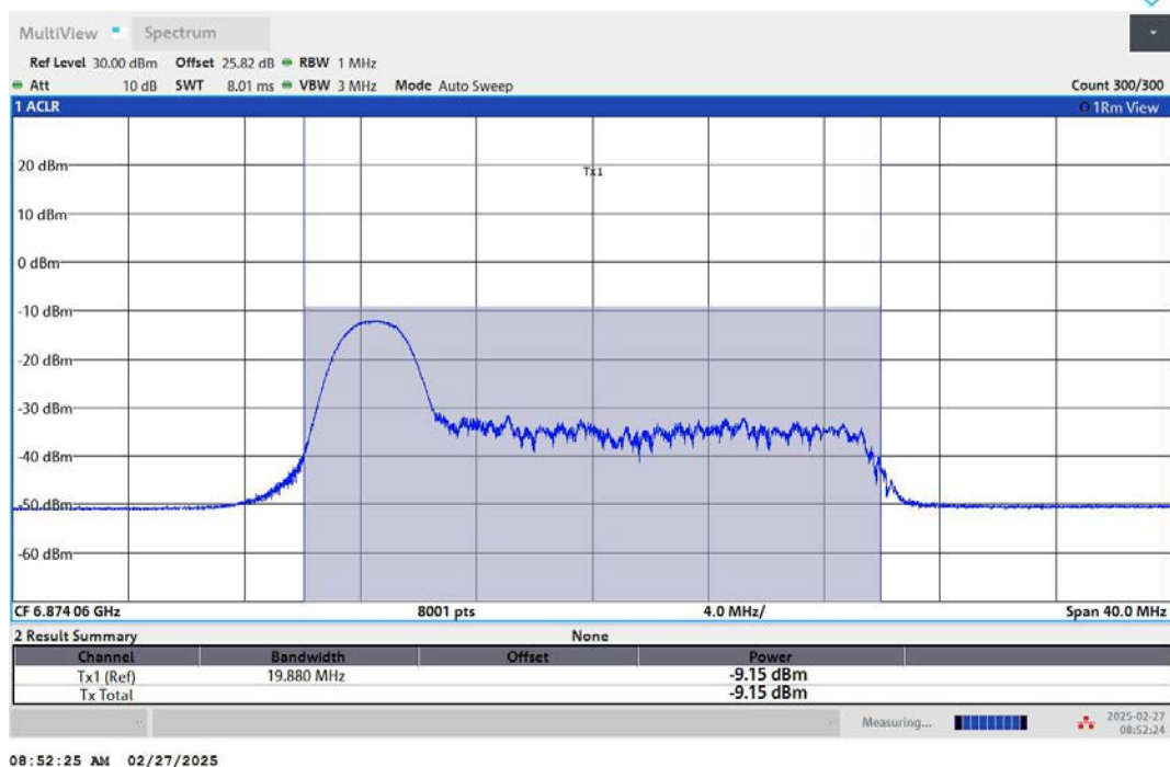
11AX20MIMO-Ant1-6875-52Tone-RU37-PASS
