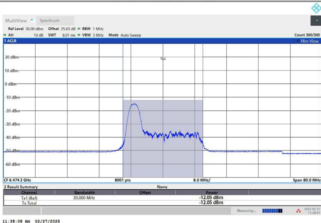
11AX40MIMO-Ant1-6485-52Tone-RU37-PASS
