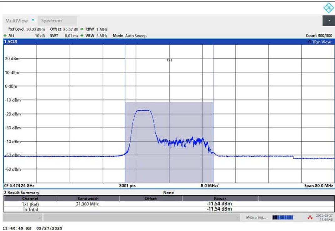
11AX40MIMO-Ant2-6485-52Tone-RU37-PASS
