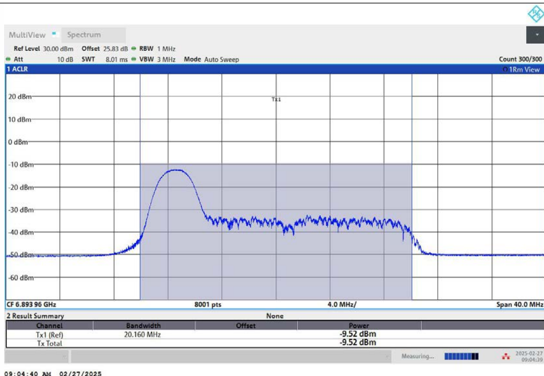
11AX20MIMO-Ant2-6895-26Tone-RU0-PASS
