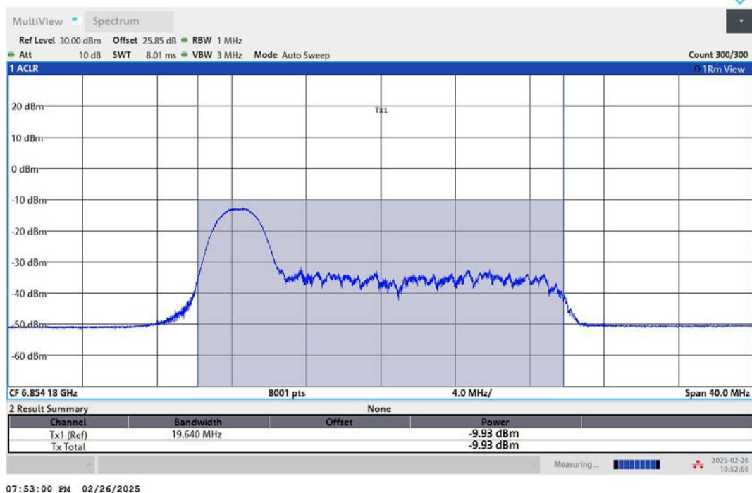
11AX20MIMO-Ant1-6855-52Tone-RU37-PASS
