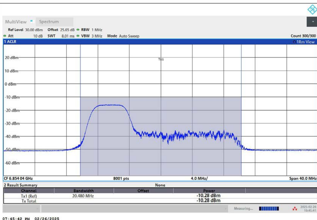
11AX20MIMO-Ant2-6855-52Tone-RU37-PASS
