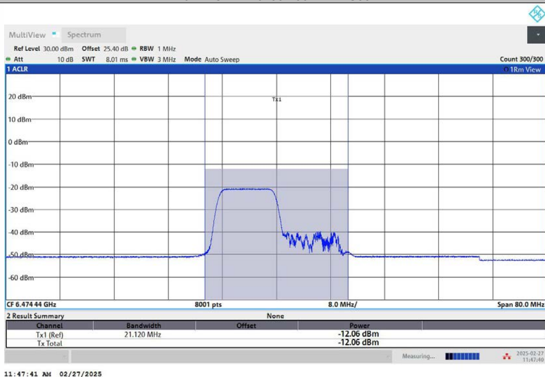
11AX40MIMO-Ant1-6485-242Tone-RU61-PASS
