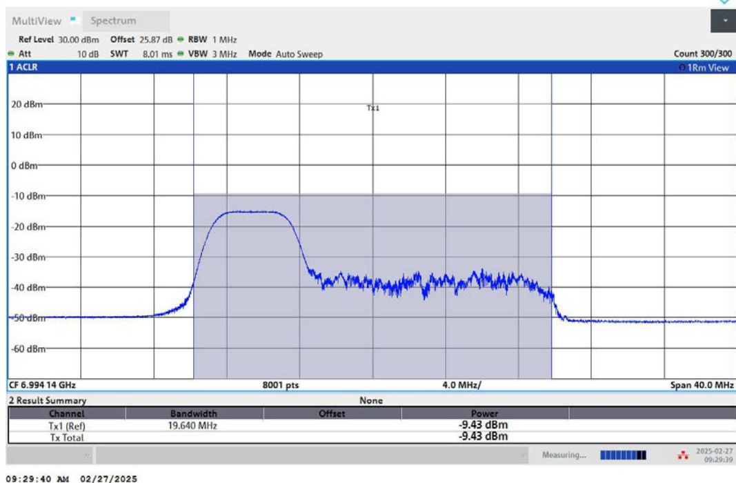
11AX20MIMO-Ant1-6995-106Tone-RU53-PASS
