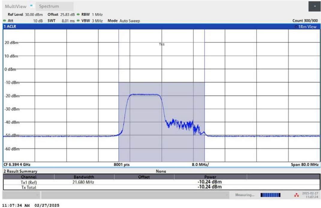
11AX40MIMO-Ant2-6405-106Tone-RU53-PASS
