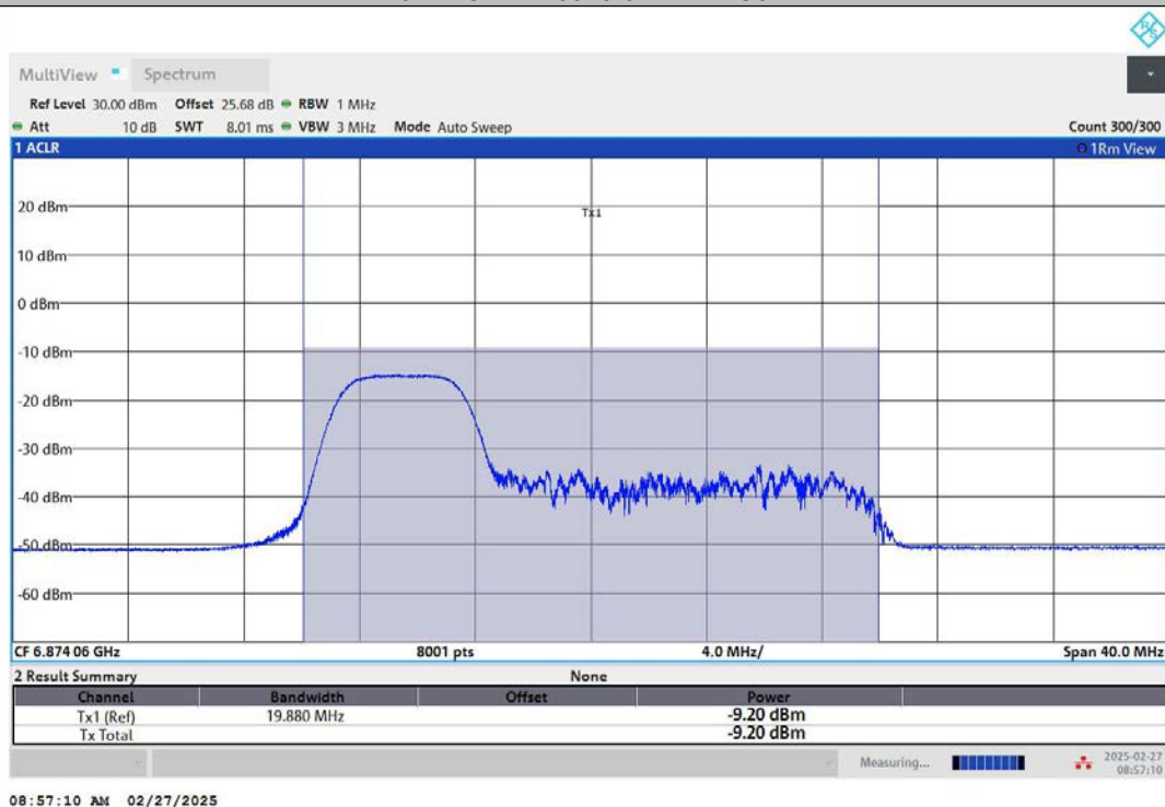
11AX20MIMO-Ant1-6875-106Tone-RU53-PASS
