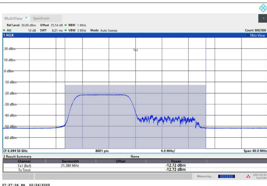
11AX20MIMO-Ant2-6695-106Tone-RU53-PASS
