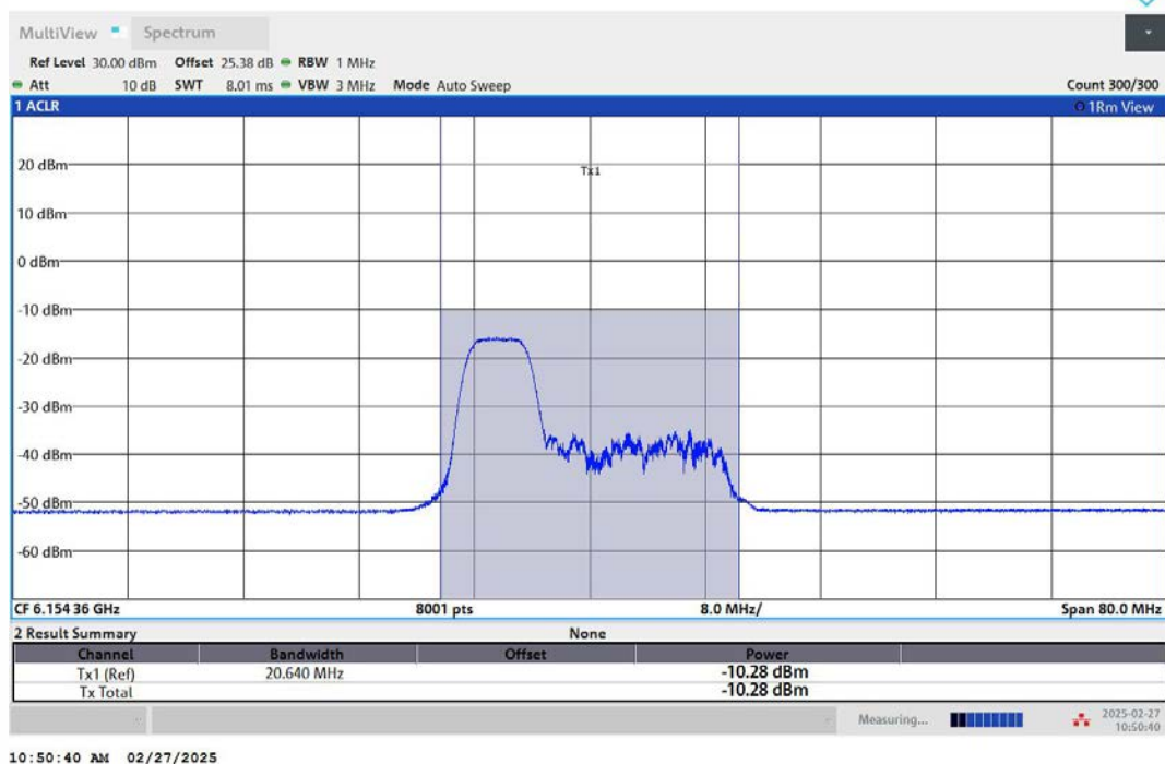
11AX40MIMO-Ant1-6165-106Tone-RU53-PASS
