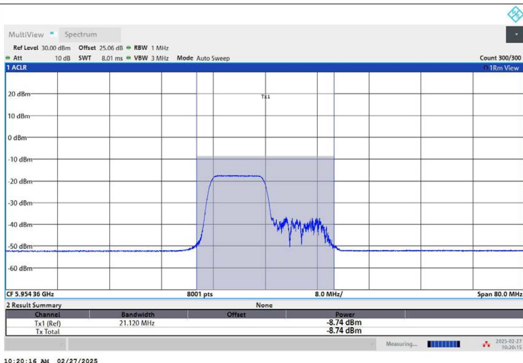
11AX40MIMO-Ant2-5965-106Tone-RU53-PASS
