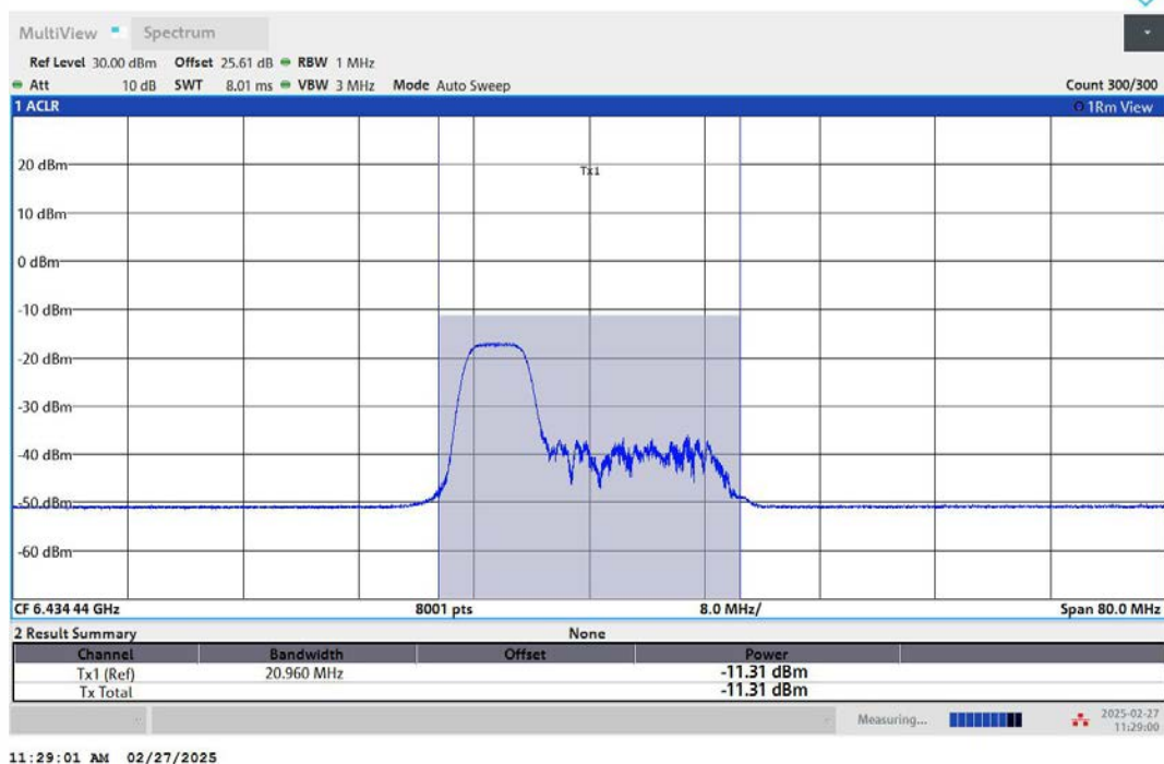
11AX40MIMO-Ant1-6445-106Tone-RU53-PASS
