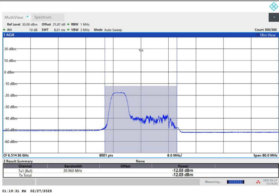
11AX40MIMO-Ant1-6525-106Tone-RU53-PASS
