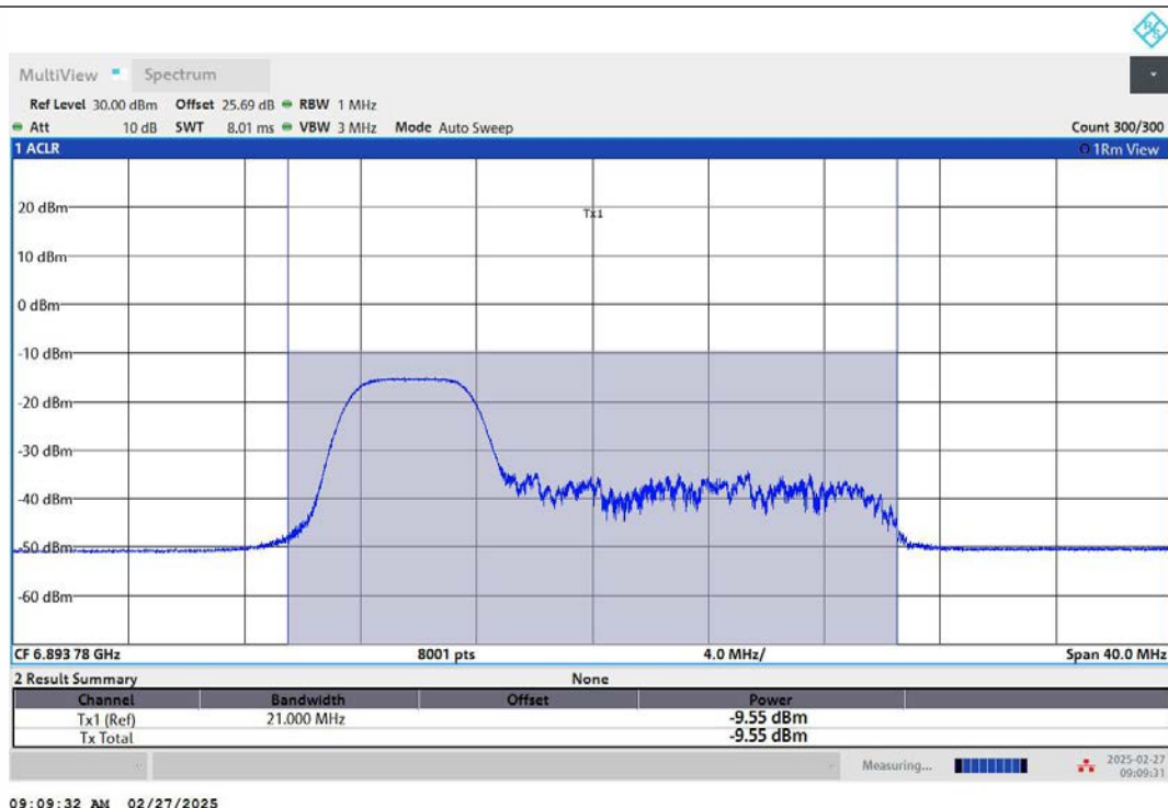
11AX20MIMO-Ant2-6895-52Tone-RU37-PASS
