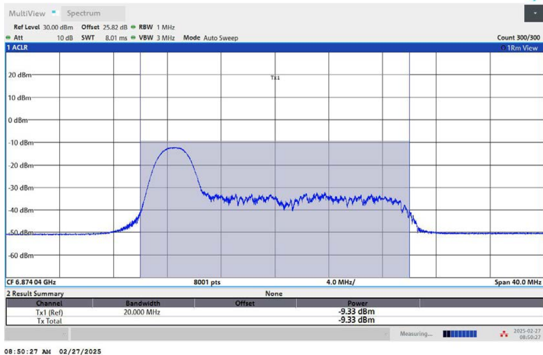
11AX20MIMO-Ant2-6875-26Tone-RU0-PASS
