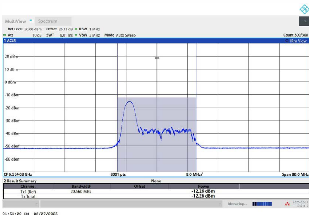
11AX40MIMO-Ant2-6565-26Tone-RU0-PASS
