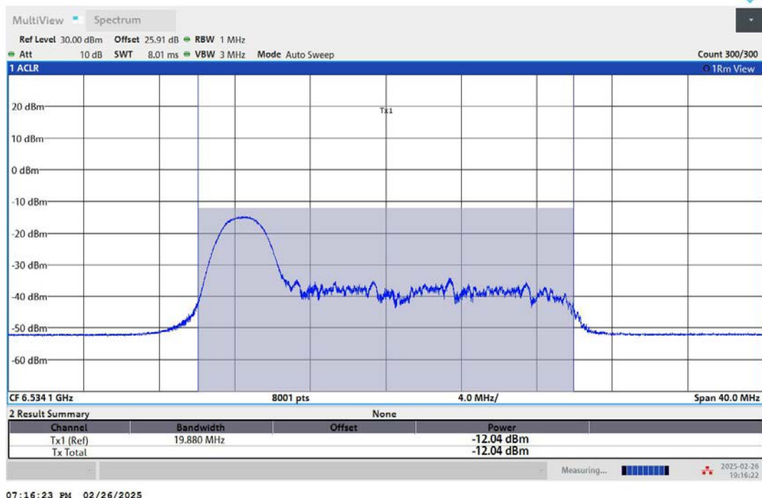
11AX20MIMO-Ant2-6535-26Tone-RU0-PASS
