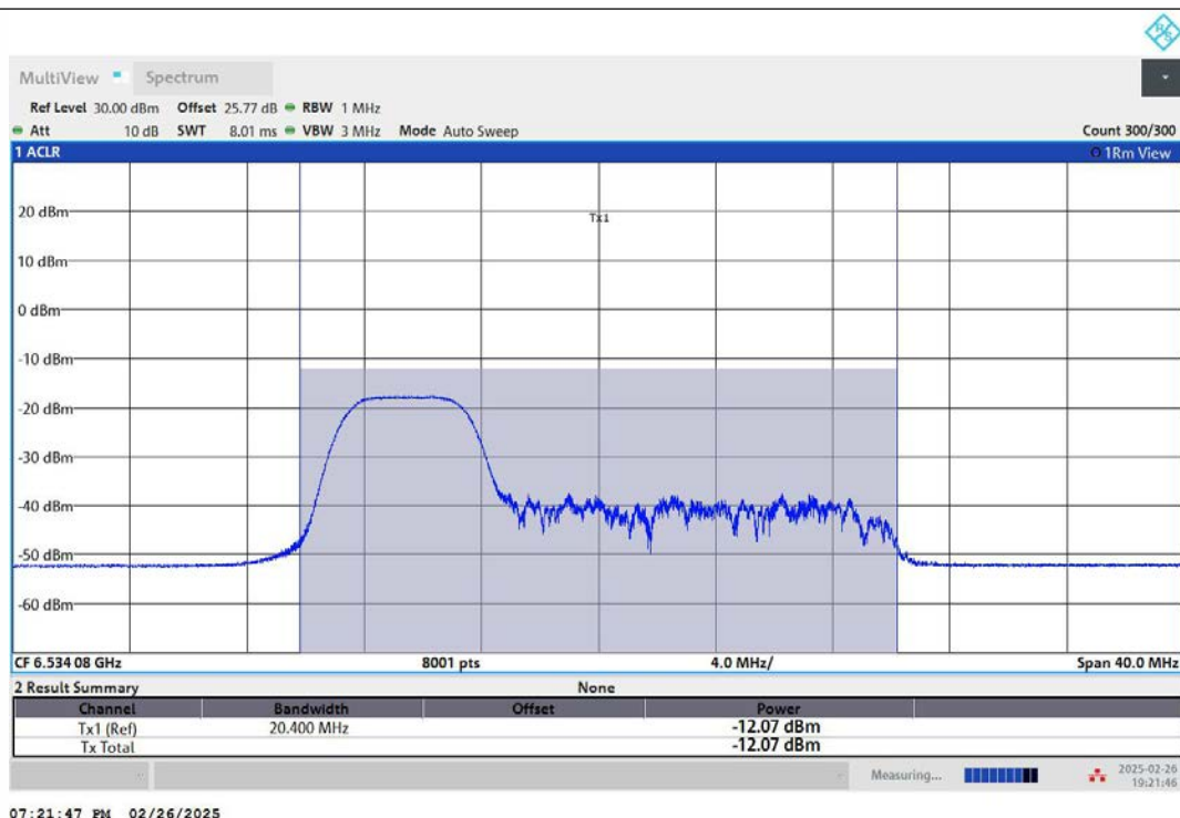
11AX20MIMO-Ant2-6535-52Tone-RU37-PASS
