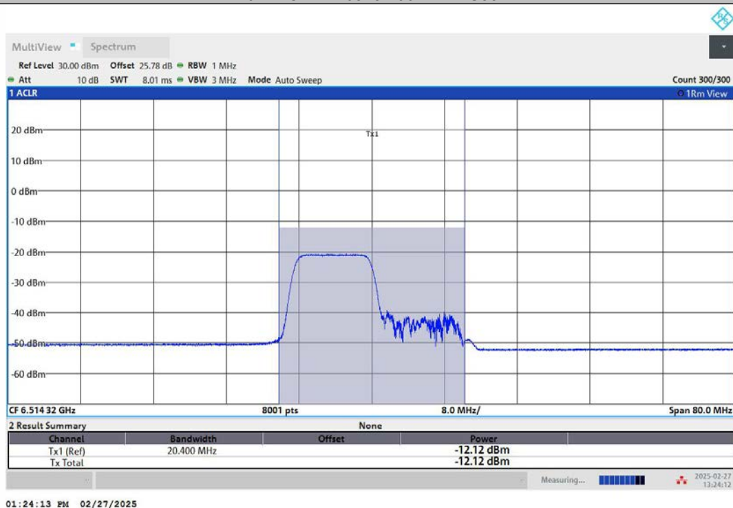
11AX40MIMO-Ant1-6525-242Tone-RU61-PASS
