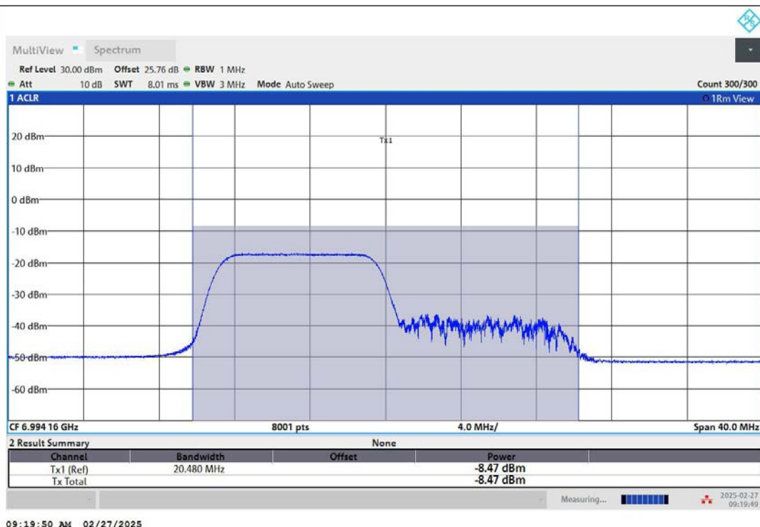
11AX20MIMO-Ant2-6995-106Tone-RU53-PASS
