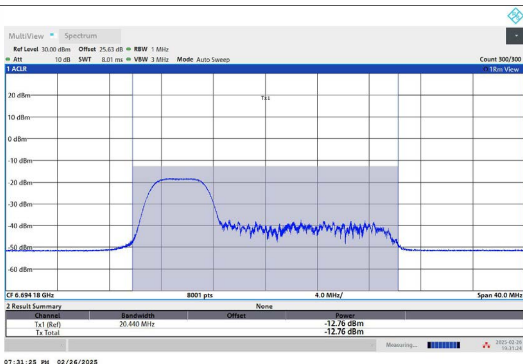
11AX20MIMO-Ant2-6695-52Tone-RU37-PASS
