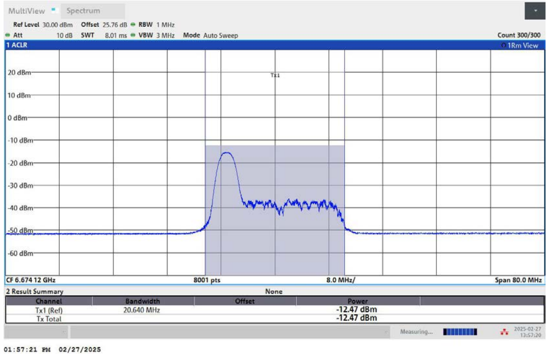
11AX40MIMO-Ant2-6685-26Tone-RU0-PASS
