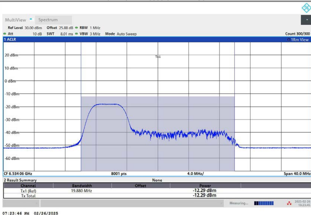
11AX20MIMO-Ant1-6535-106Tone-RU53-PASS
