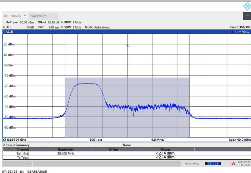
11AX20MIMO-Ant1-6695-106Tone-RU53-PASS
