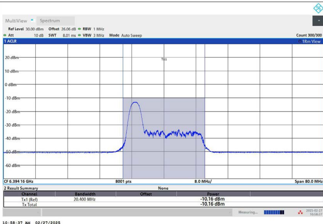
11AX40MIMO-Ant2-6405-26Tone-RU0-PASS
