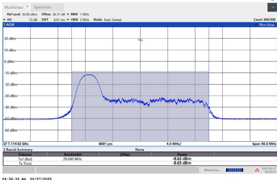
11AX20MIMO-Ant2-7115-26Tone-RU0-PASS
