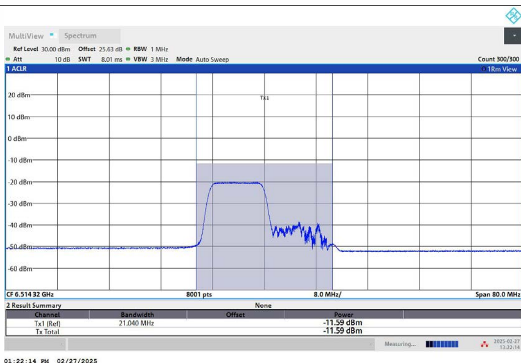
11AX40MIMO-Ant2-6525-106Tone-RU53-PASS
