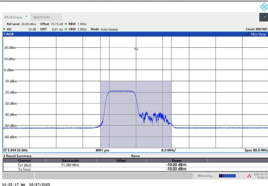
11AX40MIMO-Ant1-5965-242Tone-RU61-PASS
