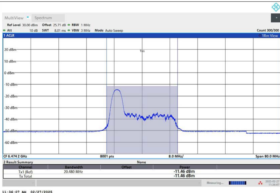
11AX40MIMO-Ant2-6485-26Tone-RU0-PASS
