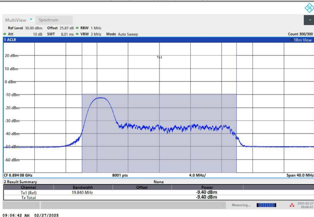
11AX20MIMO-Ant1-6895-52Tone-RU37-PASS
