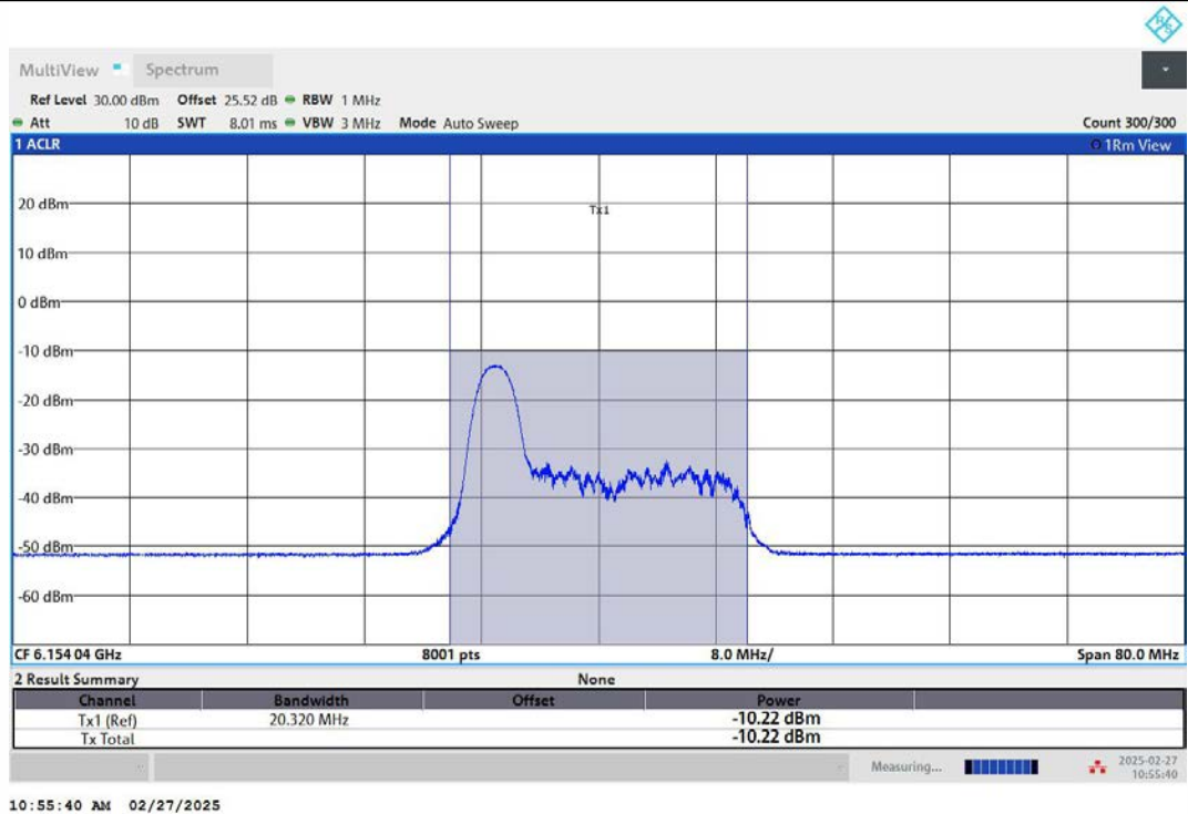
11AX40MIMO-Ant1-6165-52Tone-RU37-PASS
