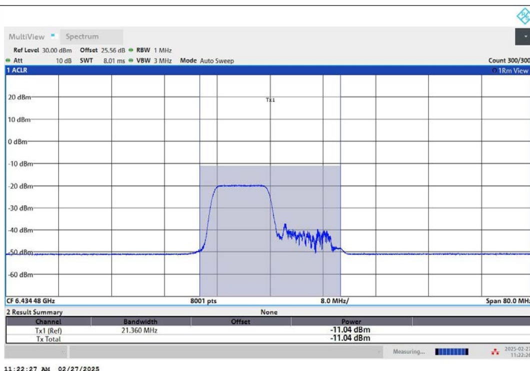
11AX40MIMO-Ant2-6445-106Tone-RU53-PASS
