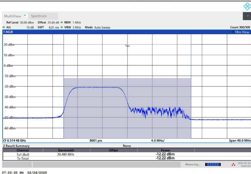
11AX20MIMO-Ant1-6535-26Tone-RU0-PASS
