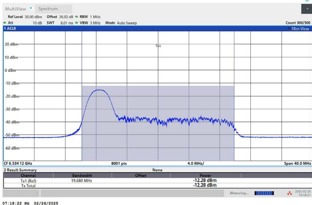
11AX20MIMO-Ant1-6535-52Tone-RU37-PASS
