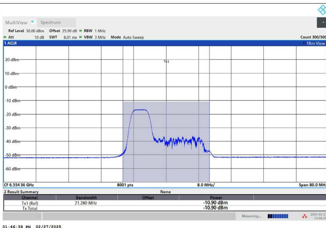
11AX40MIMO-Ant2-6565-52Tone-RU37-PASS
