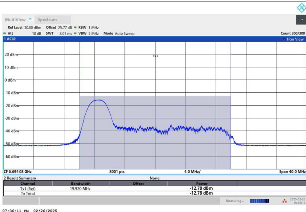
11AX20MIMO-Ant2-6695-26Tone-RU0-PASS
