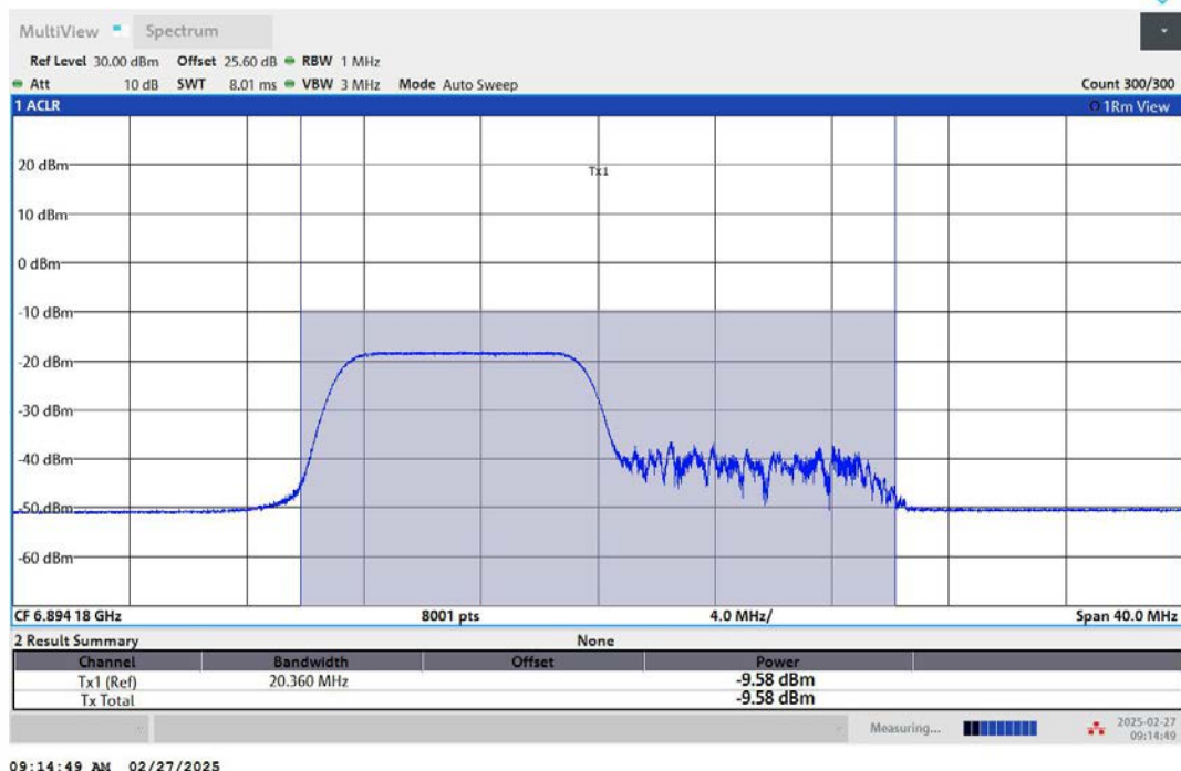
11AX20MIMO-Ant2-6895-106Tone-RU53-PASS
