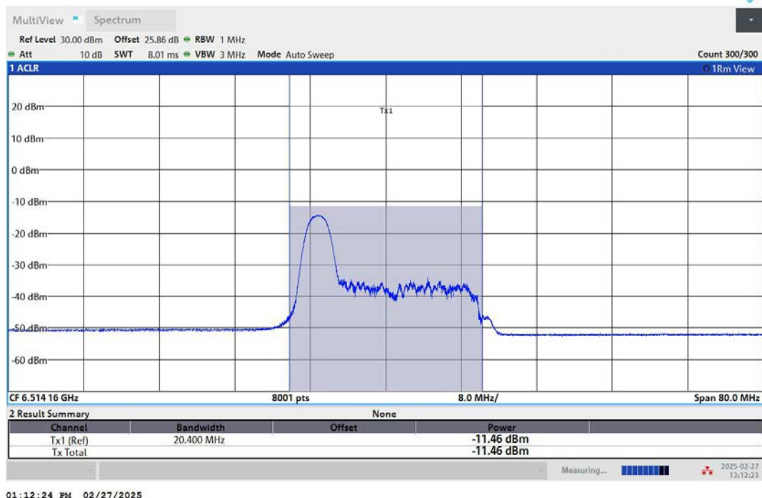
11AX40MIMO-Ant2-6525-26Tone-RU0-PASS
