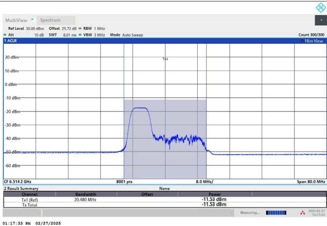
11AX40MIMO-Ant2-6525-52Tone-RU37-PASS
