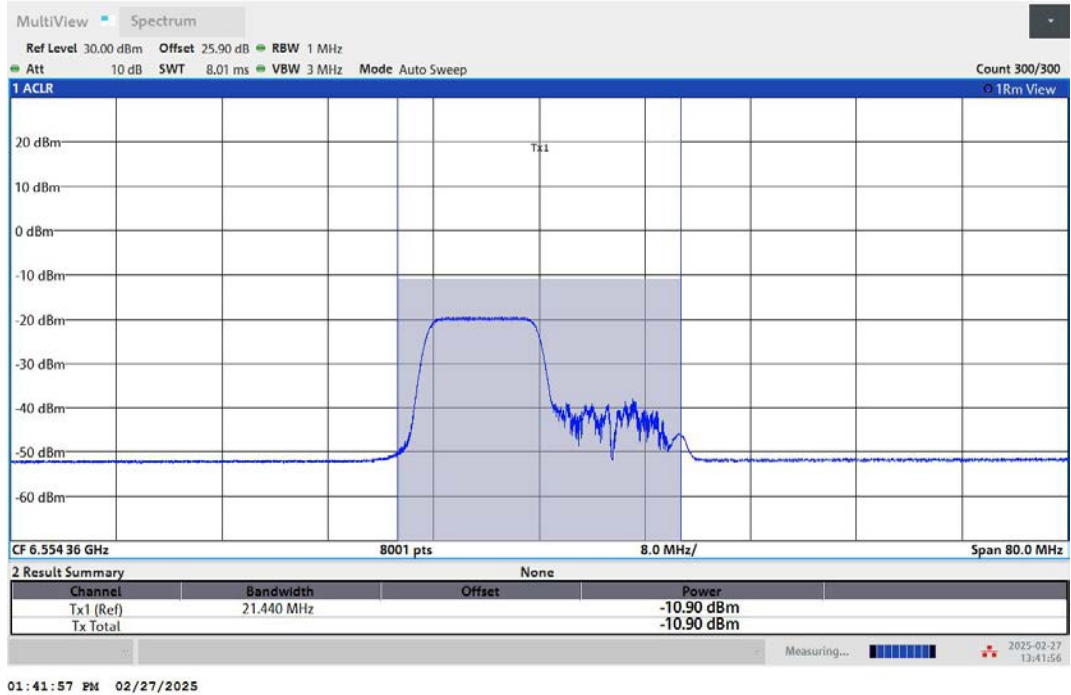
11AX40MIMO-Ant2-6565-106Tone-RU53-PASS
