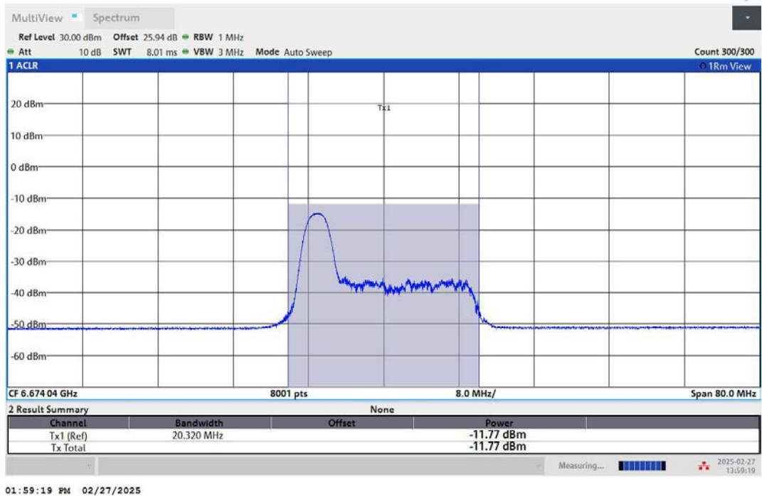
11AX40MIMO-Ant1-6685-52Tone-RU37-PASS
