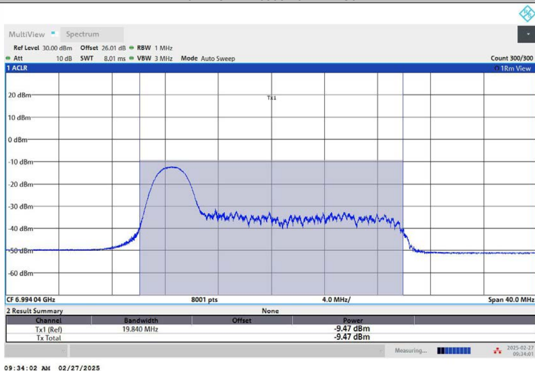
11AX20MIMO-Ant1-6995-52Tone-RU37-PASS
