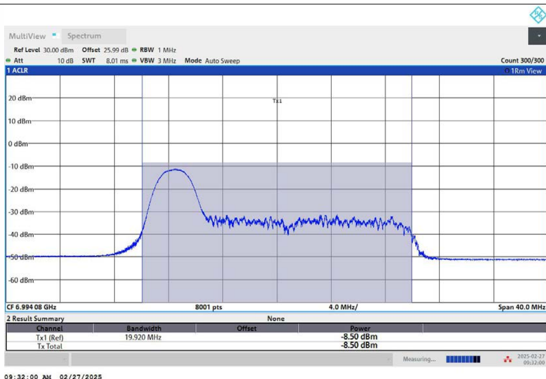
11AX20MIMO-Ant2-6995-26Tone-RU0-PASS
