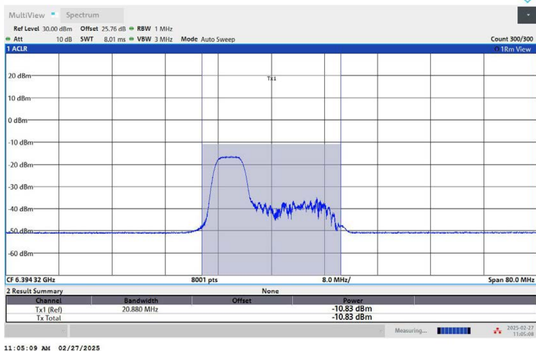
11AX40MIMO-Ant1-6405-106Tone-RU53-PASS
