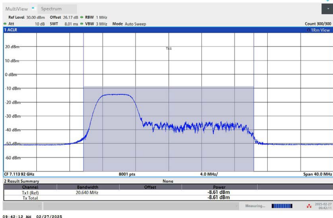
11AX20MIMO-Ant2-7115-52Tone-RU37-PASS
