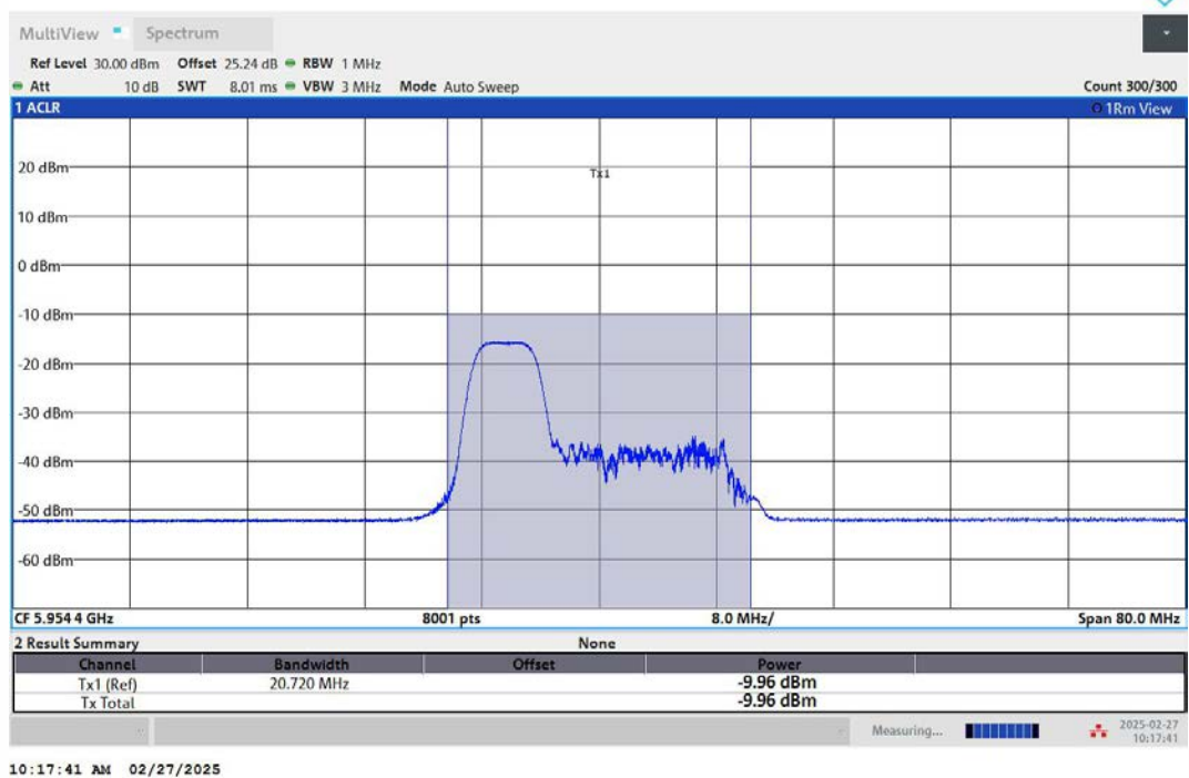
11AX40MIMO-Ant1-5965-106Tone-RU53-PASS
