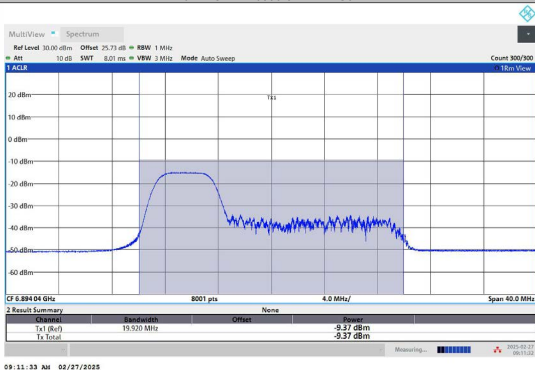
11AX20MIMO-Ant1-6895-106Tone-RU53-PASS
