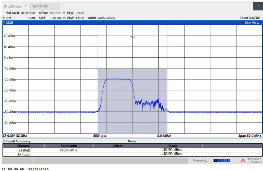
11AX40MIMO-Ant1-6405-242Tone-RU61-PASS
