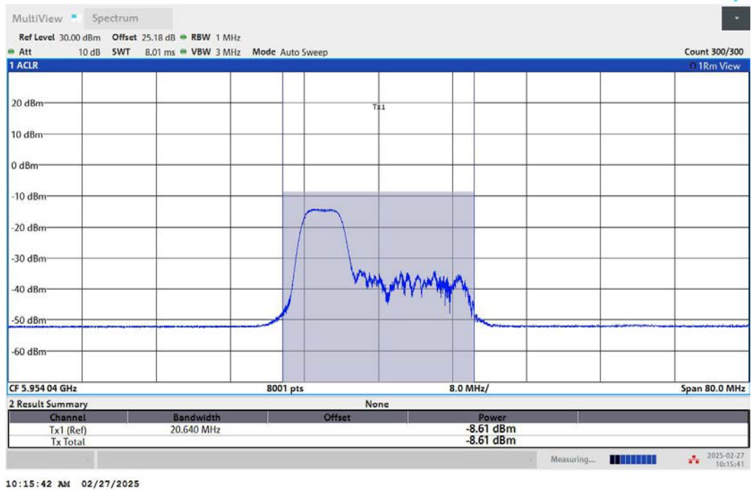
11AX40MIMO-Ant2-5965-52Tone-RU37-PASS
