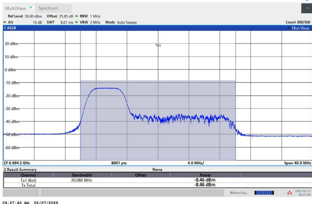
11AX20MIMO-Ant2-6995-52Tone-RU37-PASS
