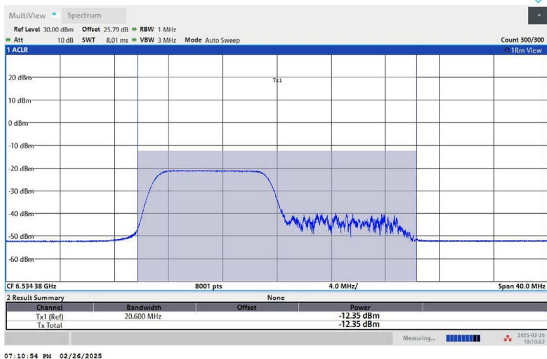
11AX20MIMO-Ant1-6695-26Tone-RU0-PASS
