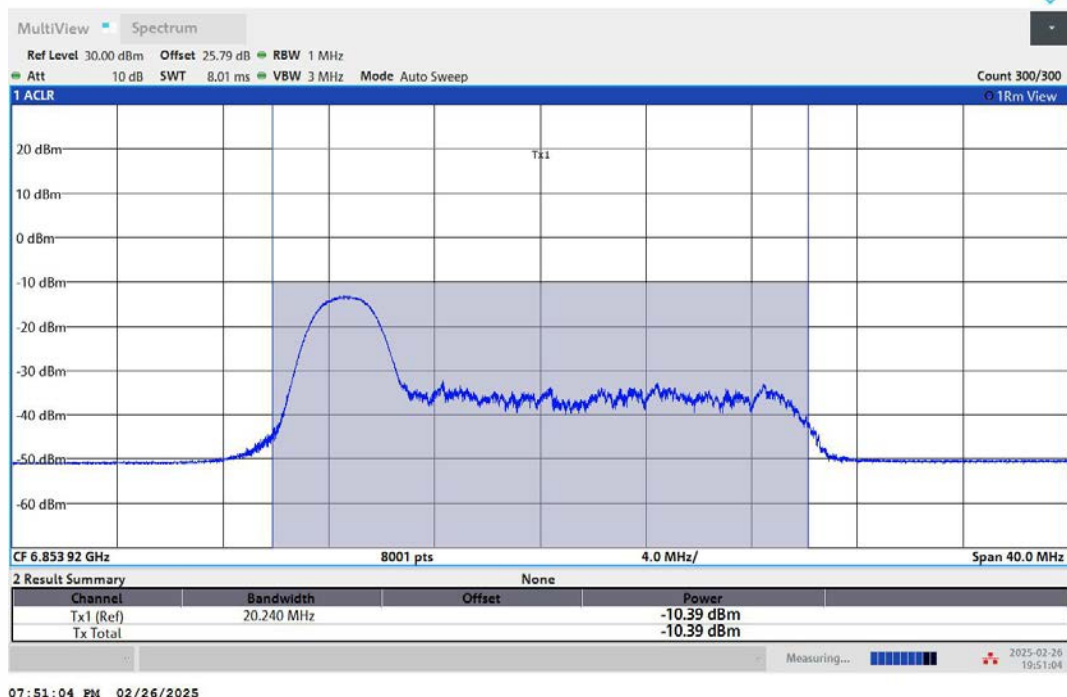
11AX20MIMO-Ant2-6855-26Tone-RU0-PASS
