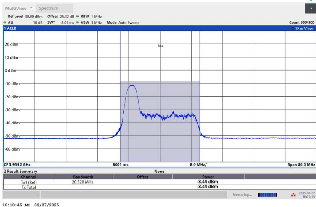
11AX40MIMO-Ant2-5965-26Tone-RU0-PASS
