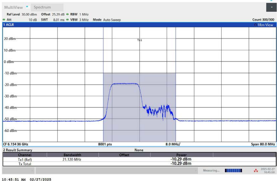
11AX40MIMO-Ant1-6165-242Tone-RU61-PASS
