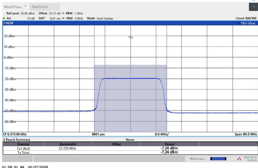
11AX40MIMO-Ant2-6525-242Tone-RU61-PASS
