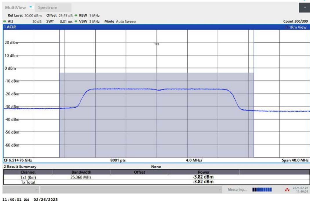
11AX20MIMO-Ant2-6515-PASS
