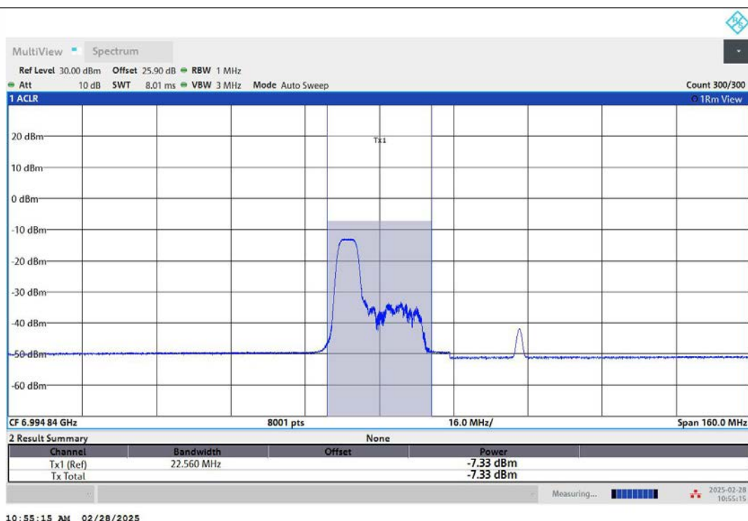
11AX80MIMO-Ant2-7025-52Tone-RU37-PASS
