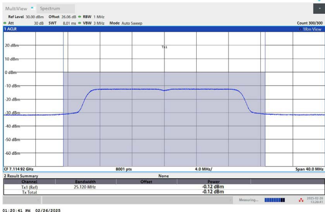
11AX20MIMO-Ant2-7115-PASS
