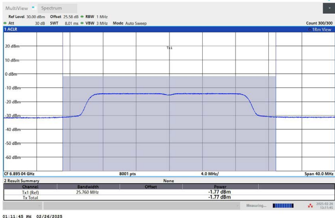
11AX20MIMO-Ant2-6895-PASS
