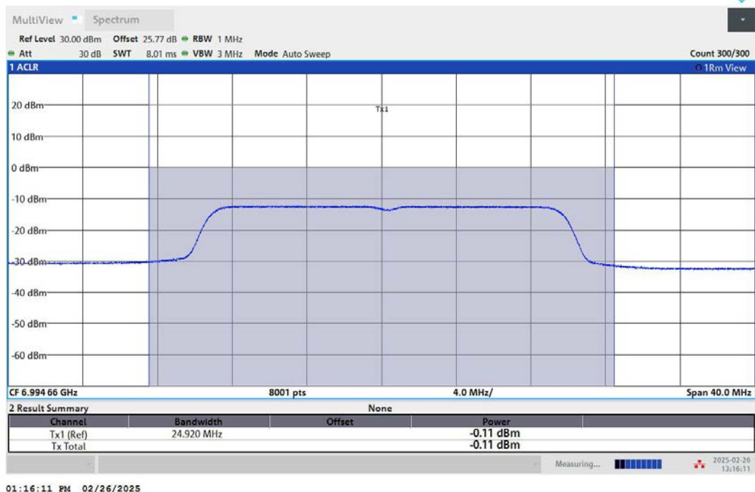
11AX20MIMO-Ant2-6995-PASS
