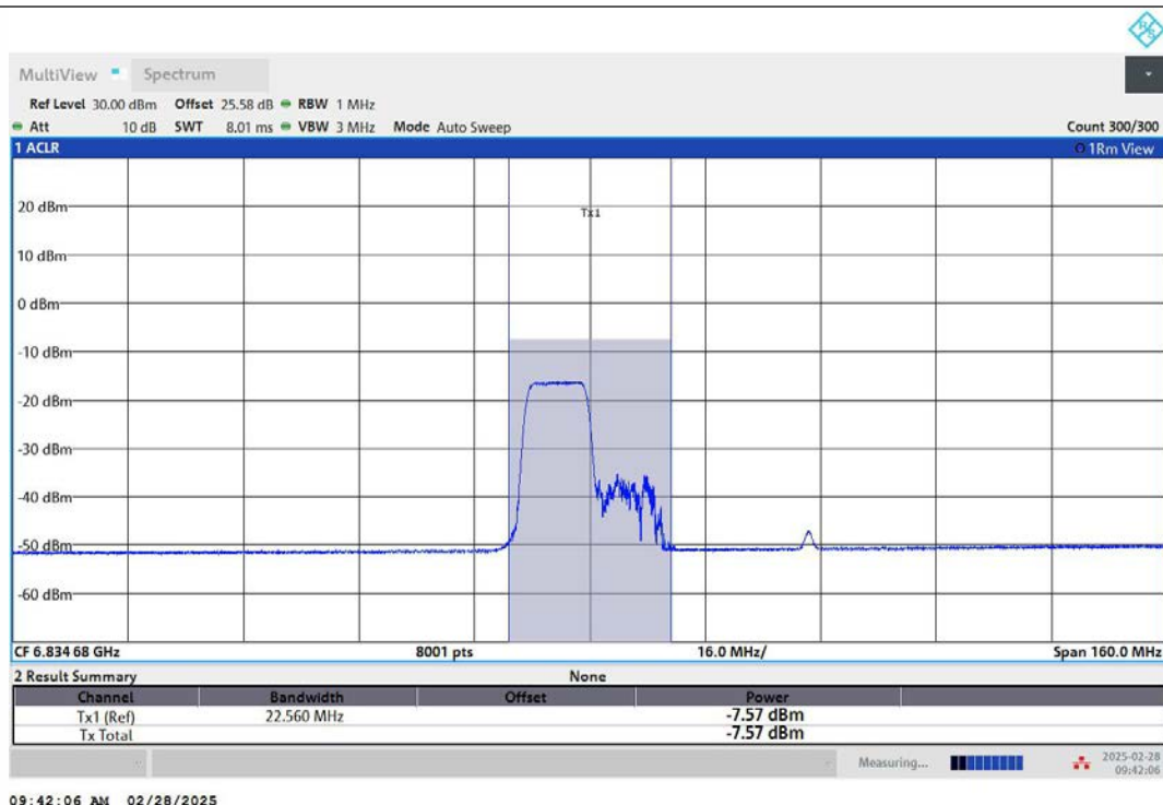
11AX80MIMO-Ant2-6865-106Tone-RU53-PASS
