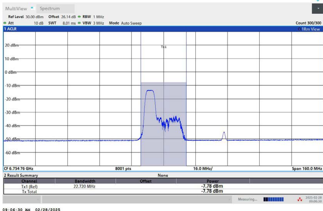
11AX80MIMO-Ant2-6785-52Tone-RU37-PASS
