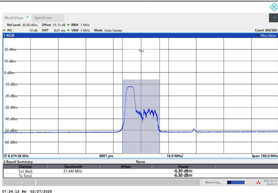
11AX80MIMO-Ant1-6705-106Tone-RU53-PASS
