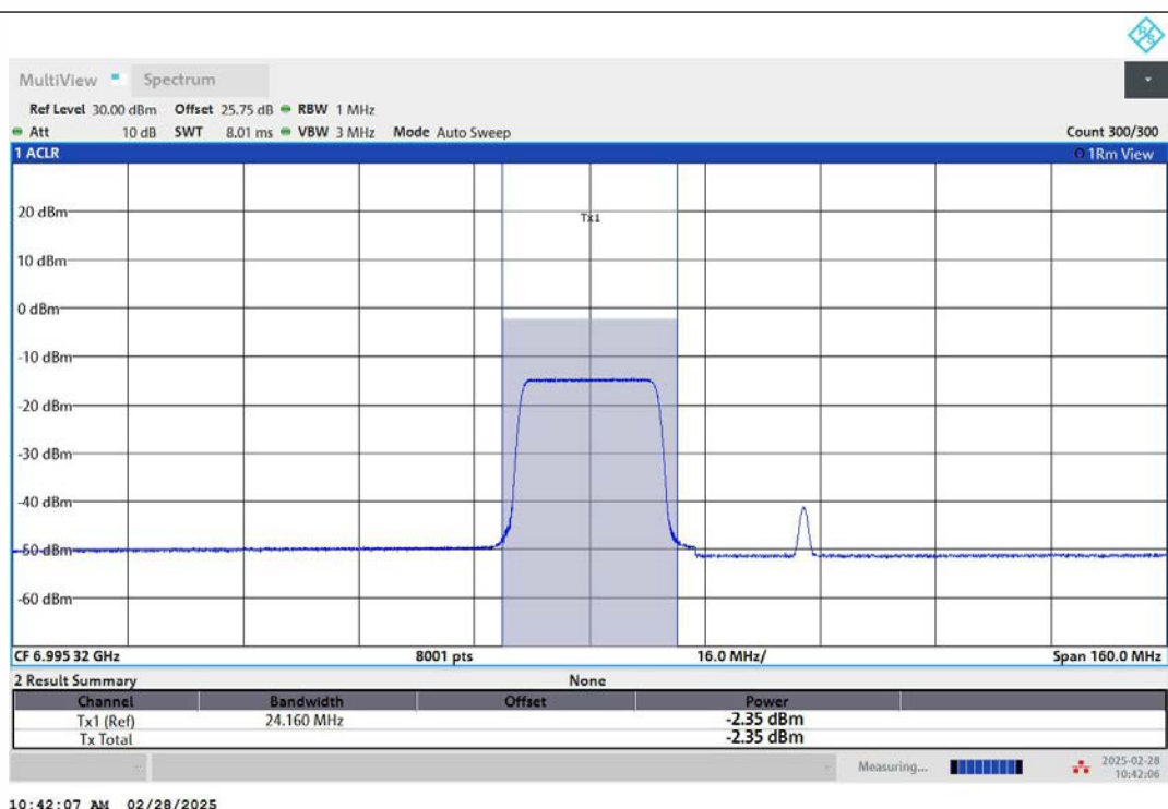
11AX80MIMO-Ant2-7025-242Tone-RU61-PASS
