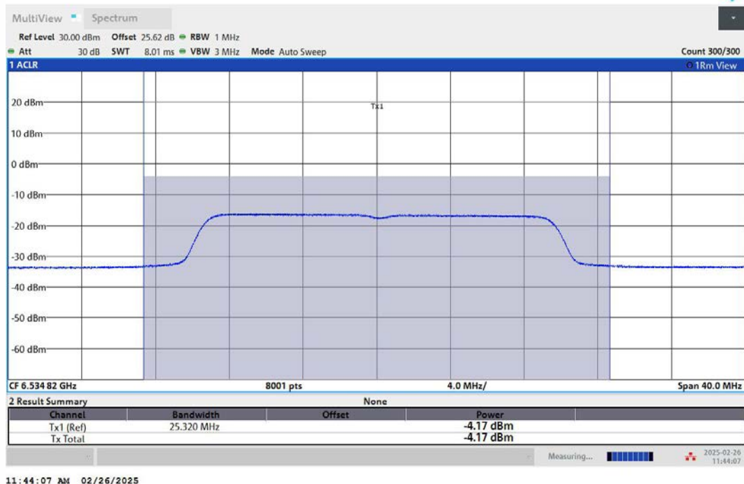
11AX20MIMO-Ant2-6535-PASS
