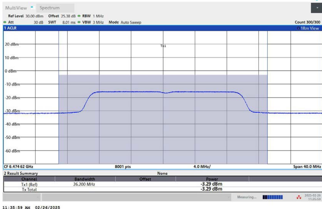
11AX20MIMO-Ant2-6475-PASS
