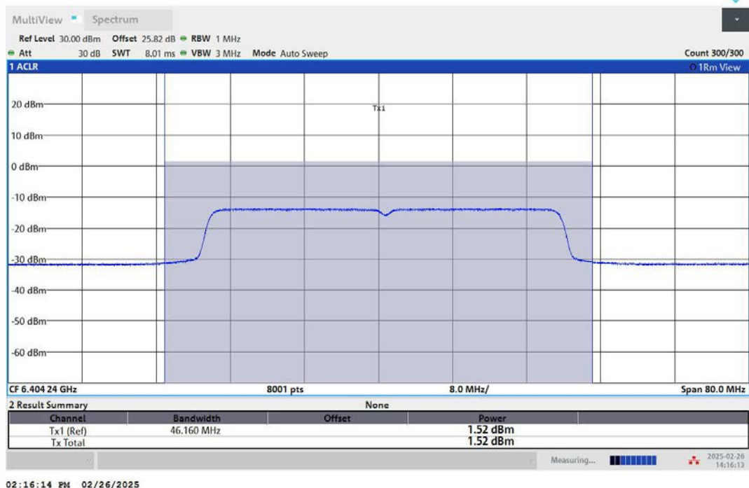
11AX40MIMO-Ant2-6405-PASS
