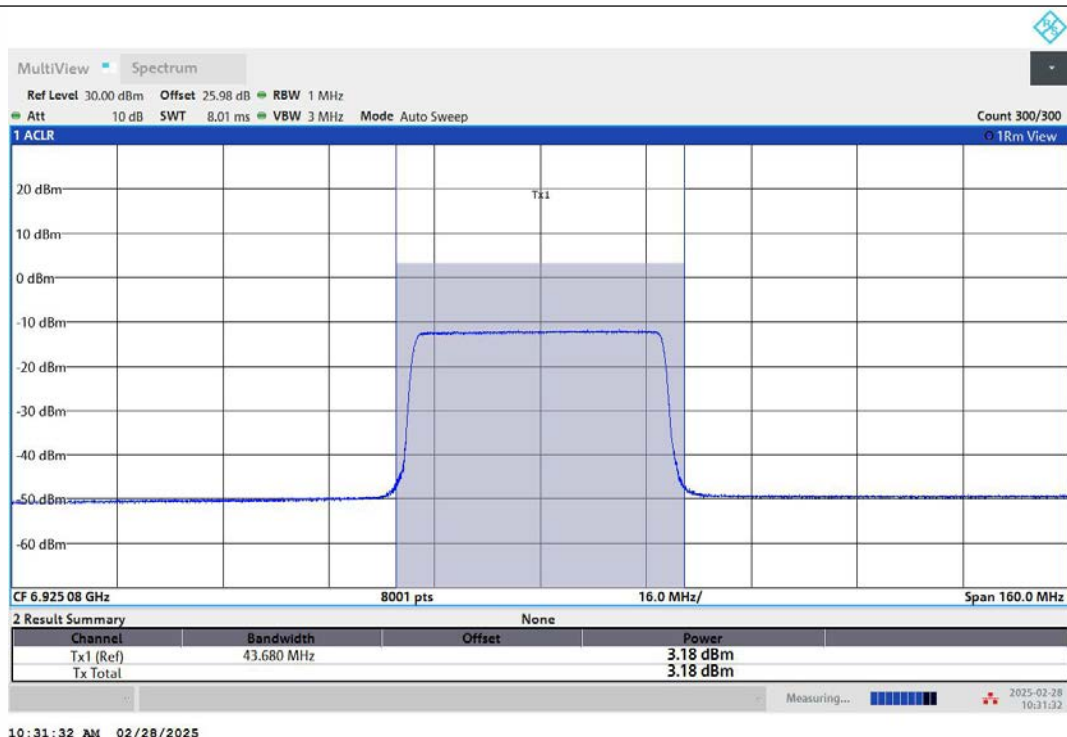
11AX80MIMO-Ant2-6945-484Tone-RU65-PASS
