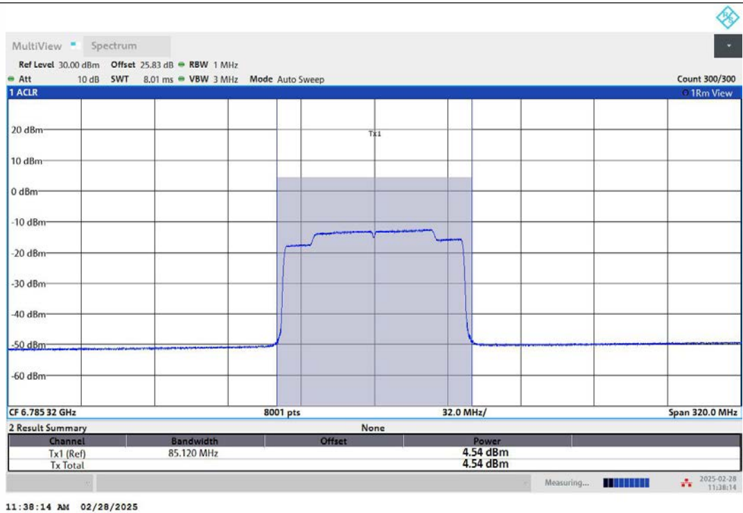
11AX160MIMO-Ant2-6825-996Tone-RU67-PASS
