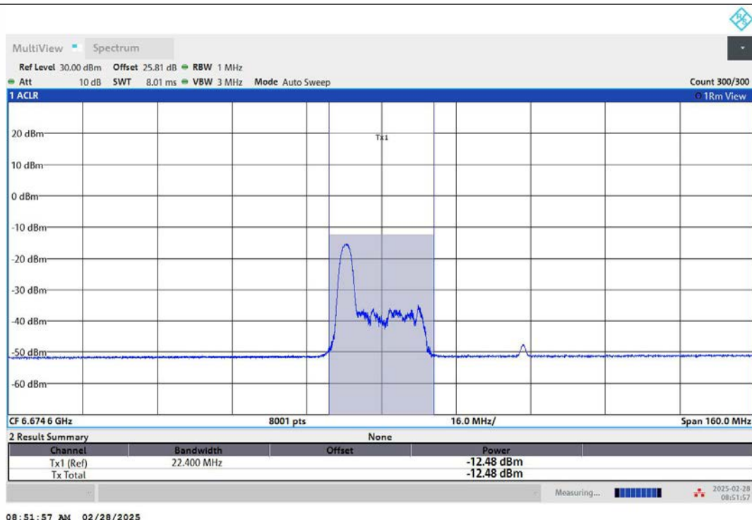
11AX80MIMO-Ant2-6705-26Tone-RU0-PASS
