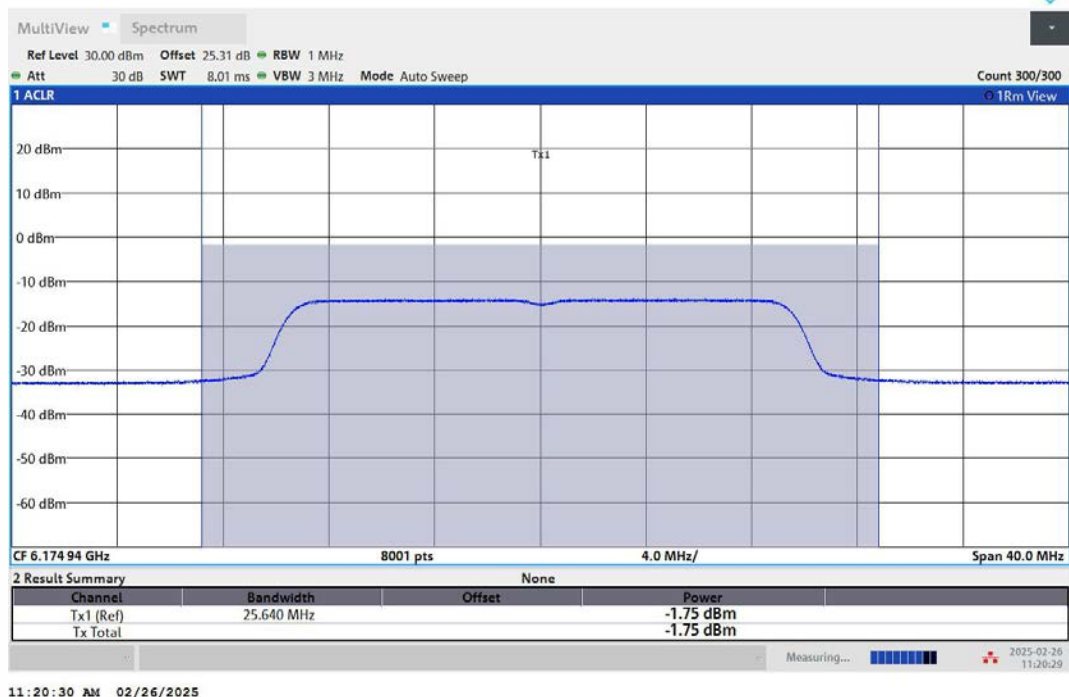
11AX20MIMO-Ant2-6175-PASS
