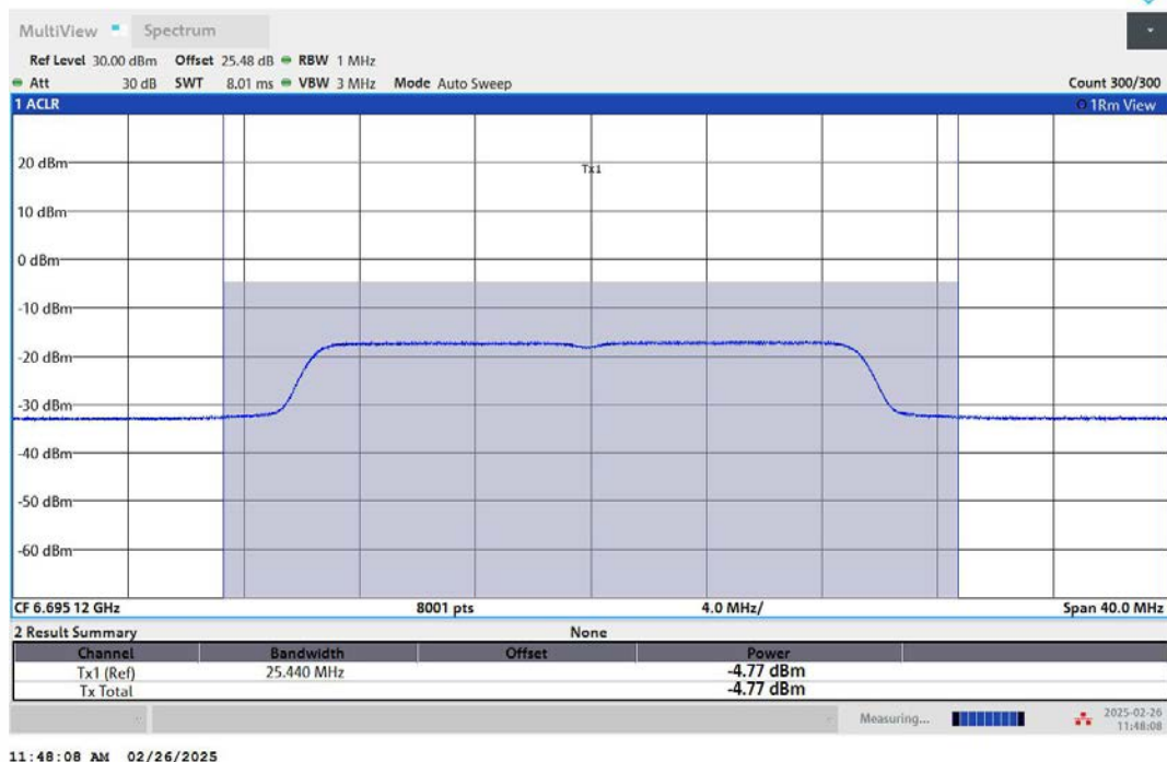
11AX20MIMO-Ant2-6695-PASS
