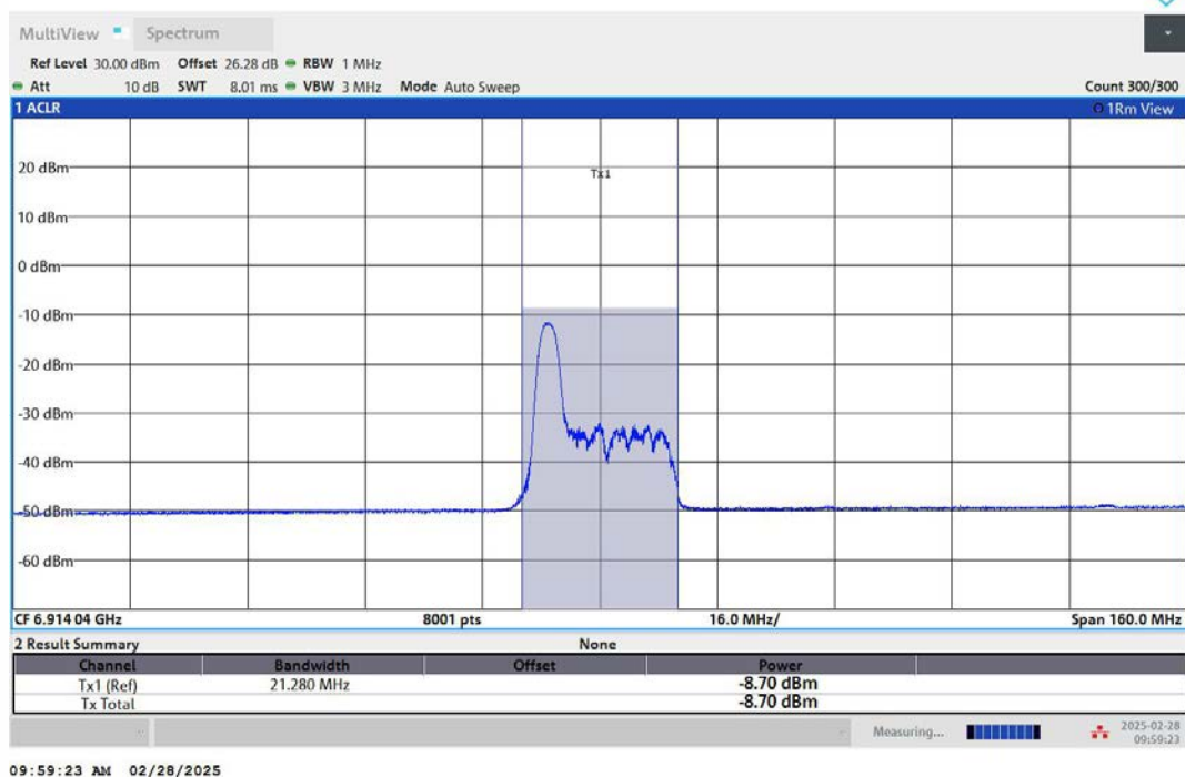
11AX80MIMO-Ant1-6945-52Tone-RU37-PASS
