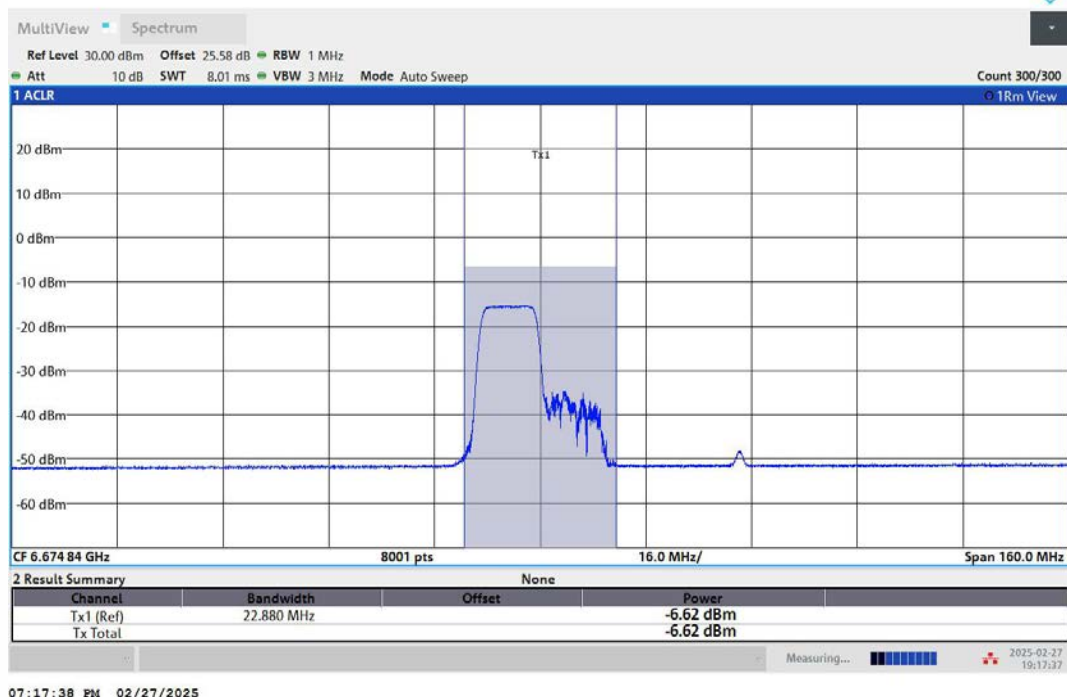
11AX80MIMO-Ant2-6705-106Tone-RU53-PASS
