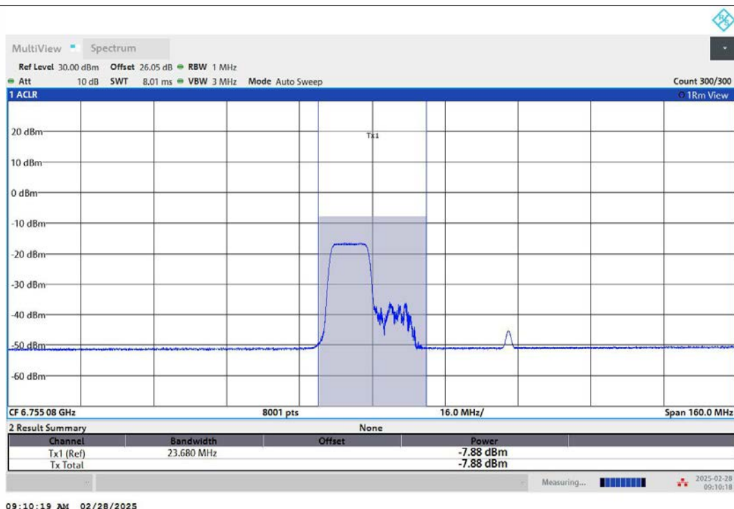
11AX80MIMO-Ant2-6785-106Tone-RU53-PASS
