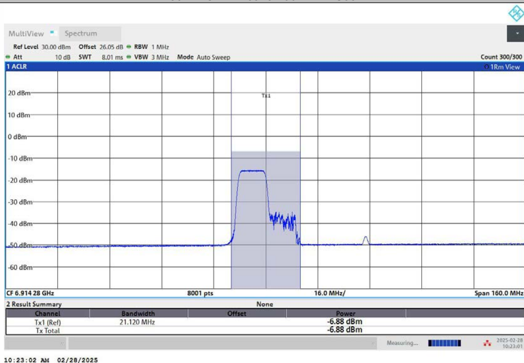
11AX80MIMO-Ant1-6945-242Tone-RU61-PASS
