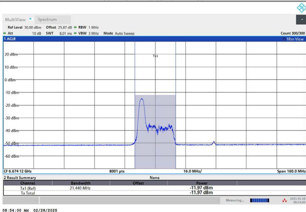
11AX80MIMO-Ant1-6705-52Tone-RU37-PASS
