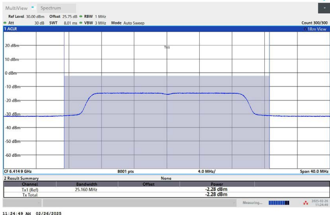
11AX20MIMO-Ant2-6415-PASS
