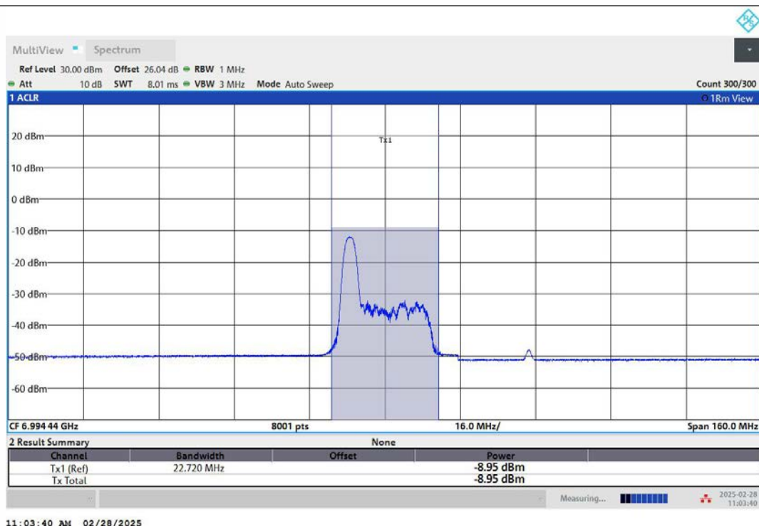
11AX80MIMO-Ant2-7025-26Tone-RU0-PASS
