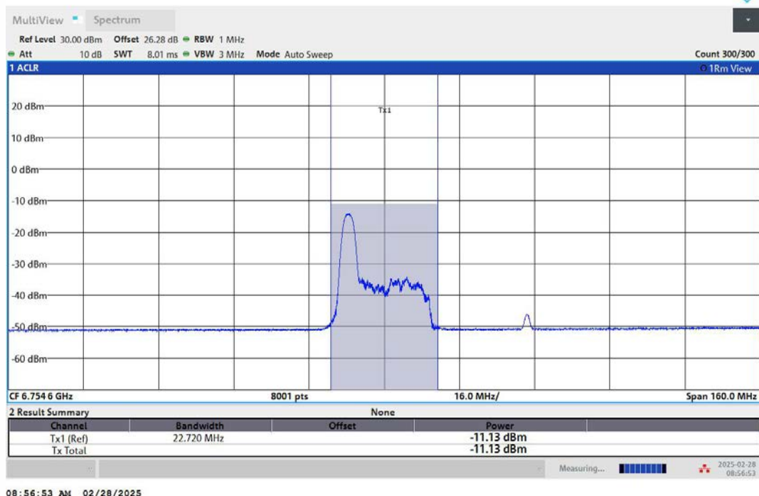
11AX80MIMO-Ant2-6785-26Tone-RU0-PASS
