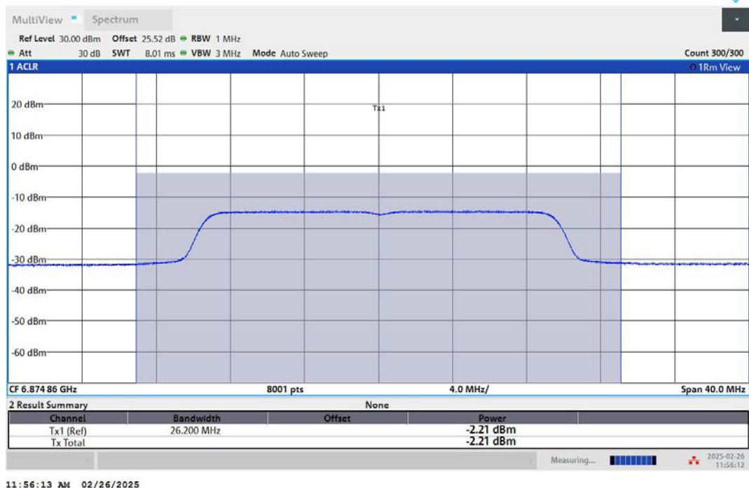
11AX20MIMO-Ant2-6875-PASS
