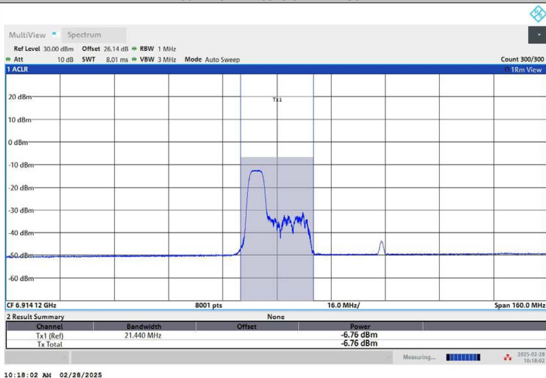
11AX80MIMO-Ant1-6945-106Tone-RU53-PASS
