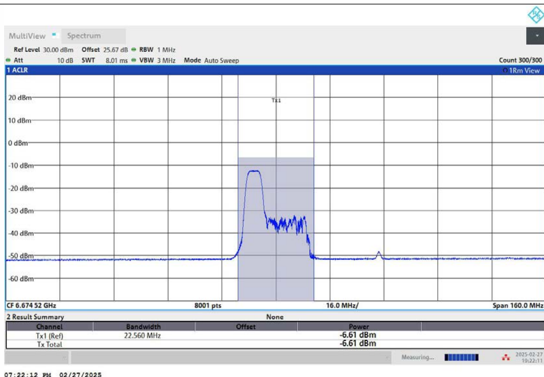
11AX80MIMO-Ant2-6705-52Tone-RU37-PASS
