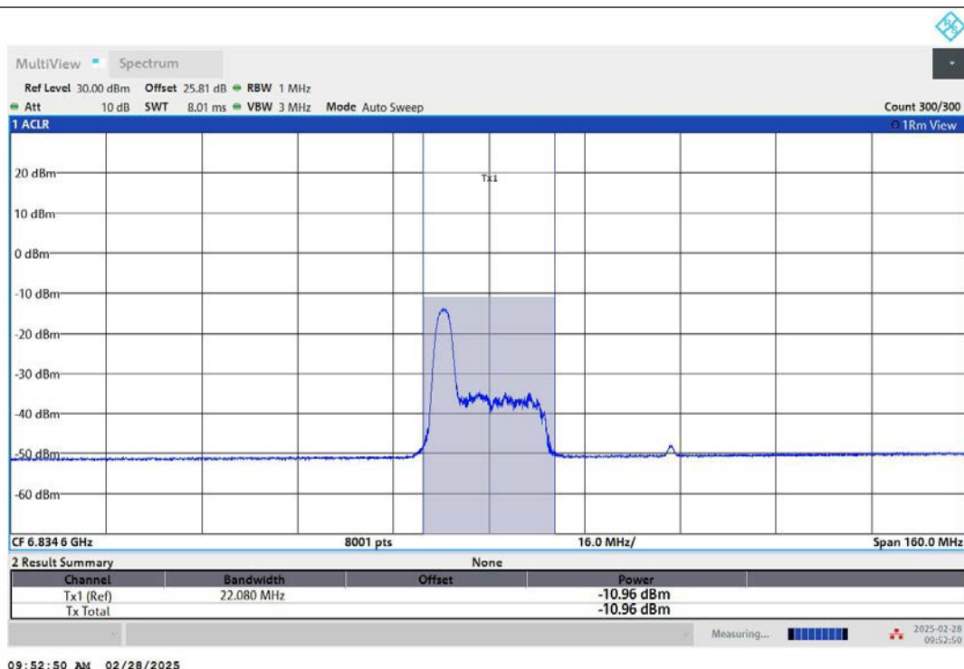
11AX80MIMO-Ant2-6865-26Tone-RU0-PASS
