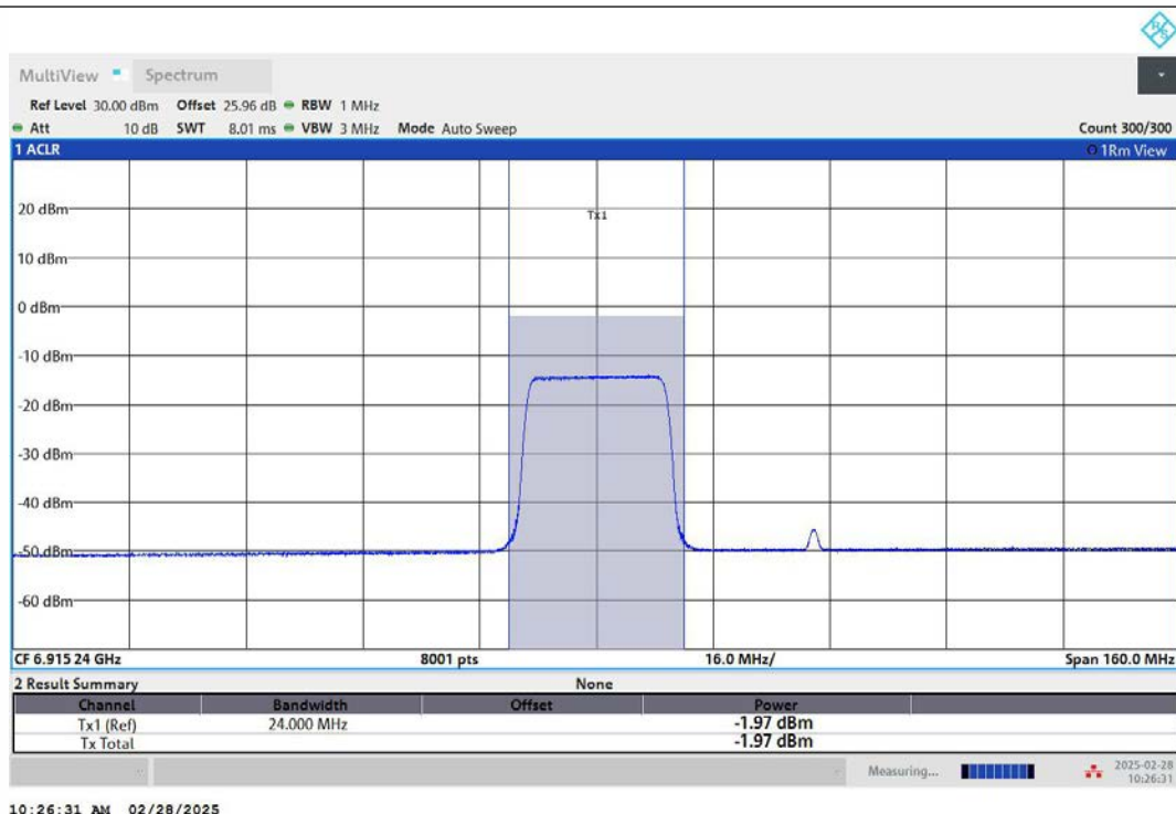
11AX80MIMO-Ant2-6945-242Tone-RU61-PASS
