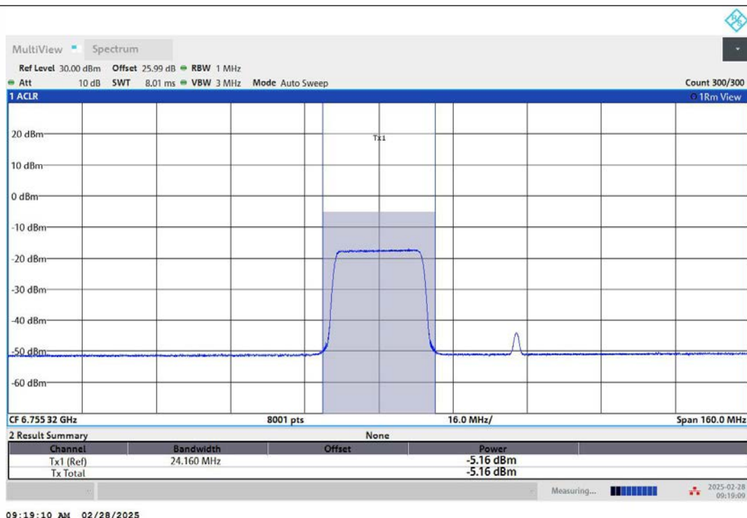
11AX80MIMO-Ant2-6785-242Tone-RU61-PASS
