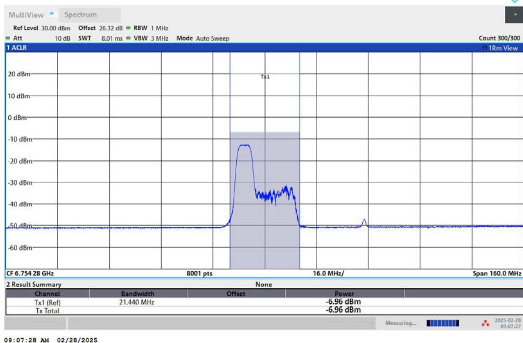
11AX80MIMO-Ant1-6785-106Tone-RU53-PASS
