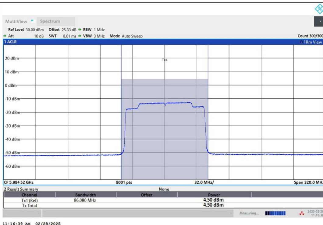
11AX160MIMO-Ant2-6025-996Tone-RU67-PASS
