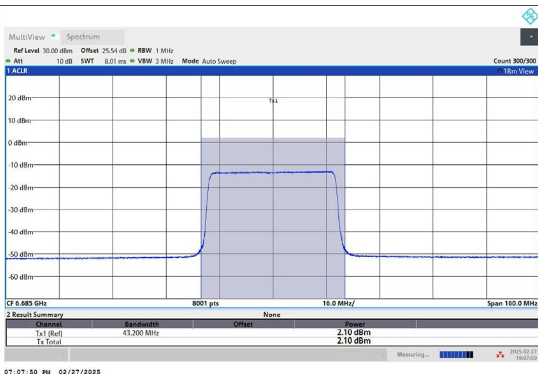
11AX80MIMO-Ant2-6705-484Tone-RU65-PASS
