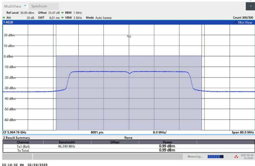
11AX40MIMO-Ant2-5965-PASS
