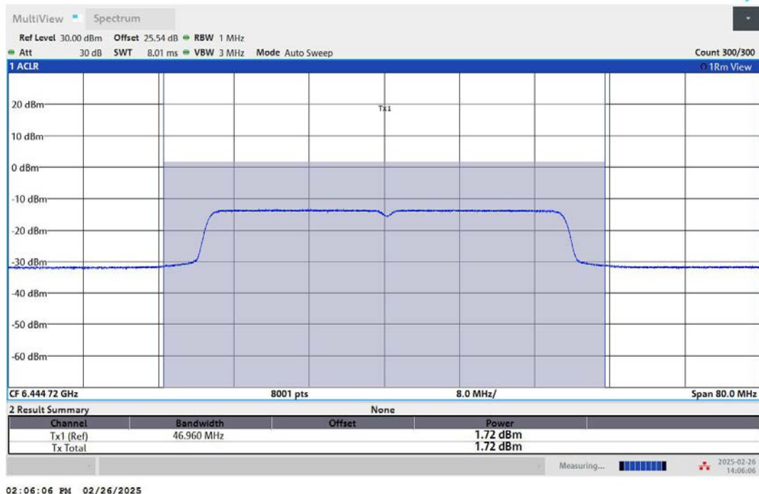
11AX40MIMO-Ant2-6445-PASS
