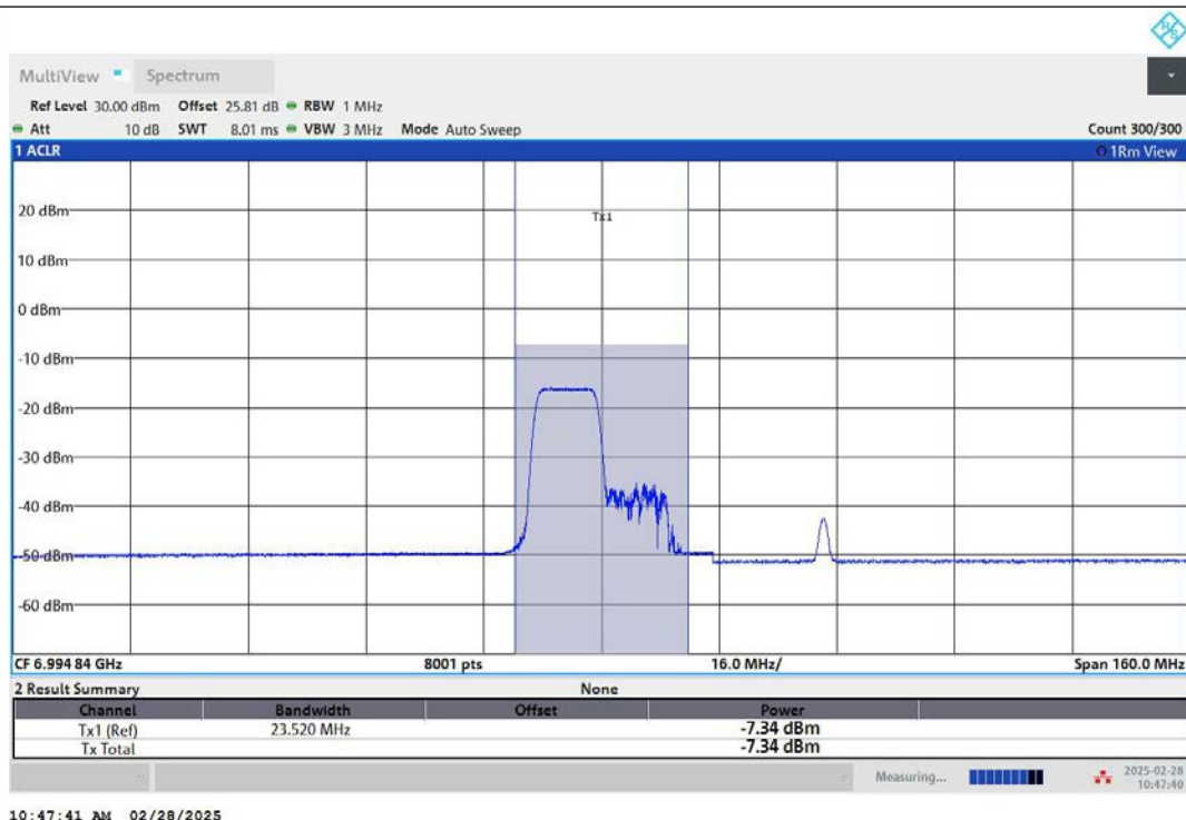
11AX80MIMO-Ant2-7025-106Tone-RU53-PASS
