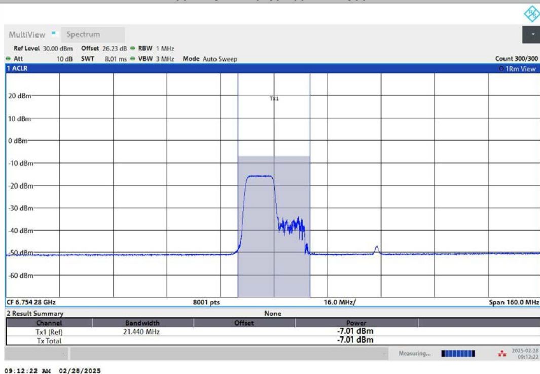
11AX80MIMO-Ant1-6785-242Tone-RU61-PASS
