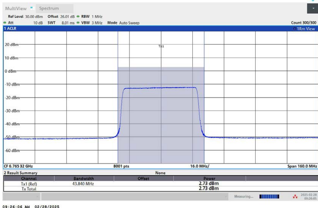
11AX80MIMO-Ant2-6785-484Tone-RU65-PASS
