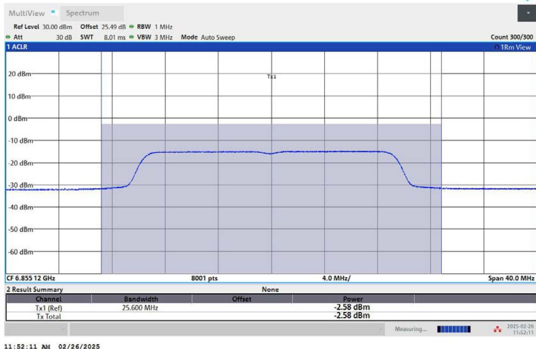
11AX20MIMO-Ant2-6855-PASS
