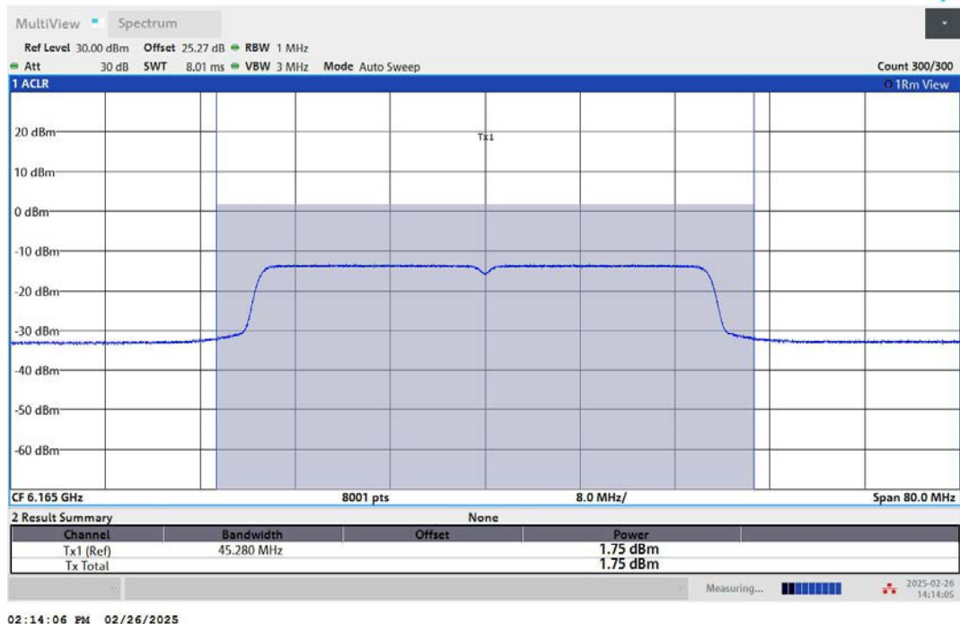
11AX40MIMO-Ant2-6165-PASS
