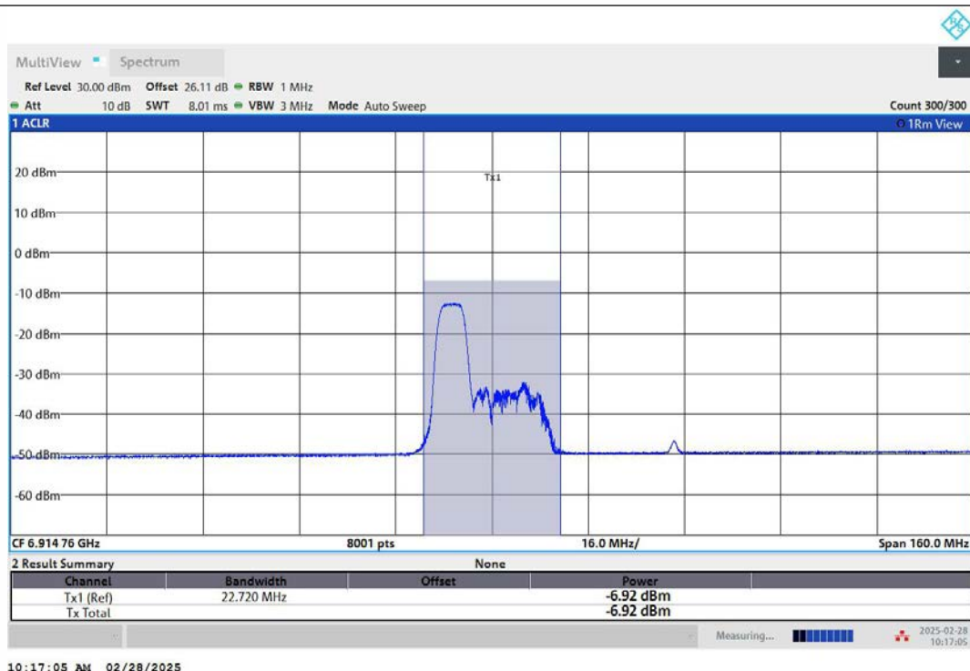
11AX80MIMO-Ant2-6945-52Tone-RU37-PASS
