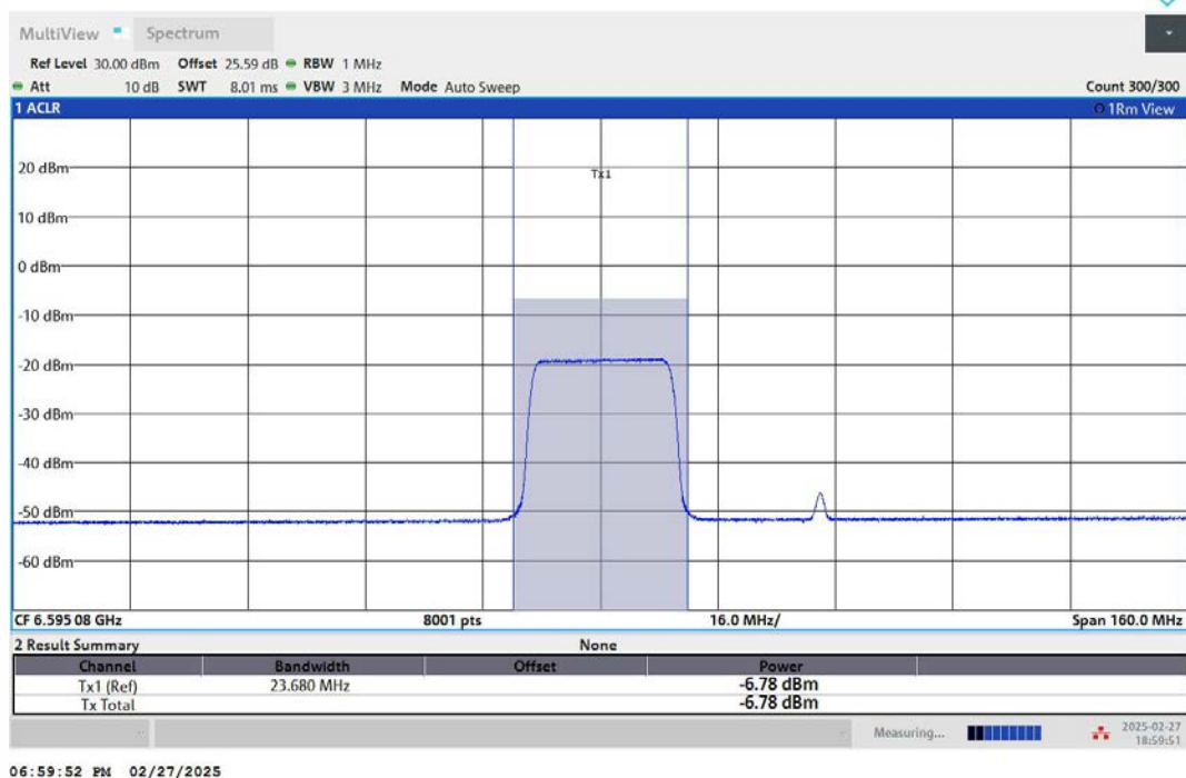
11AX80MIMO-Ant1-6625-484Tone-RU65-PASS
