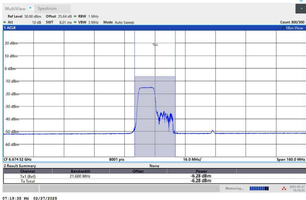
11AX80MIMO-Ant1-6705-242Tone-RU61-PASS
