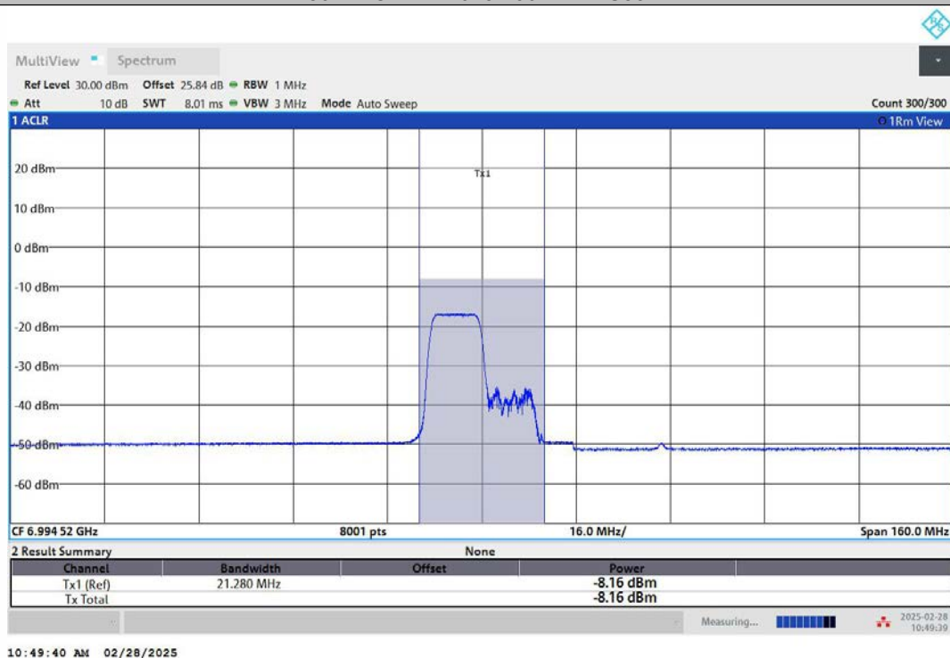
11AX80MIMO-Ant1-7025-242Tone-RU61-PASS
