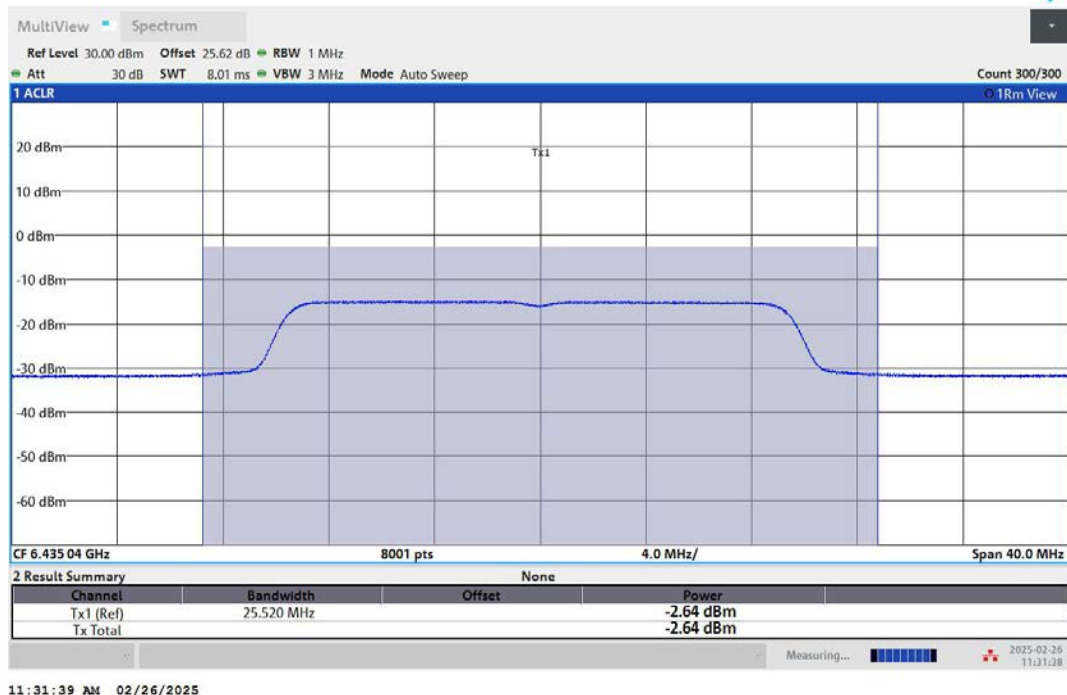
11AX20MIMO-Ant2-6435-PASS
