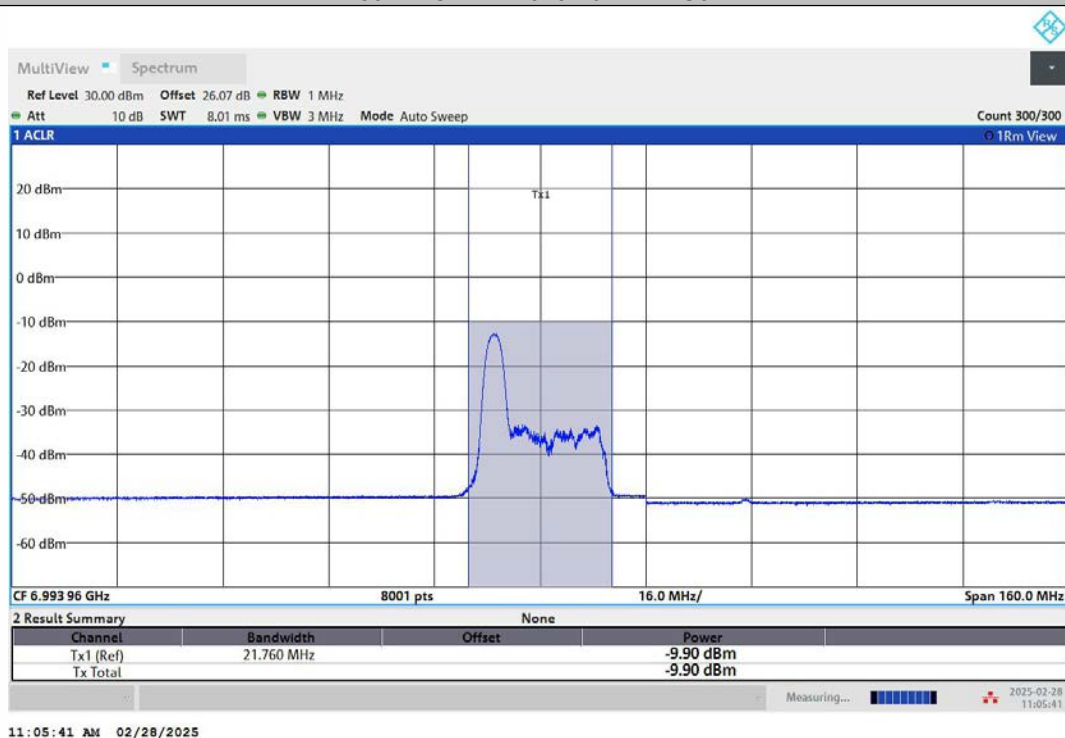
11AX80MIMO-Ant1-7025-52Tone-RU37-PASS
