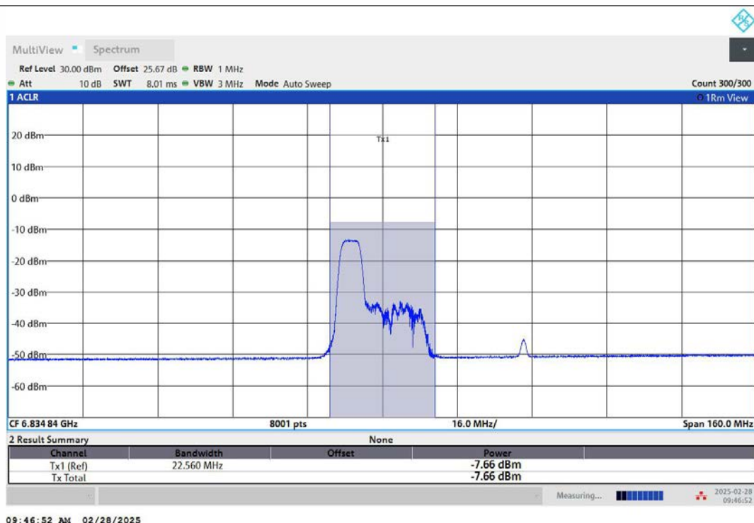
11AX80MIMO-Ant2-6865-52Tone-RU37-PASS
