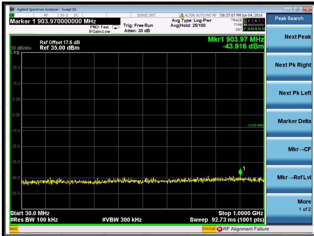
(Plot H2: WCDMA1700MHz Channel = 1412, 30MHz to 1GHz)
