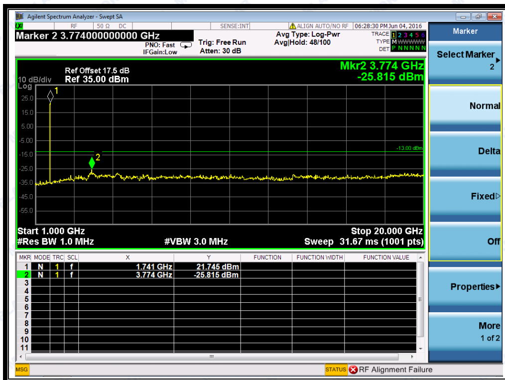
(Plot H2.1: WCDMA1700MHz Channel = 1412, 1GHz to 20GHz)
