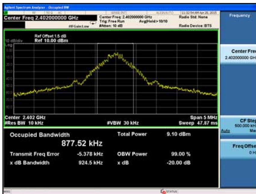
Channel 00 (2402MHz)
