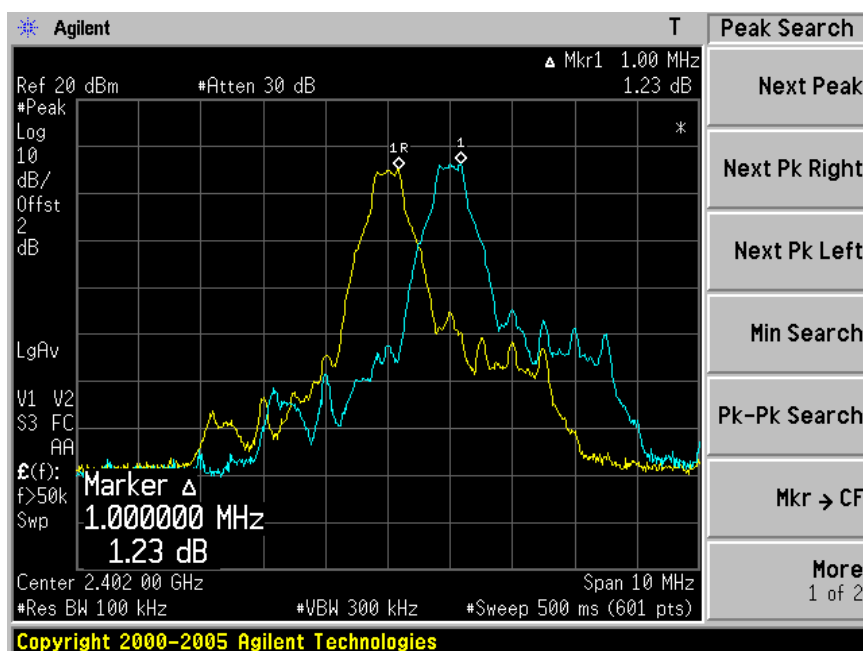
Channel 00 (2402MHz)
