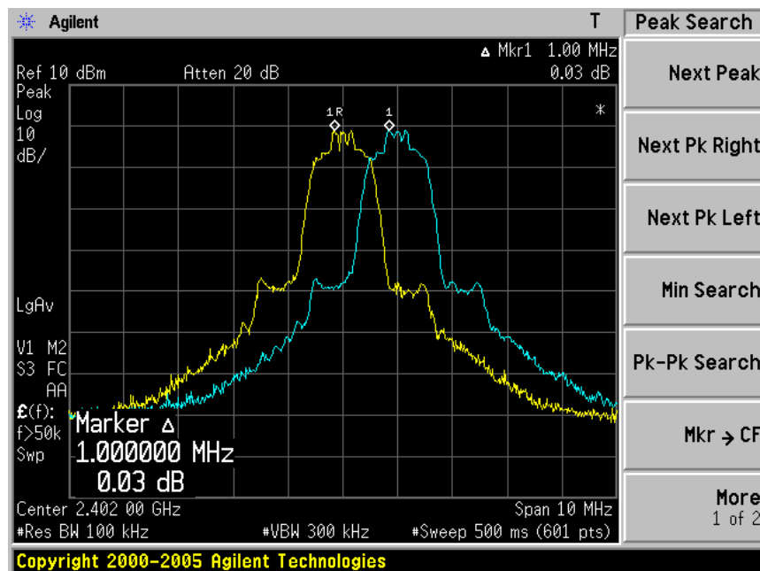
Channel 00 (2402MHz)
