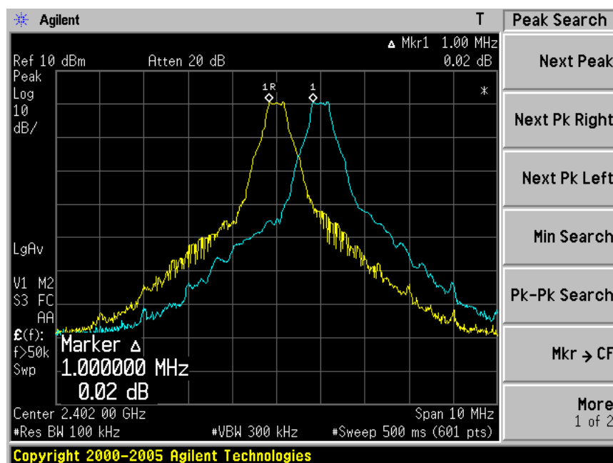
Channel 00 (2402MHz)
