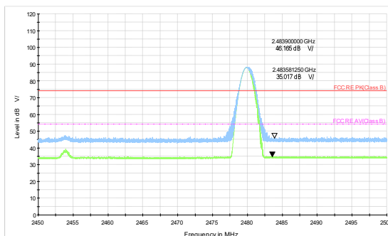
DH5-Channel 78: Peak + Average
