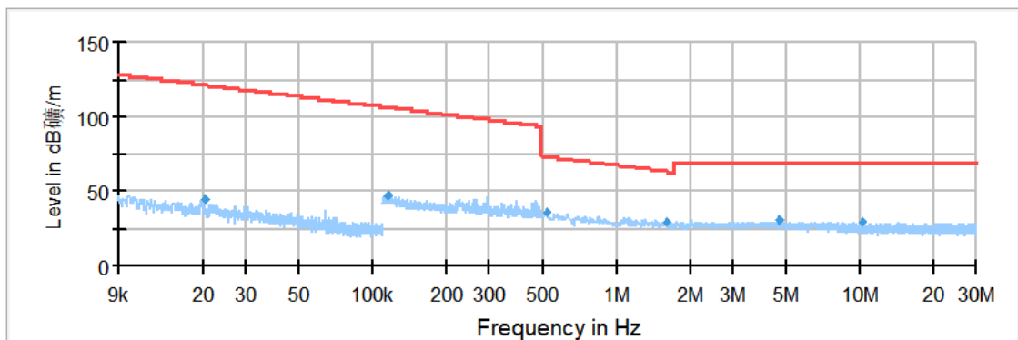
Radiates Emission from 9kHz to 30MHz
