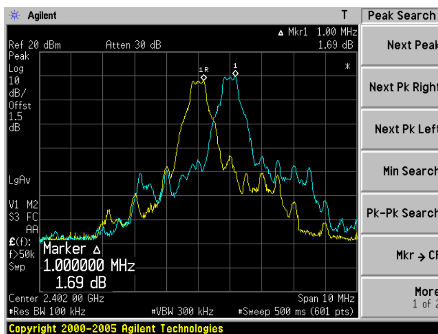
Channel 00 (2402MHz)
