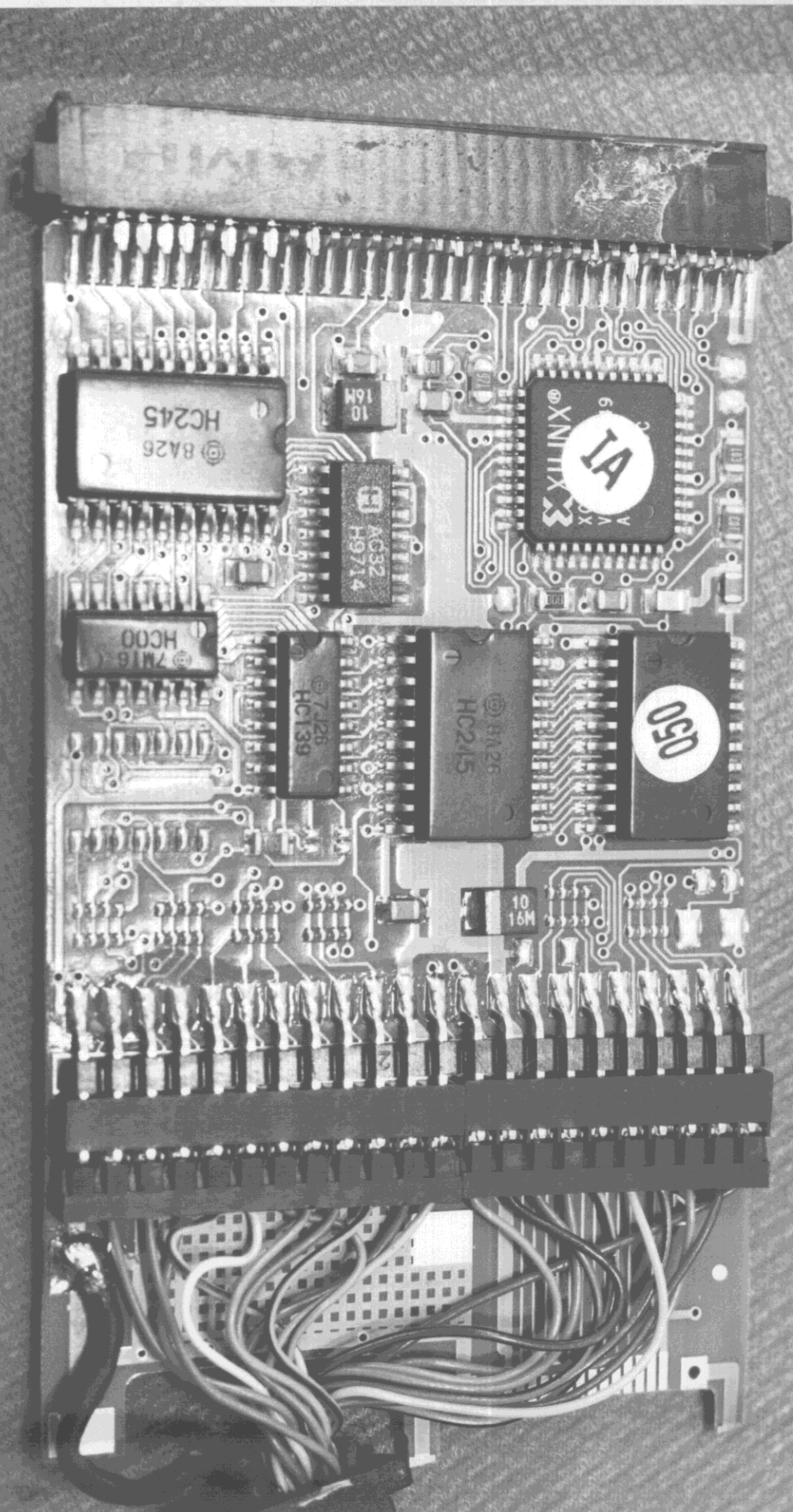
PHOTO 12. PCMCIA CARD COMPONENT SIDE VIEW
