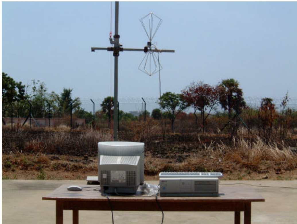
Radiated Emission (Vertical Polarisation)
