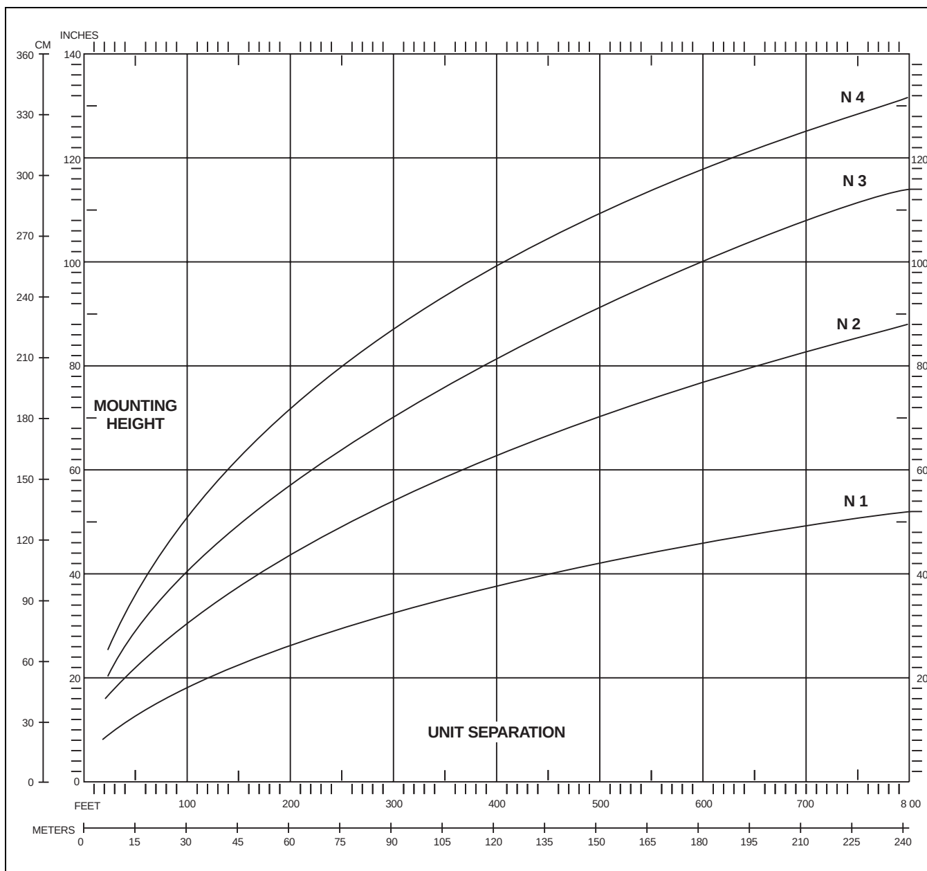
Figure 3-4: Mounting height chart
