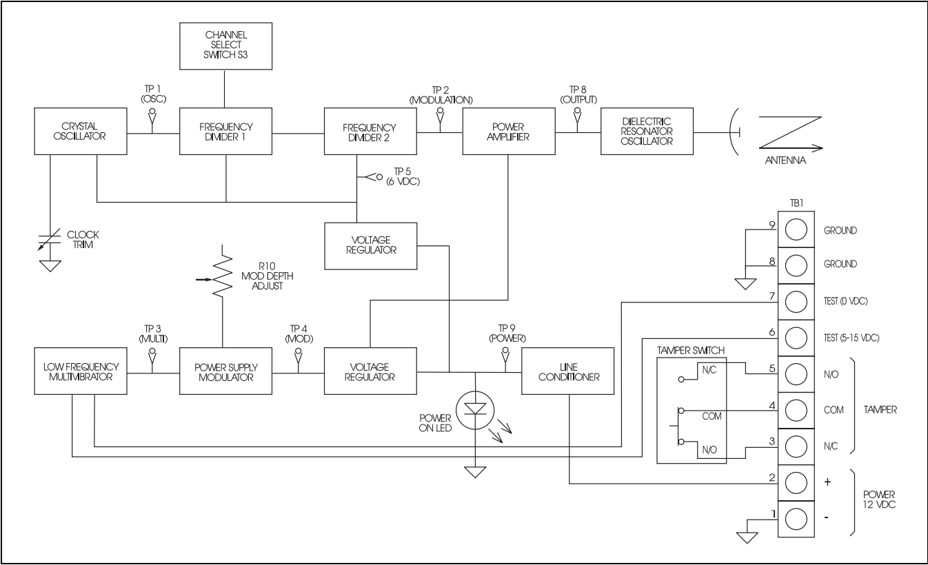
Figure 5-4: Transmitter block diagram
