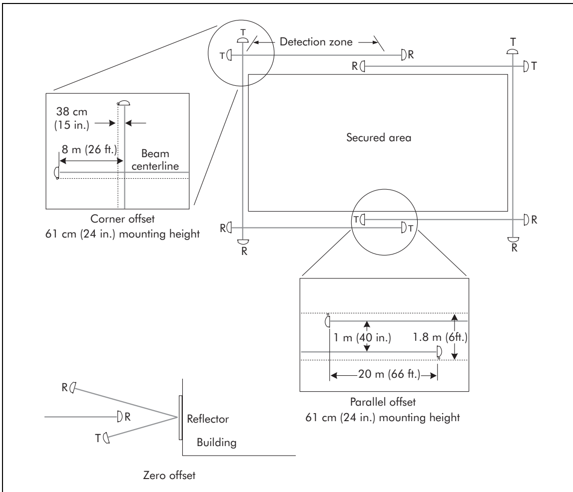
Figure 2-2: Offset arrangements - high-security application
