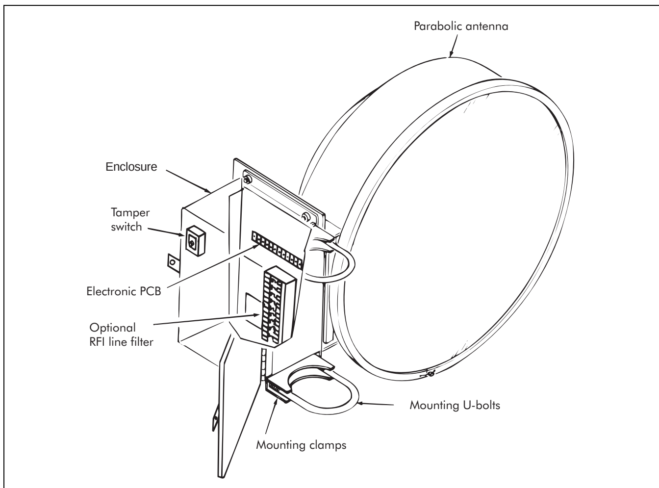
Figure 3-1: Series 14000 microwave unit
