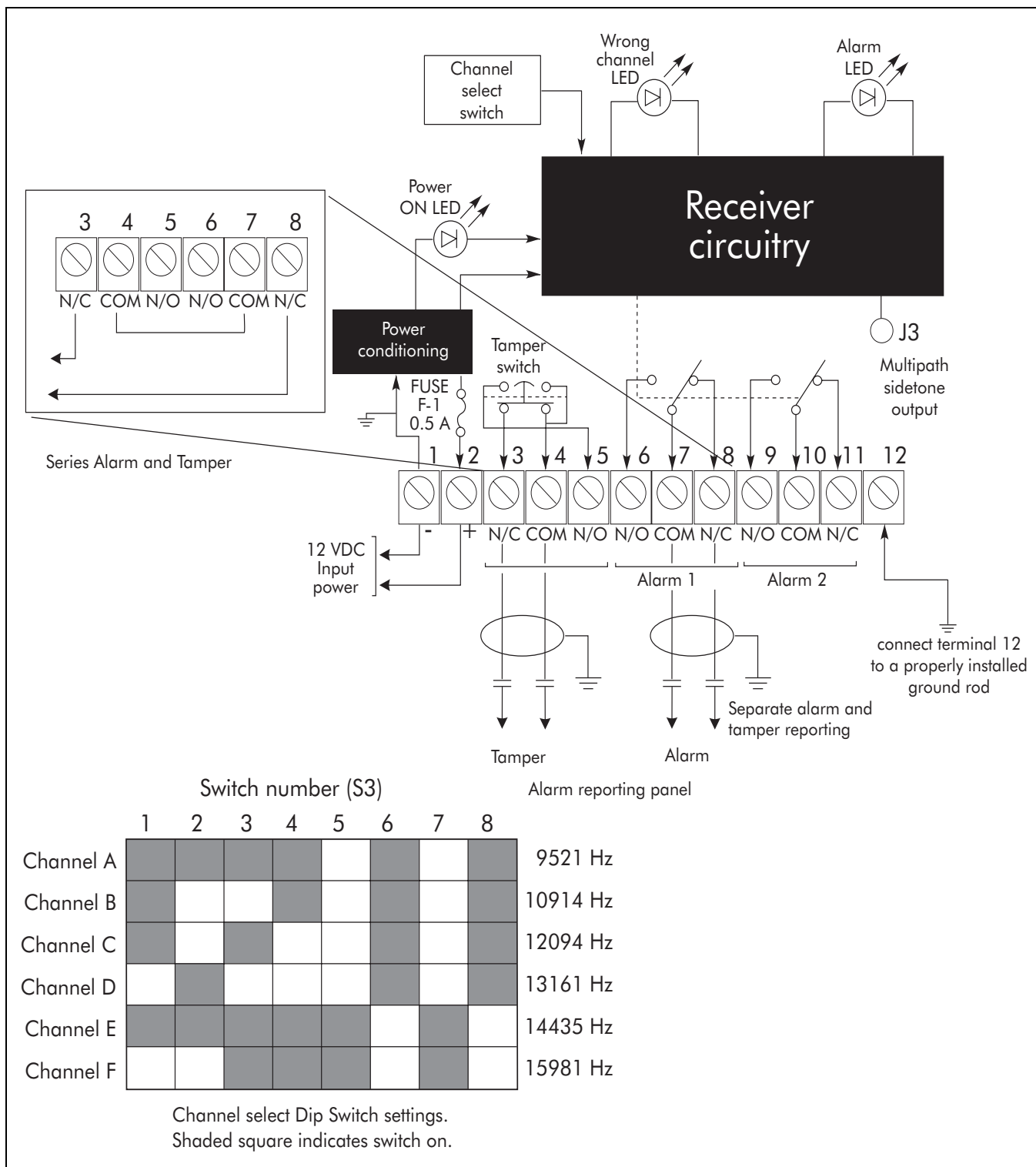
Figure 3-6: Receiver wiring
