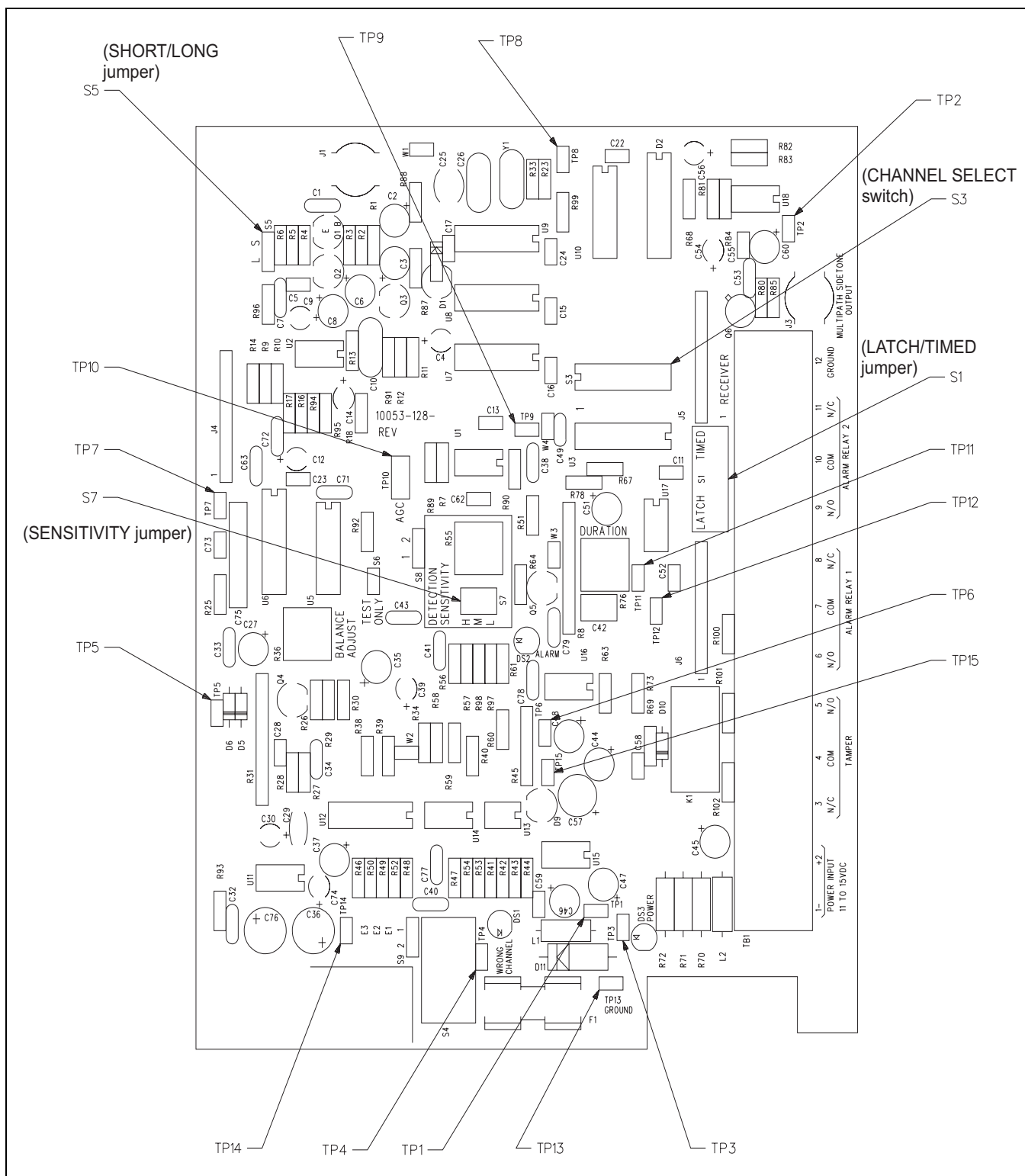
Figure 5-1: Receiver PCB
