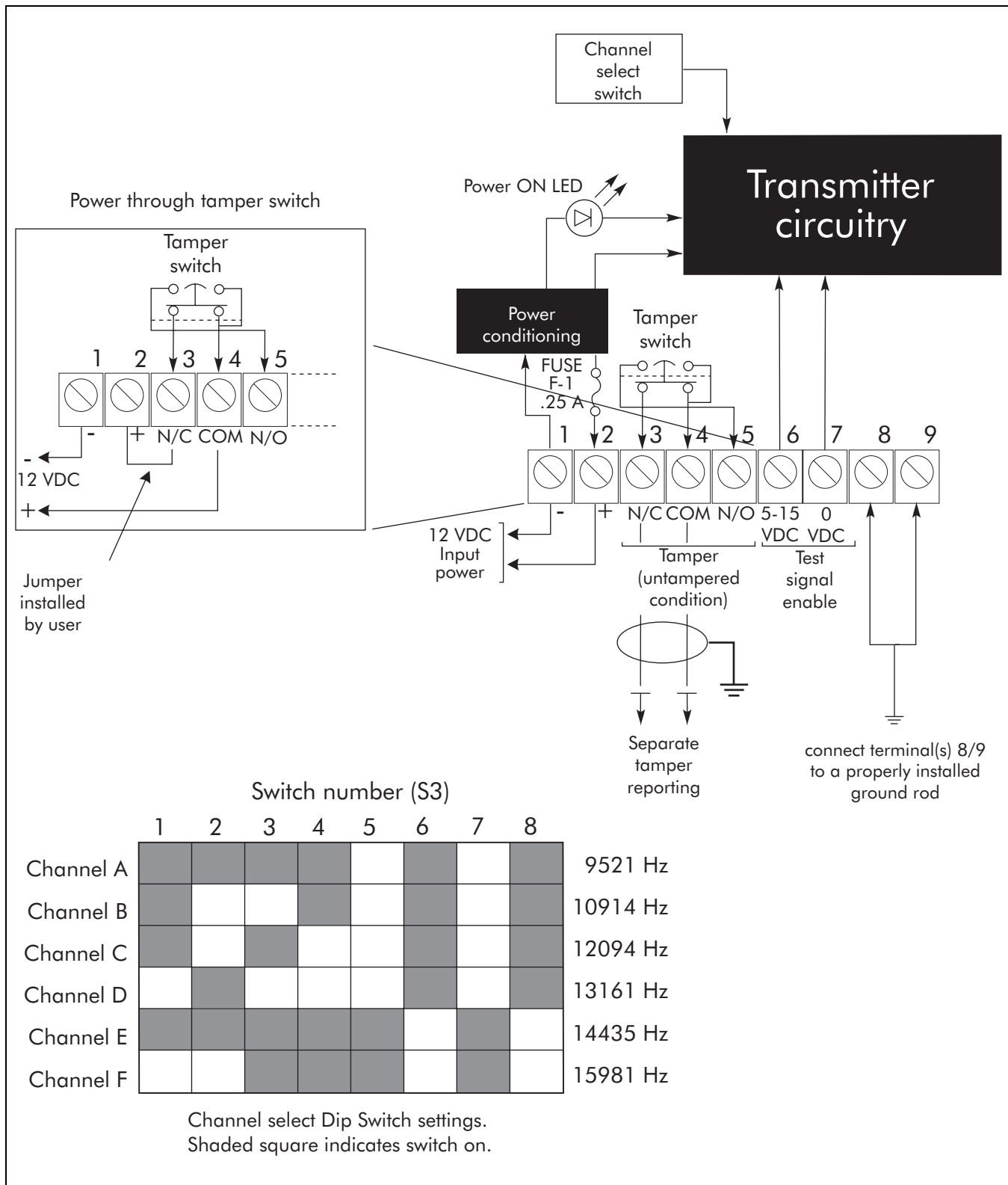
Figure 3-5: Transmitter wiring
