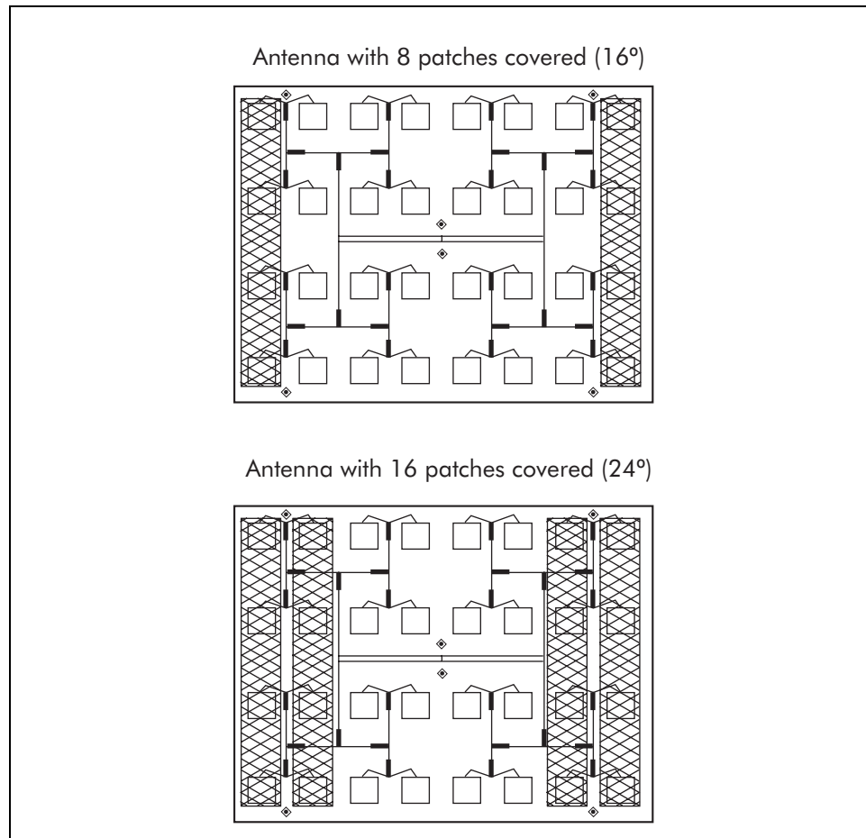
Figure 4-1: Antenna patterns
