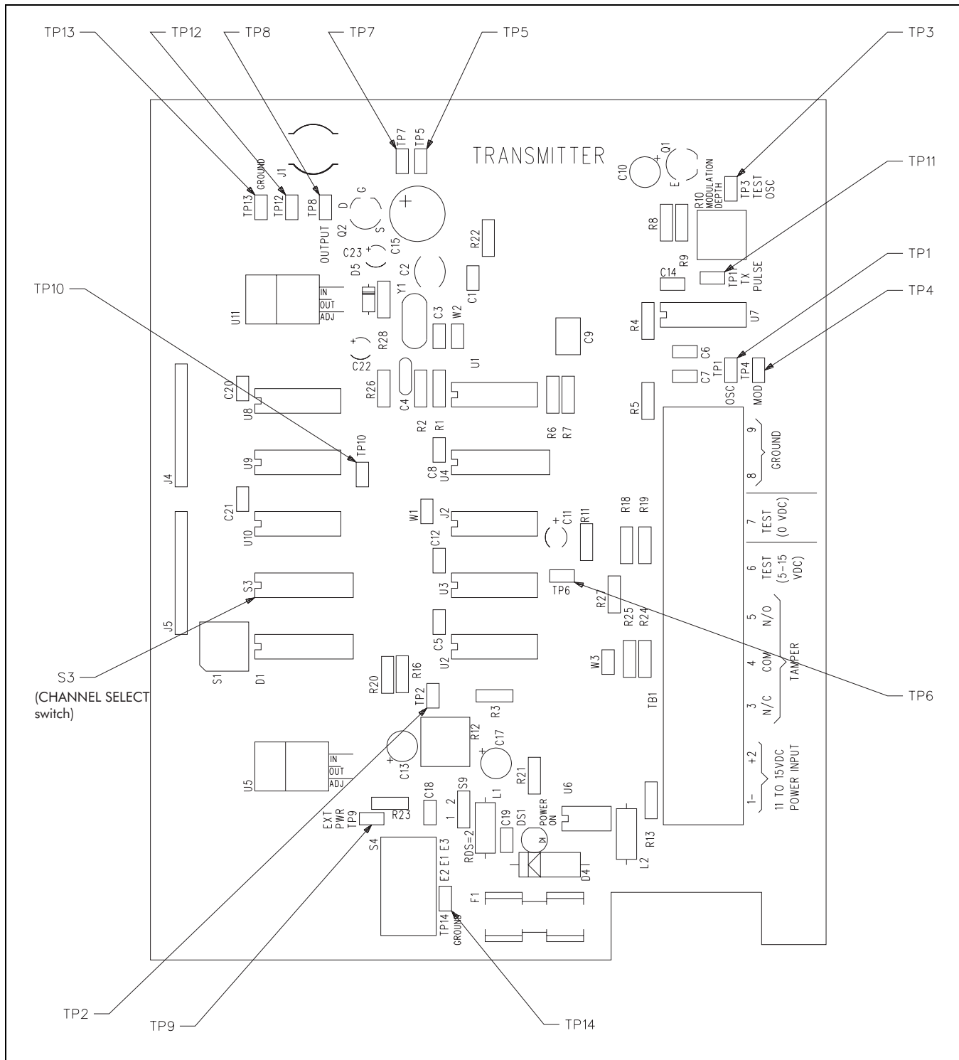
Figure 5-2: Transmitter PCB
