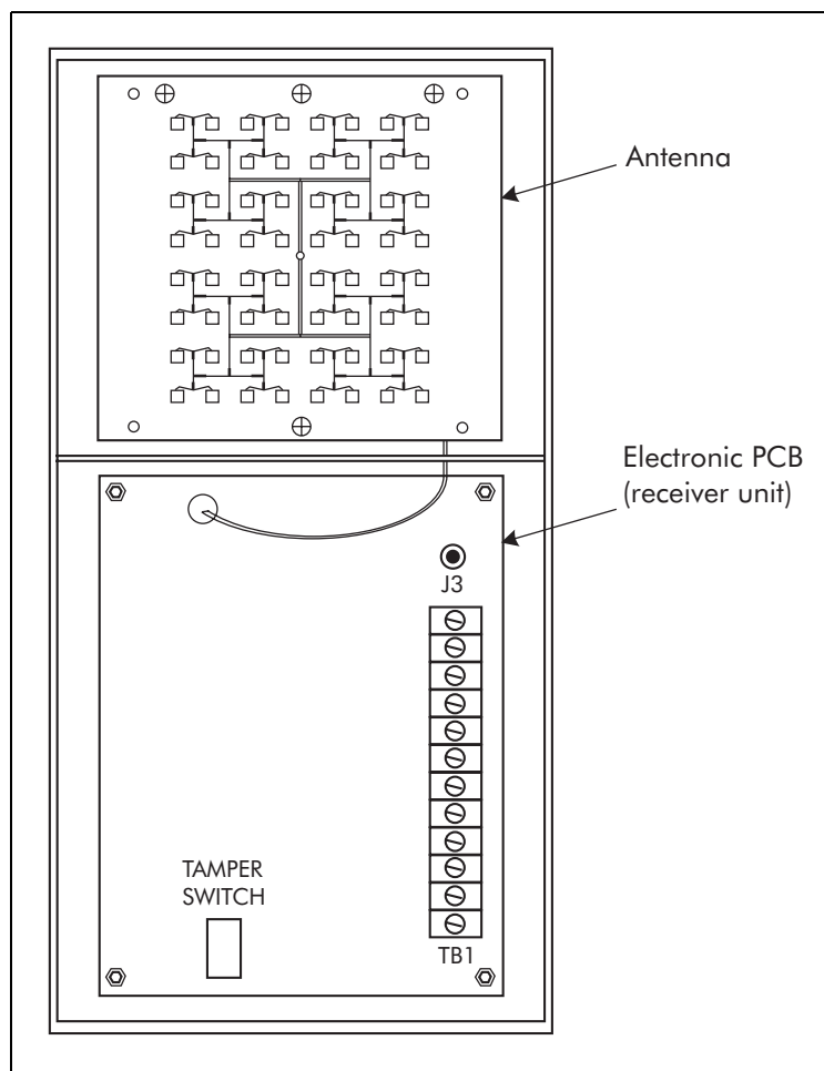
Figure 3-1: Series 24000 microwave unit (receiver)
