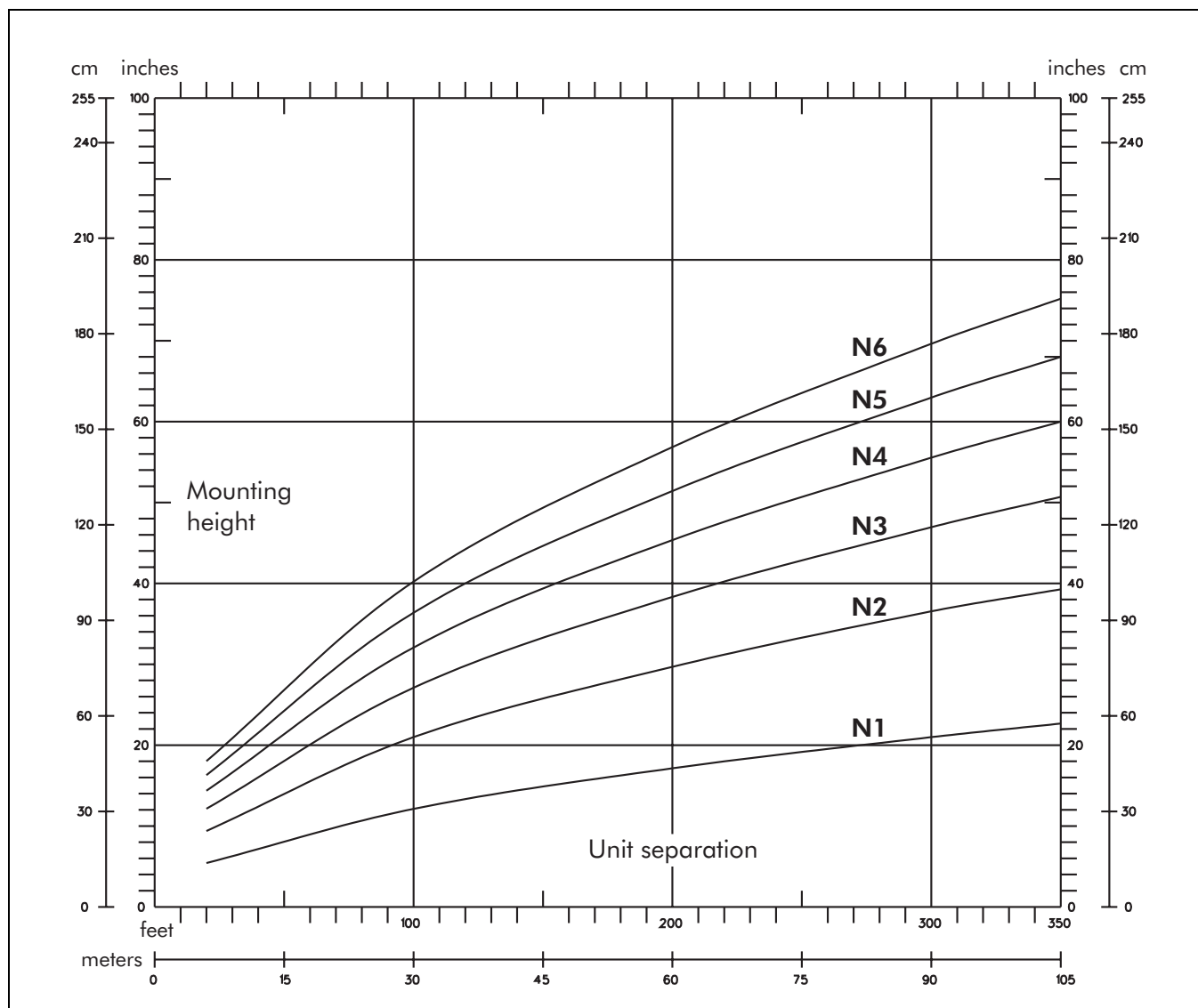
Figure 3-3: Mounting height chart
