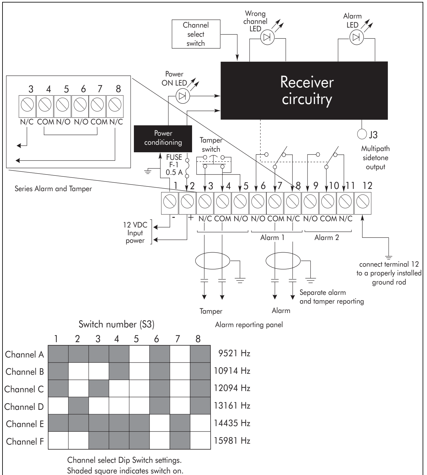
Figure 3-5: Receiver wiring
