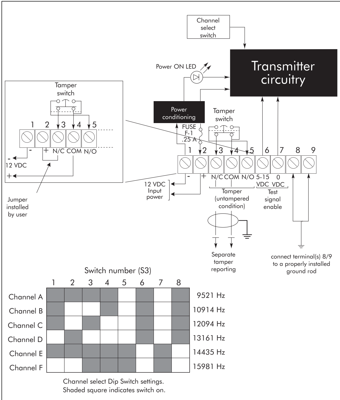
Figure 3-4: Transmitter wiring
