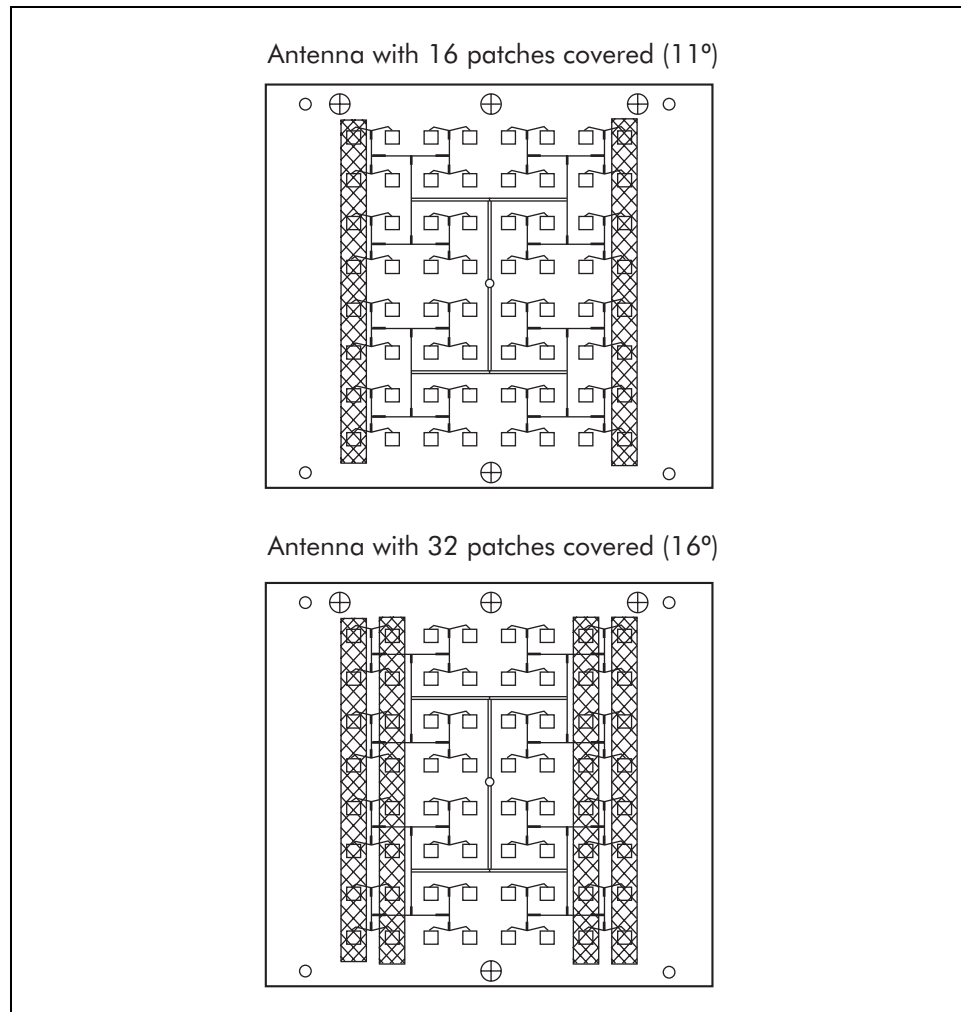
Figure 4-1: Antenna patterns
