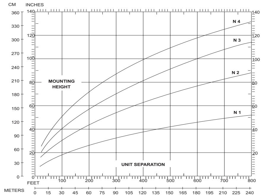
Chart 1: X-band sensor
