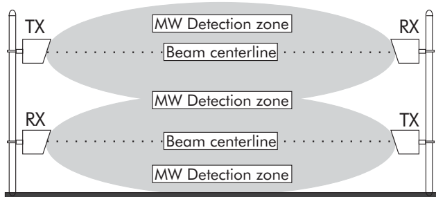
Figure 1: Stacked standalone microwave detection zones
