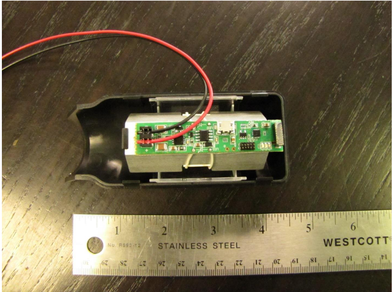
PCB Mounted on LED / Heatsink Assembly and Lower Cover
