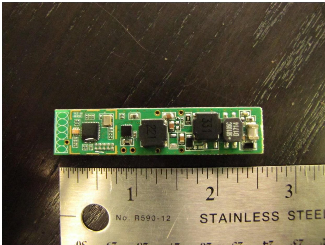
PCB Bottom Side View
