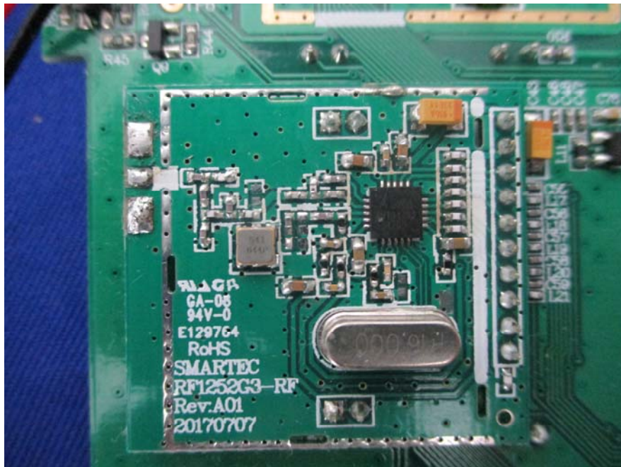
EUT – 915MHz Module View
