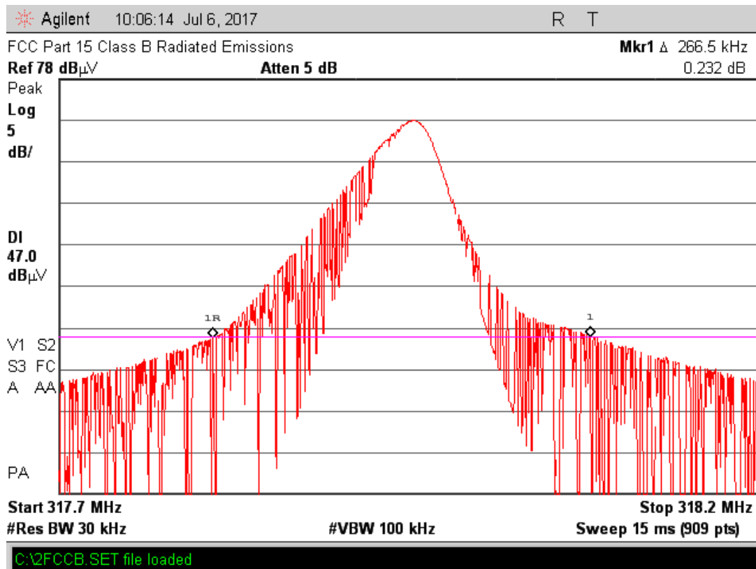
Figure 2.1.9-2 - 99% Occupied Bandwidth
