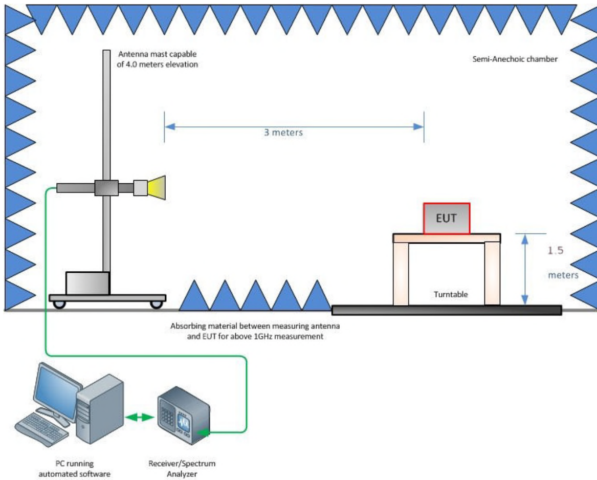
Figure 4.1-2 - Radiated Emission Test Setup (Above 1GHz)
