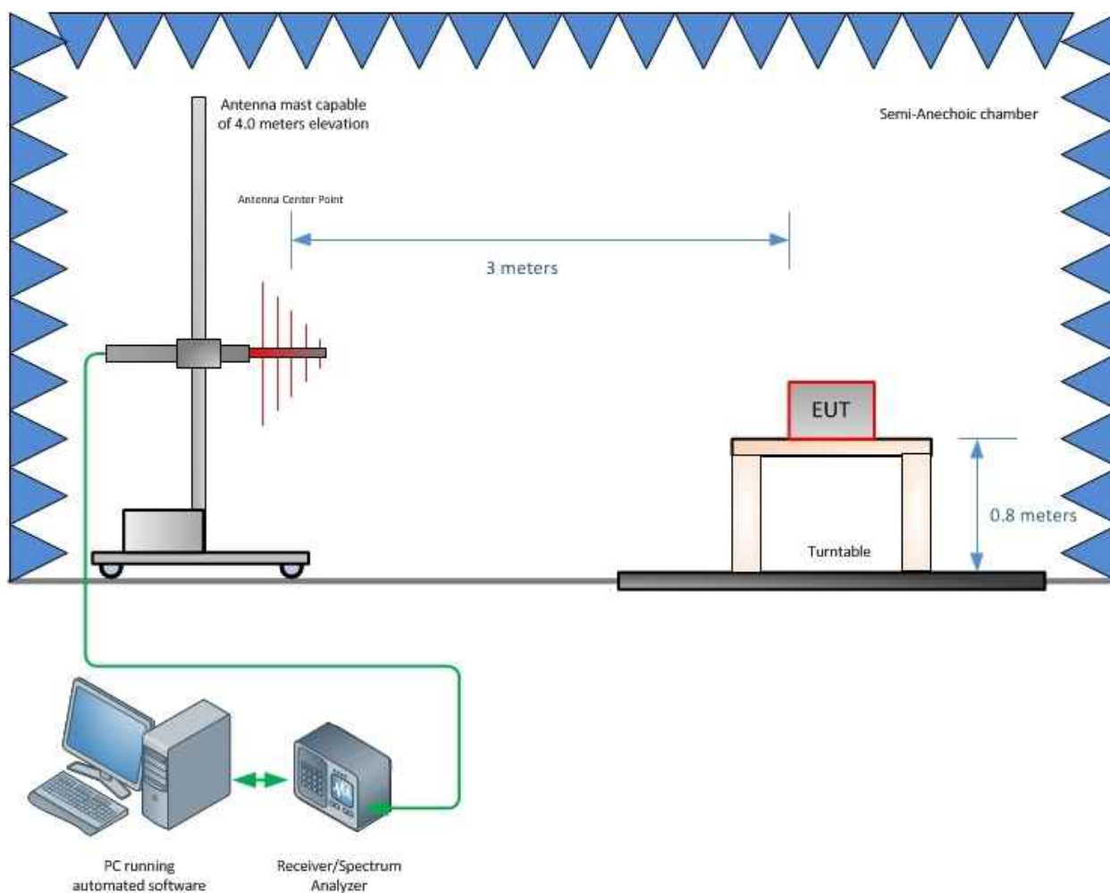
Figure 4.1-1 - Radiated Emission Test Setup (Below 1 GHz)
