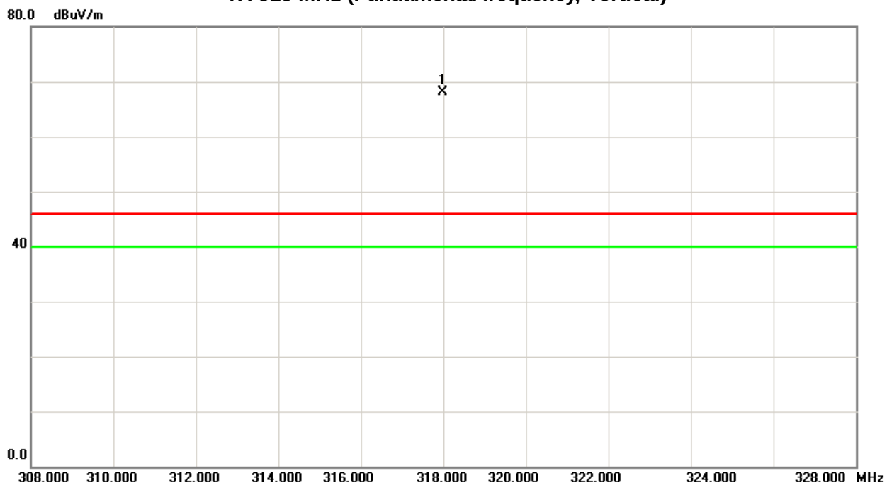
Orthogonal Axis: X TX 318 MHz (Fundamental frequency, Vertical)
