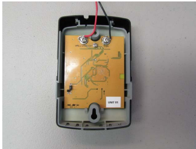
Figure 3: Back with PCB
