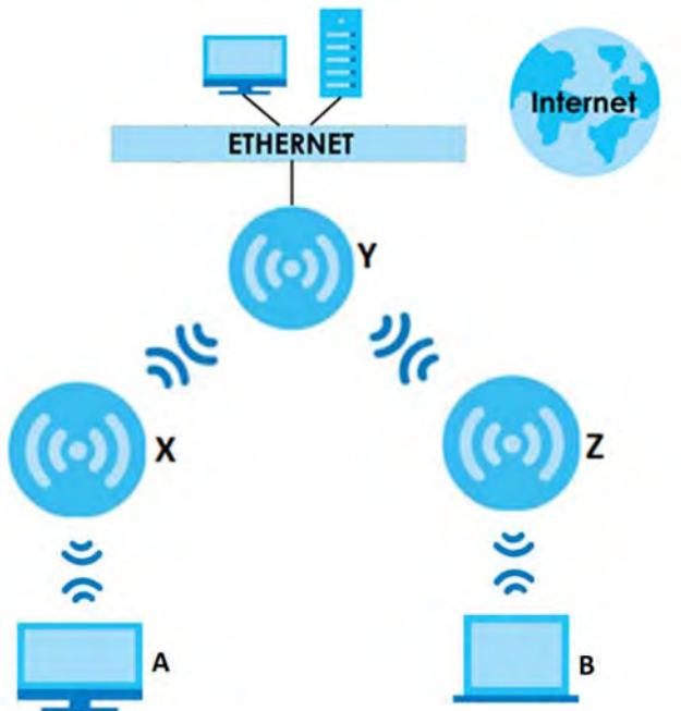
Figure 2 Wireless Distribution System Network Example
