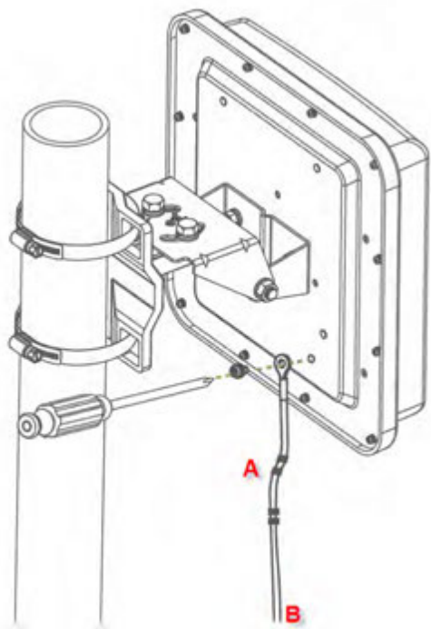
Figure 15 Grounding Example
