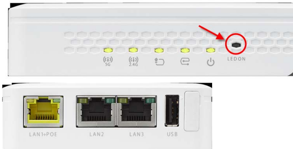
Figure 24 NWA1302-AC LEDs
