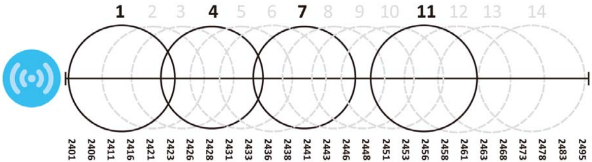
Figure 85 An Example Four-Channel Deployment
