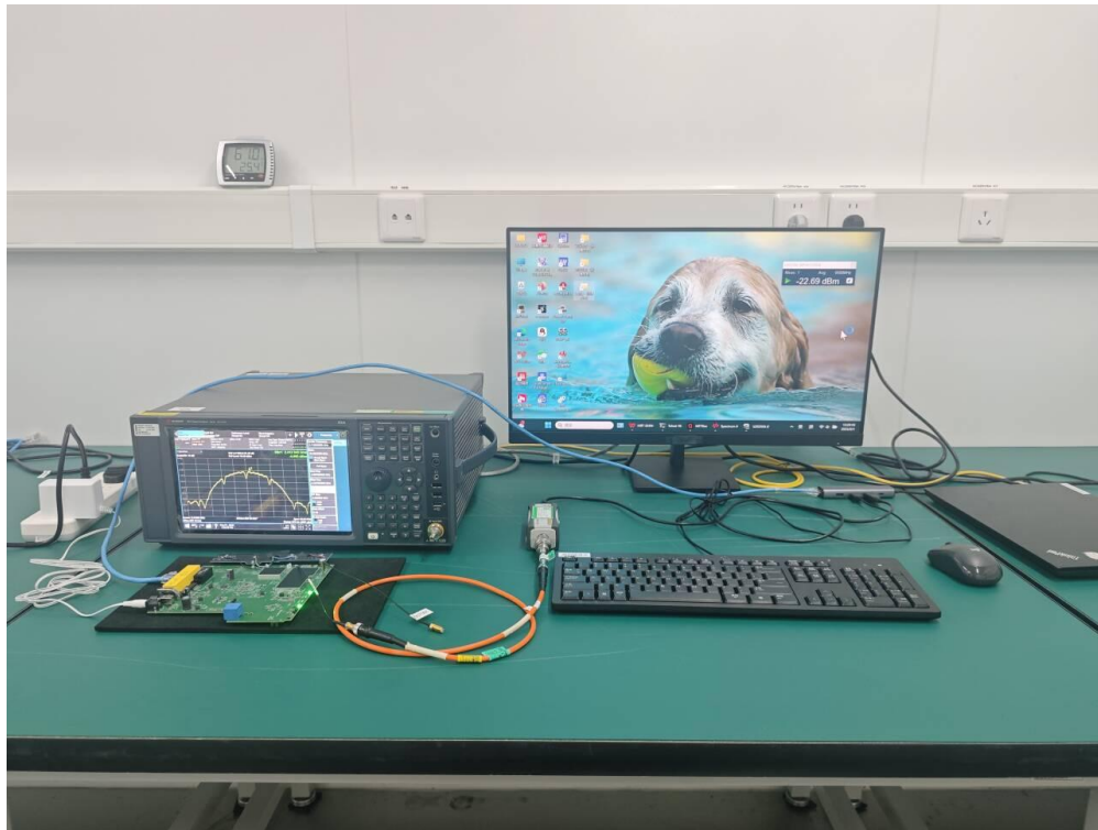
Description: Dynamic Frequency Selection Test Setup (WJ-SR7)
