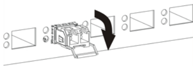
Figure 29 Transceiver Removal Example
