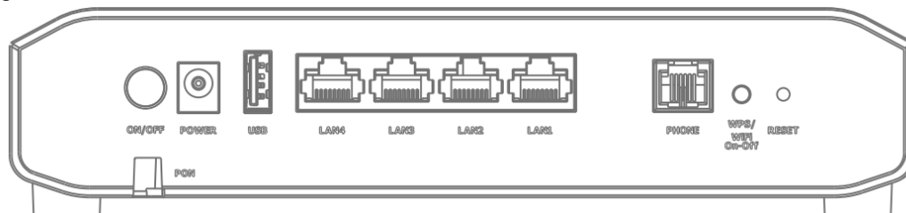
Figure 52 PX5311-T0
