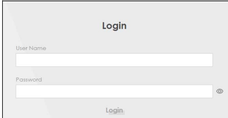
Figure 59 Login Screen
