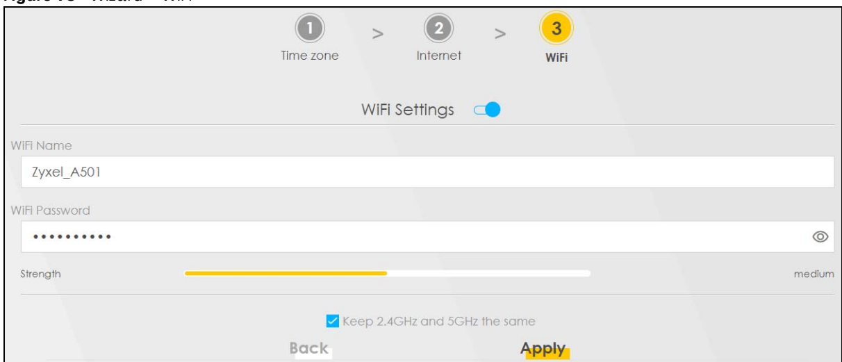
Figure 73 Wizard – WiFi
