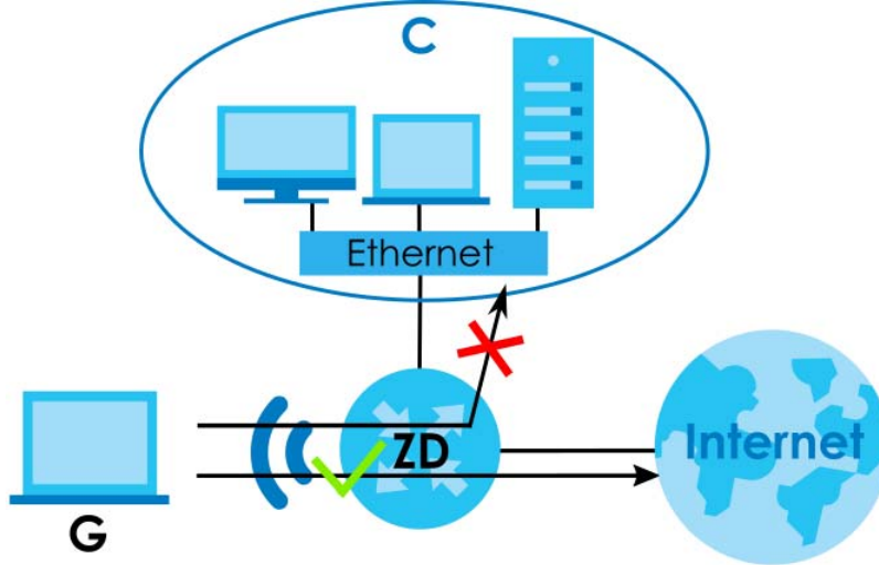
Figure 83 Visiting Guests Blocked from Company Network
