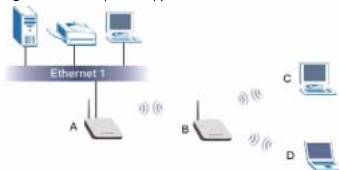
Figure 7 AP+Repeater Application
