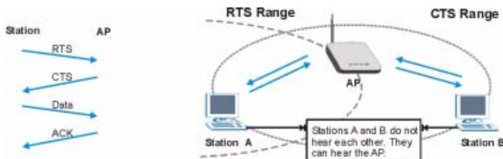
Figure 35 RTS/CTS
