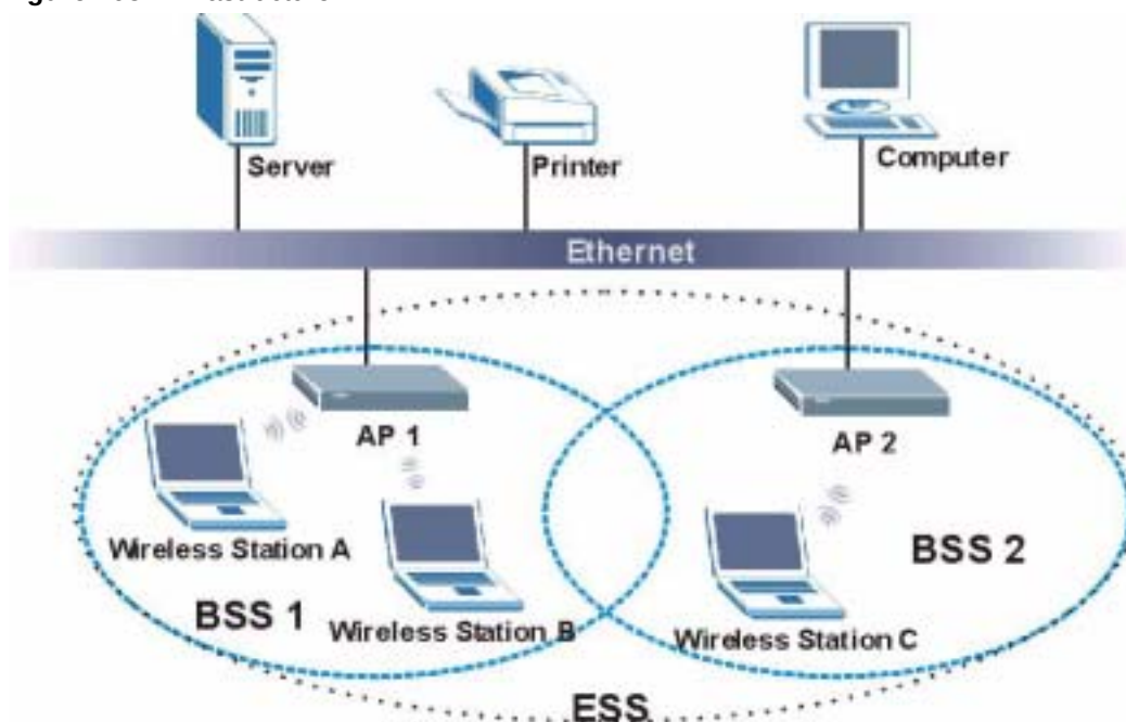
Figure 105 Infrastructure WLAN
