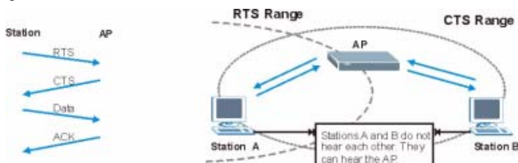
Figure 106 RTS/CTS
