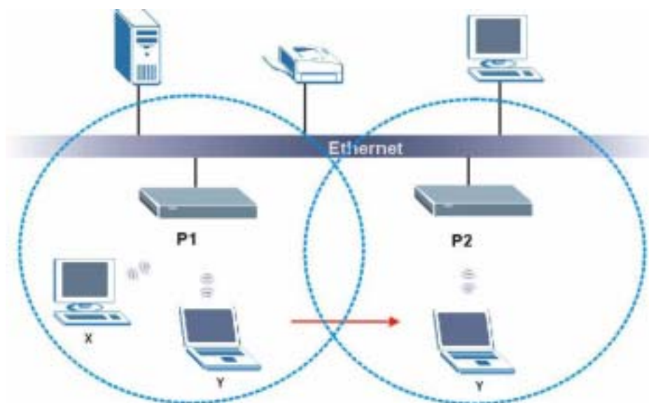
Figure 109 Roaming Example
