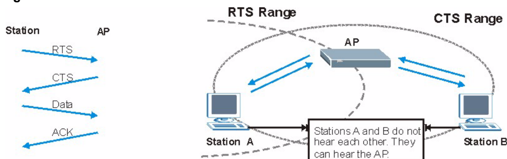
Figure 188 RTS/CTS
