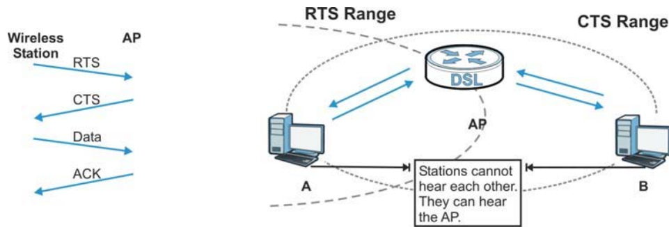
Figure 170 RTS/CTS
