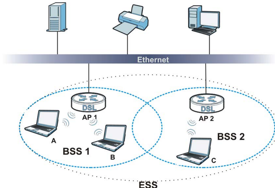
Figure 169 Infrastructure WLAN
