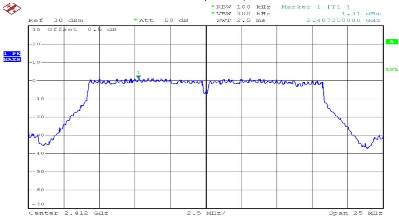
Channel 01 (2412MHz)
