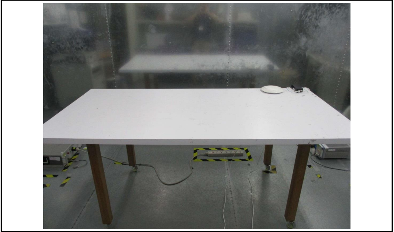
Conducted Emission Test (Model: WAC6103D-I, NAP203)
