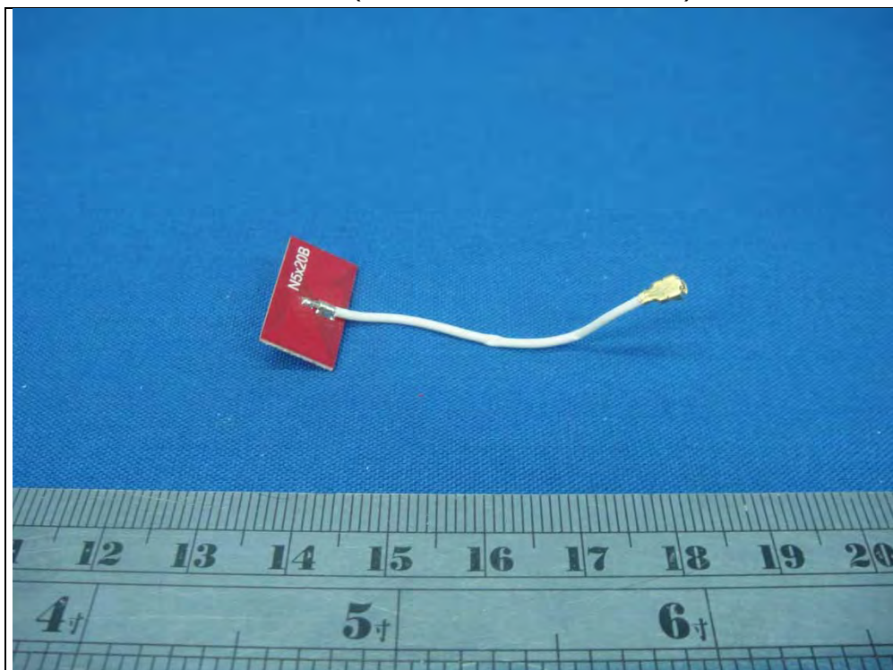
Antenna 3 (P/N: N5X20B-PK1-W50U)
