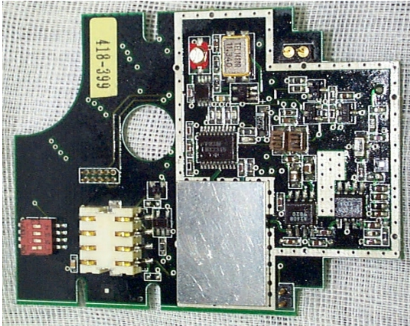
Photo 15. Top View of Transceiver Board with Shield Removed
