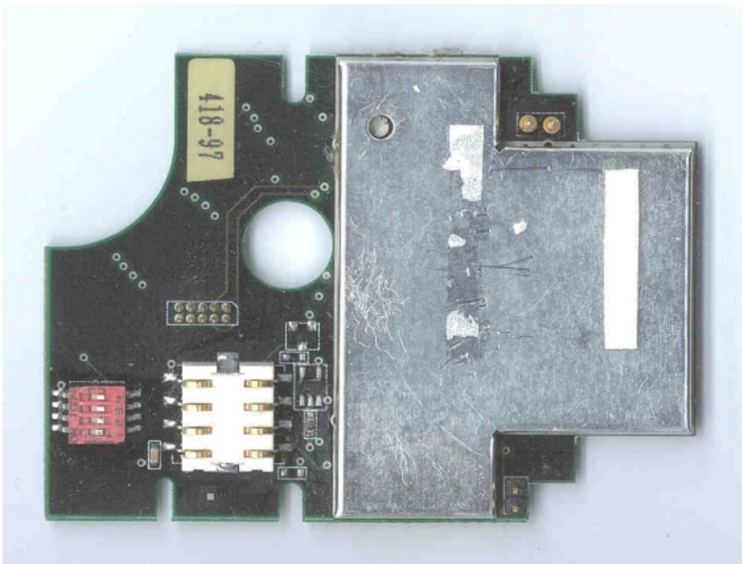
Photo 14. Top View of Transceiver Board with Shield Installed
