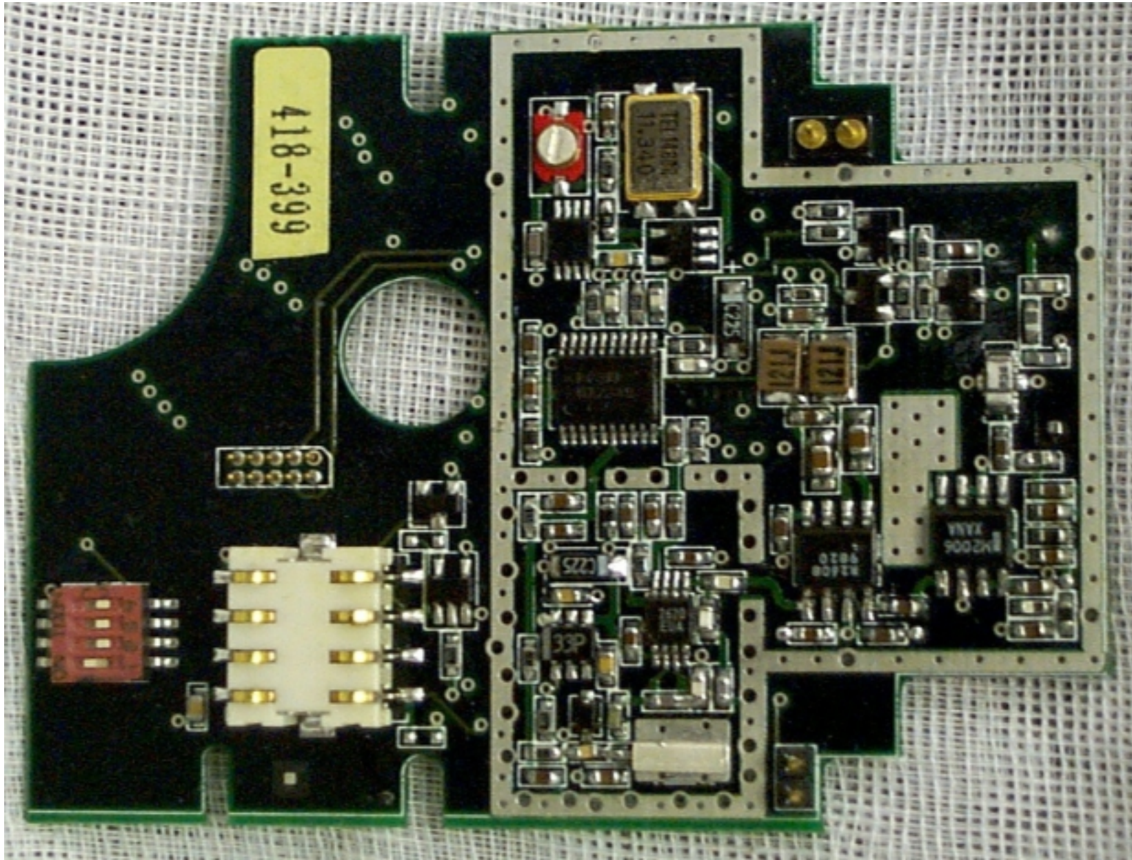
Photo 16. Top View of Transceiver Board with Secondary Shield Removed
