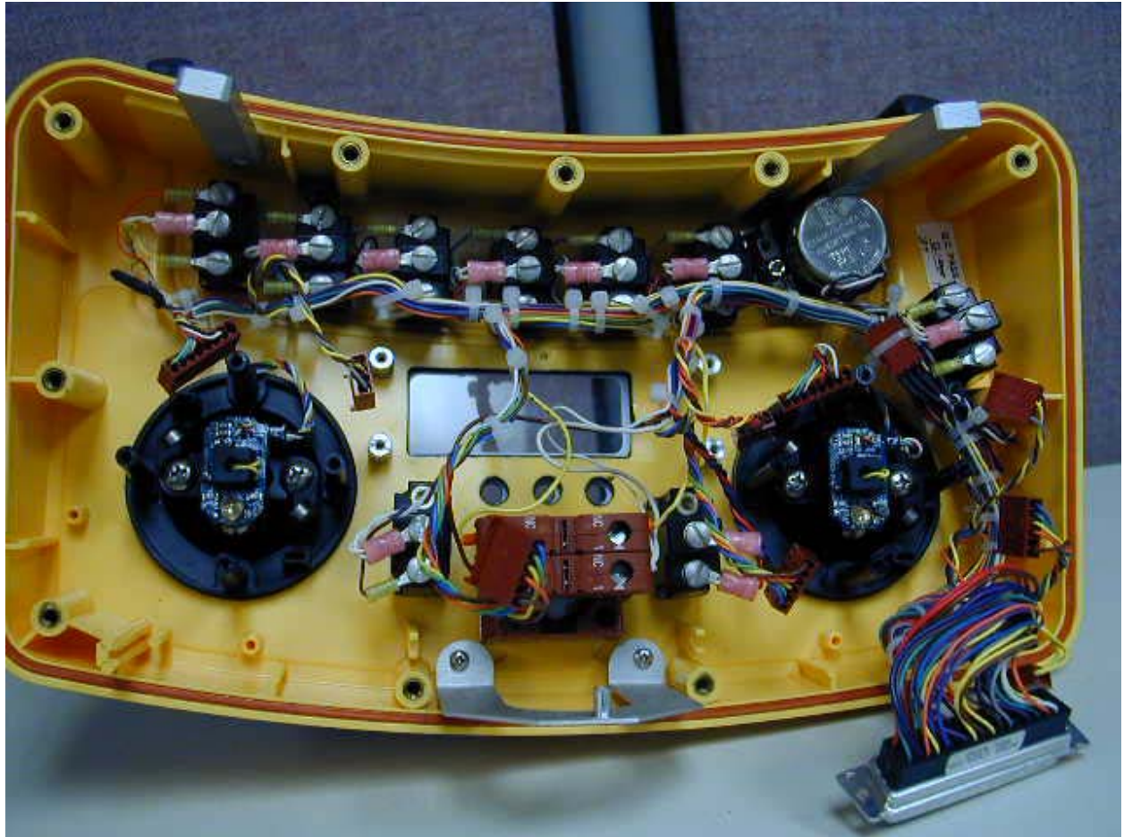
INSIDE WITHOUT BOARDS
