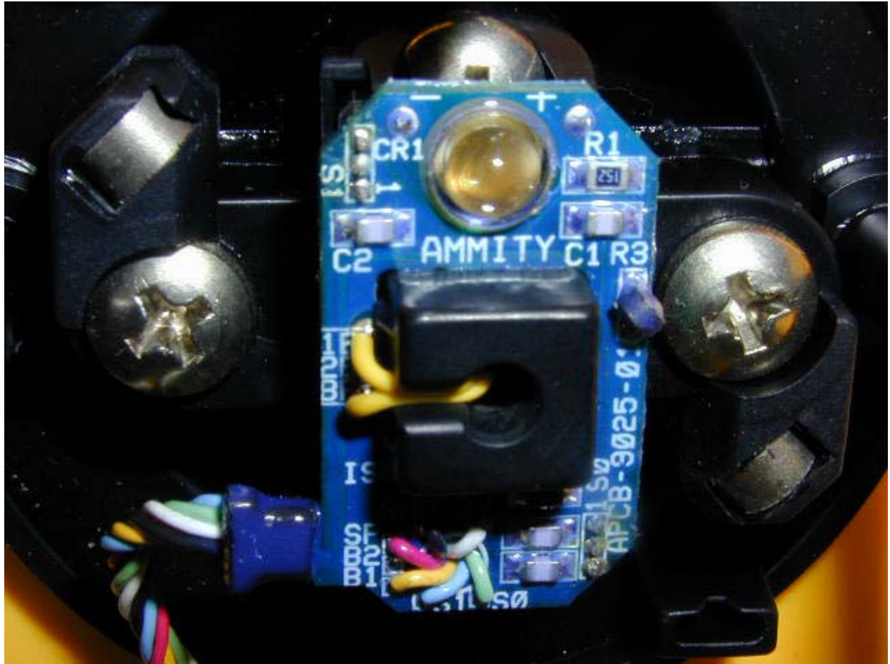
APCB-9025-01 BOARD 2
