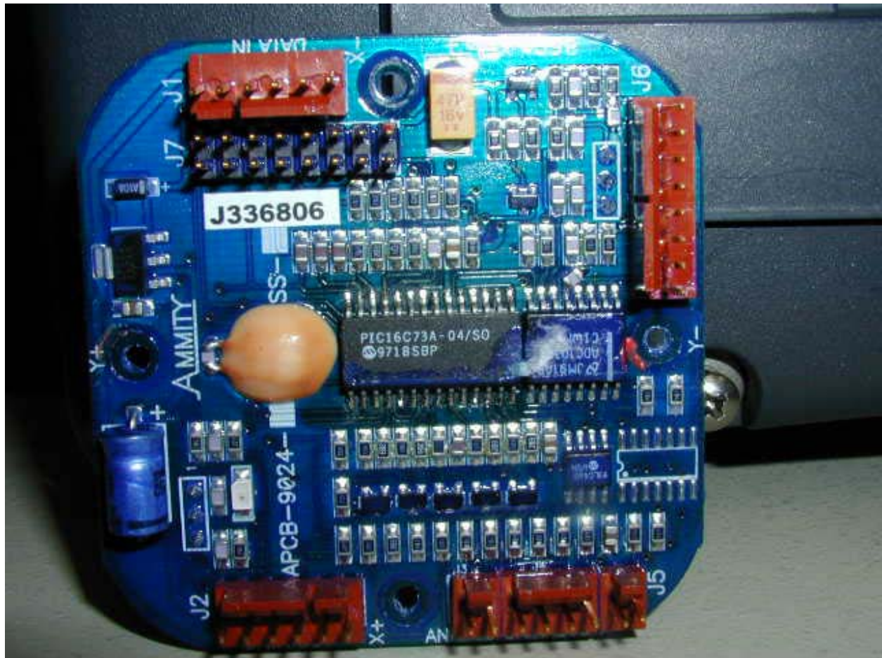
J336806 BOARD TOP
