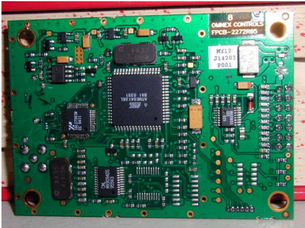
BACK OF BOARD
