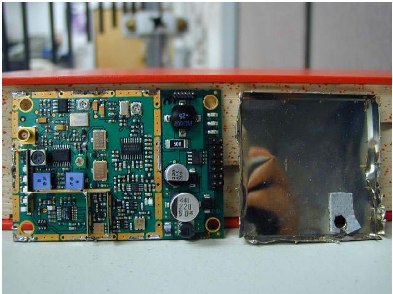
TOP OF BOARD WITH CAN REMOVED
